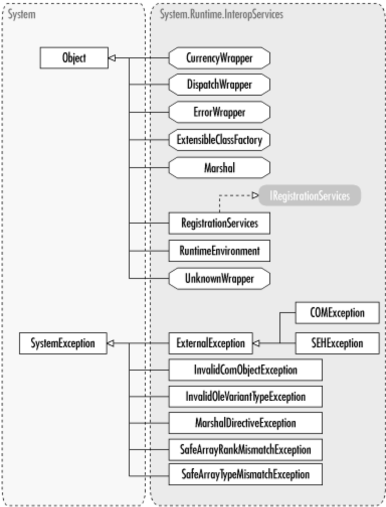
Figure 37-1. The System.Runtime.InteropServices namespace
