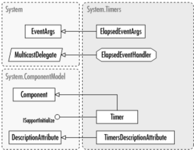
Figure 43-1. The System.Timers namespace
