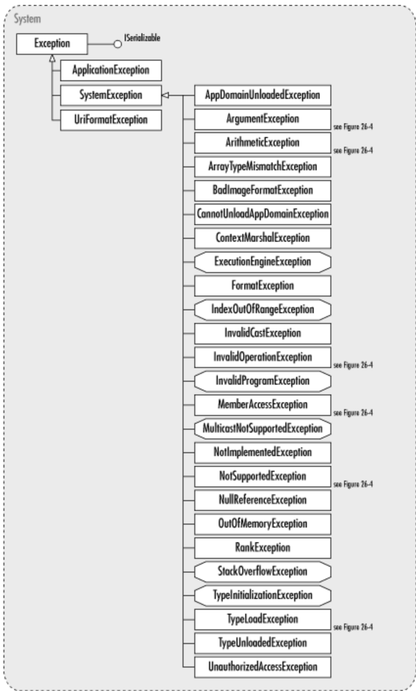
Figure 26-4. Specialized exceptions in the System namespace
