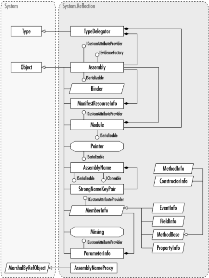
Figure 35-2. Exceptions, delegates, and attributes from System.Reflection
