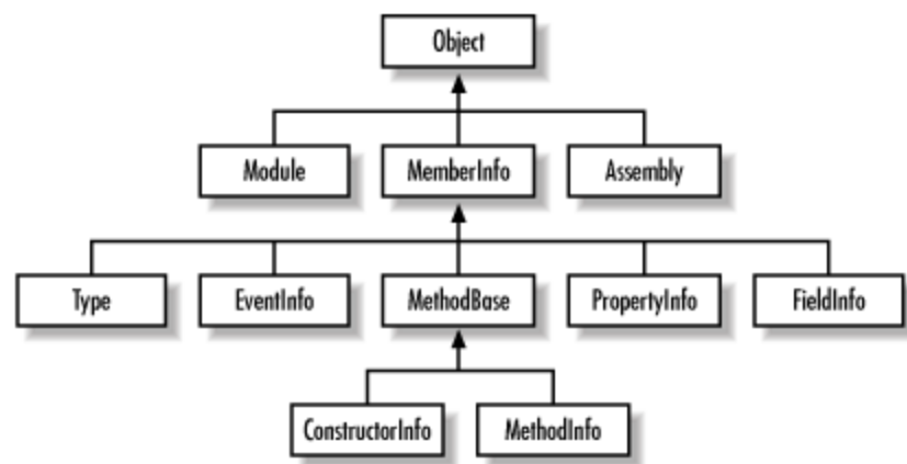
Figure 13-1. Inheritance relationships among the .NET reflection types
