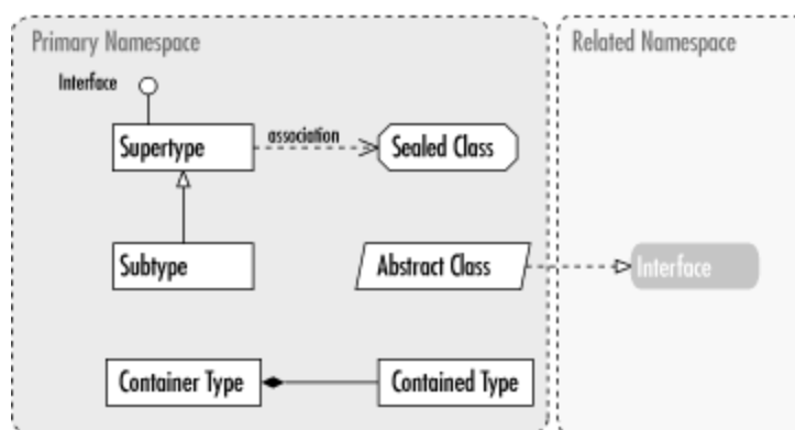
Figure 24-1. Class hierarchy notation
