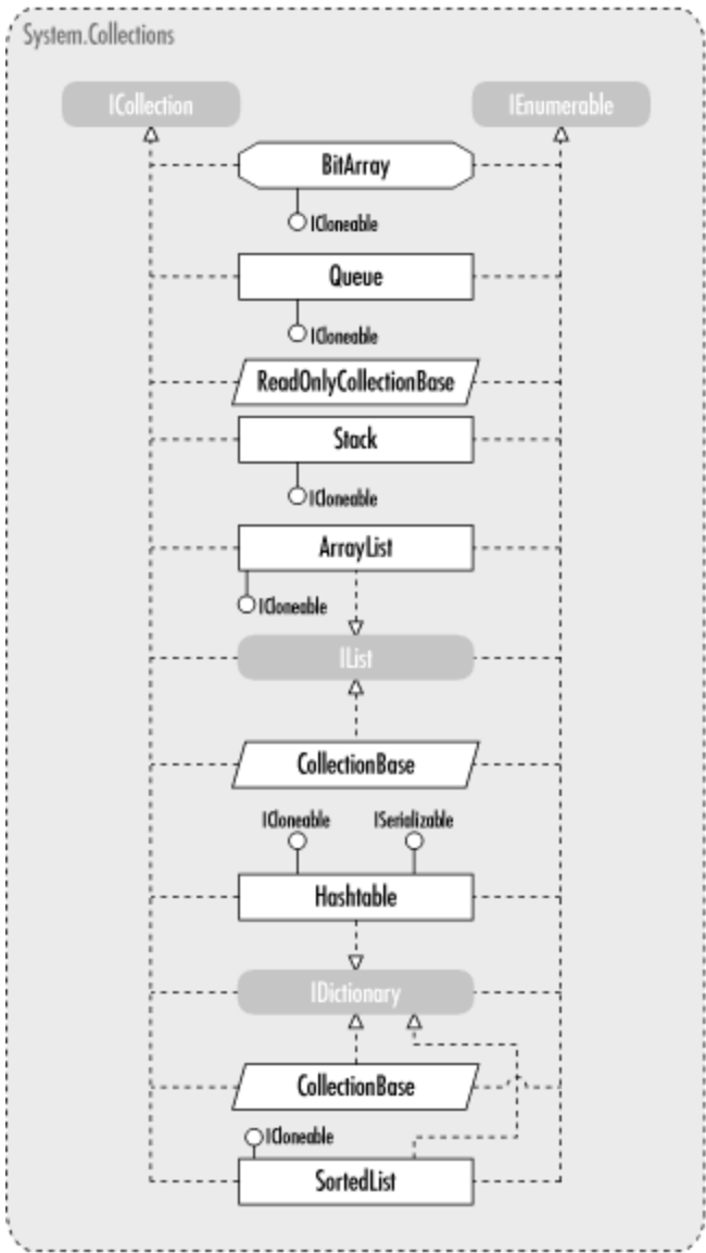
Figure 27-2. More types from the System.Collections namespace
