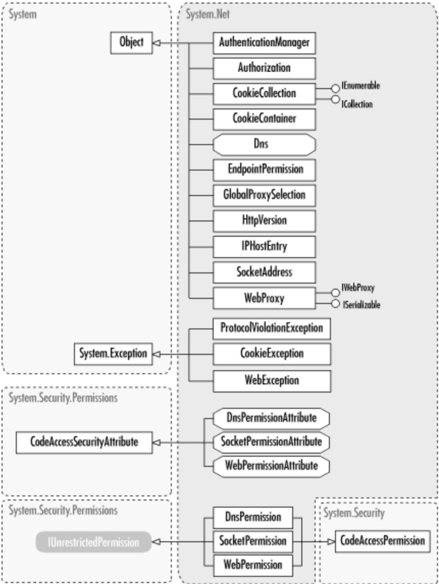
Figure 33-3. Other classes in the System.Net namespace
