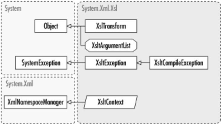
Figure 46-1. The System.Xml.Xsl namespace
