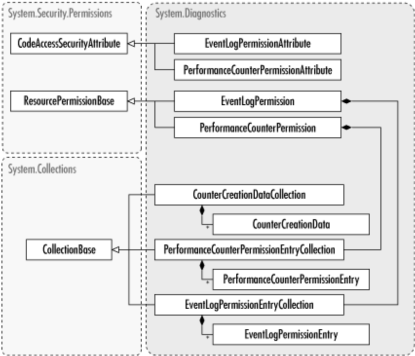
Figure 29-4. CodeAccessSecurityAttributes, collections, and relate
