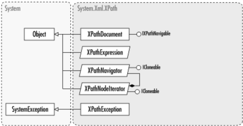
Figure 45-1. The System.Xml.XPath namespace
