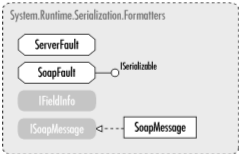
Figure 39-1. The System.Runtime.Serialization.Formatters namespace
