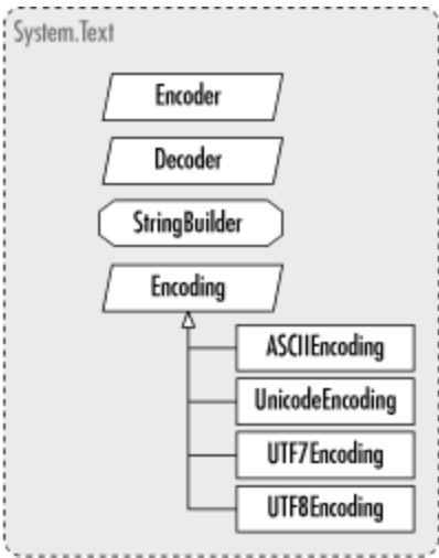
Figure 40-1. The System.Text namespace
