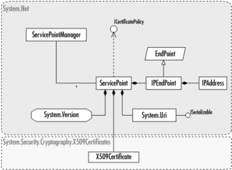
Figure 33-2. Endpoints, service points, and associated types
