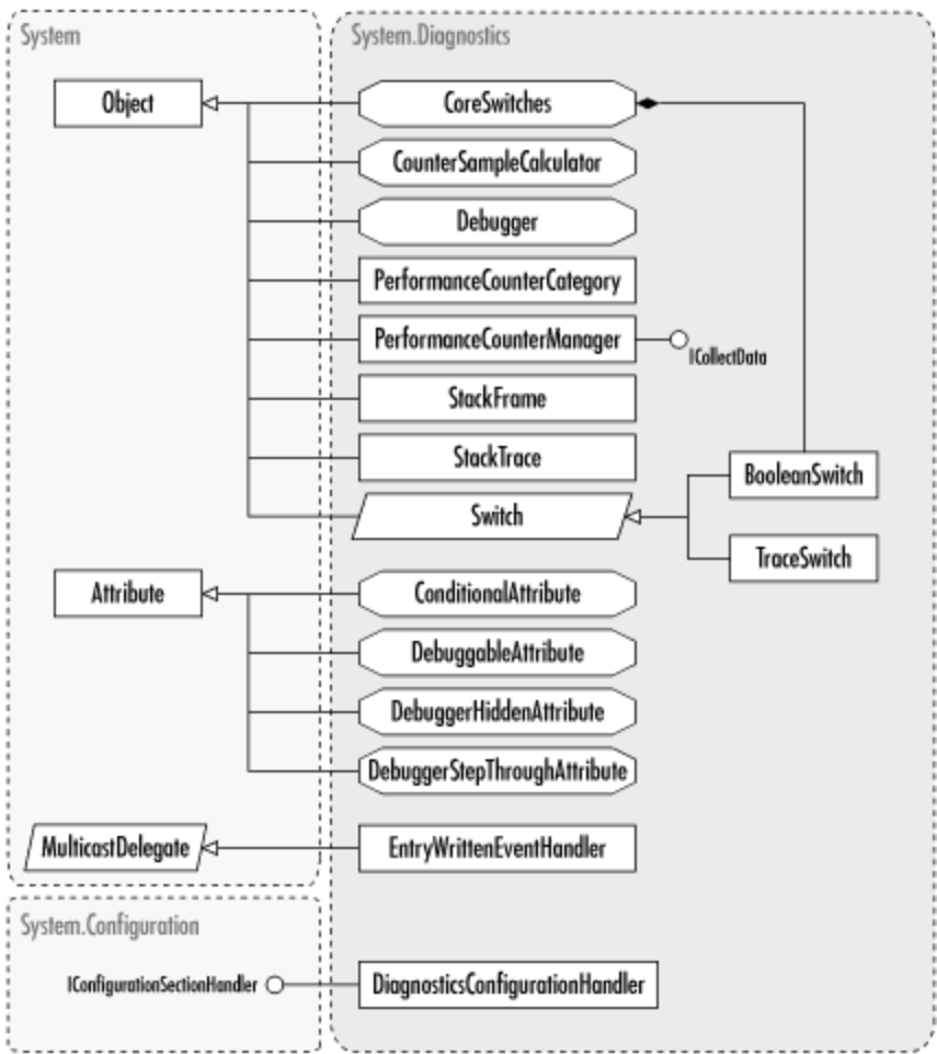
Figure 29-2. More classes from the System.Diagnostics namespace
