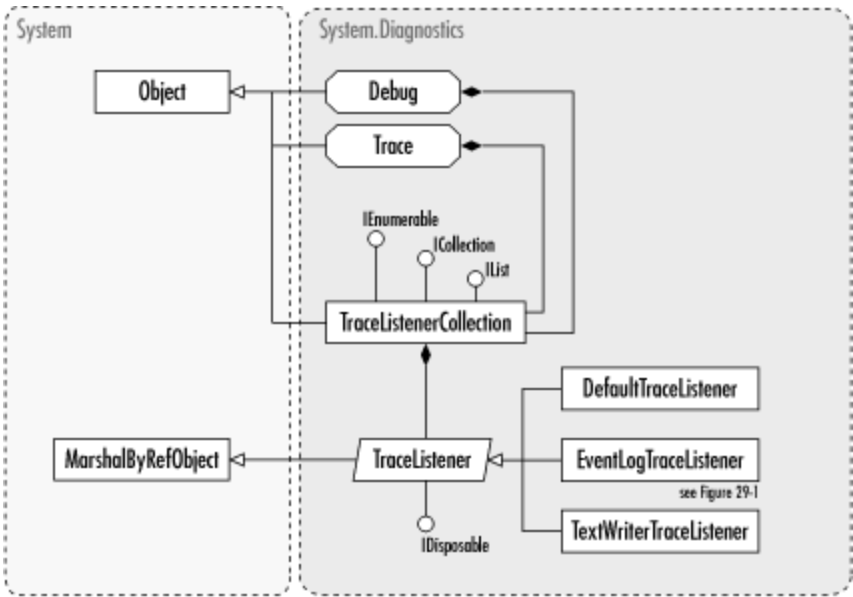
Figure 29-3. TraceListener and related classes
