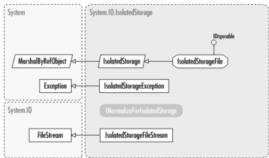
Figure 32-1. The System.IO.IsolatedStorage namespace
