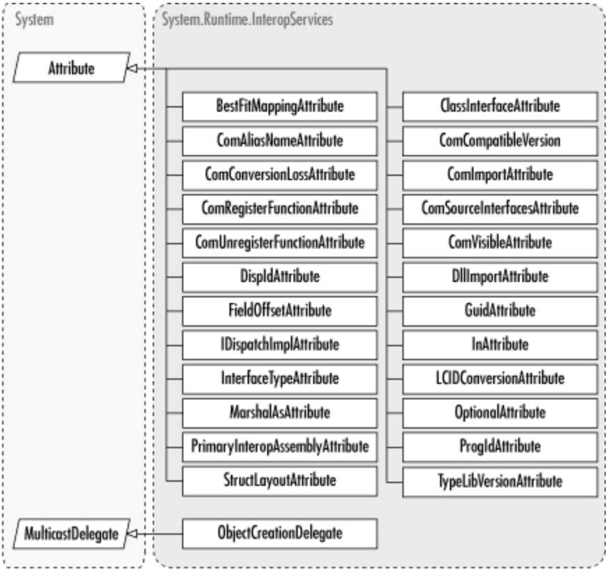
Figure 37-2. Attributes and delegates from System.Runtime.InteropServices
