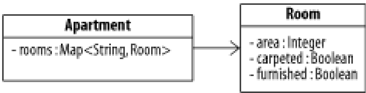
Figure 3-4. Diagram of the Apartment and Room beans
