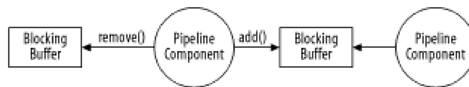
Figure 5-2. Using a BlockingBuffer to create a pipeline
