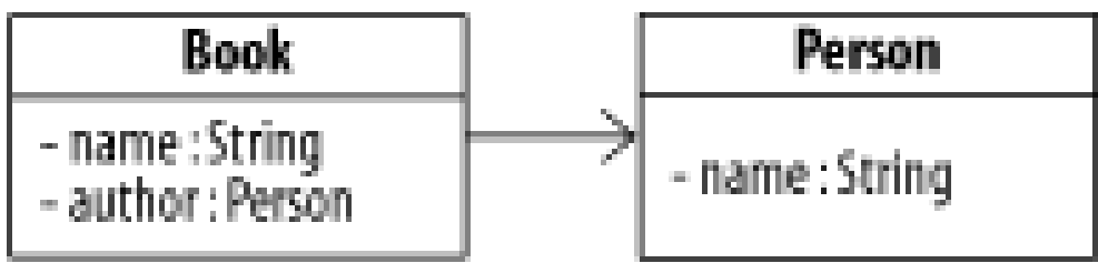
Figure 3-3. Structure of two simple beans: Book and Person
