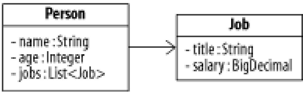
Figure 3-2. Representing a list of Job objects
