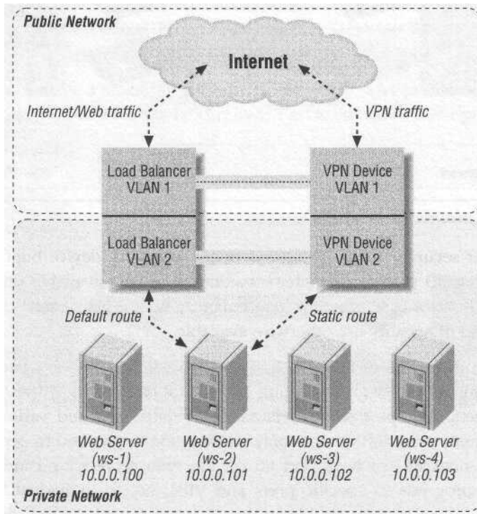
Figure 7-6. VPN devices not in the path of traffic
