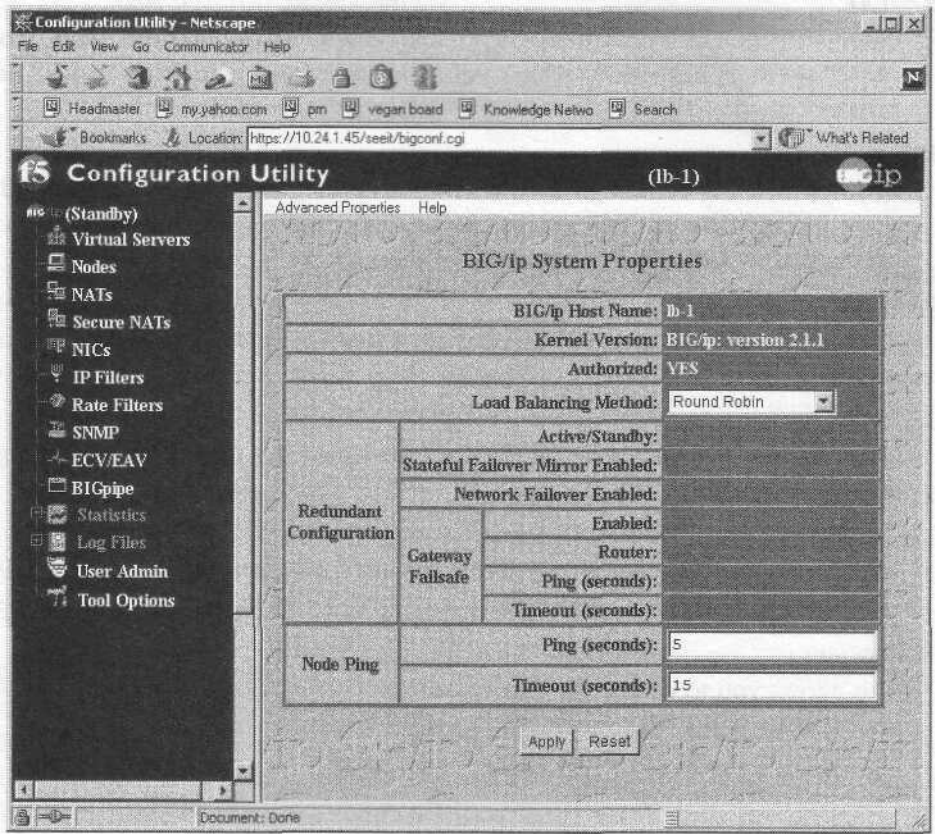
Figure 10-2. Configuration utility menu
