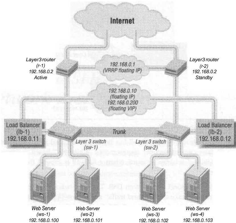
Figure 6-2. Flat-based, route-path, one-armed SLB
