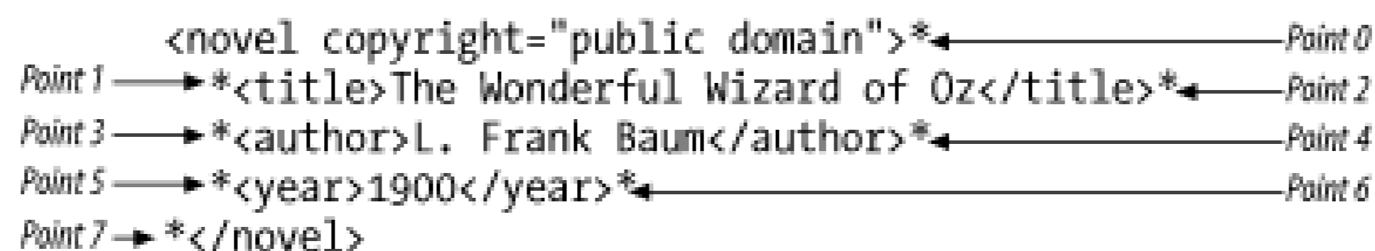
Figure 11-1. The points inside the novel element
