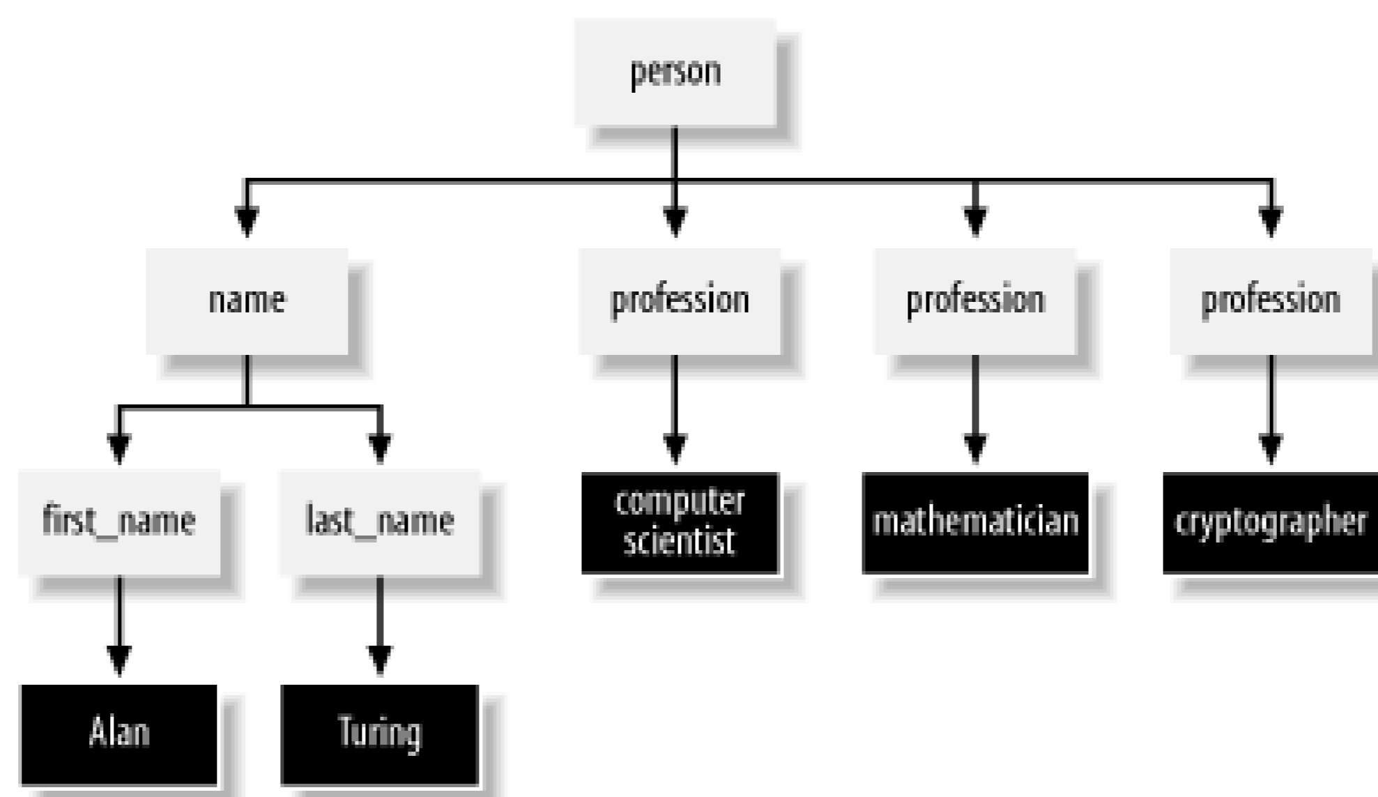
Figure 2-1. A tree diagram for Example 2-2
