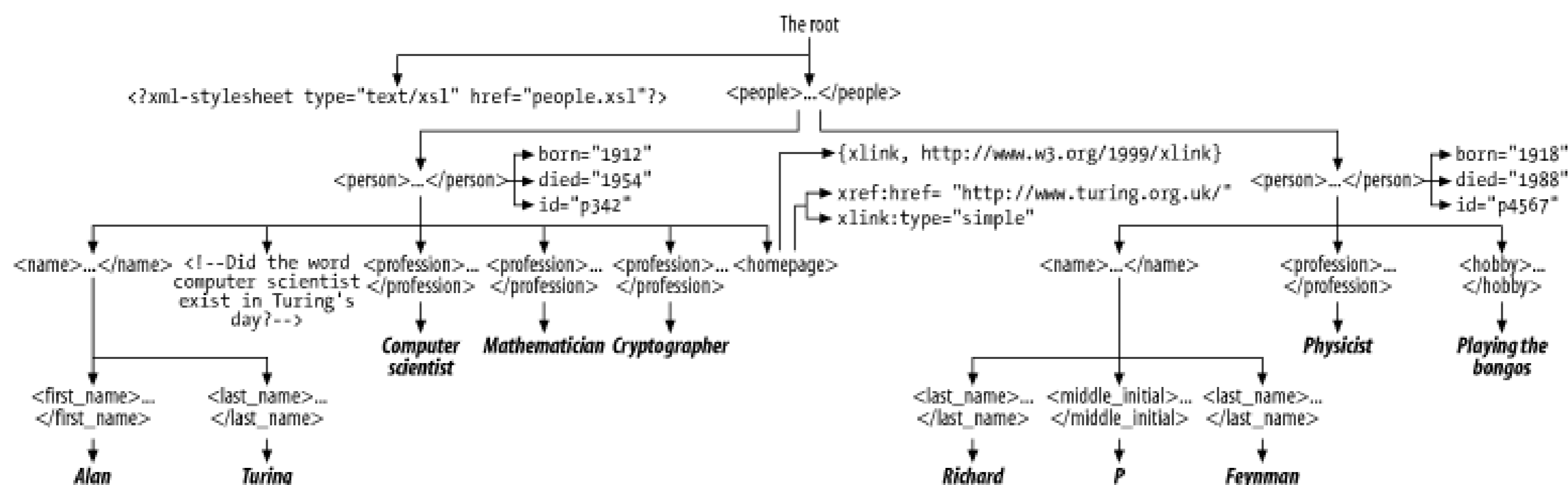
Figure 9-1. The tree structure of Example 9-1
