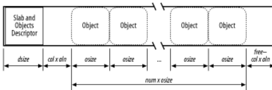
Figure 7-6. Slab with color col and alignment alm
