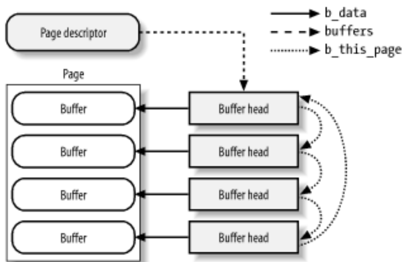
Figure 14-1. A buffer page including four buffers and their buffer heads
