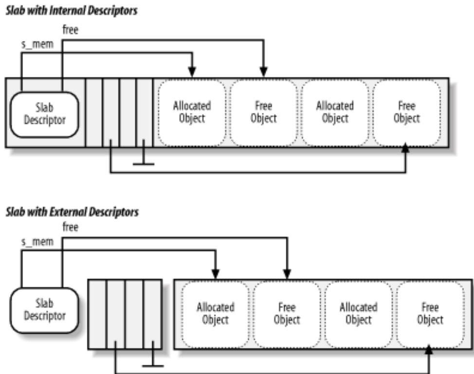
Figure 7-3. Relationships between slab and object descriptors
