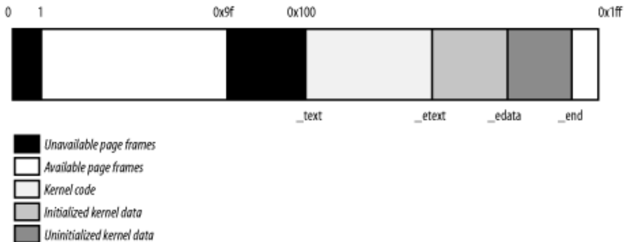
Figure 2-12. The first 512 page frames (2 MB) in Linux 2.4
