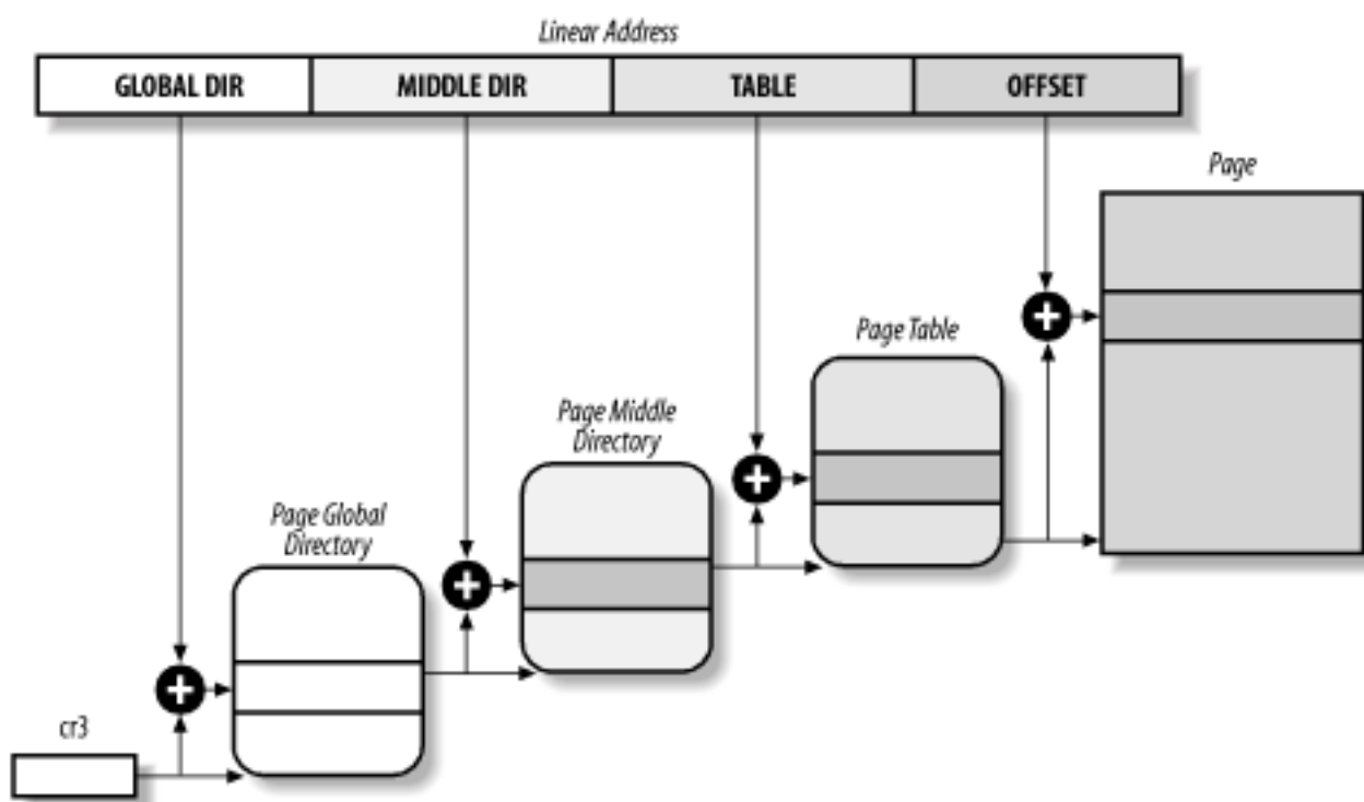
Figure 2-11. The Linux paging model
