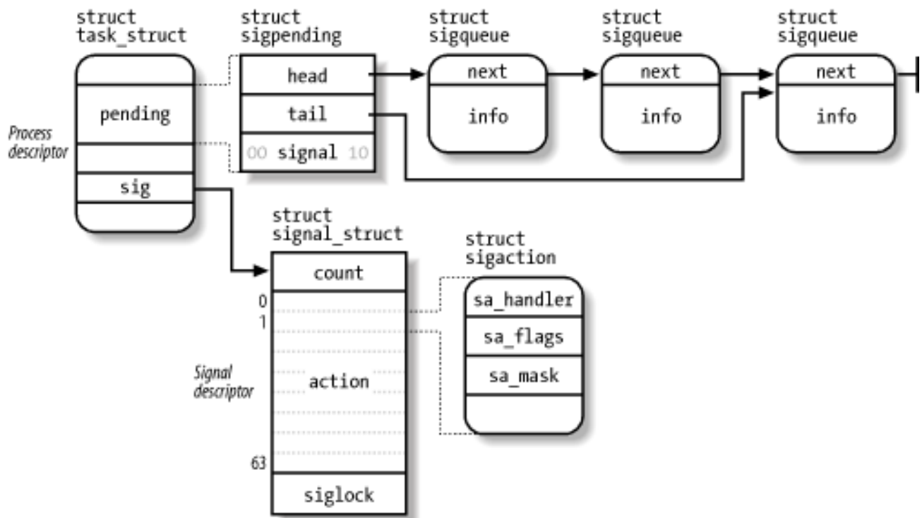
Figure 10-1. The most significant data structures related to signal handling
