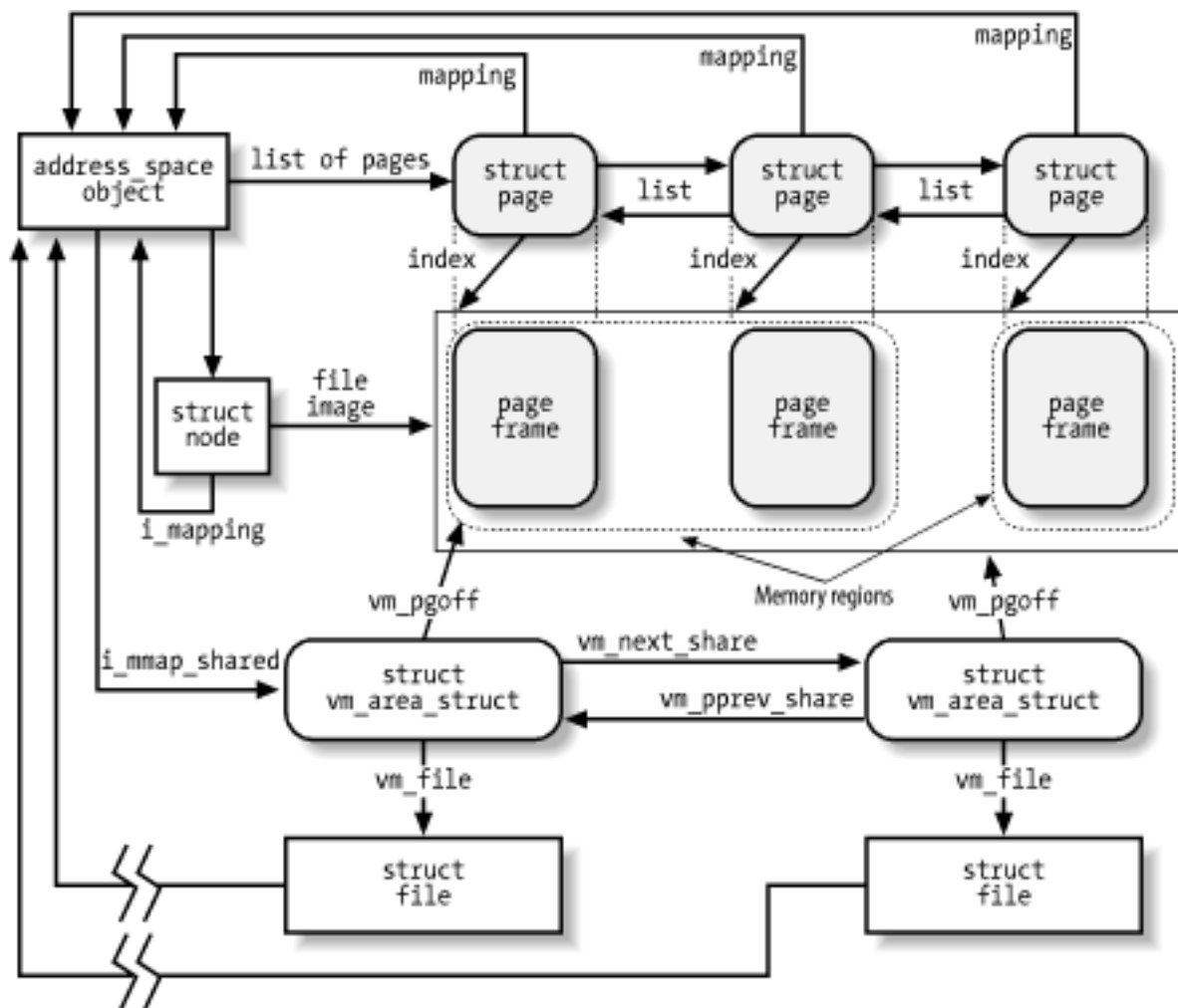
Figure 15-4. Data structures for file memory mapping
