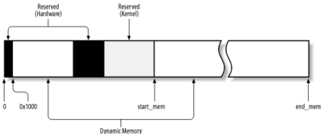
Figure 7-1. Memory layout
