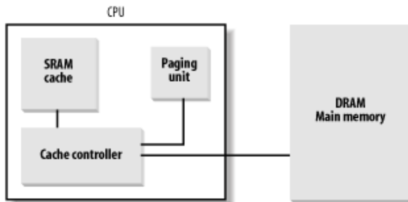
Figure 2-9. Processor hardware cache
