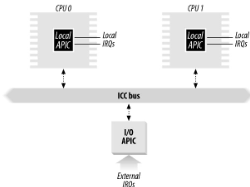
Figure 4-1. Multi-APIC system
