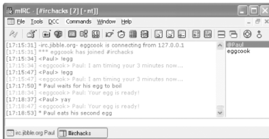
Figure 9-2. The working egg timer
