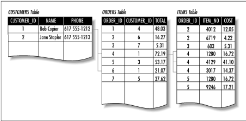
Figure 8–1. Three related tables
