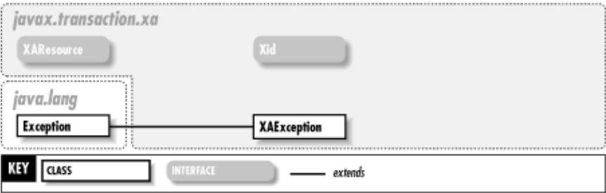
Figure 29–1. The javax.transaction.xa package
