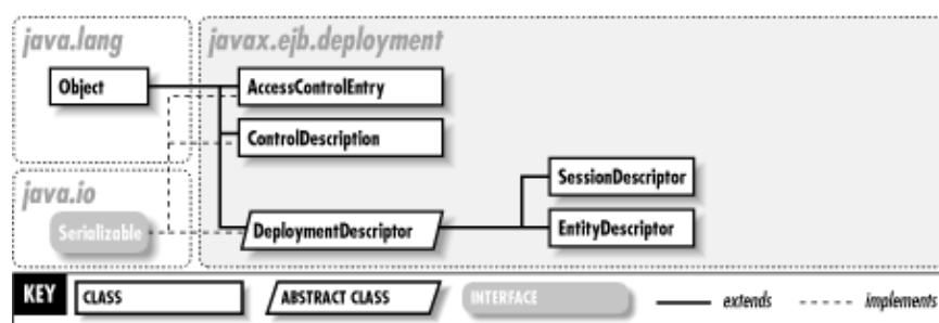
Figure 20–1. The javax.ejb.deployment package class hierarchy
