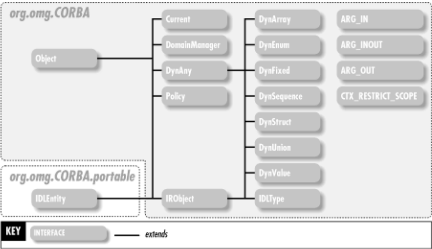
Figure 30–1. The interfaces in the org.omg.CORBA package
