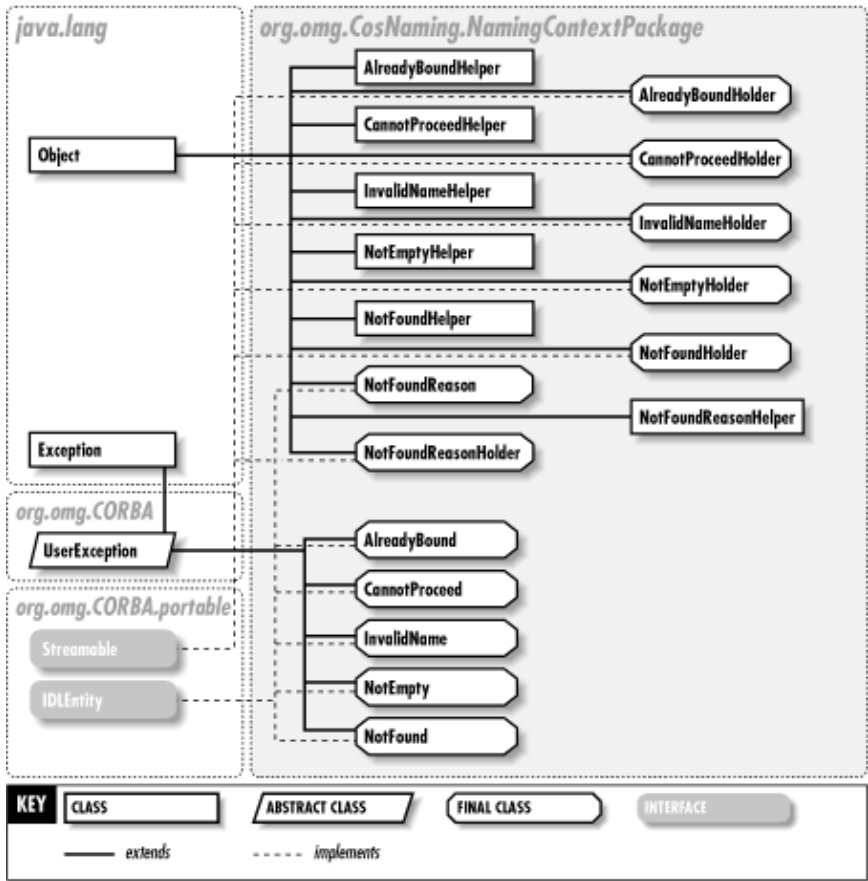
Figure 36–1. The org.omg.CosNaming.NamingContextPackage package
