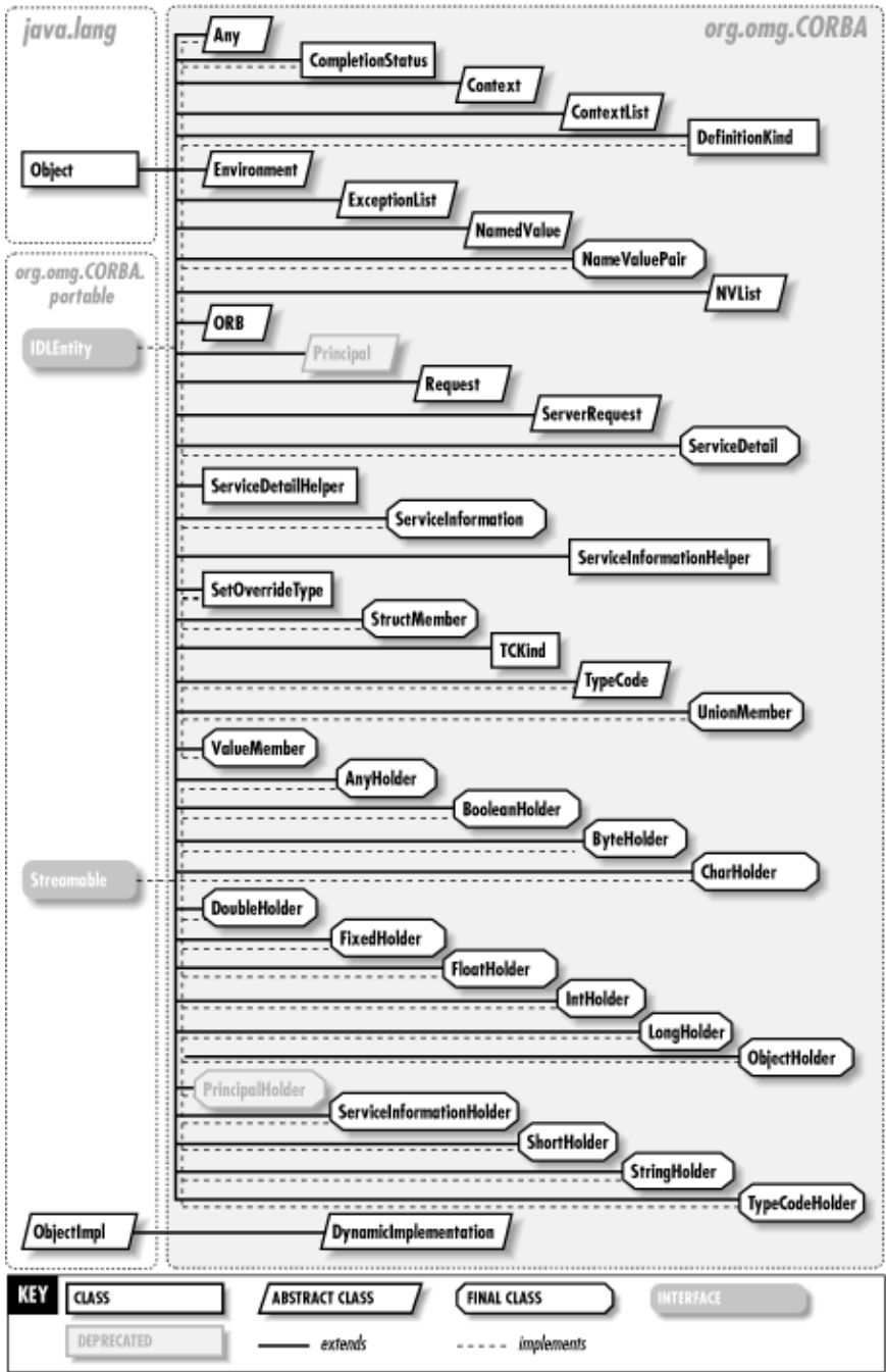
Figure 30–2. The classes in the org.omg.CORBA package
