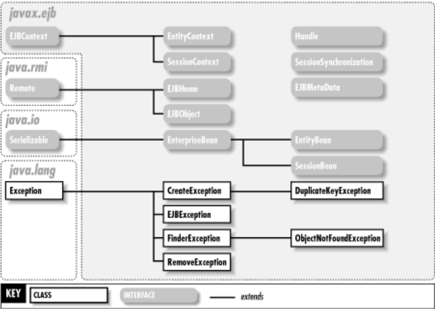
Figure 19-1. The javax.ejb package
