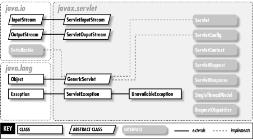
Figure 25–1. The javax.servlet package
