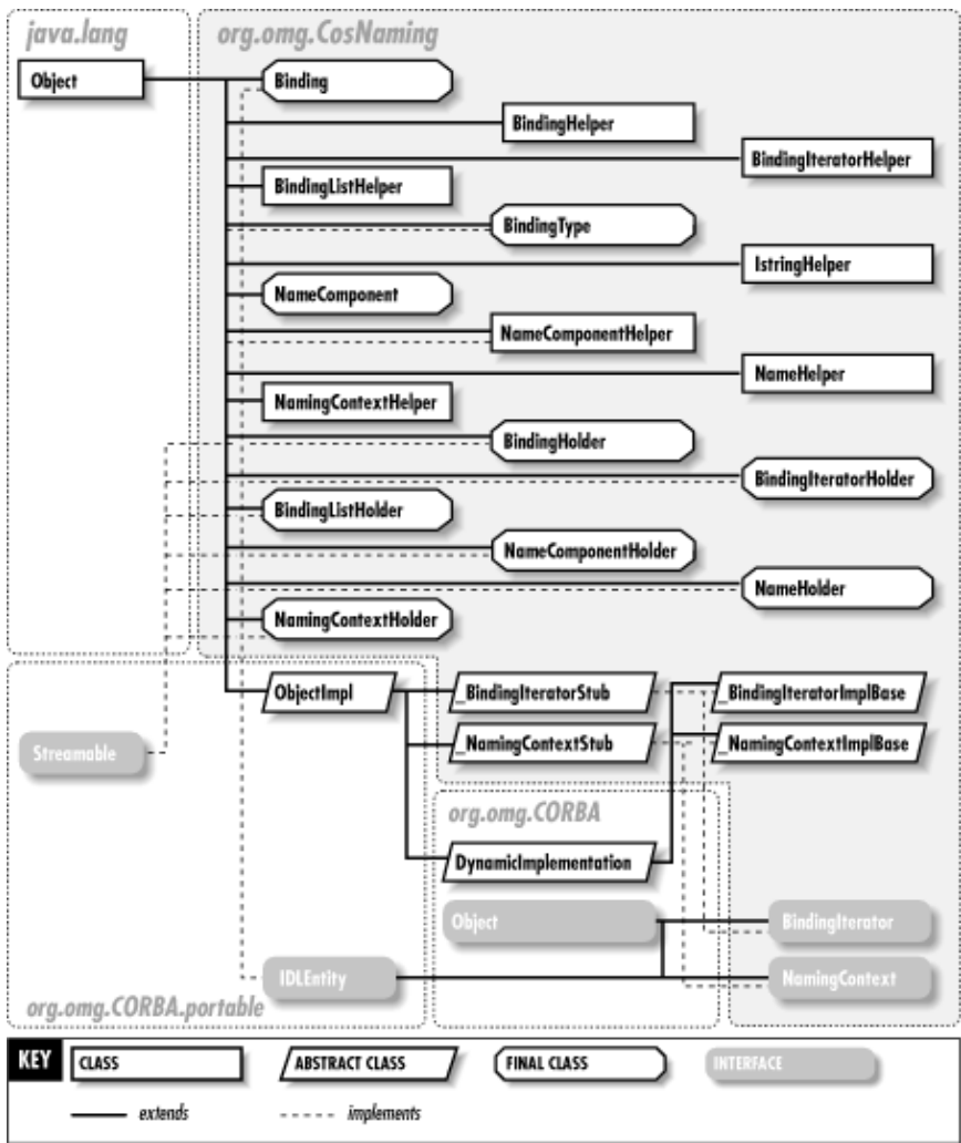
Figure 35–1. The org.omg.CosNaming package
