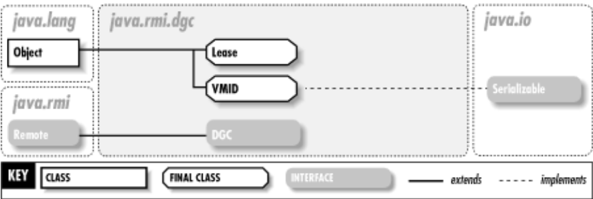
Figure 15–1. The java.dgc.activation package
