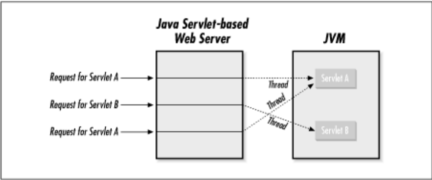
Figure 5–1. The servlet life cycle
