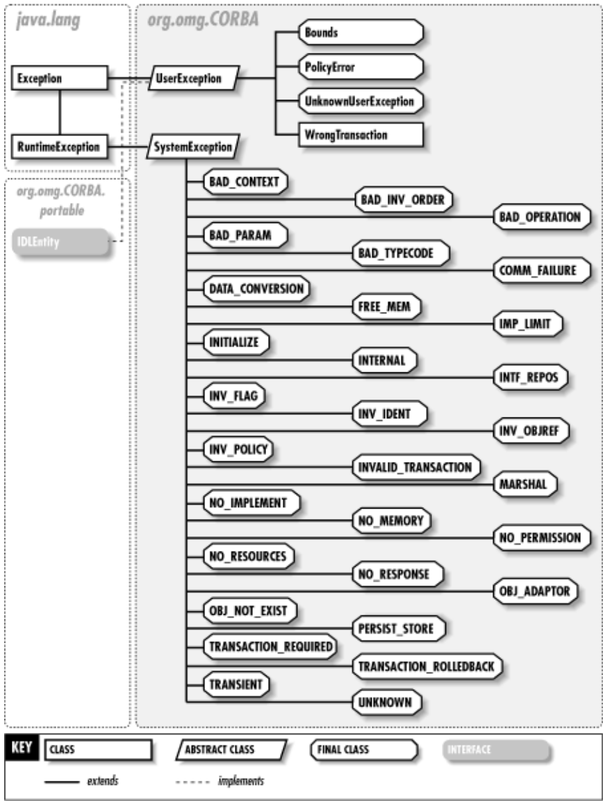
Figure 30–3. The exceptions in the org.omg.CORBA package
