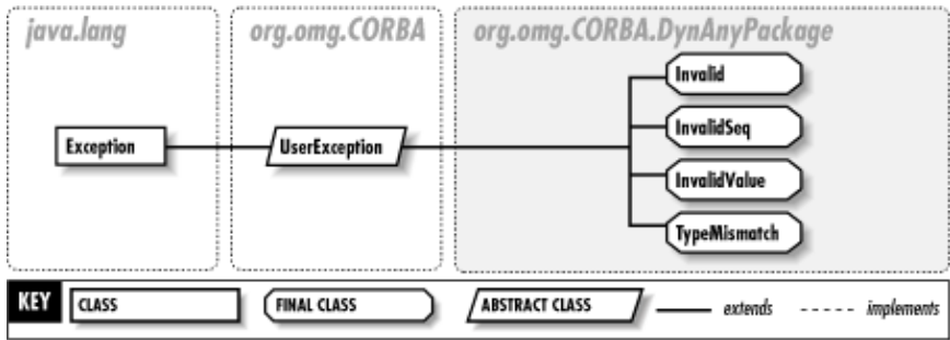
Figure 31–1. The org.omg.CORBA.DynAnyPackage package
