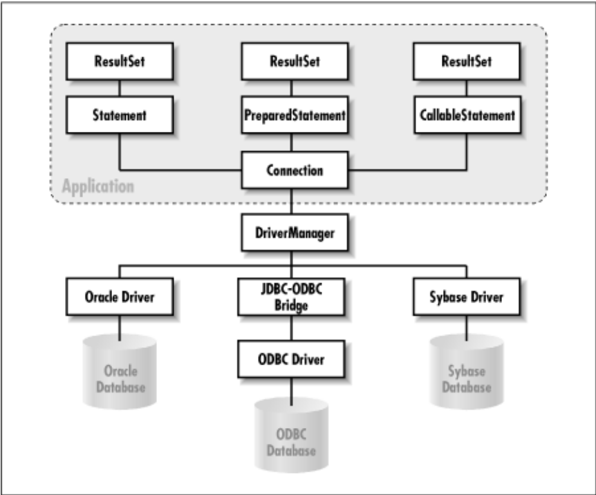
Figure 2–1. JDBC–database interaction
