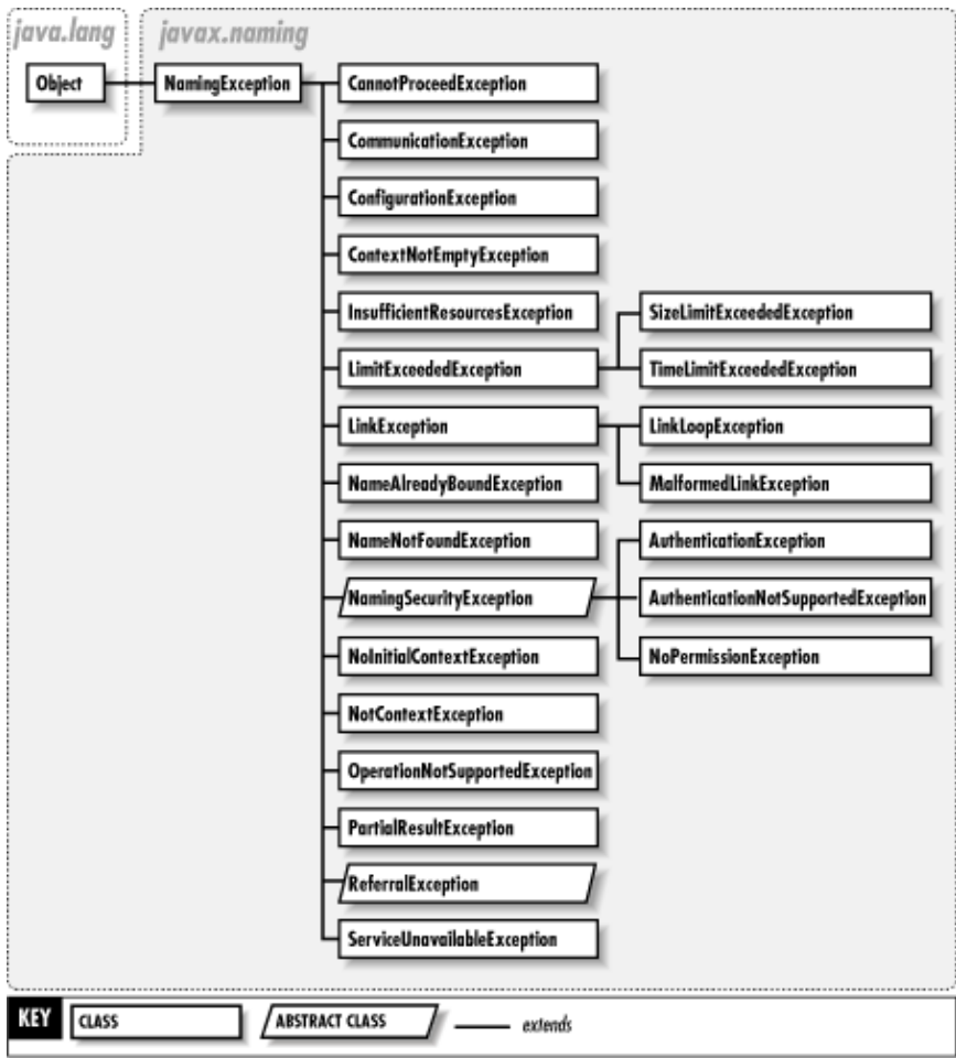
Figure 22–2. The exception hierarchy of the javax.naming package
