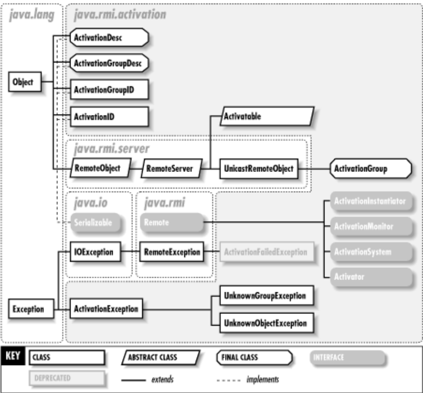
Figure 14–1. The java.rmi.activation package
