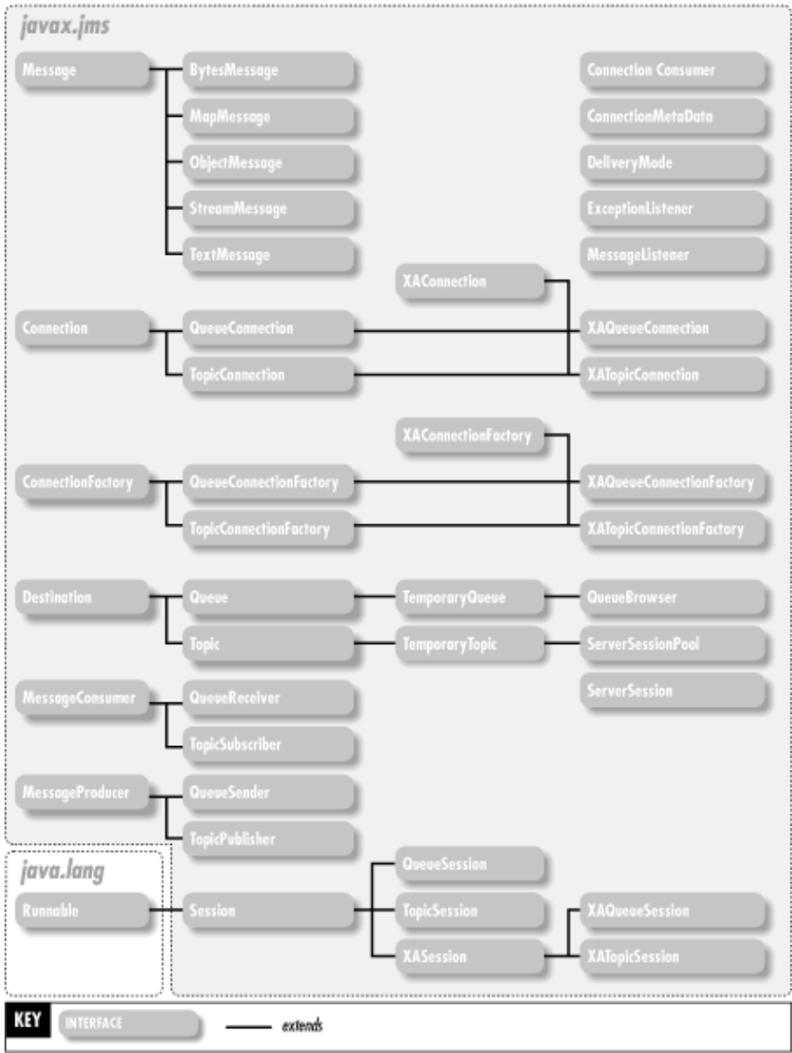
Figure 21–1. The interfaces of the javax.jms package
