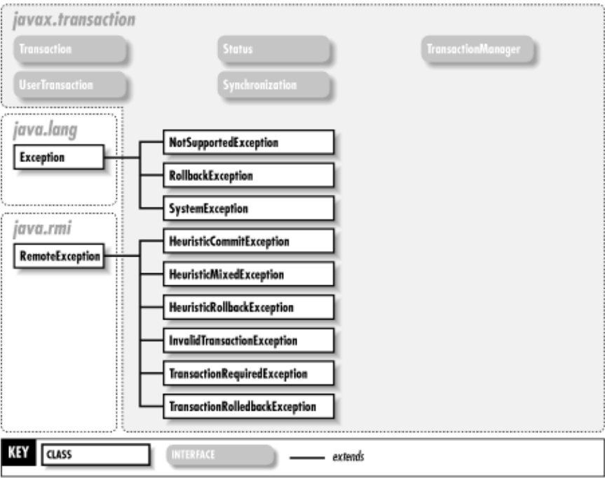
Figure 28–1. The javax.transaction package
