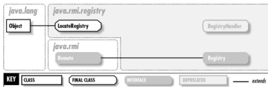
Figure 16–1. The java.rmi.registry package
