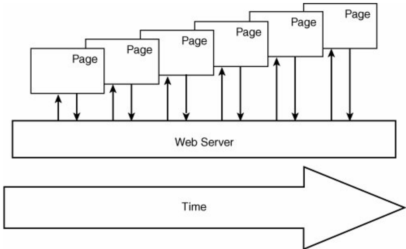
Figure 8-1. The traditional unload/reload cycle
