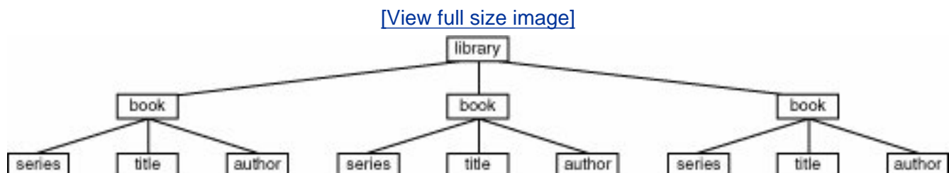
Figure 6-1. An XML document as a tree
