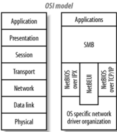
Figure 13-1. OSI model depicting relationship of SMB and other protocols
