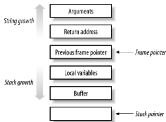
Figure 5-4. Representation of stack structure after a function call
