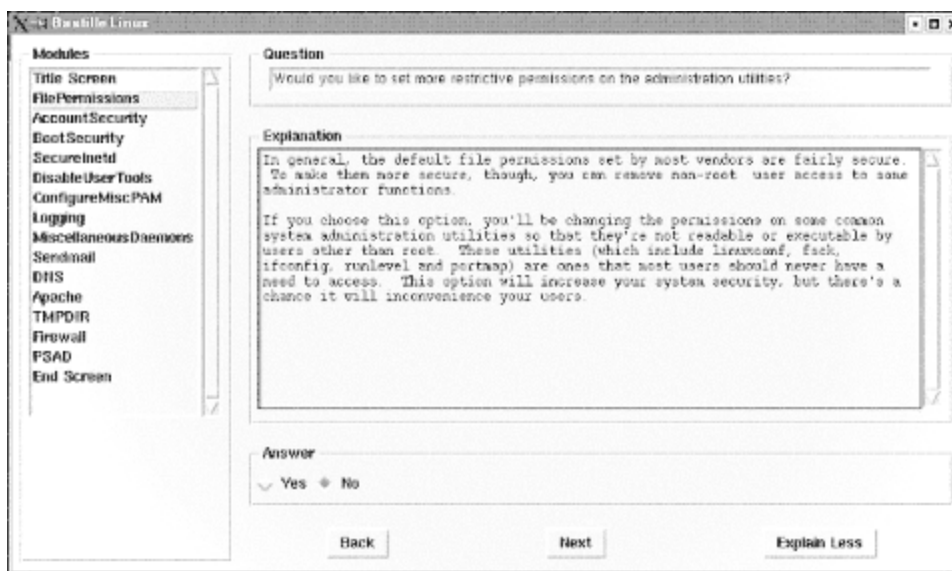
Figure 11-1. An example Bastille screen
