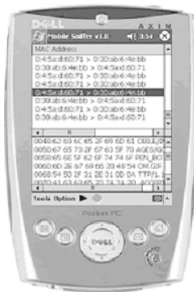
Figure 17-2. Using the free Airscanner Mobile Sniffer to perform wireless sniffing
