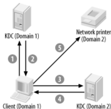
Figure 14-2. Cross-domain Kerberos authentication
