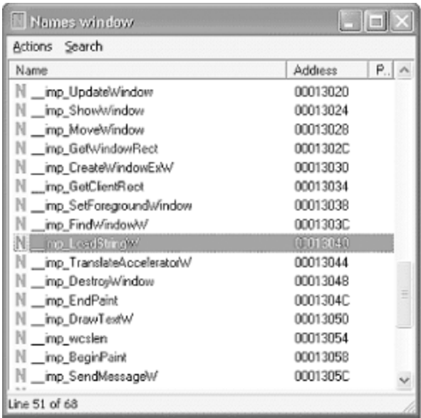
Figure 4-4. Names window in IDA, listing the CE functions used
