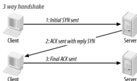
Figure 6-4. TCP / IP handshake
