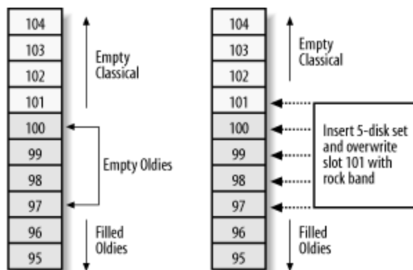
Figure 5-3. A sample buffer overflow
