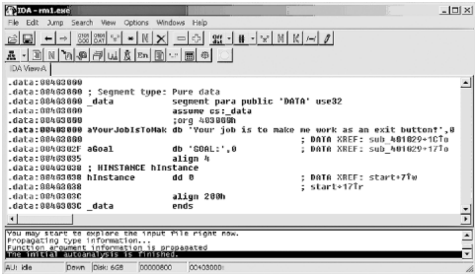
Figure 2-14. Using strings to find target code in the disassembly
