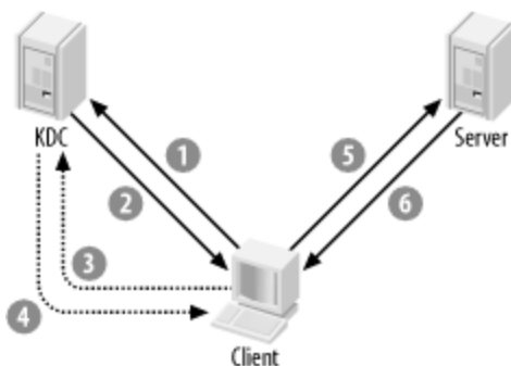
Figure 14-1. The steps of Kerberos authentication
