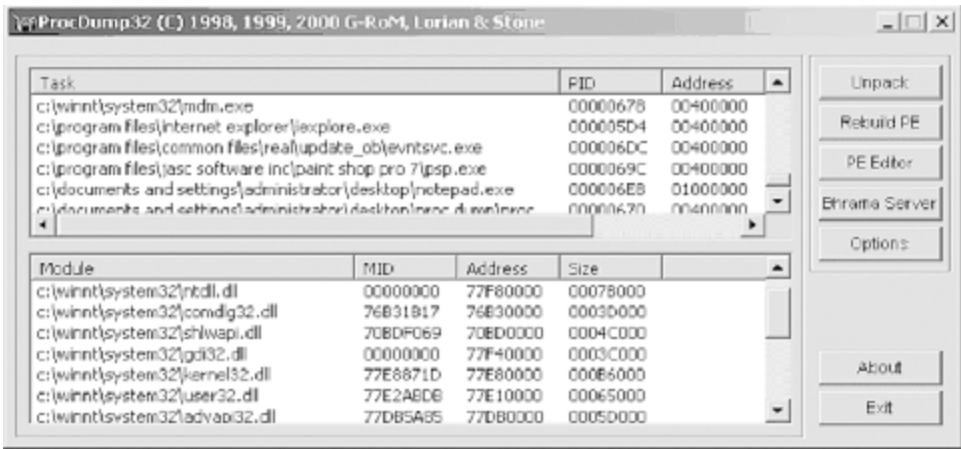
Figure 2-9. Using ProcDump to unpack a compressed program
