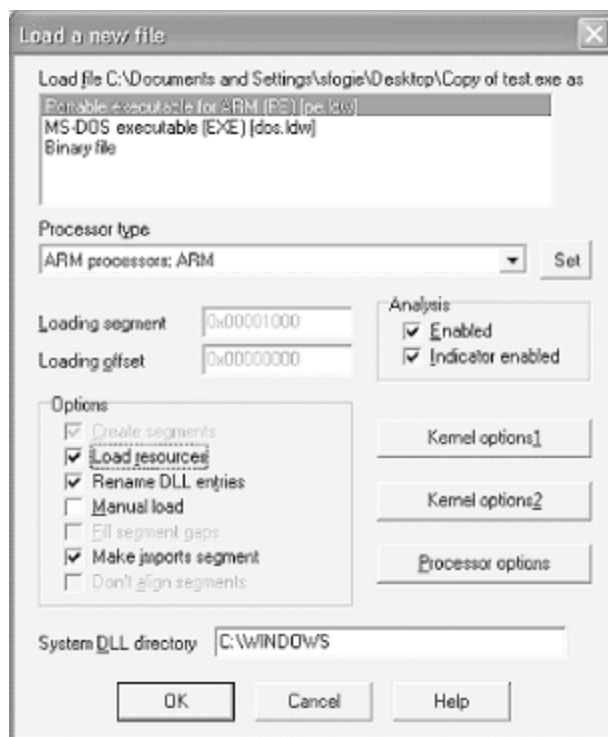
Figure 4-6. IDA Pro startup configuration for test.exe
