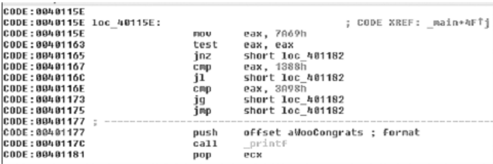
Figure 5-7. Screenshot of target code in IDA Pro
