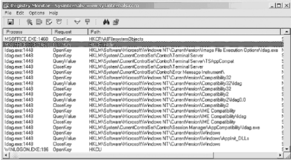
Figure 2-7. Using regmon to trace hidden registry calls
