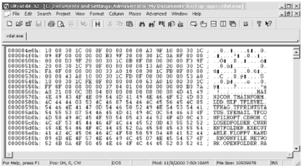
Figure 2-1. For opcode patching, we recommend UltraEdit, an advanced Windows hex editor
