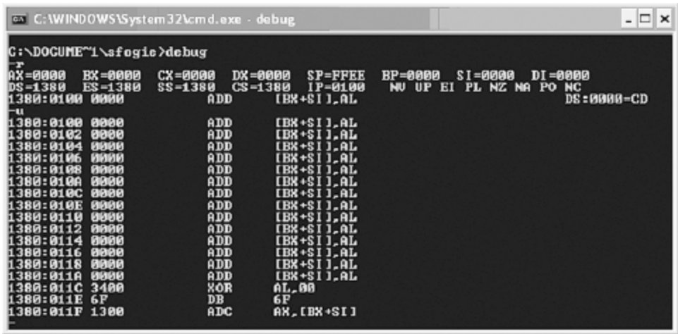
Figure 1-1. Example registers on an x86 processor shown using the debug -r command on Windows XP
