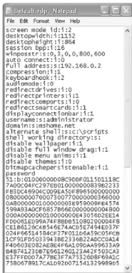
Figure 13-6. Inside a saved *.rdp file
