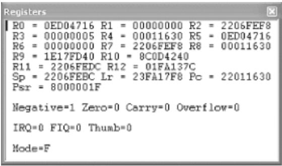
Figure 4-1. MVT illustrating the registers
