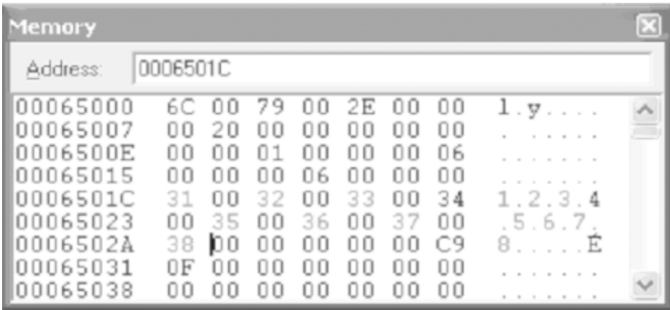
Figure 4-17. Using the Memory window to update values
