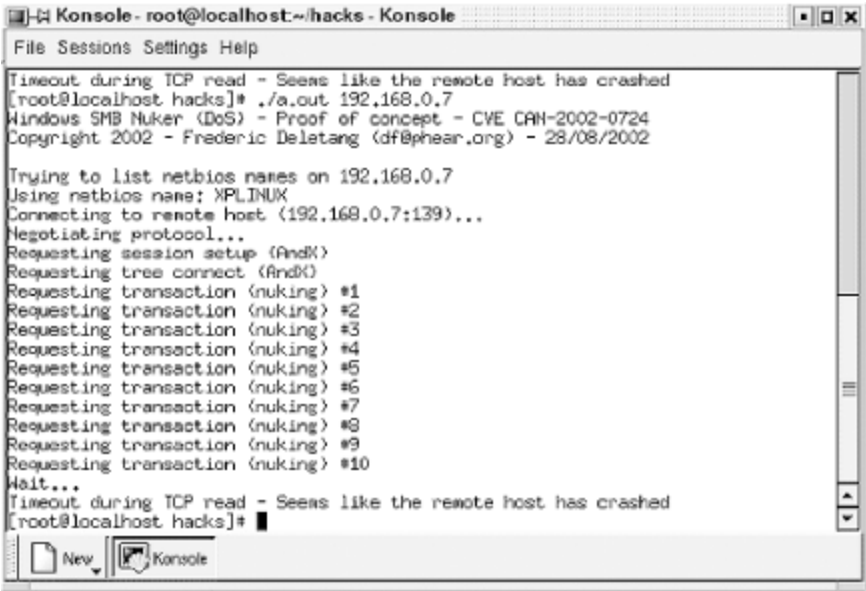
Figure 13-3. smbnuke successfully testing Windows XP box
