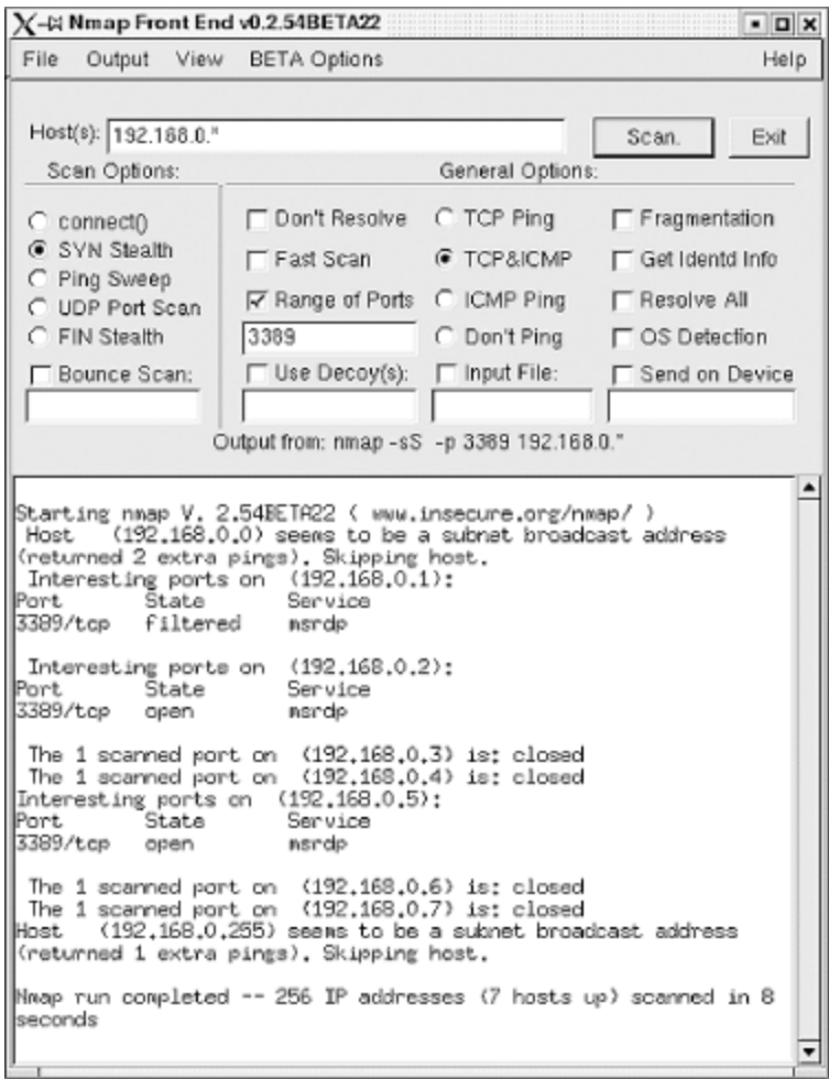
Figure 13-5. Nmap port scan for computers running Remote Desktop service
