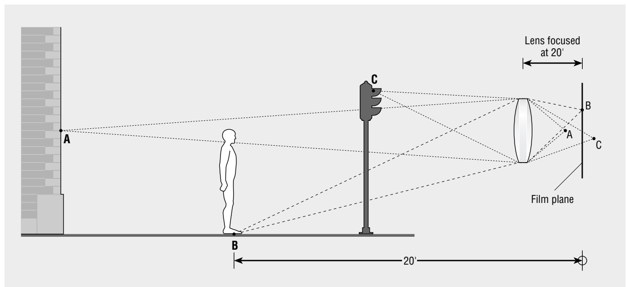
Single-element lens
