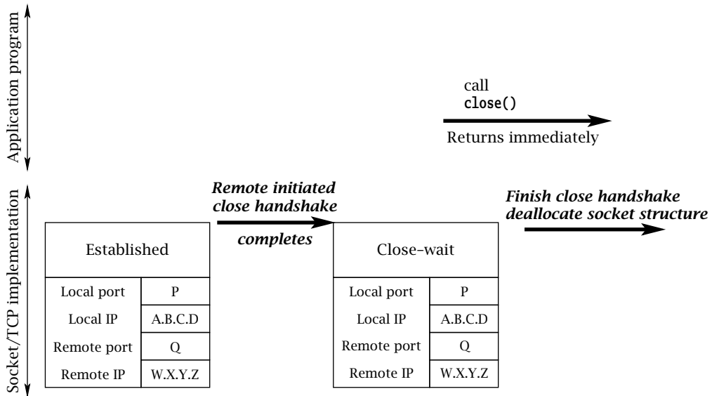
Figure 7.11: Closing after the other end closes.
