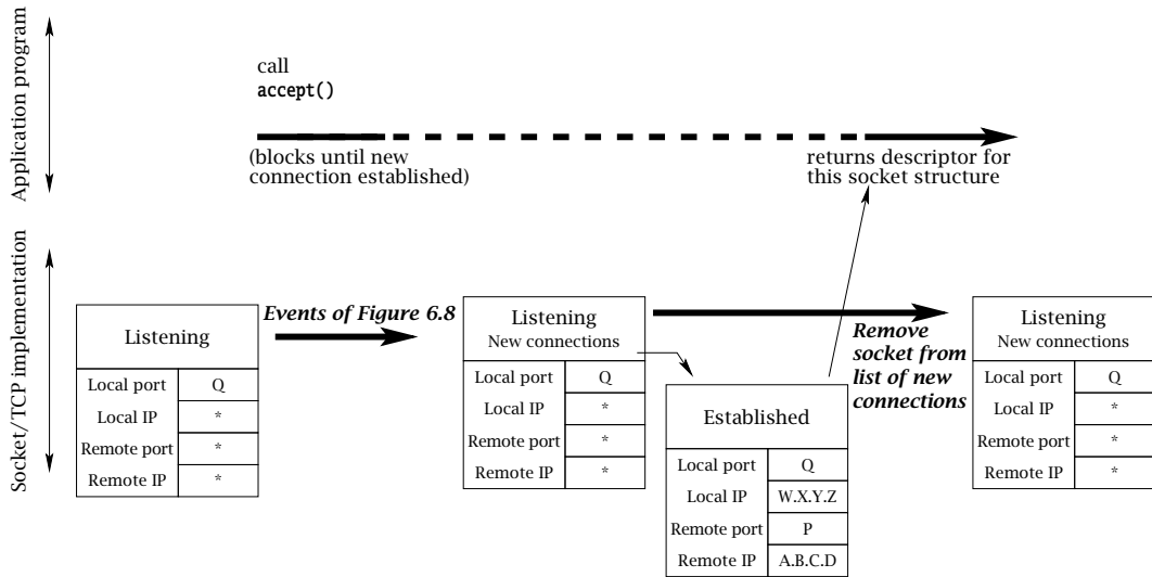
Figure 7.9: accept().
