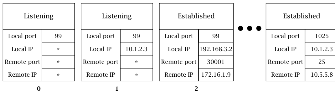
Figure 7.12: Demultiplexing with multiple matching sockets.
