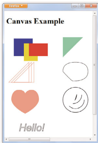
FIGURE 2.8 Drawing text.
