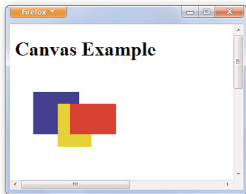
FIGURE 2.2 Drawing rectangles.
