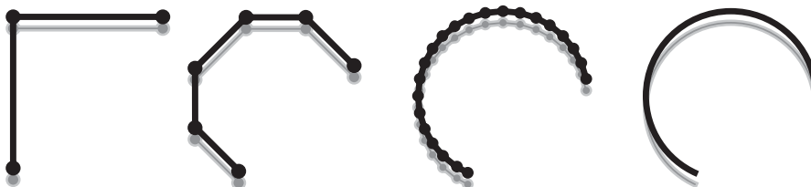
Figure 2-5 Approximating Curves
