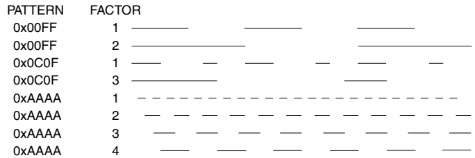
Figure 2-8 Stippled Lines
