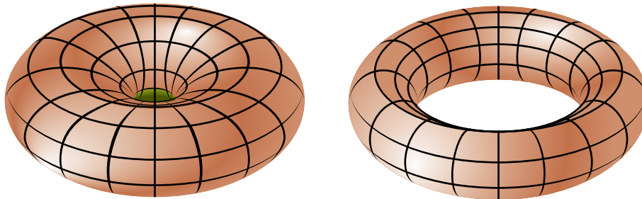
Figure 9-9 Texture-Map Distortion
