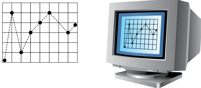
Figure 3-16 Viewport Rectangle
