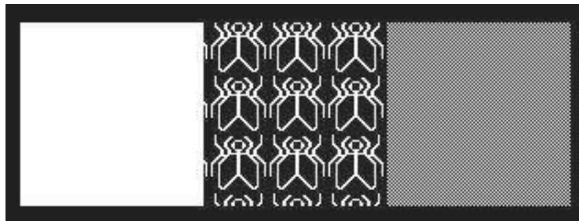
Figure 2-11 Stippled Polygons
