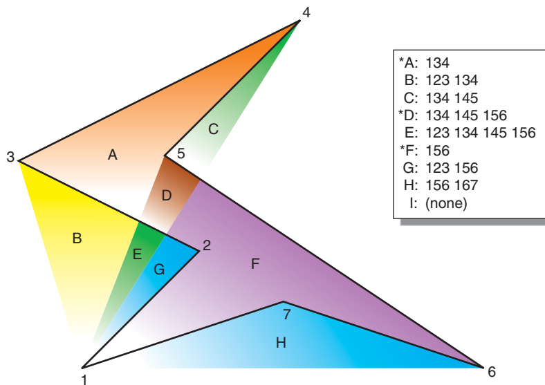
Figure 14-2 Concave Polygon
