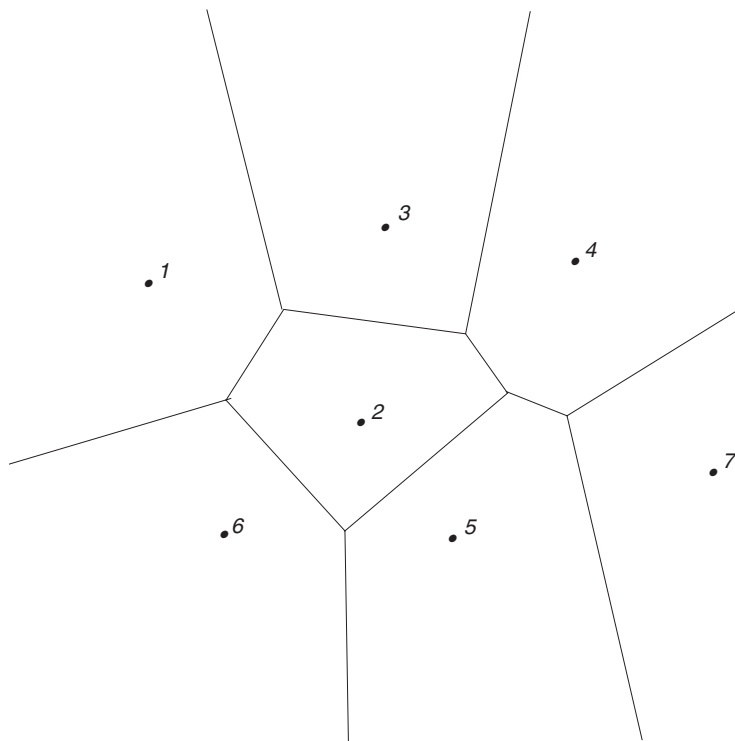
Figure 14-3 Dirichlet Domains
