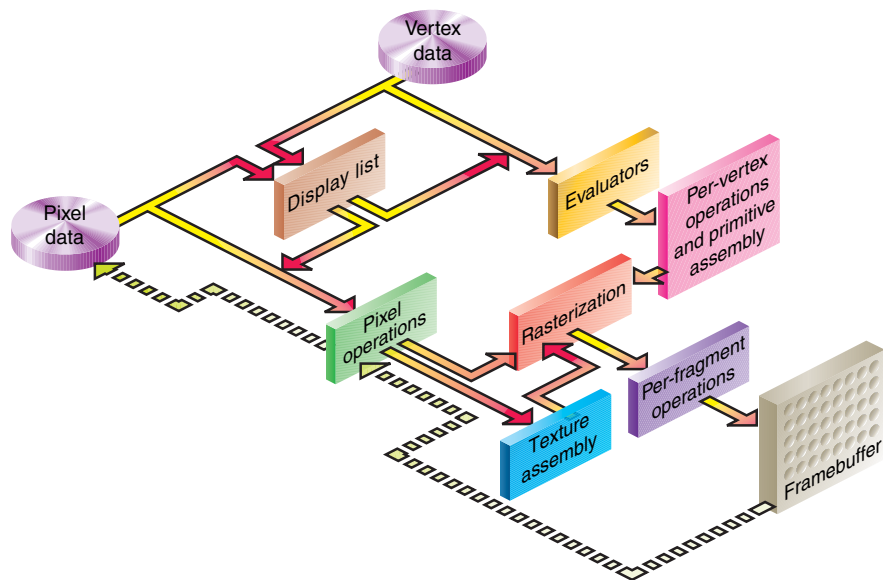
Figure 1-2 Order of Operations
