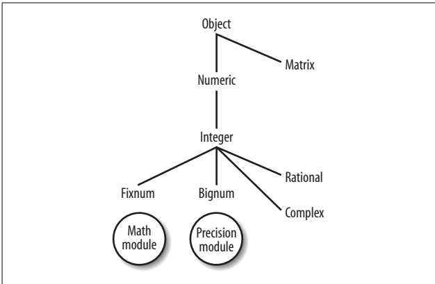
Figure 1. Hierarchy of Ruby math classes
