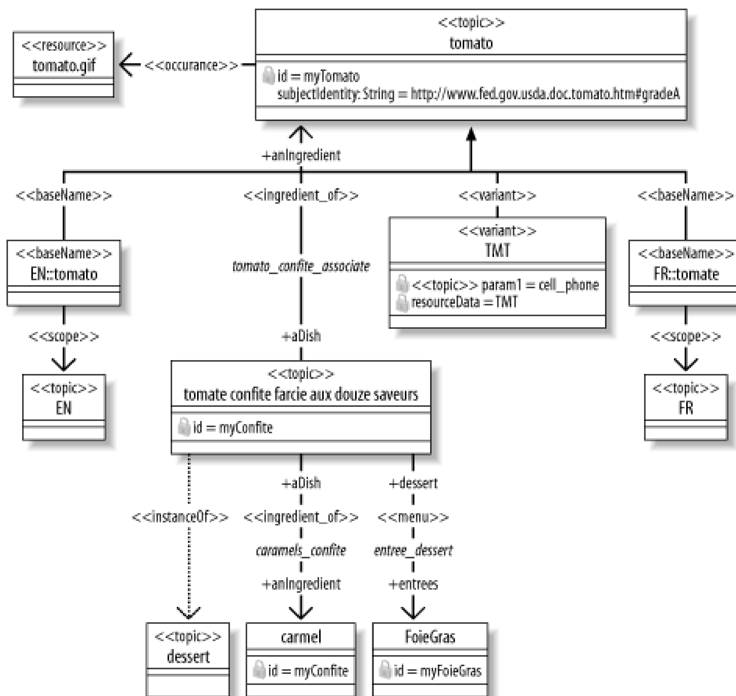
Figure 11-2. UML diagram of a tomato topic map
