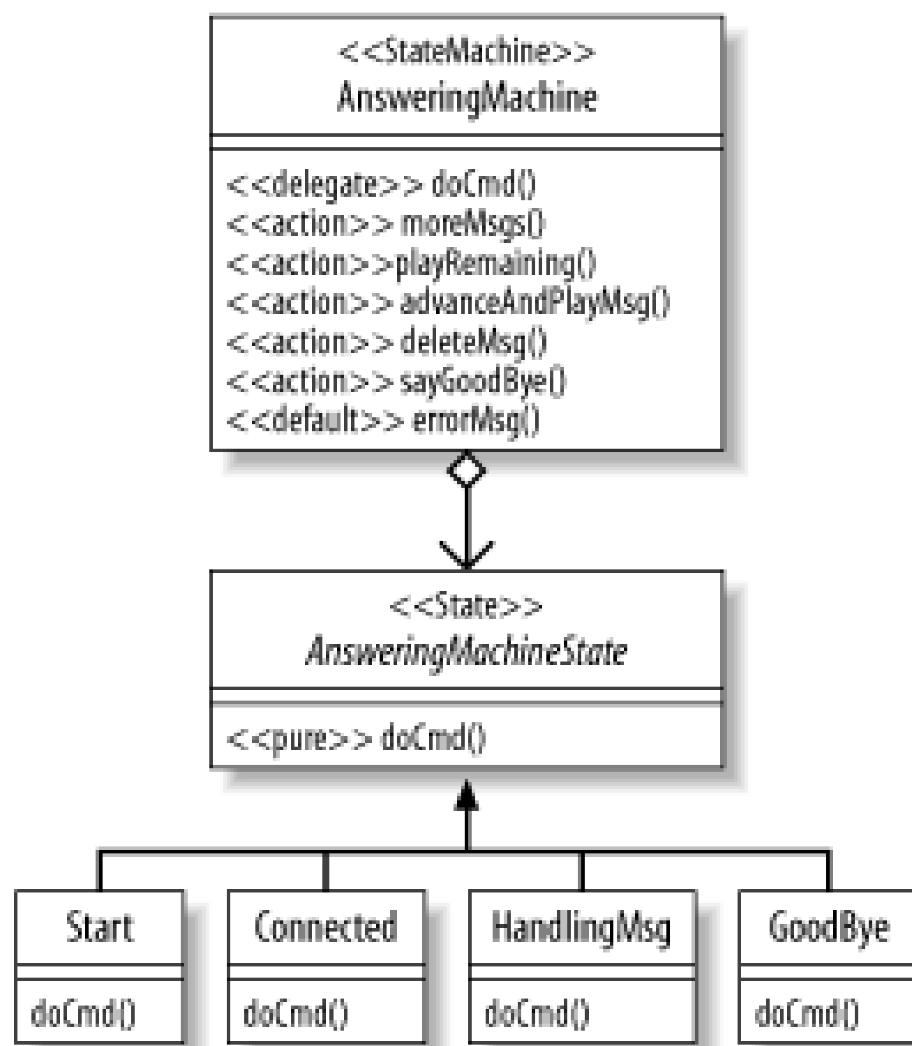
Figure 10-3. State chart for answering machine
