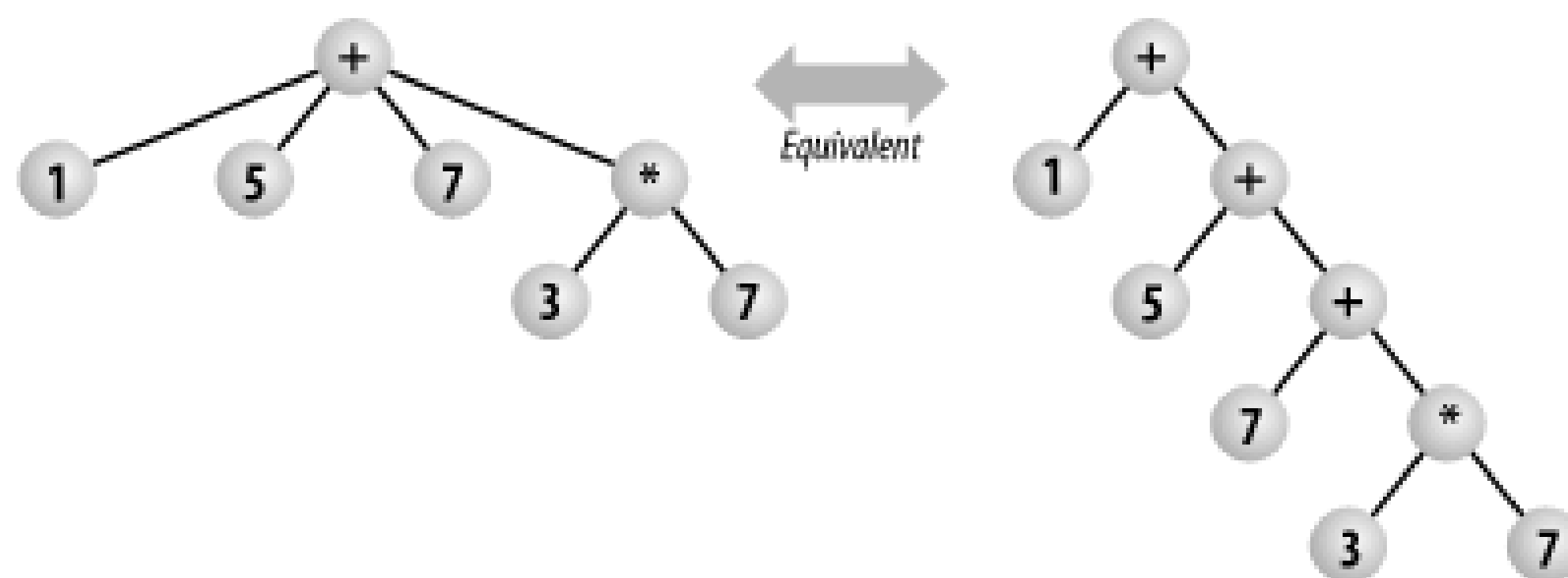
Figure 4-1. N-ary to binary tree equivalent
