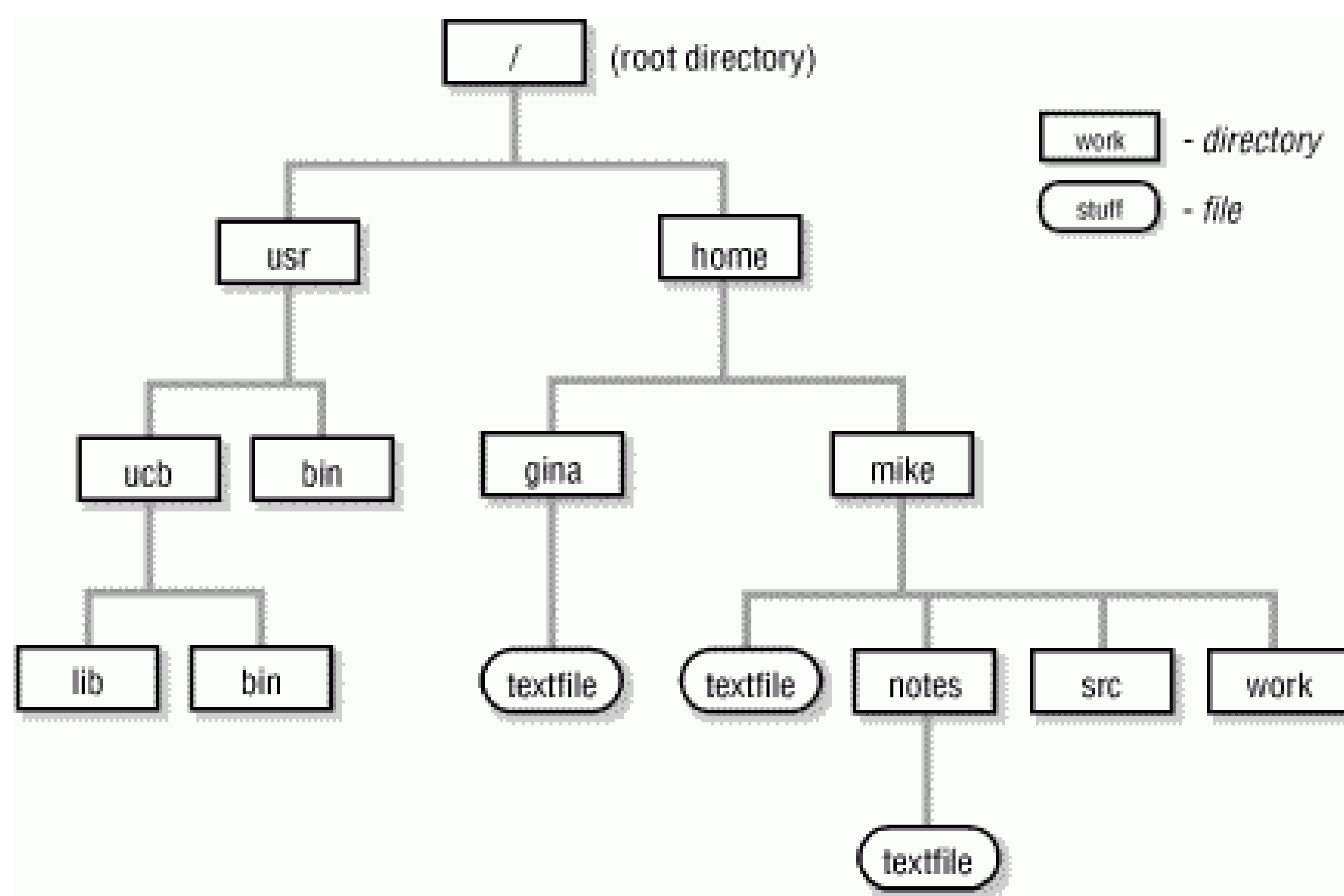
Figure 1-4. Part of a Unix filesystem tree
