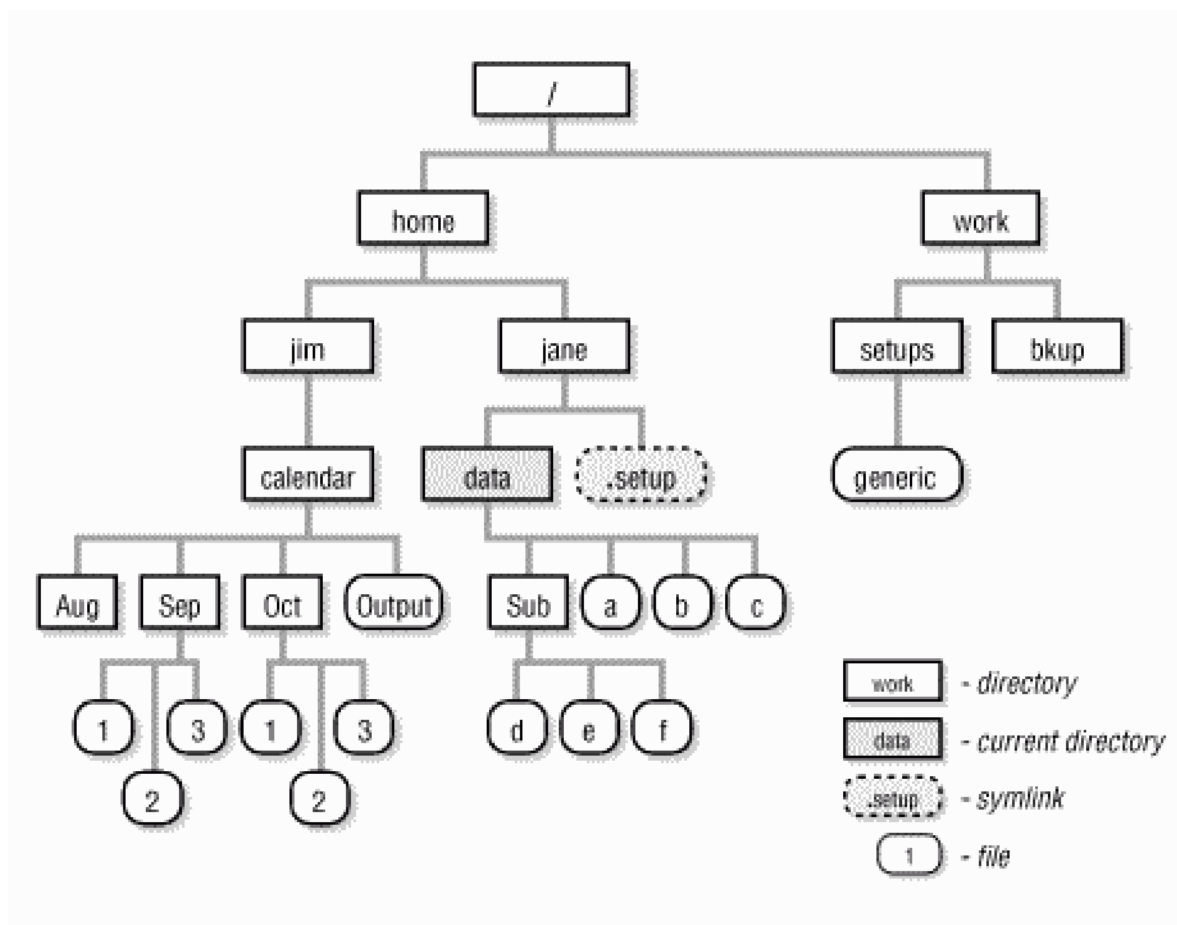
Figure 31-1. A Unix filesystem tree
