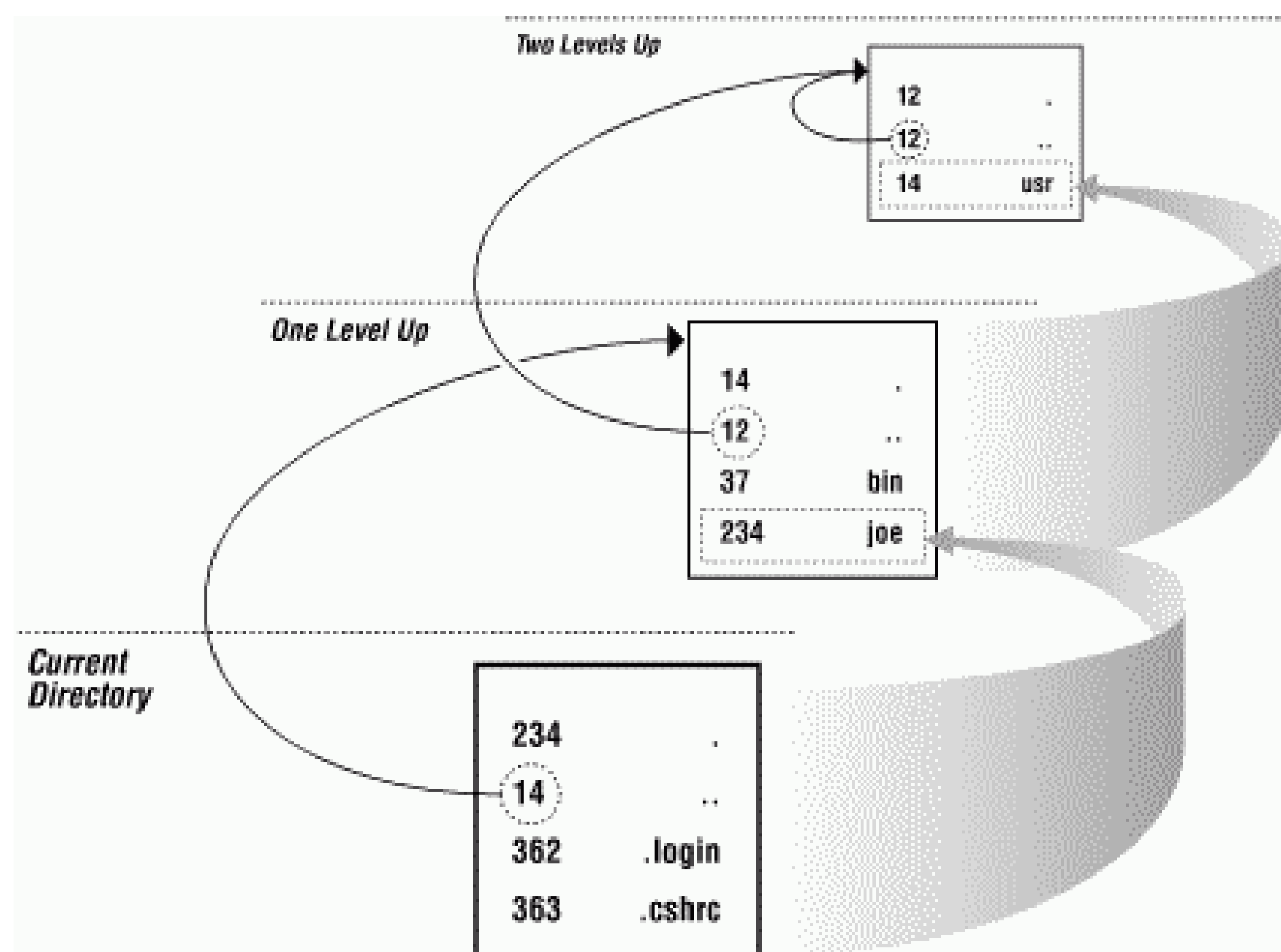
Figure 31-2. Finding the current directory name
