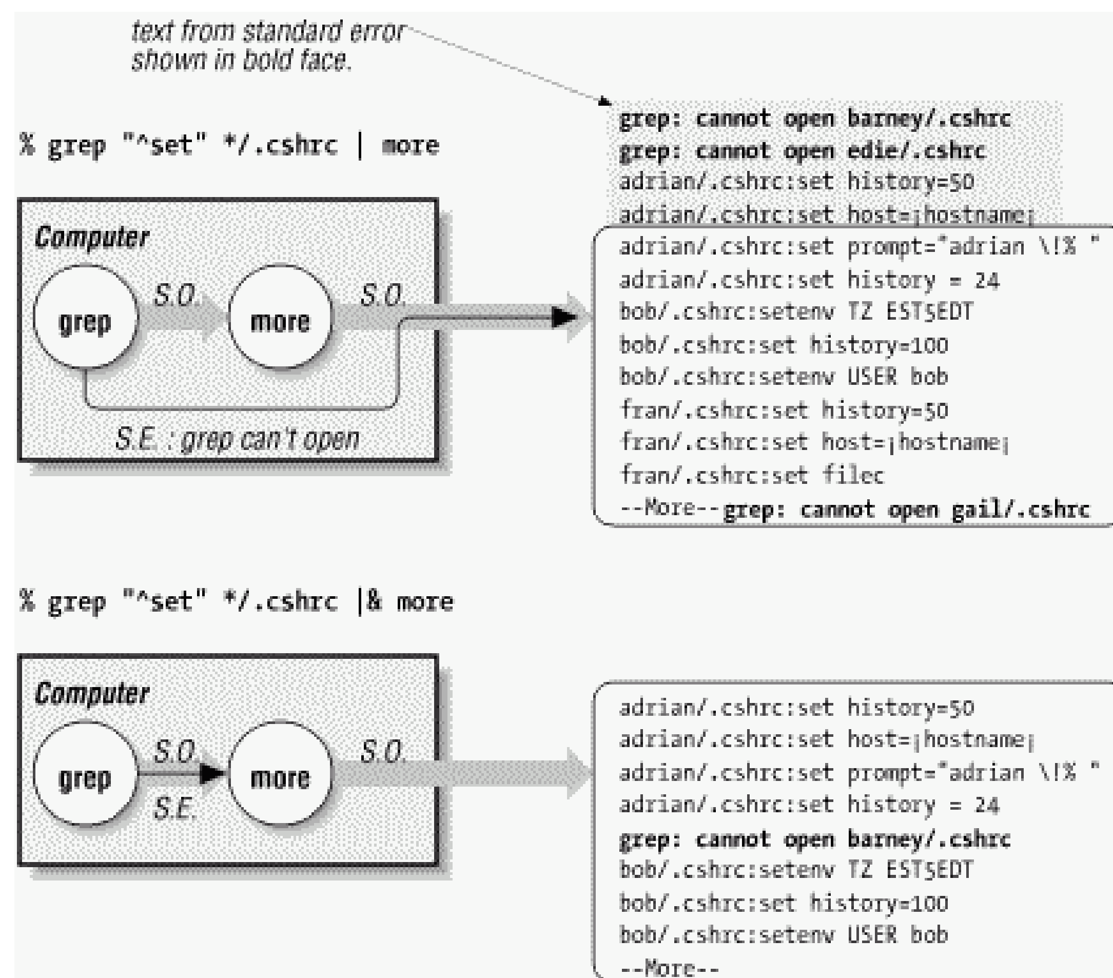
Figure 43-1. Standard error bypassing pipe, going through pipe
