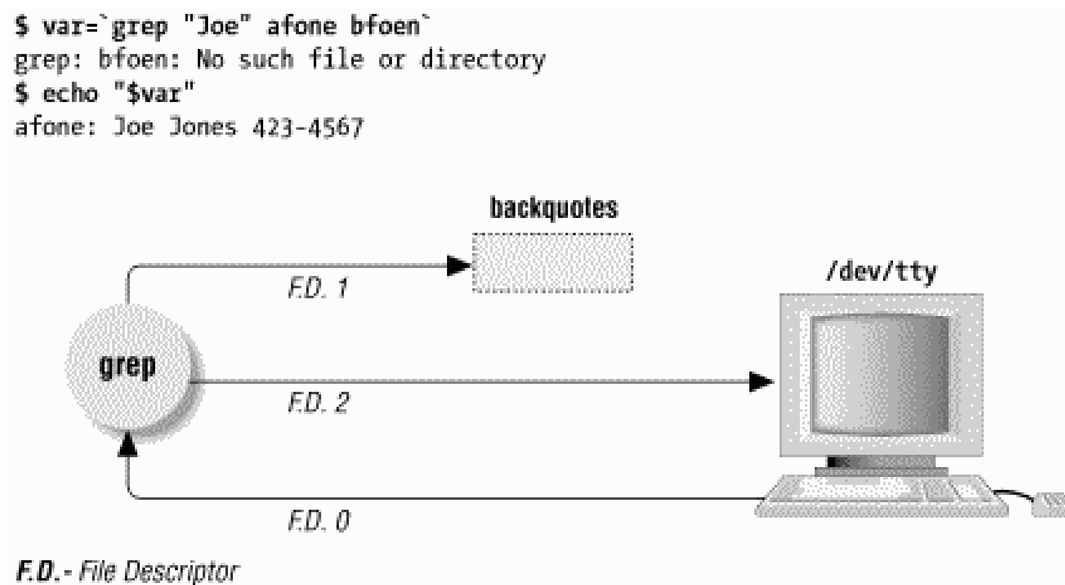
Figure 36-4. File descriptors after 3>&2 redirection
