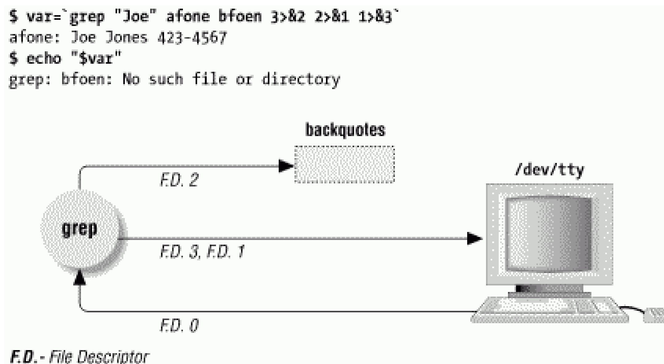
Figure 36-6. File descriptors after 3>&2 2>&1 1>&3 redirection
