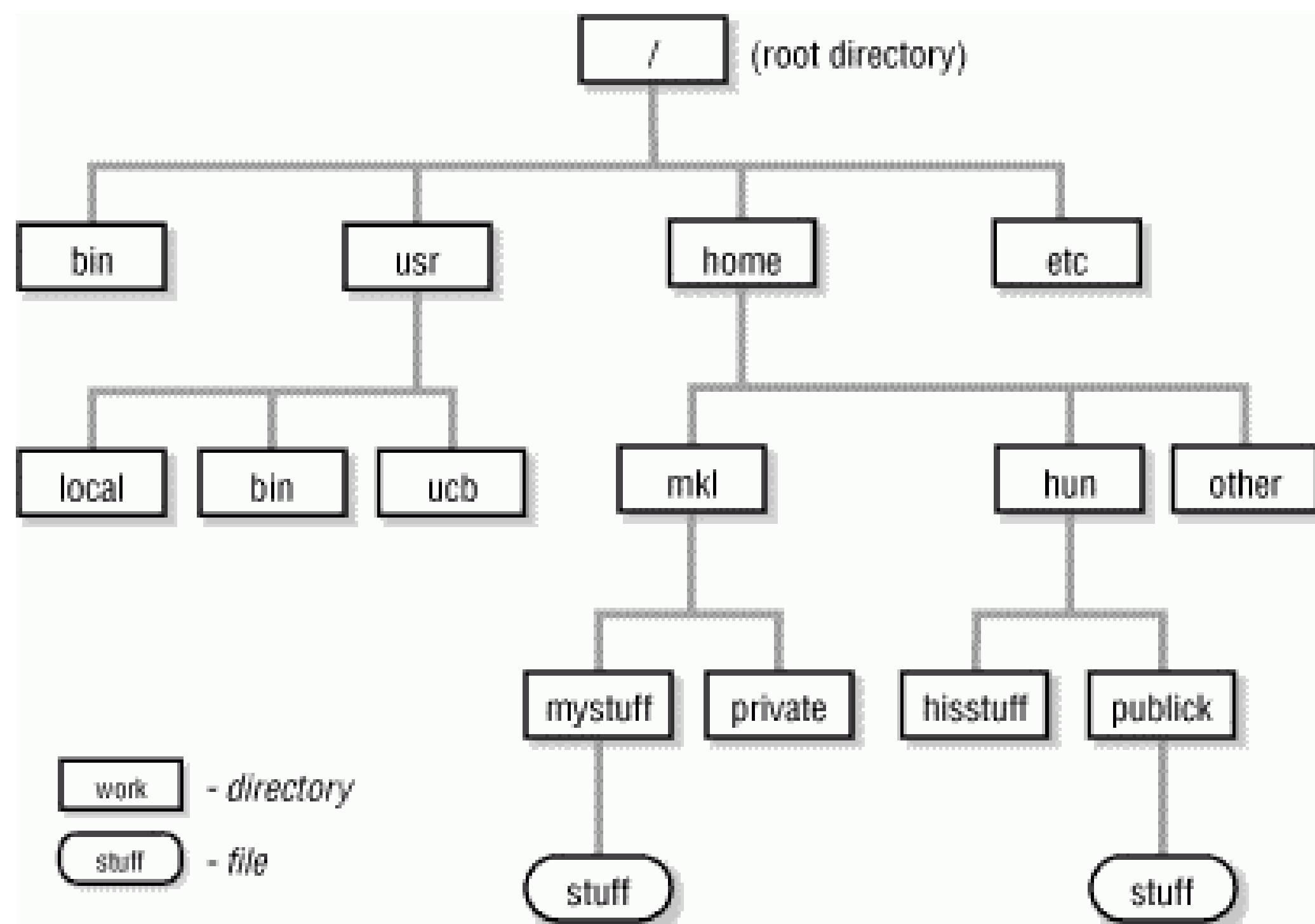
Figure 1-3. A Unix filesystem tree
