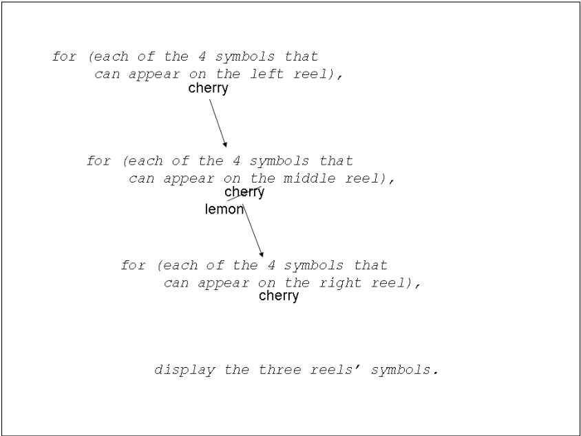
Figure 15-13: Restarting the inner loop.
