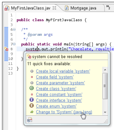
Figure 3-13: Eclipse offers some helpful sug- gestions.
