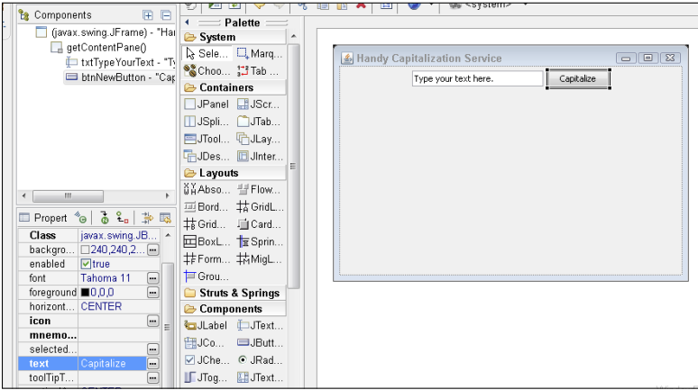
Figure 20-19: Changing the text on the face of the button.
