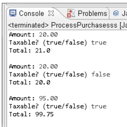
Figure 17-5: Running the code in Listing 17-5.
