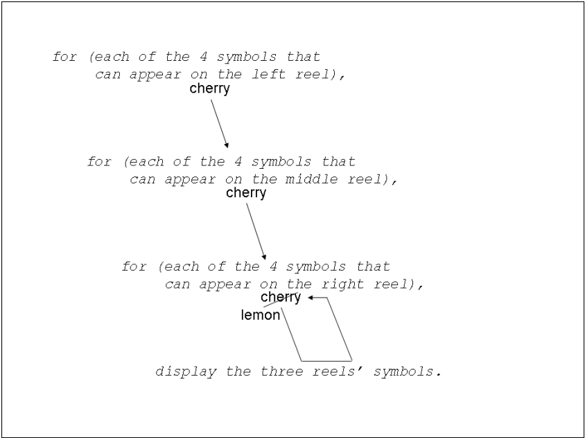
Figure 15-11: Changing from cherry to lemon in the inner- most loop.
