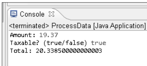
Figure 18-9: Do you have change for 20.3385000 0000003?
