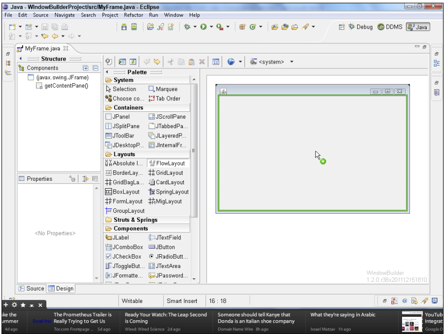
Figure 20-13: Preparing to add a FlowLayout to your frame.
