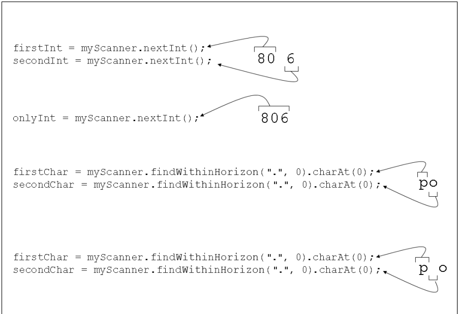
Figure 8-8: Reading numbers and characters.
