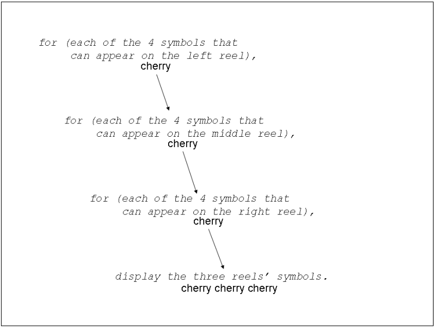
Figure 15-10: Entering loops for the first time in the program of Listing 15-6.
