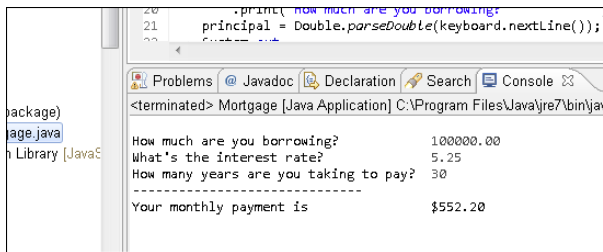
Figure 3-1: A run of this chapter's text-based mortgage program.
