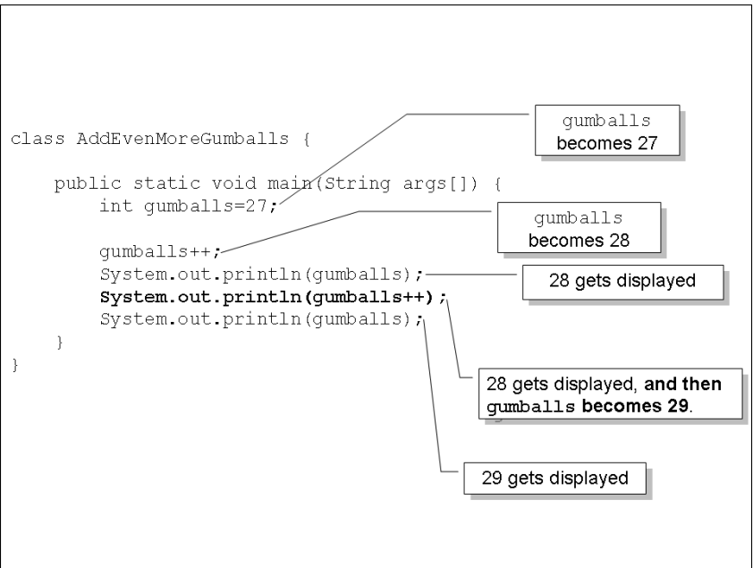
Figure 7-11: Using post-increment.
