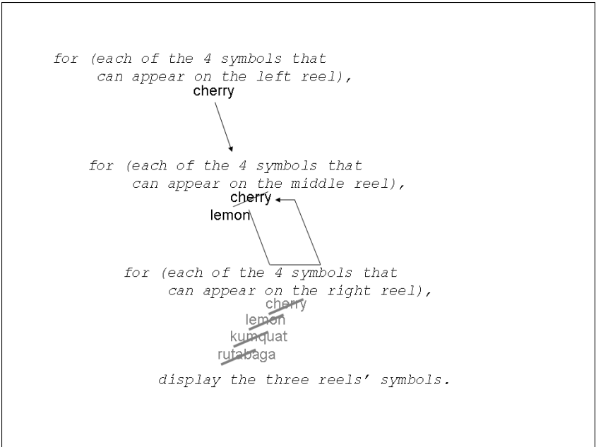
Figure 15-12: Changing from cherry to lemon in the middle loop.
