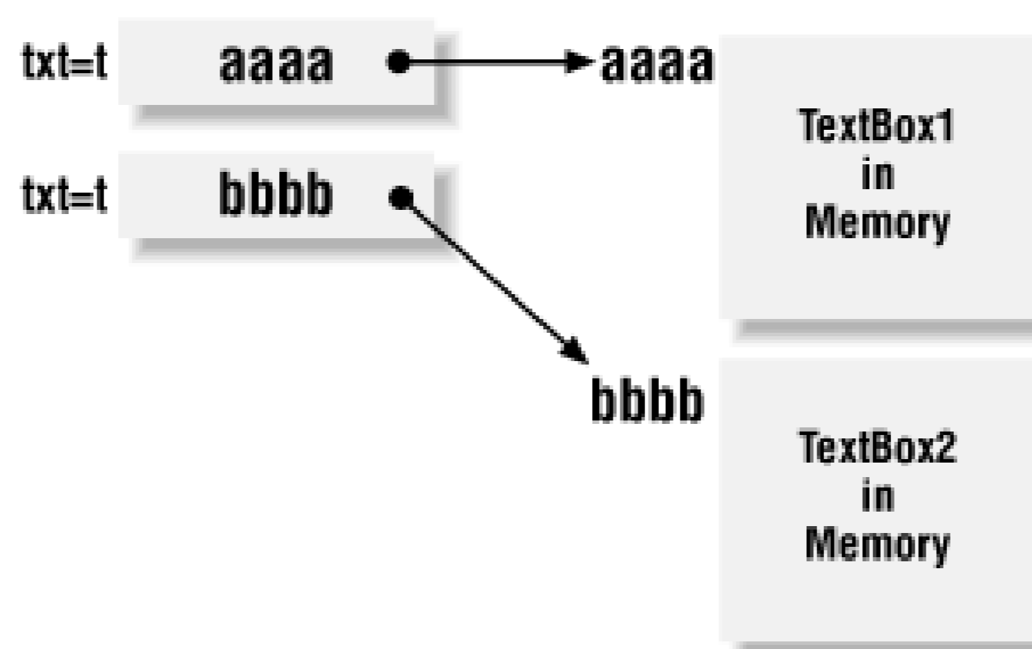
Figure 3-5. Assigning a new object reference
