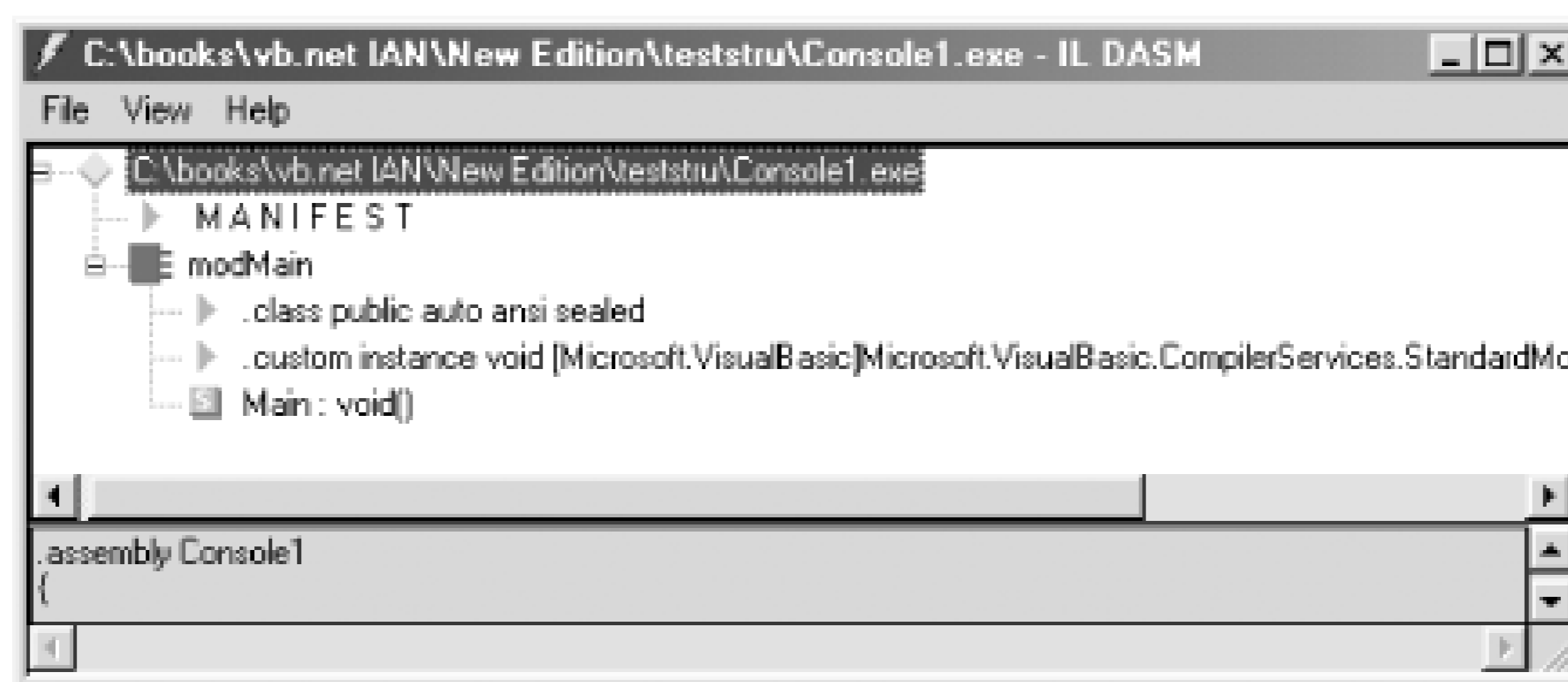
Figure 2-2. IL for the Main procedure
