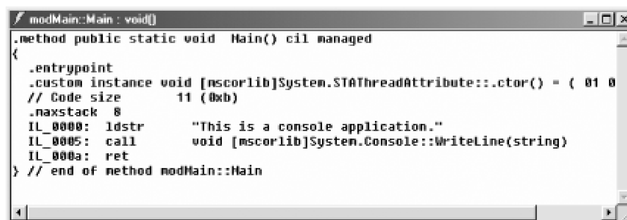
Figure 2-2. IL for the Main procedure
