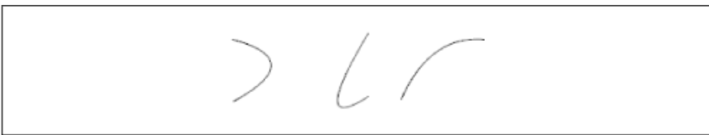
Figure 3.4. Quadratic curves
