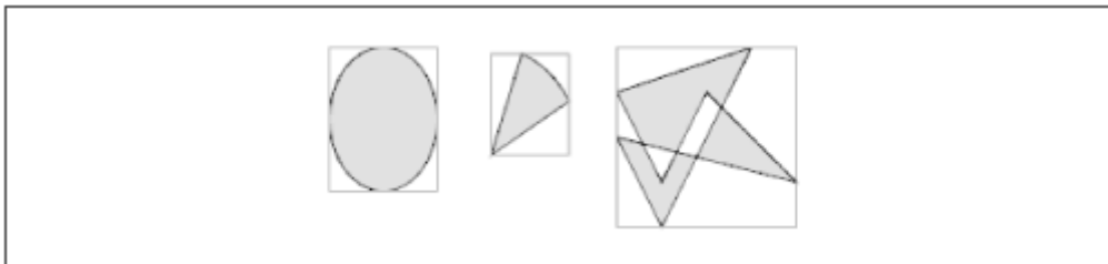
Figure 3.2. Bounds rectangles
