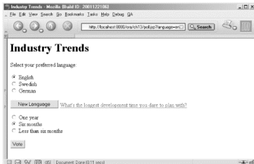
Figure 13-2. The language selection and question page
