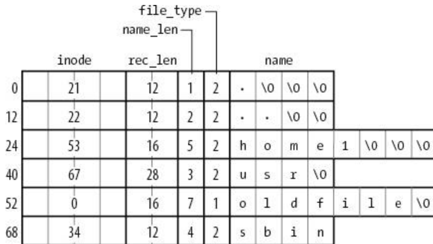
Figure 18-3. An example of the Ext2 directory
