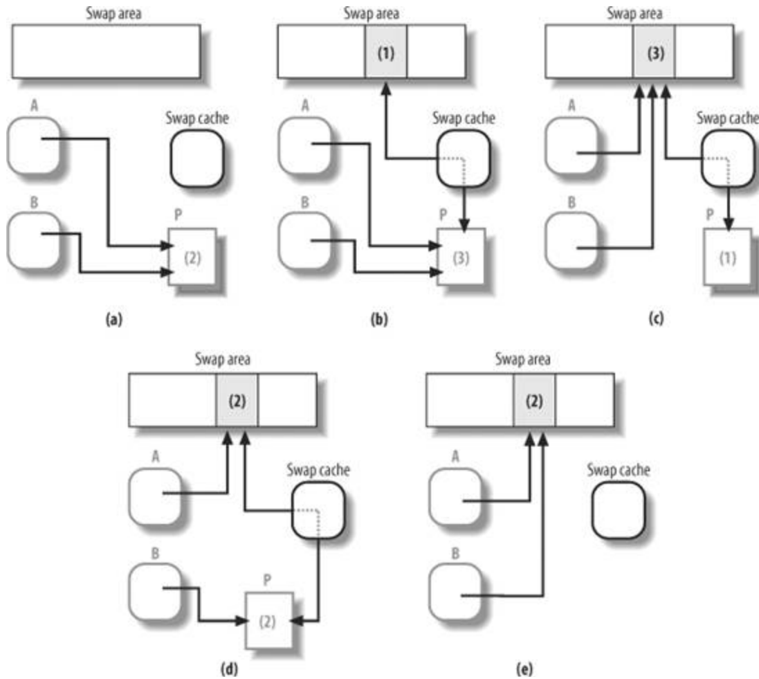
Figure 17-8. The role of the swap cache
