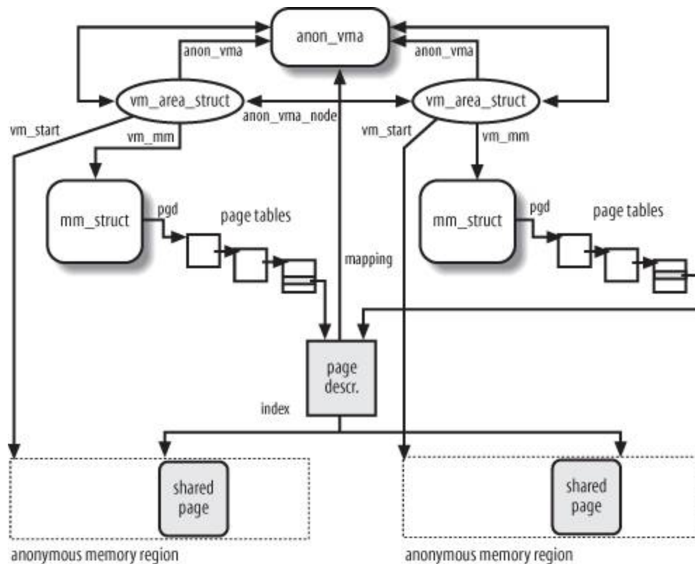
Figure 17-1. Object-based reverse mapping for anonymous pages
