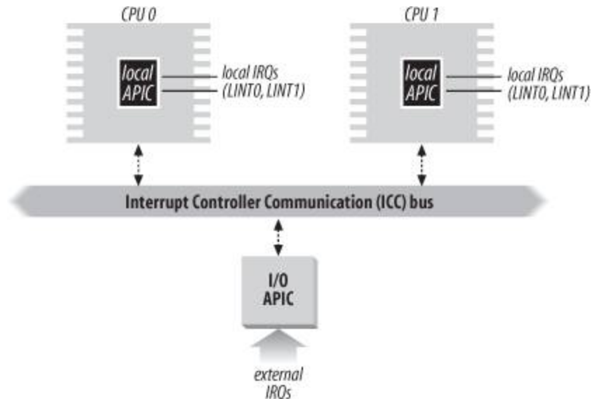
Figure 4-1. Multi-APIC system
