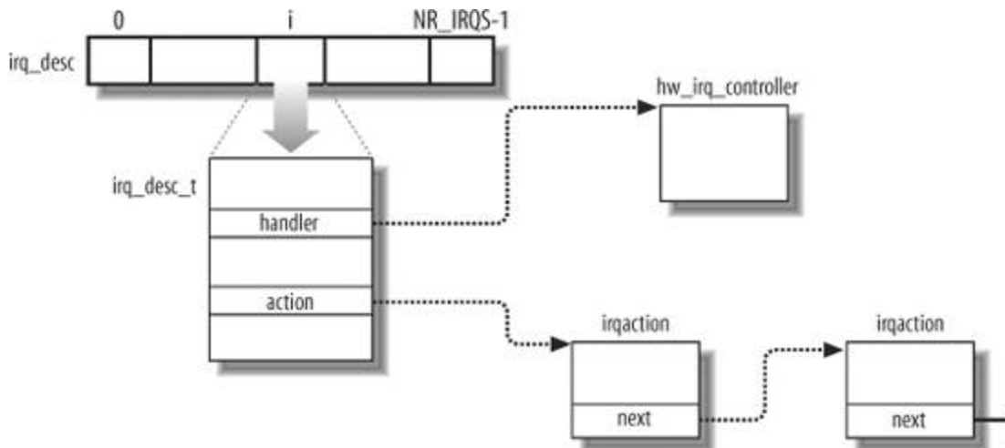
Figure 4-5. IRQ descriptors
