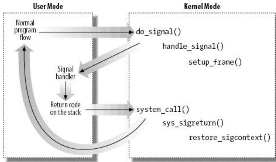
Figure 11-2. Catching a signal
