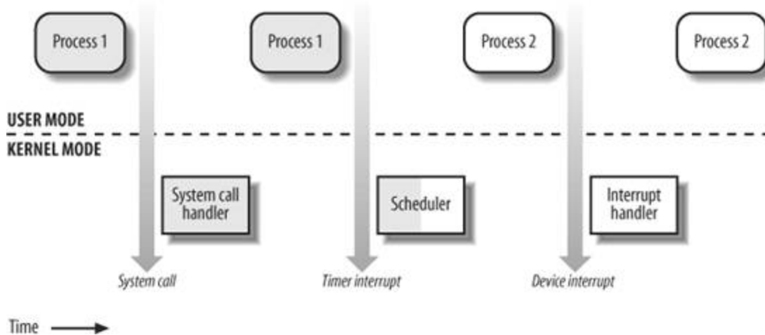
Figure 1-2. Transitions between User and Kernel Mode
