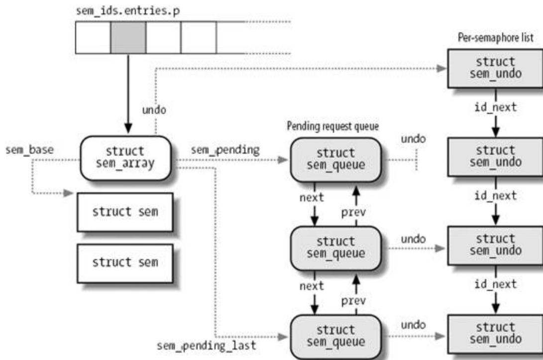
Figure 19-1. IPC semaphore data structures
