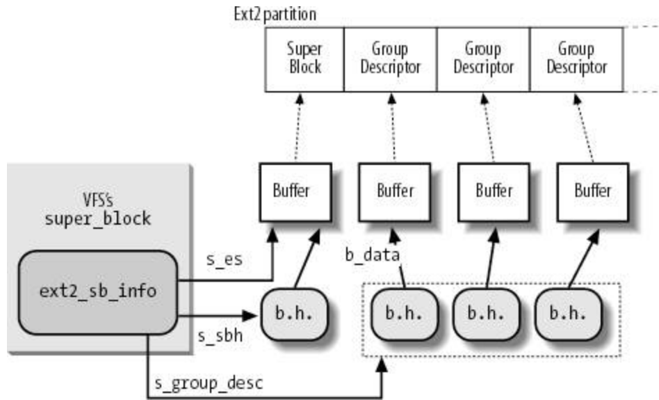
Figure 18-4. The ext2_sb_info data structure
