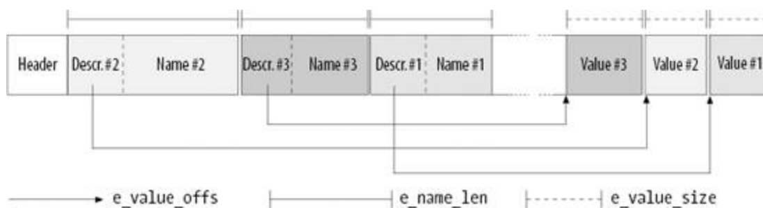
Figure 18-2. Layout of a block containing extended attributes
