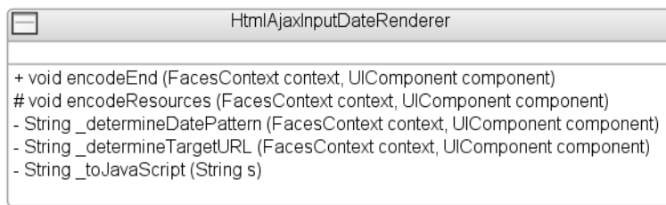
Figure 7-5. Class diagram showing the HtmlAjaxInputDateRenderer
