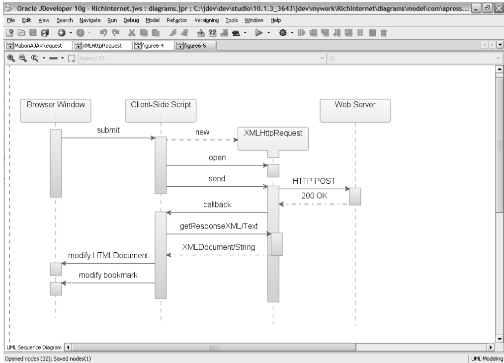
Figure 6-3. Sequence diagram over your Ajax postback implementation
