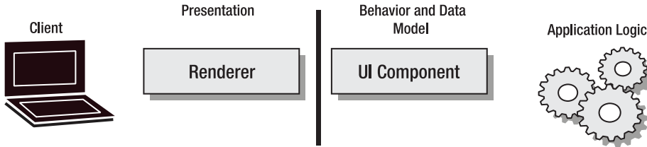
Figure 1-5. Separation of UI from behavior and data model
