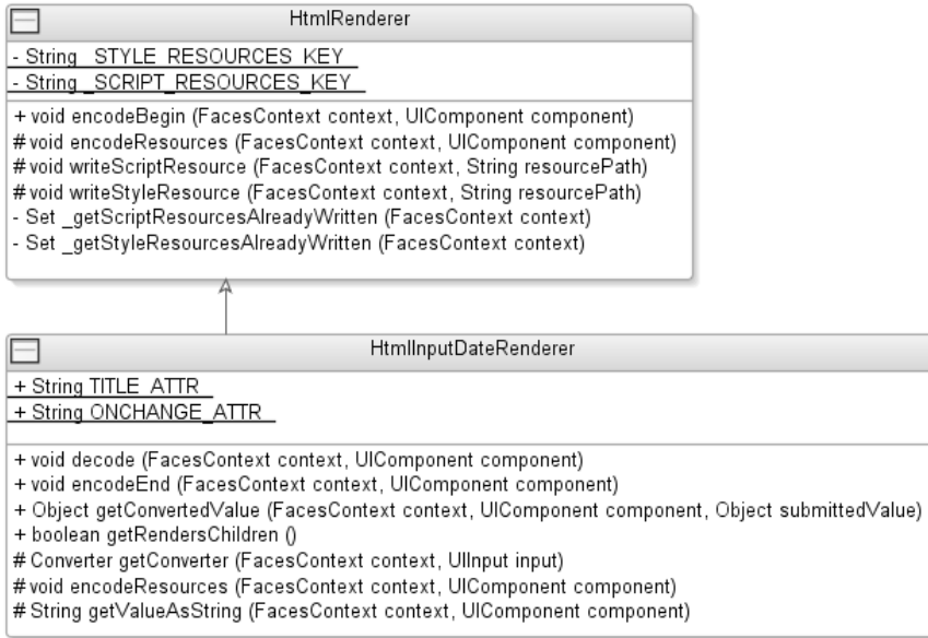
Figure 2-3. Class diagram over the HtmlInputDateRenderer class created in this chapter
