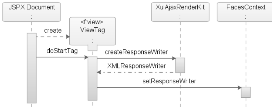
Figure 8-13. Sequence diagram of creating the right ResponseWriter for the response
