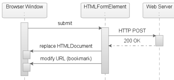
Figure 4-1. Sequence diagram over a regular postback
