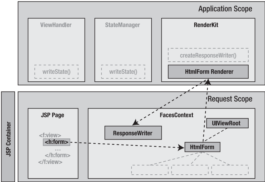
Figure 1-14. Writing <form> start element to the <f:view> body content buffer
