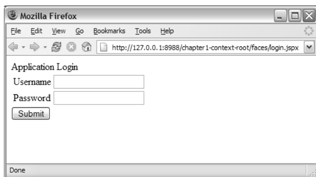
Figure 1-25. Rendering of non-JSF content using the <f:verbatim> tag
