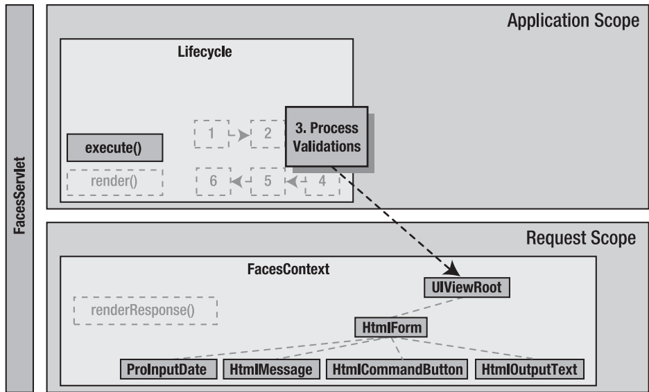
Figure 2-7. Process Validations phase
