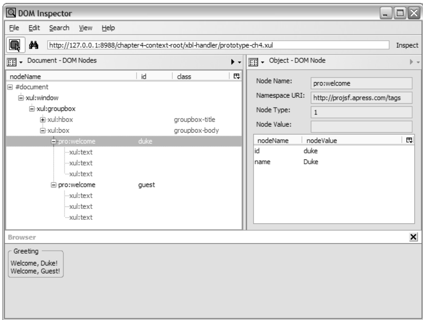
Figure 4-7. A page's DOM tree with an XBL component
