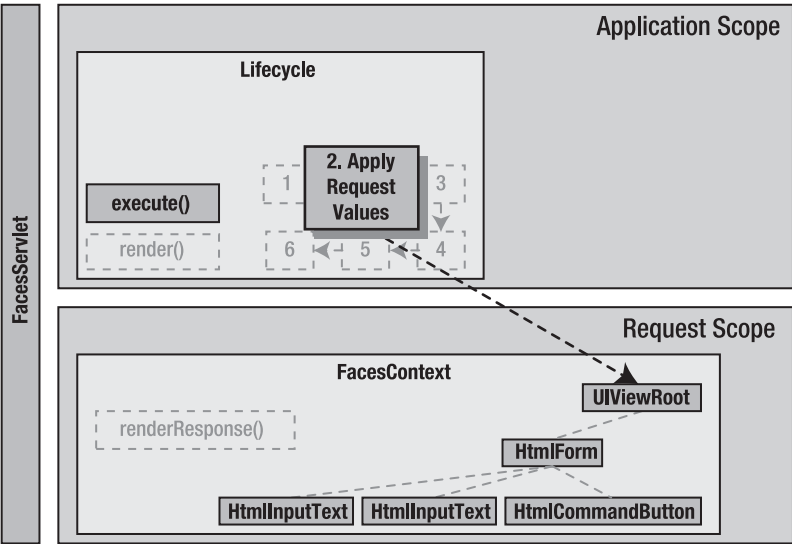
Figure 1-18. Applying new values passed on the request to the components
