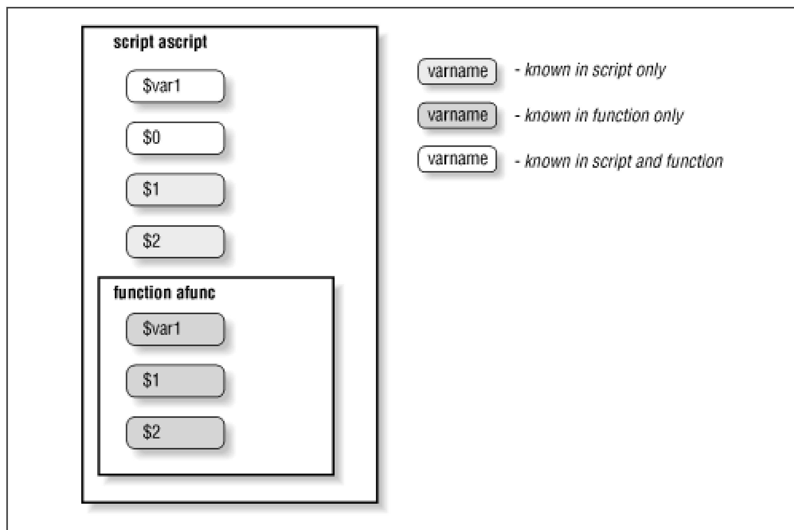
Figure 4.3. Functions can have local variables
