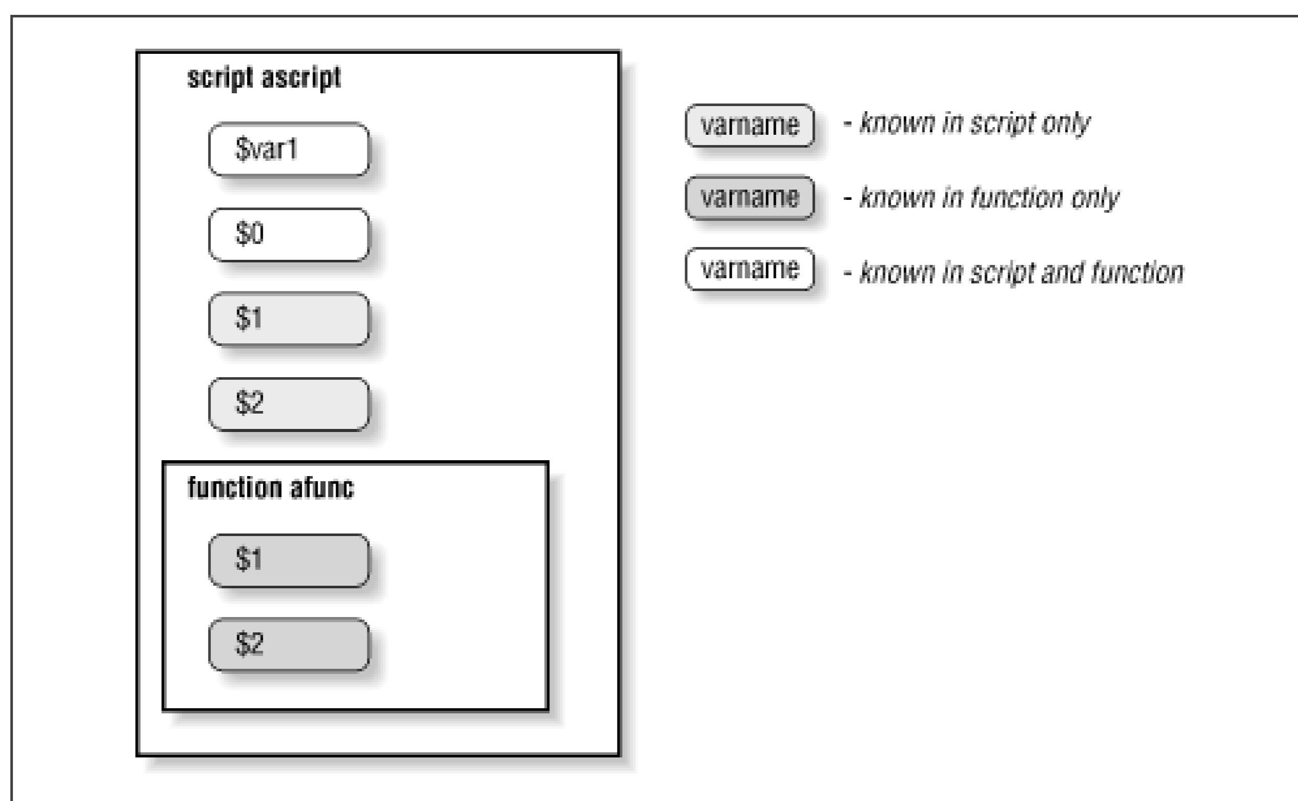
Figure 4.2. Functions have their own positional parameters
