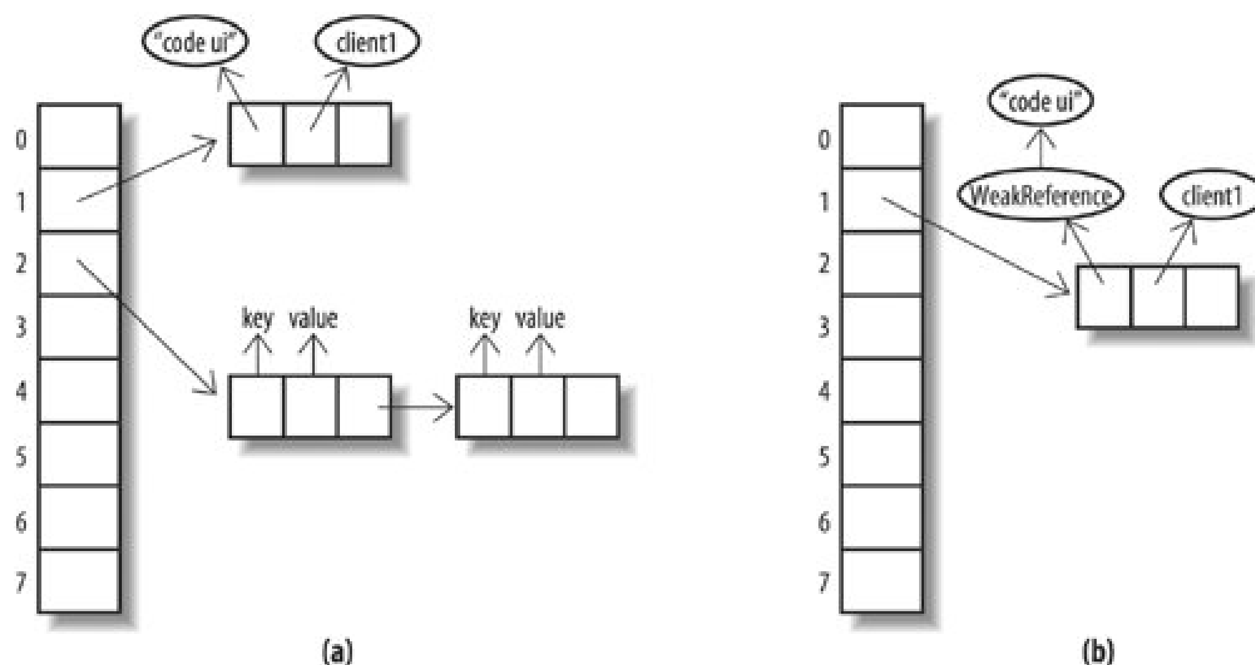
Figure 16-3. HashMap and WeakHashMap
