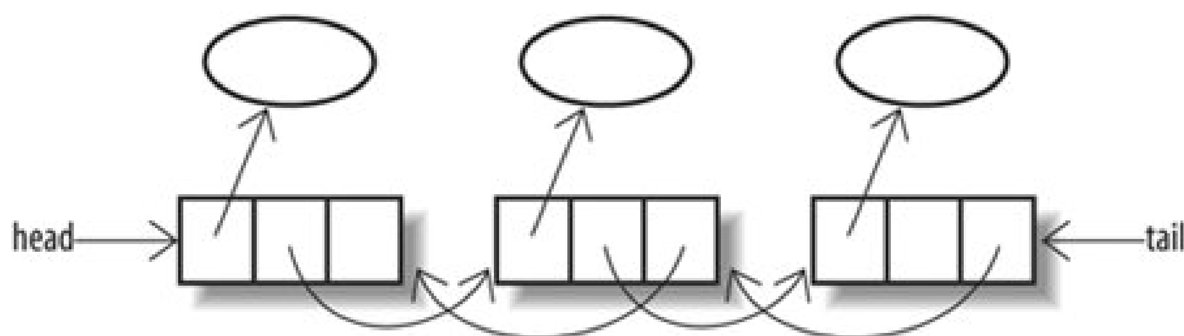
Figure 14-8. A doubly linked list
