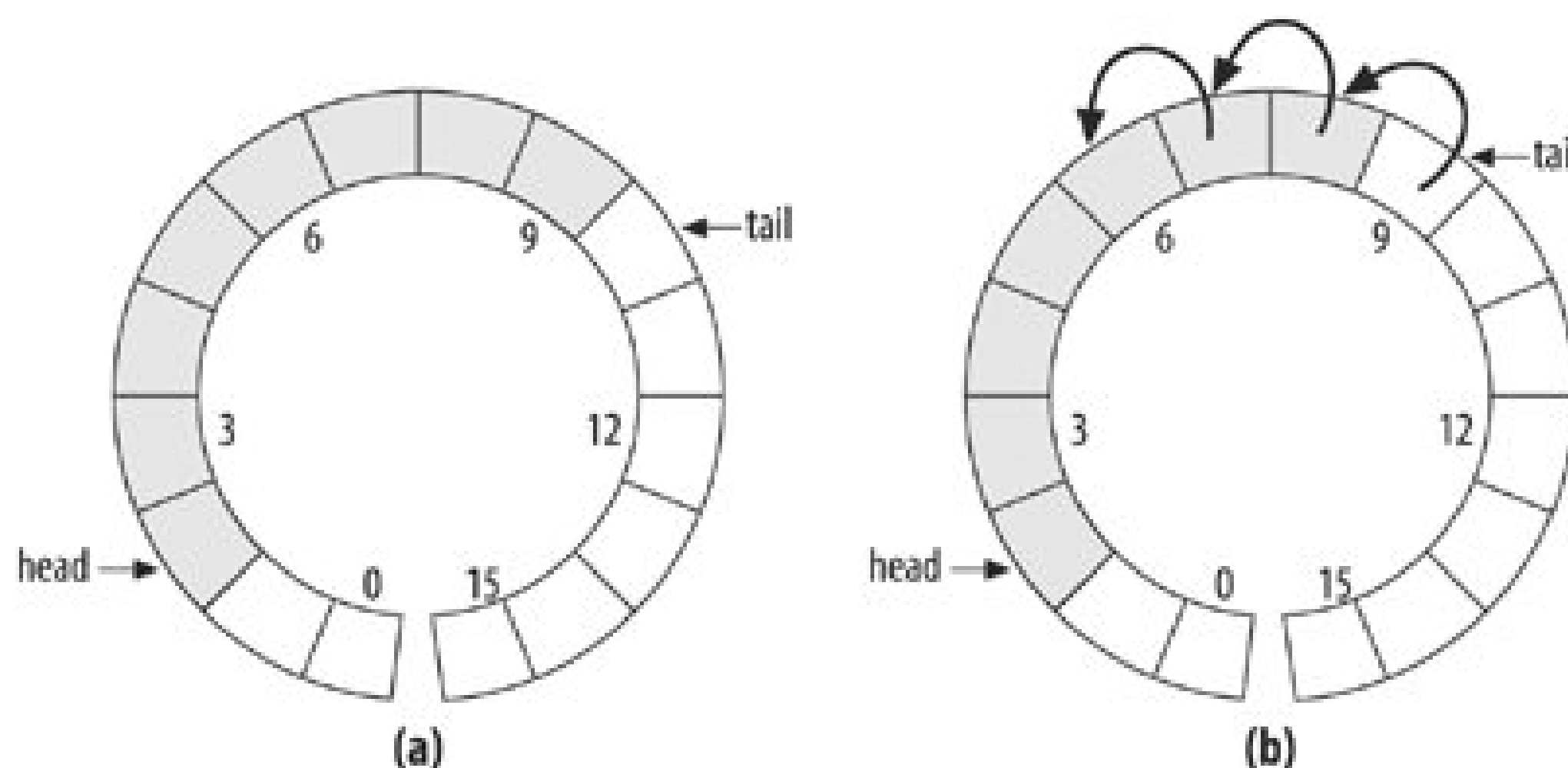
Figure 14-6. A circular array
