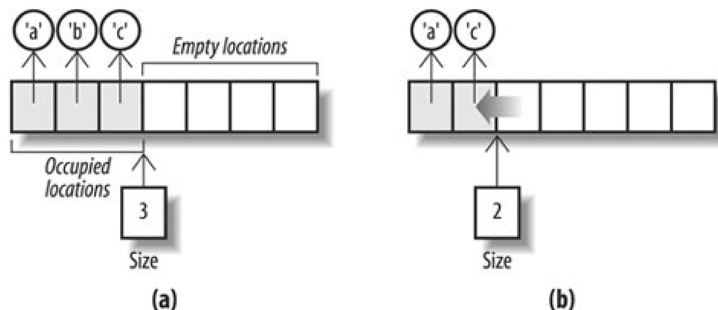
Figure 15-4. Removing an element from an ArrayList
