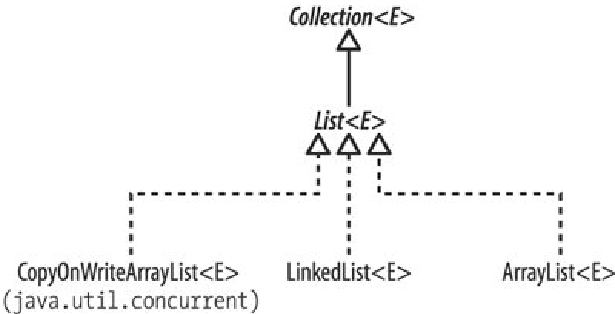
Figure 15-3. Implementations of the List interface
