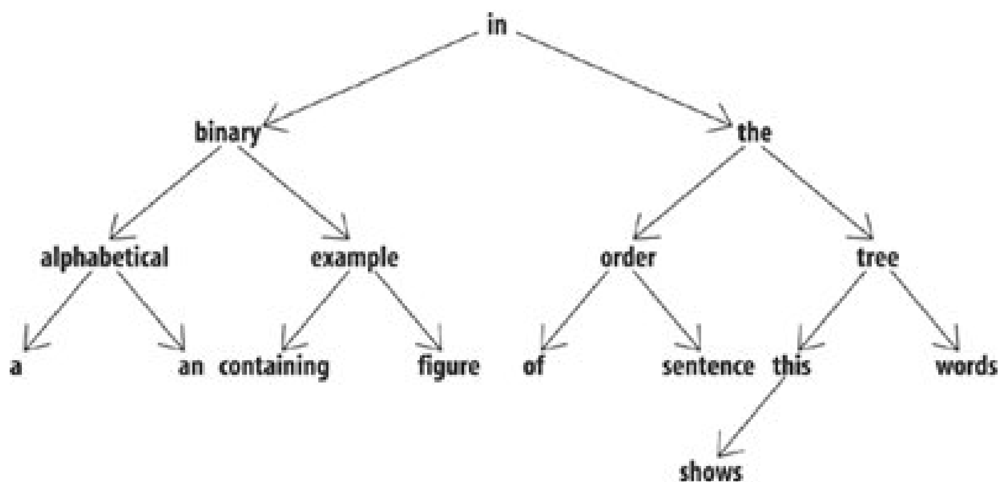
Figure 13-6. An ordered, balanced binary tree
