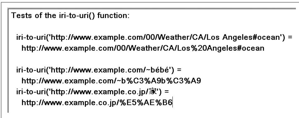
Figure C-4. Sample with illegal URI characters escaped
