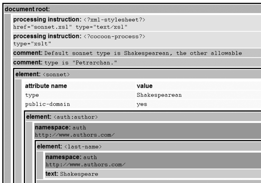
Figure 3-1. XPath tree view of an XML document
