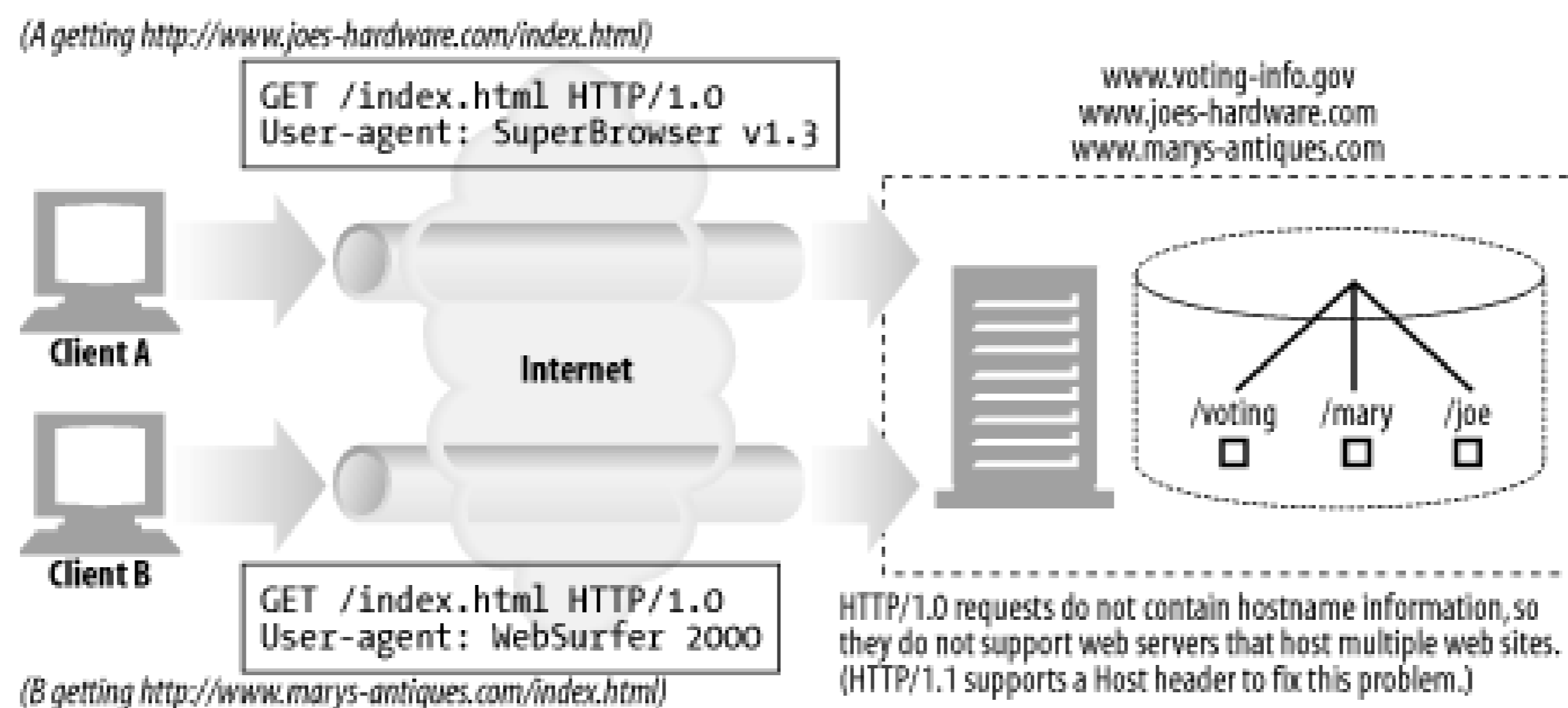
Figure 18-3. HTTP/1.0 server requests don't contain hostname information
