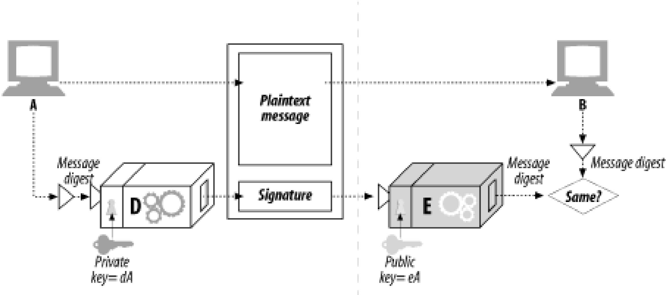
Figure 14-10. Unencrypted digital signature
