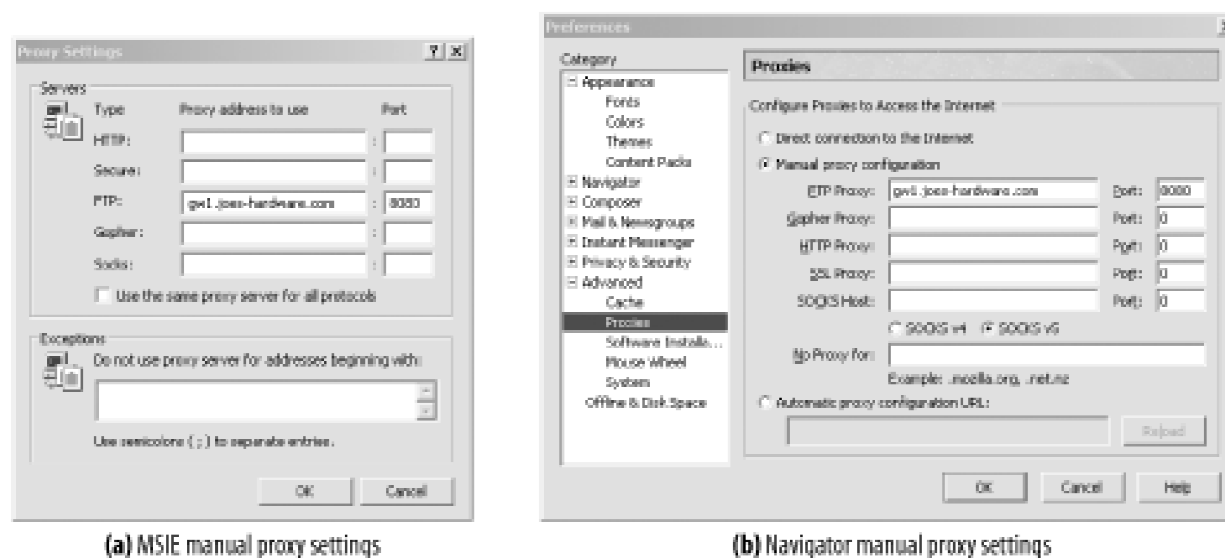
Figure 8-3. Configuring an HTTP/FTP gateway
