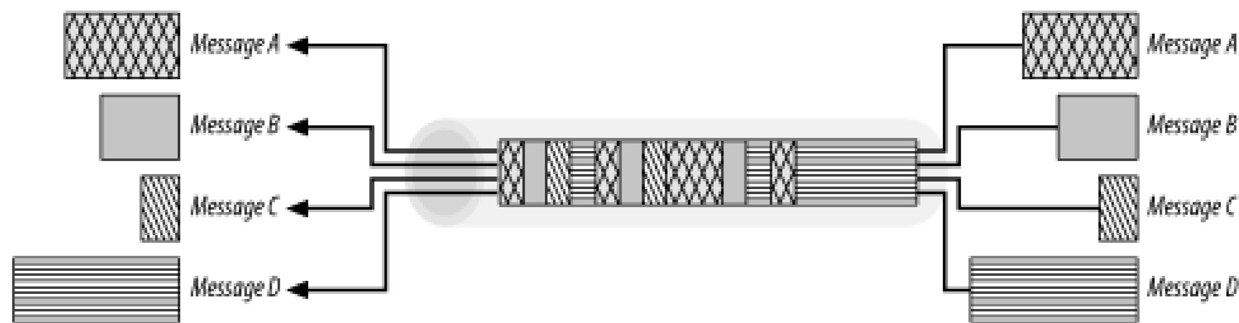
Figure 10-2. WebMUX can multiplex multiple messages over a single connection
