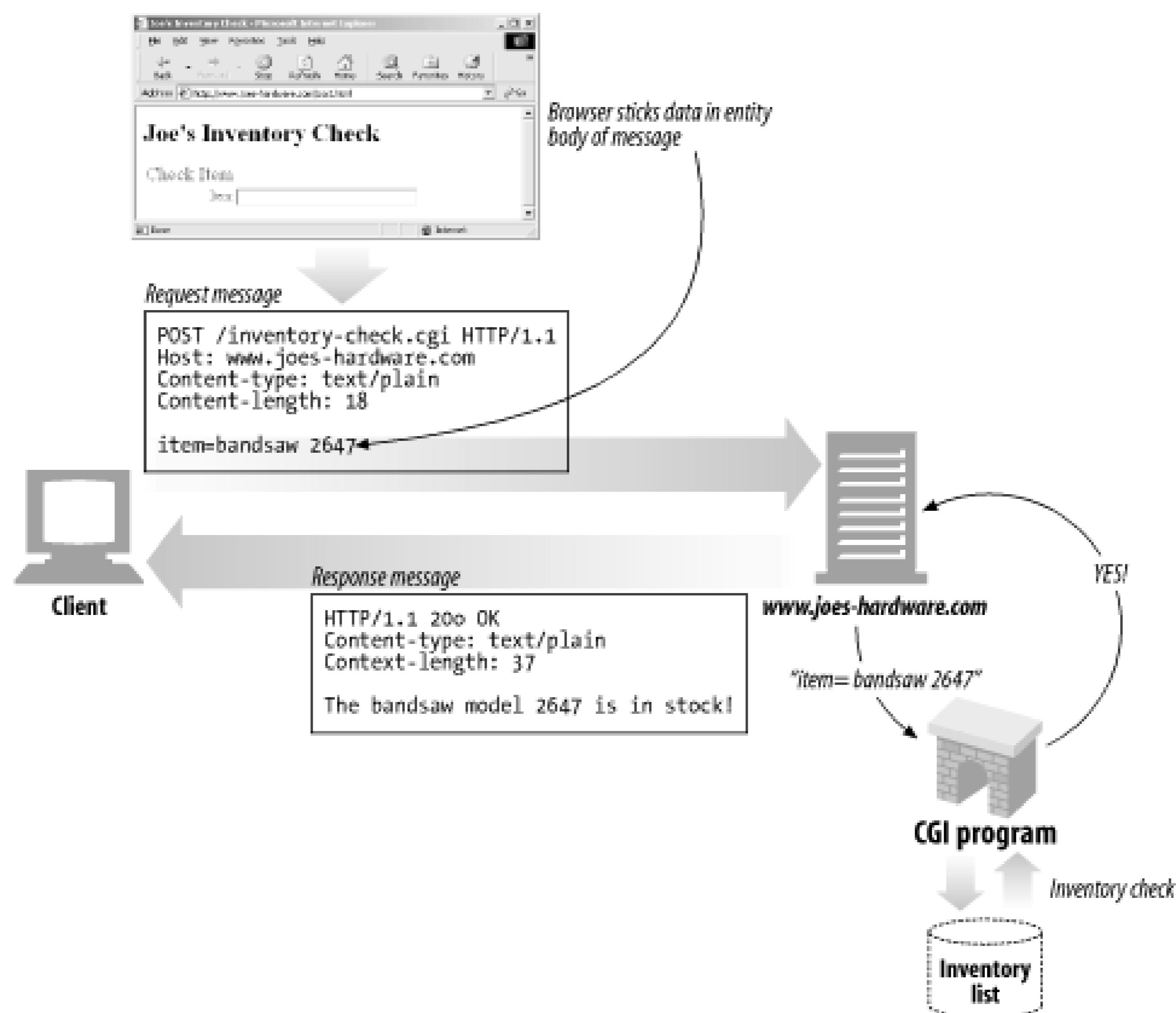
Figure 3-10. POST example
