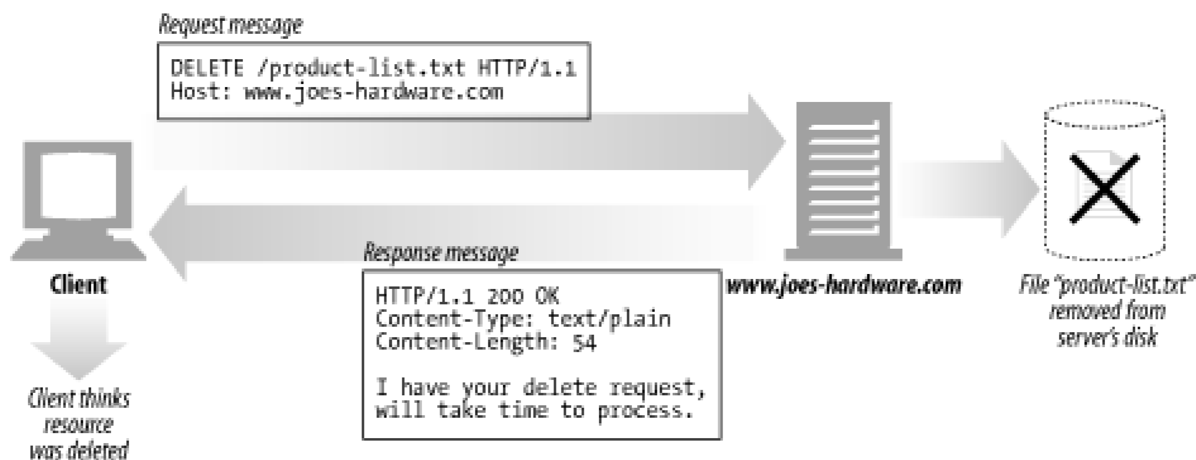
Figure 3-13. DELETE example
