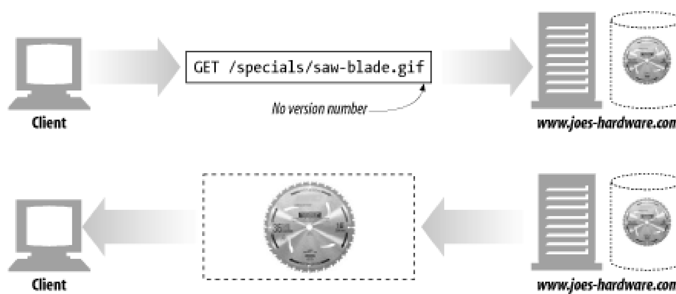
Figure 3-6. HTTP/0.9 transaction
