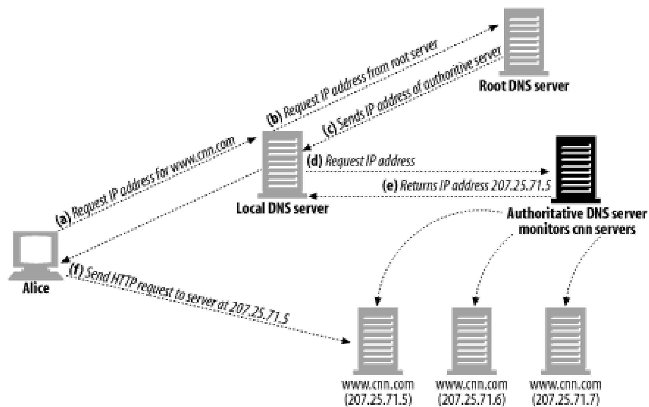
Figure 20-4. DNS request involving authoritative server
