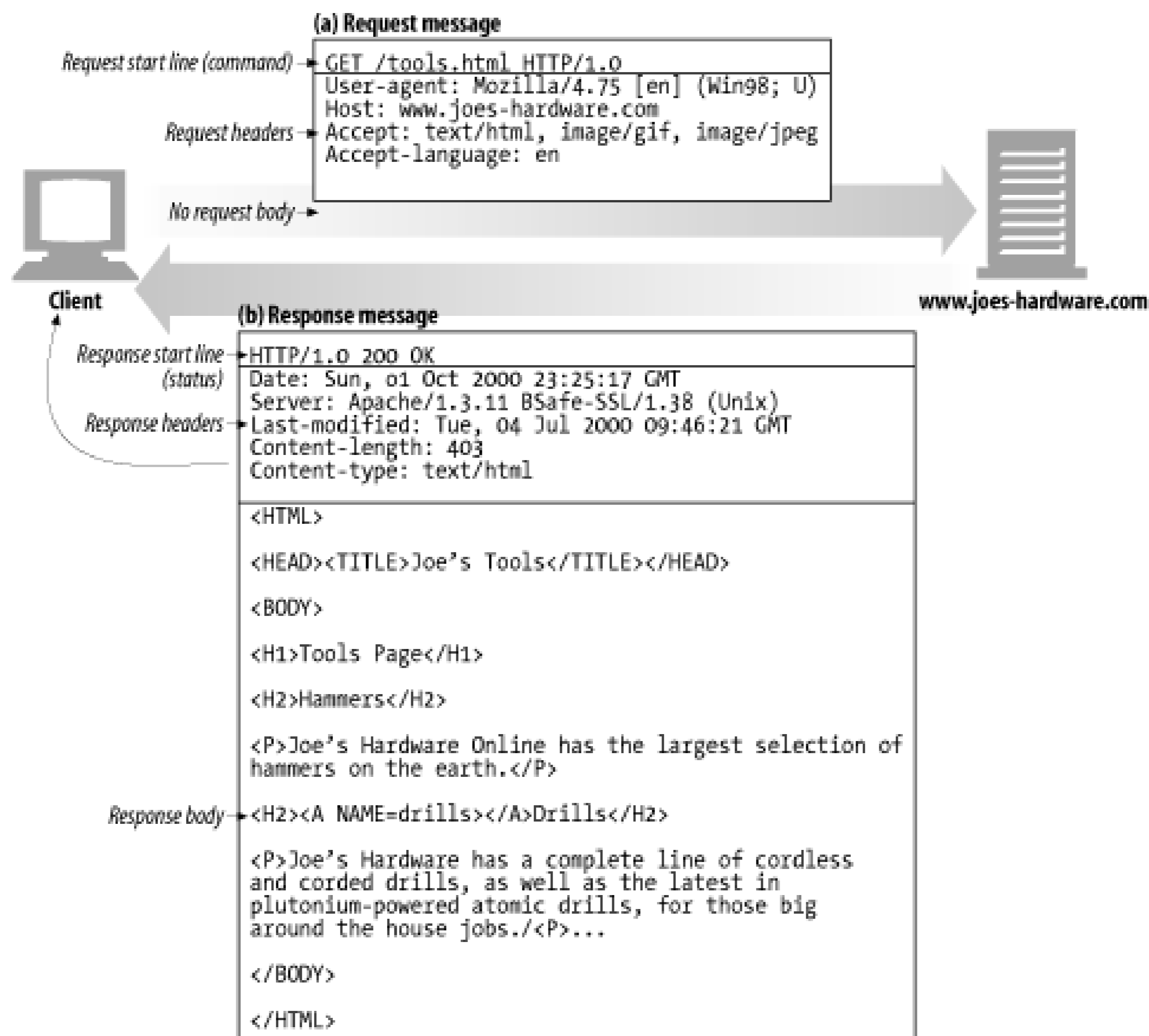
Figure 1-8. Example GET transaction for http://www.joes-hardware.com/tools.html
