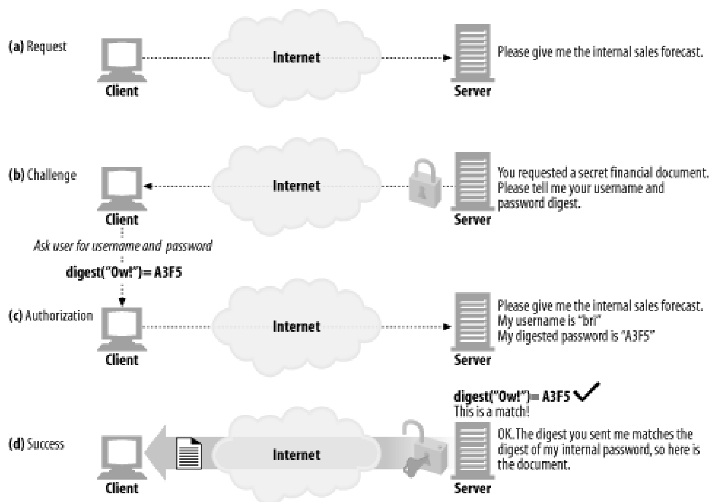
Figure 13-1. Using digests for password-obscured authentication
