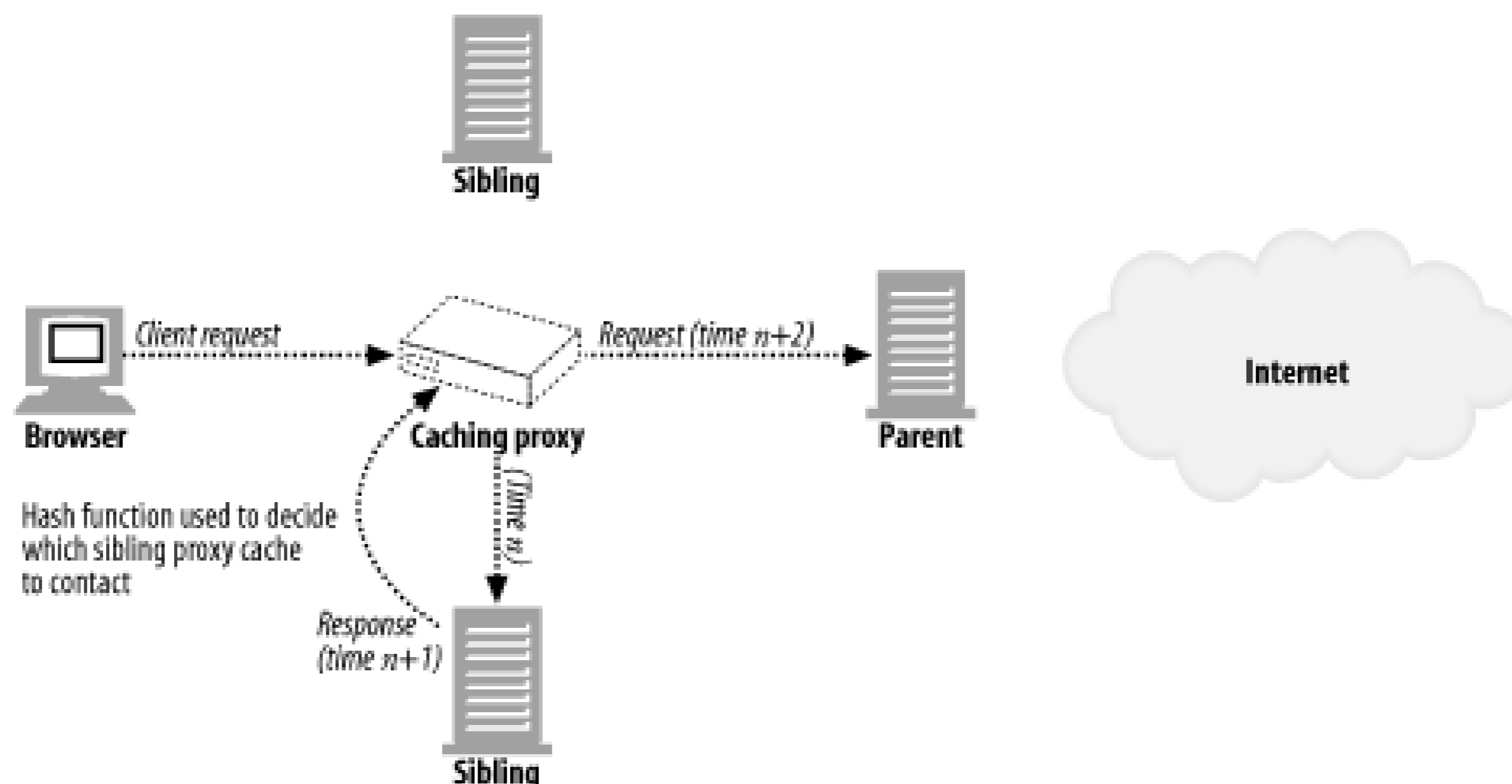
Figure 20-14. CARP redirection
