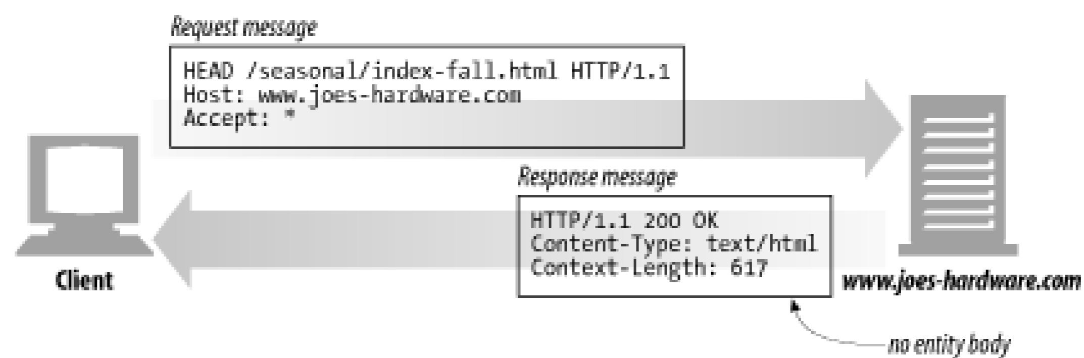
Figure 3-8. HEAD example
