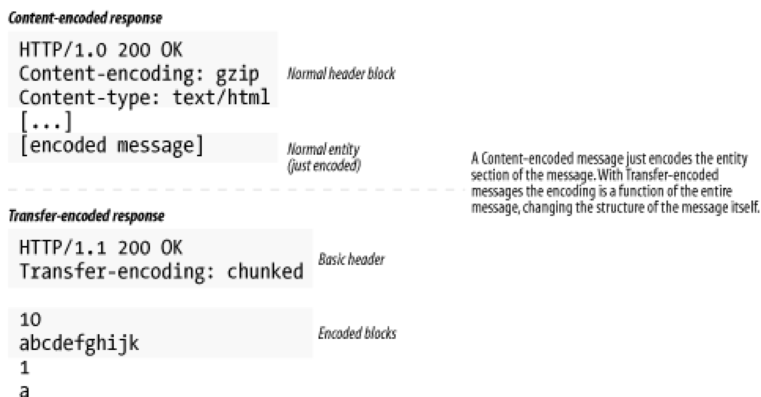
Figure 15-5. Content encodings versus transfer encodings
