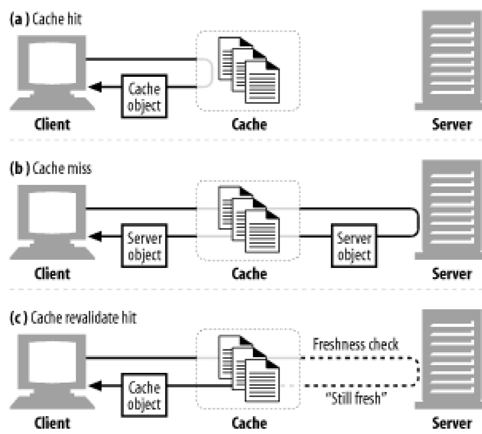
Figure 7-4. Cache hits, misses, and revalidations
