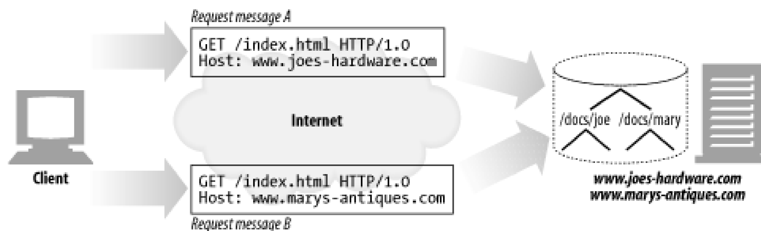
Figure 5-9. Different docroots for virtually hosted requests
