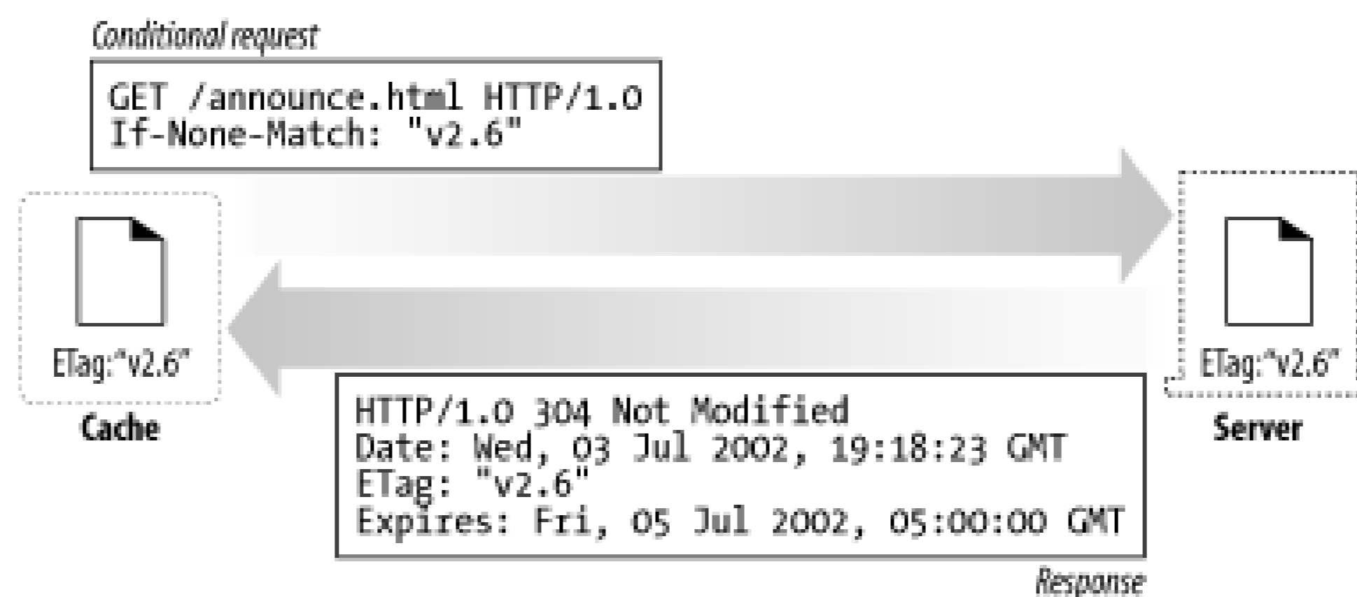
Figure 7-15. If-None-Match revalidates because entity tag still matches
