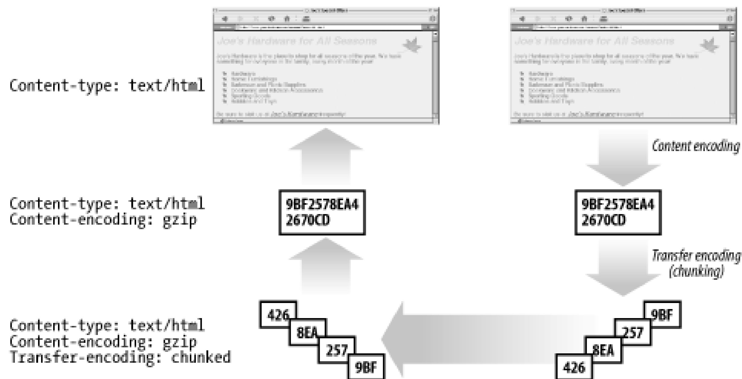
Figure 15-7. Combining content encoding with transfer encoding
