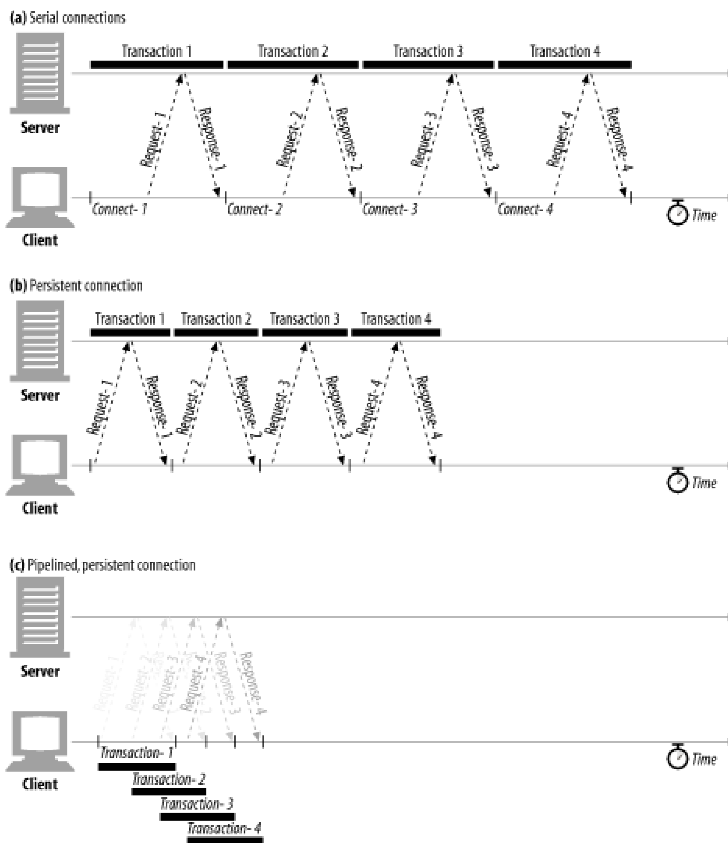
Figure 4-18. Four transactions (pipelined connections)
