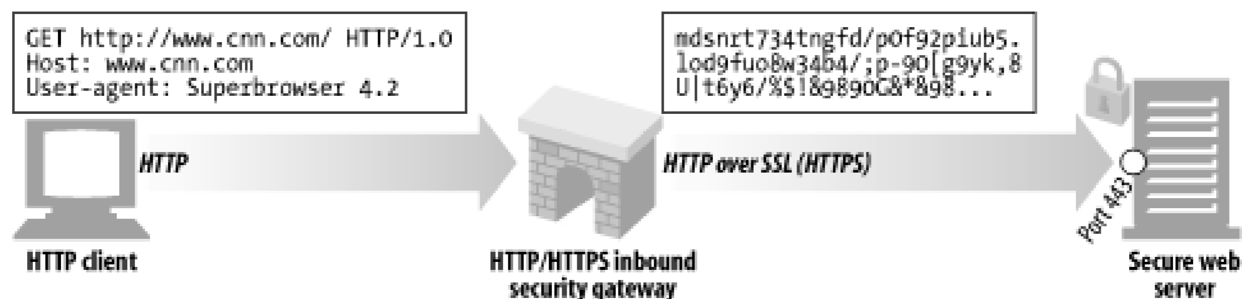
Figure 8-6. Inbound HTTP/HTTPS security gateway
