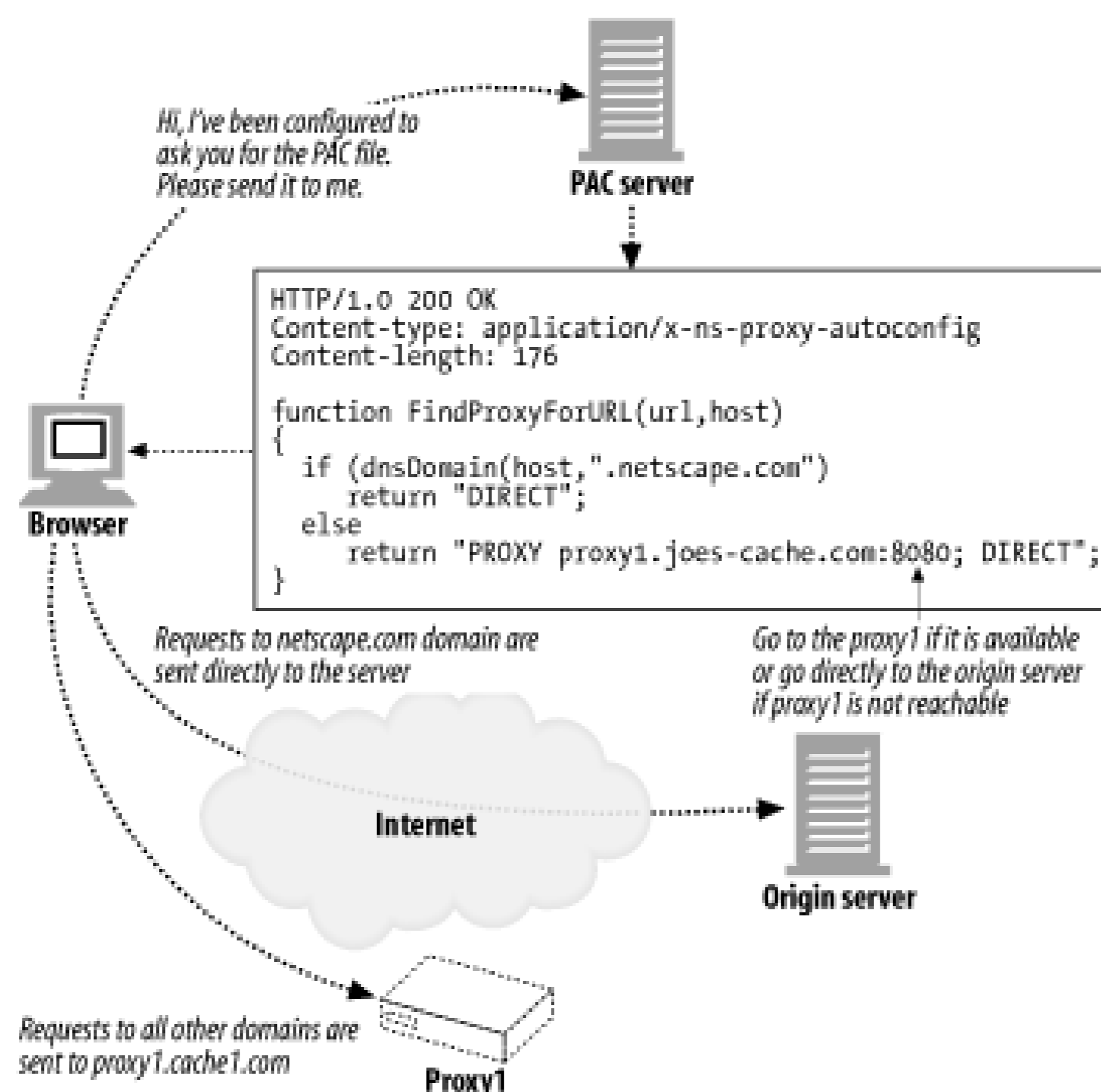
Figure 20-10. Proxy auto-configuration
