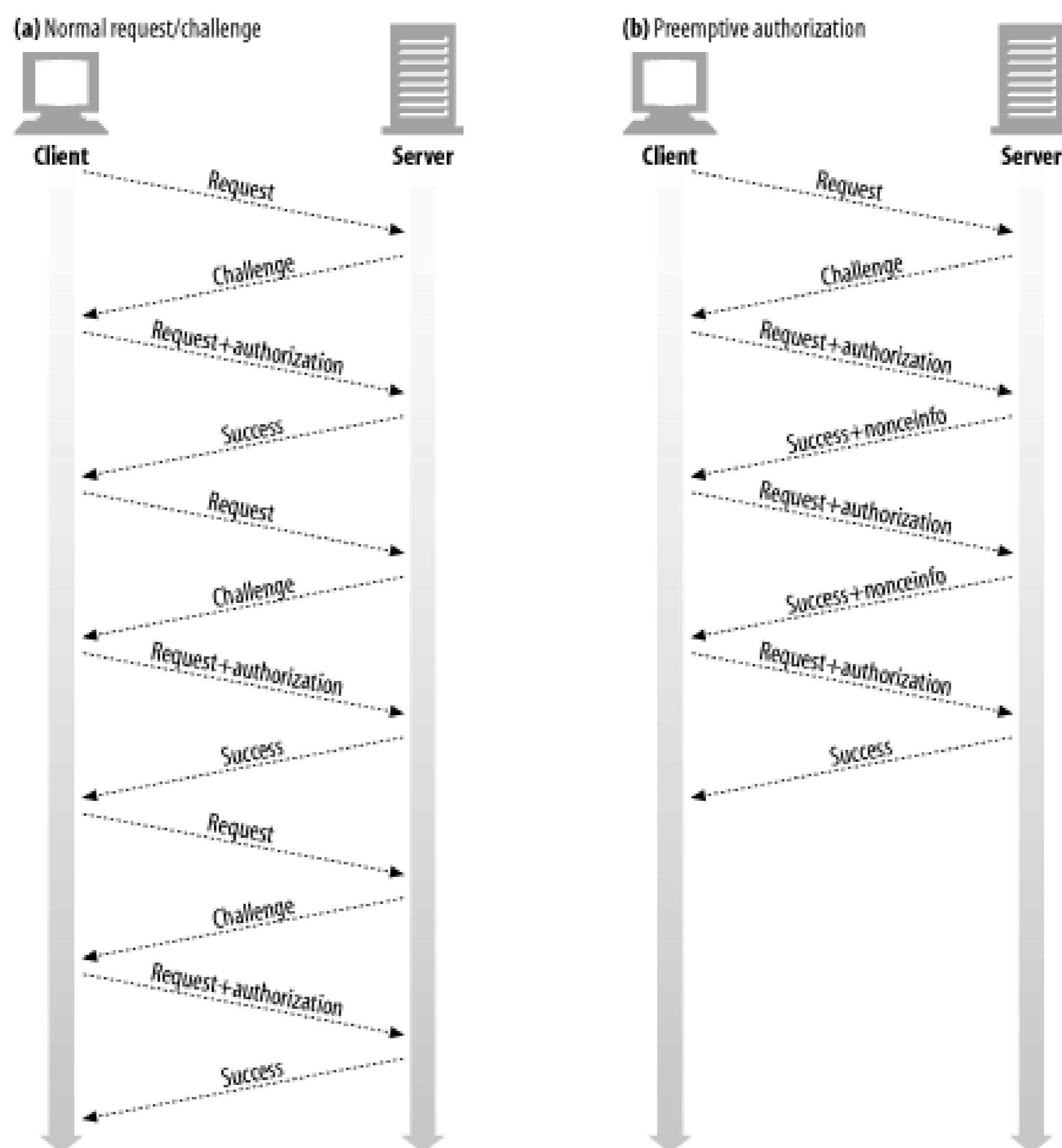
Figure 13-4. Preemptive authorization reduces message count
