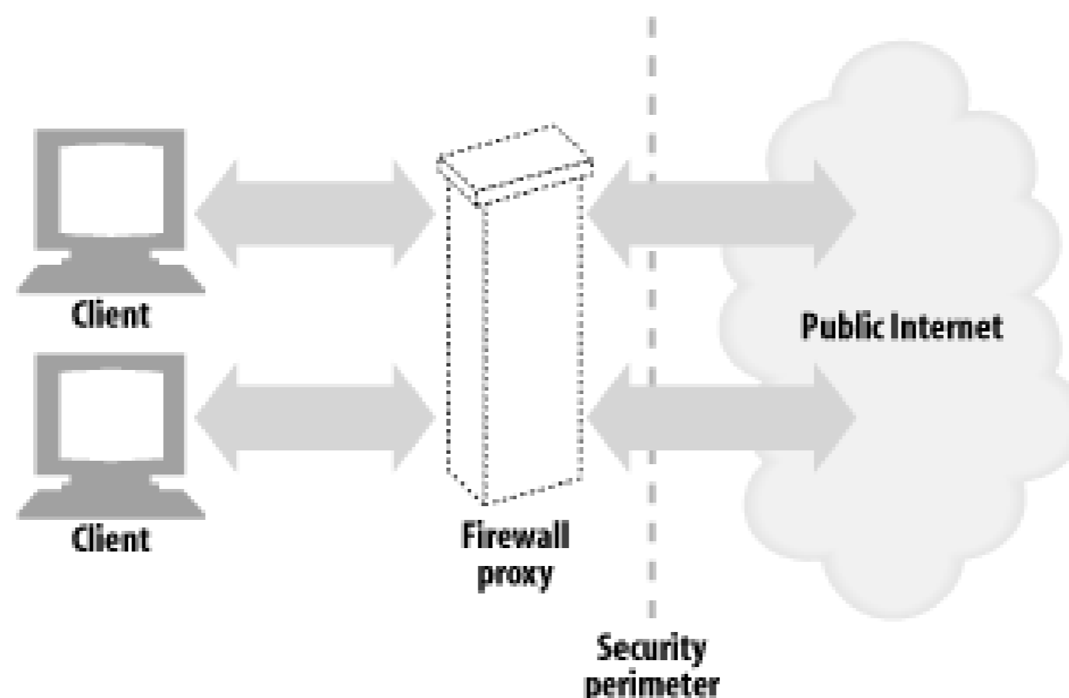
Figure 14-19. Corporate firewall proxy
