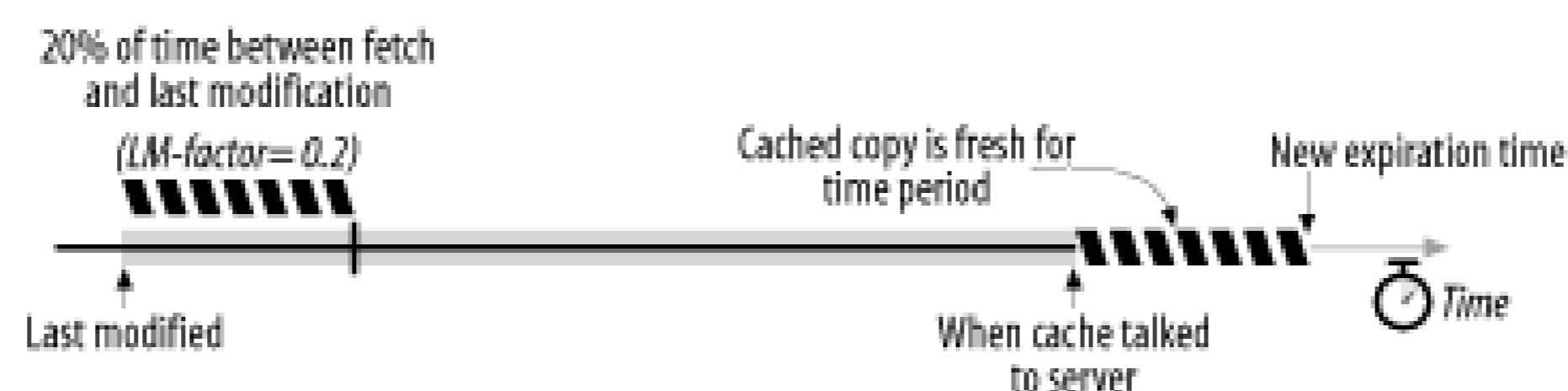
Figure 7-16. Computing a freshness period using the LM-Factor algorithm
