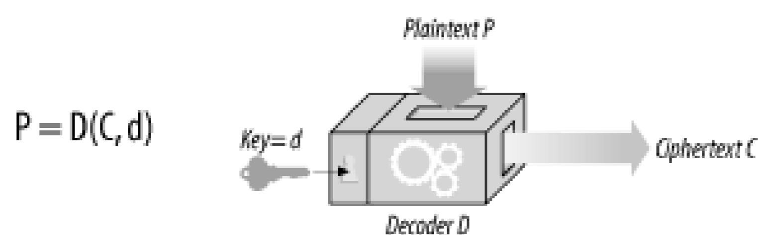
Figure 14-7. Symmetric-key cryptography algorithms use the same key for encoding and decoding
