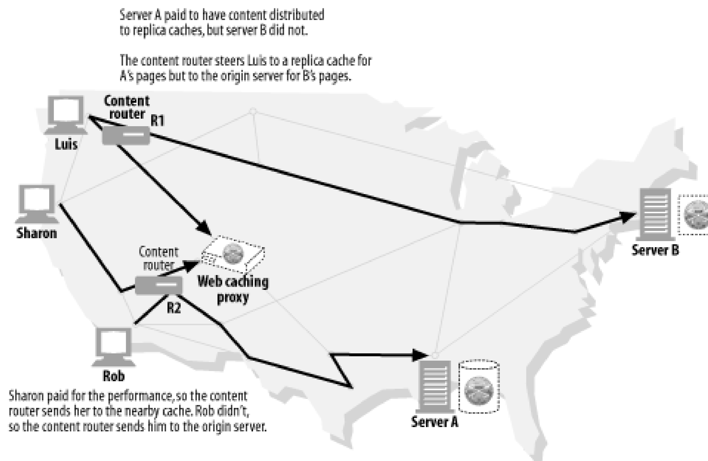
Figure 6-8. Proxy application example: content routing
