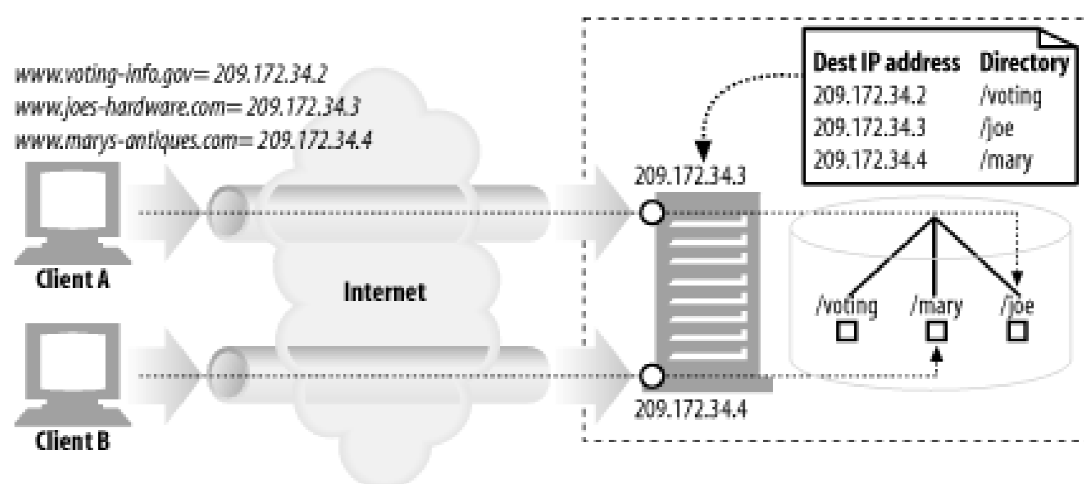
Figure 18-4. Virtual IP hosting
