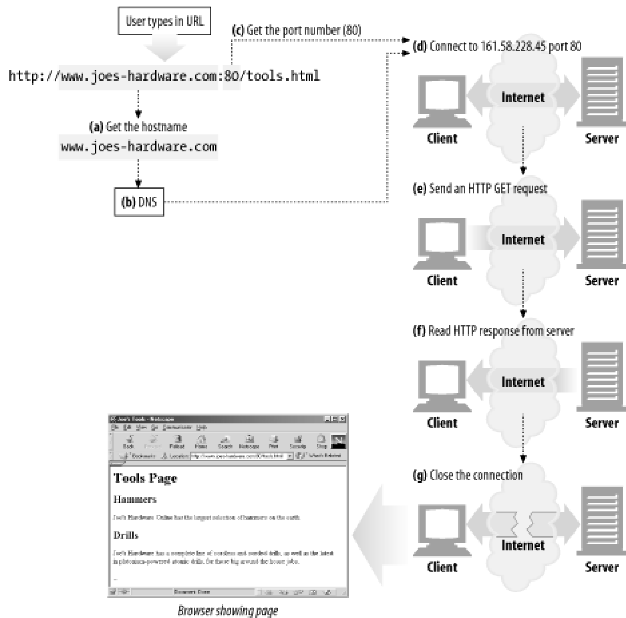
Figure 1-10. Basic browser connection process
