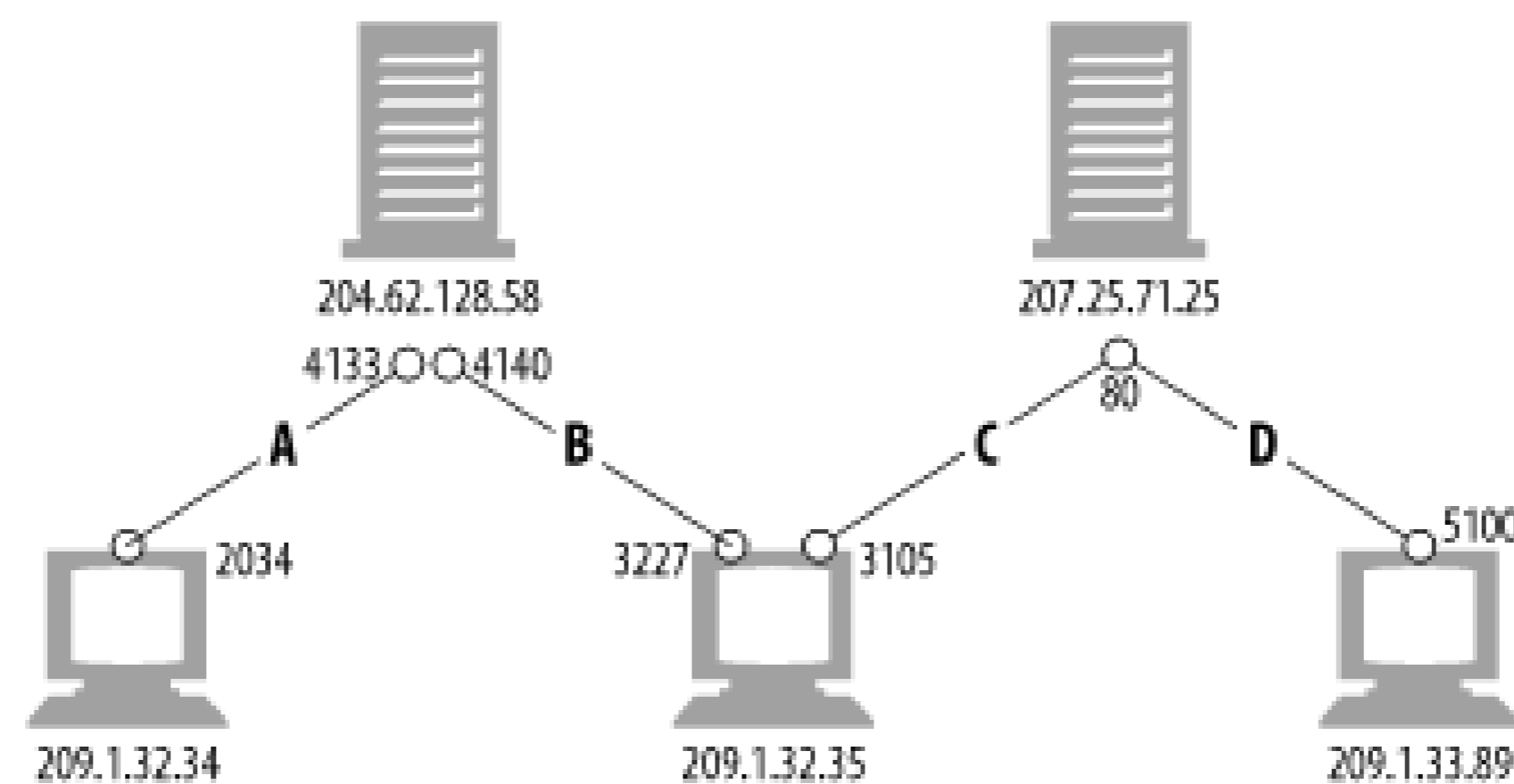
Figure 4-5. Four distinct TCP connections
