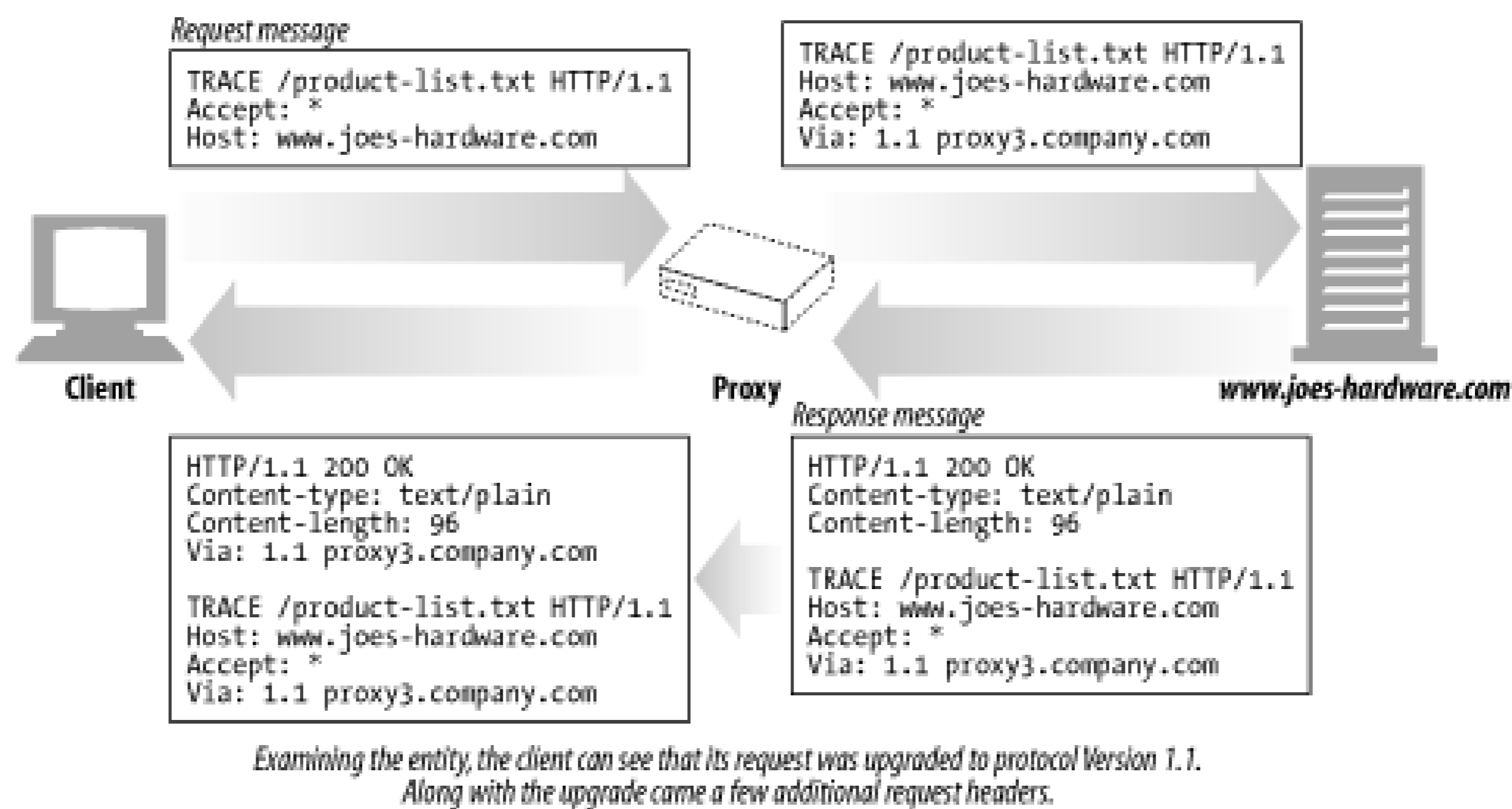
Figure 3-11. TRACE example
