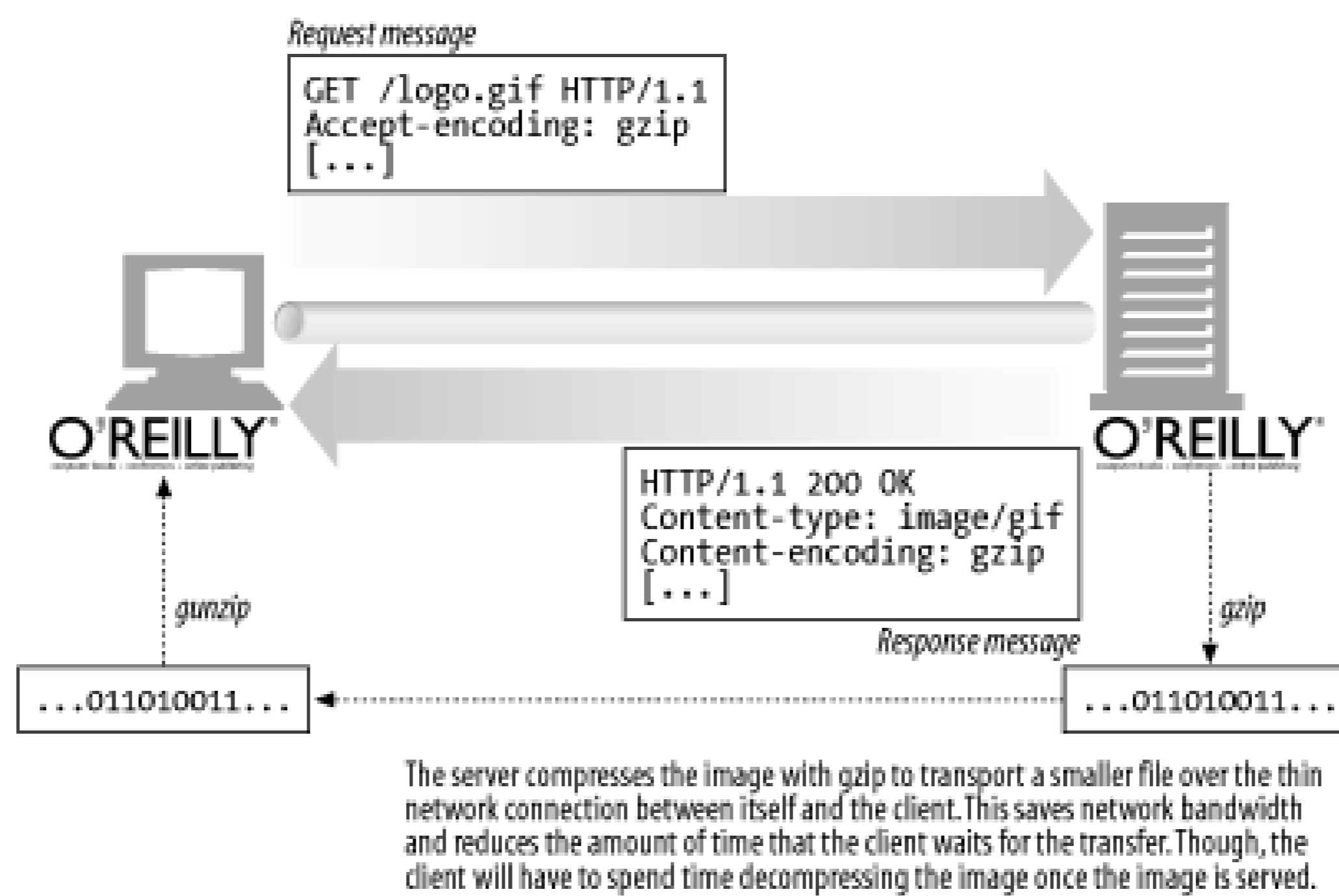
Figure 15-4. Content encoding
