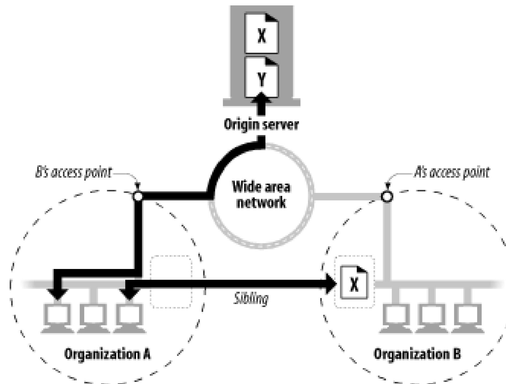
Figure 7-10. Sibling caches
