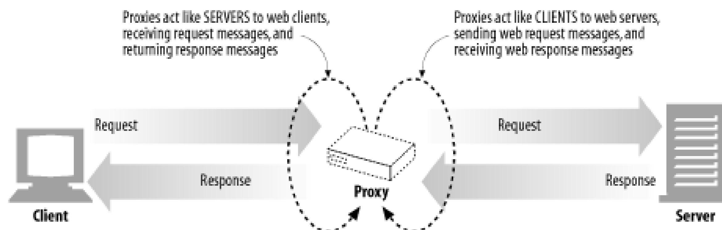
Figure 6-1. A proxy must be both a server and a client
