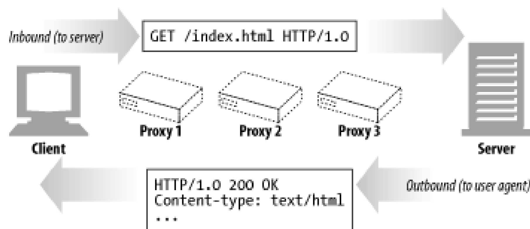
Figure 3-1. Messages travel inbound to the origin server and outbound back to the client
