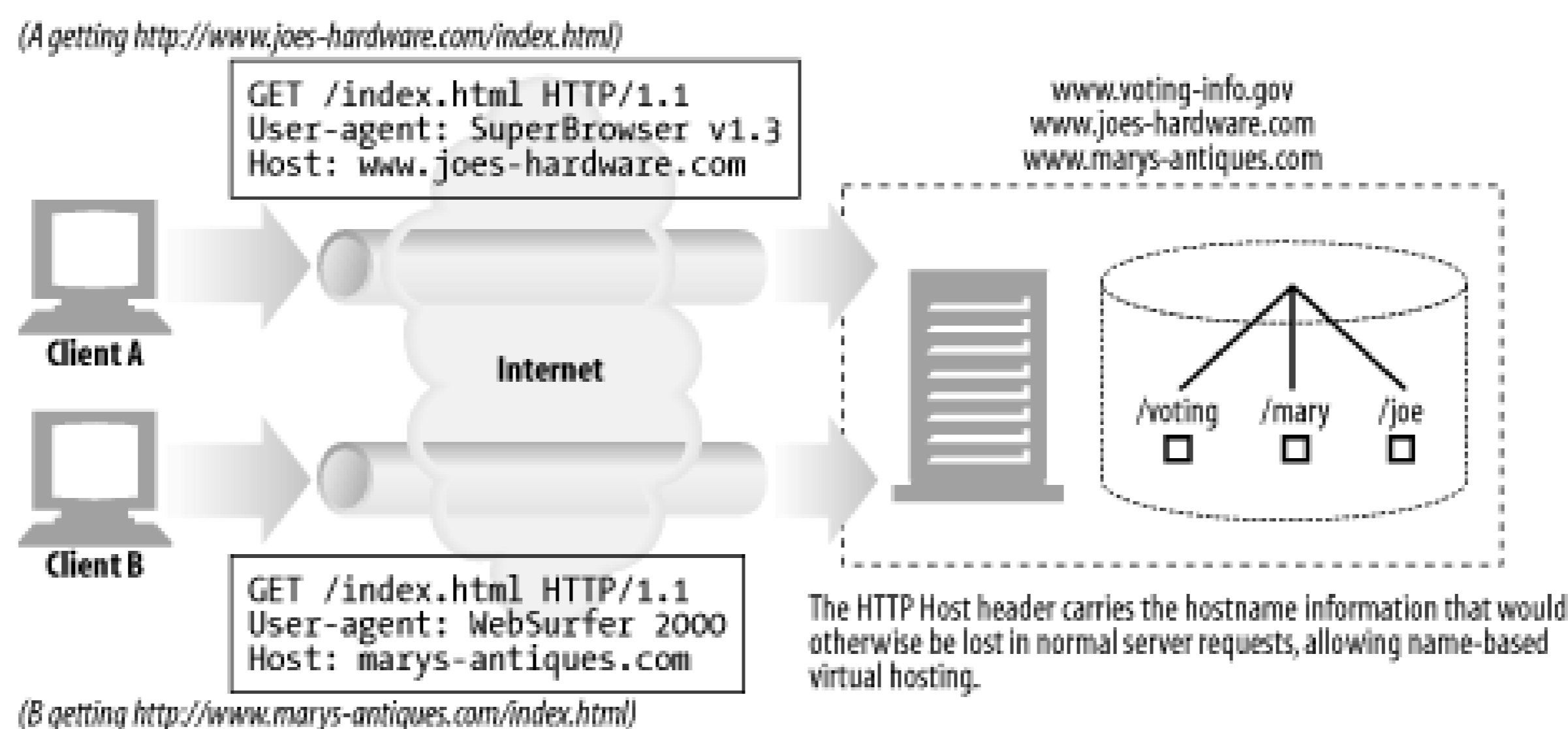
Figure 18-5. Host headers distinguish virtual host requests
