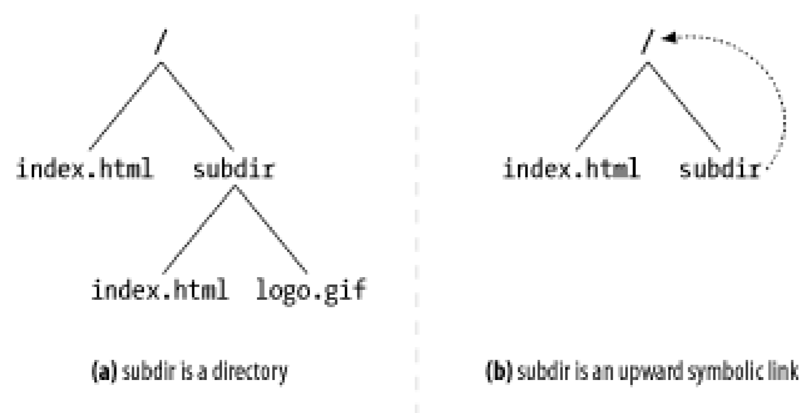
Figure 9-3. Symbolic link cycles
