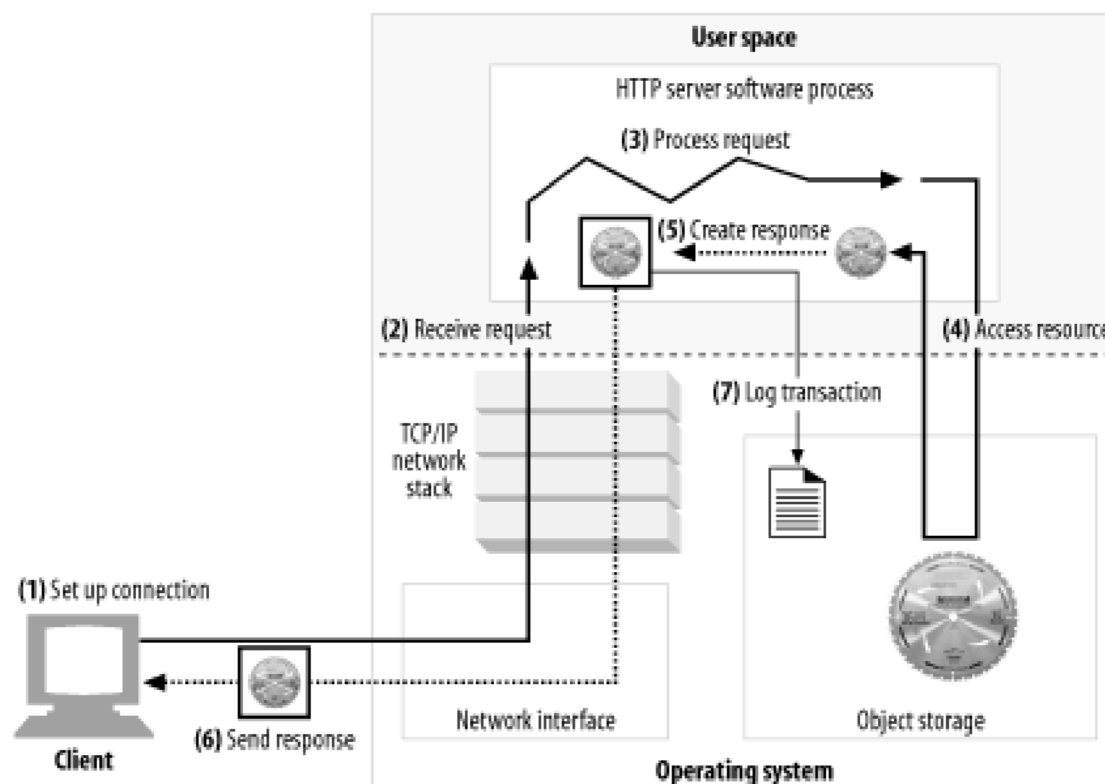
Figure 5-3. Steps of a basic web server request
