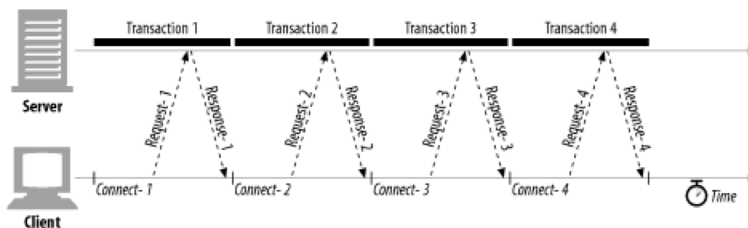
Figure 4-10. Four transactions (serial)
