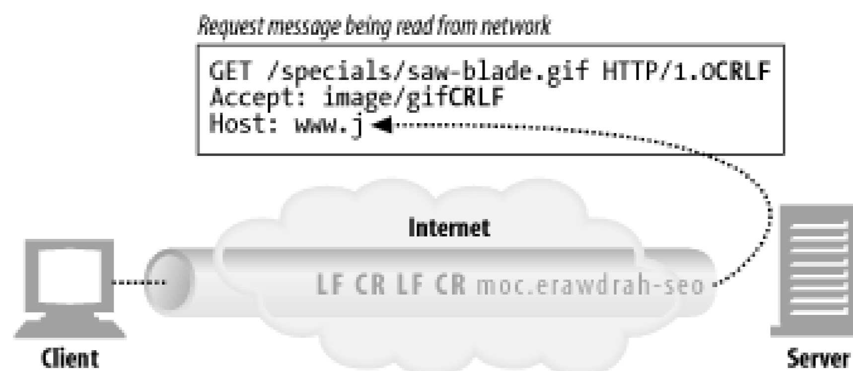
Figure 5-5. Reading a request message from a connection
