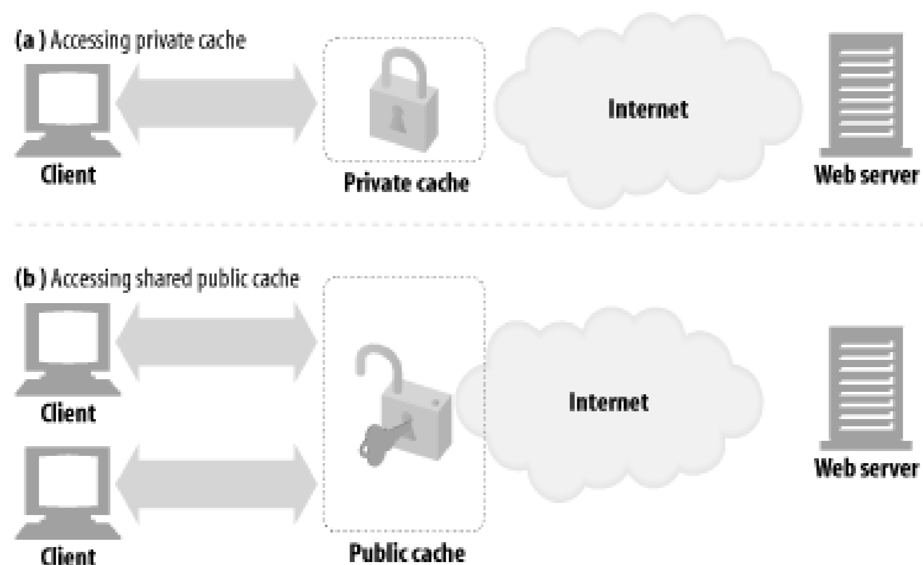
Figure 7-7. Public and private caches
