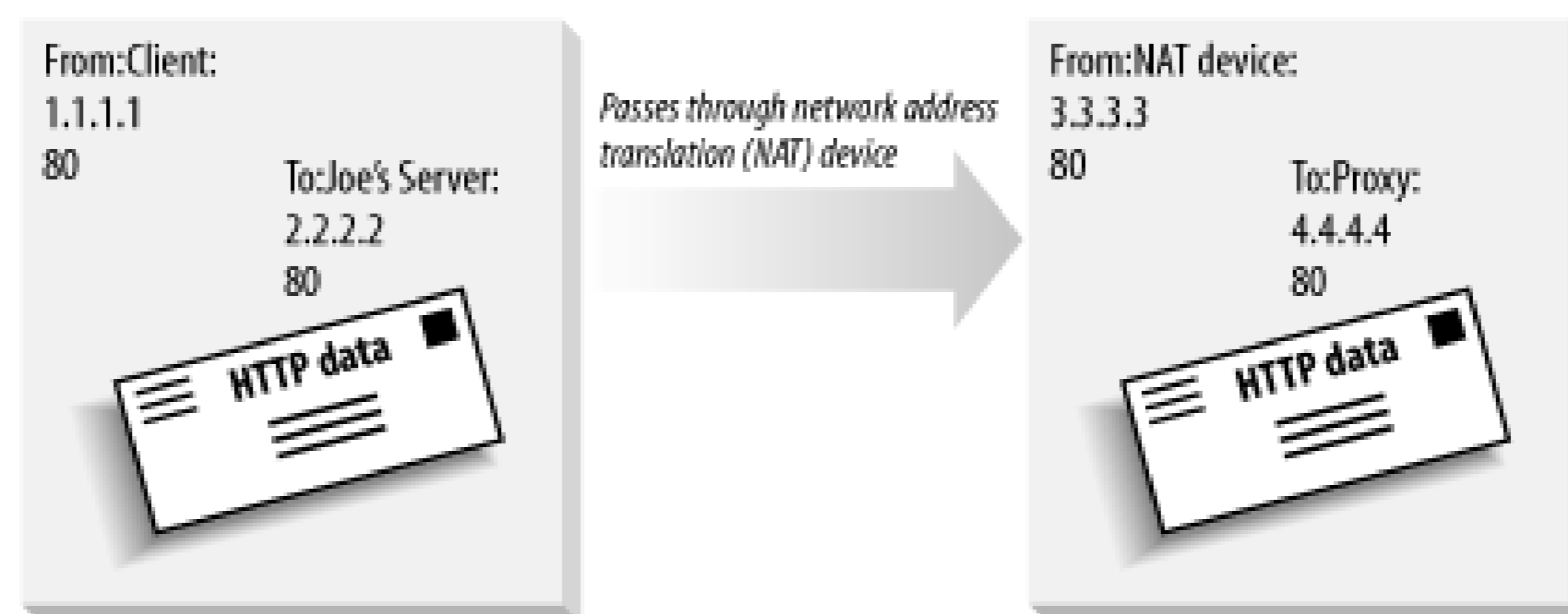
Figure 20-9. Full NAT of a TCP/IP datagram
