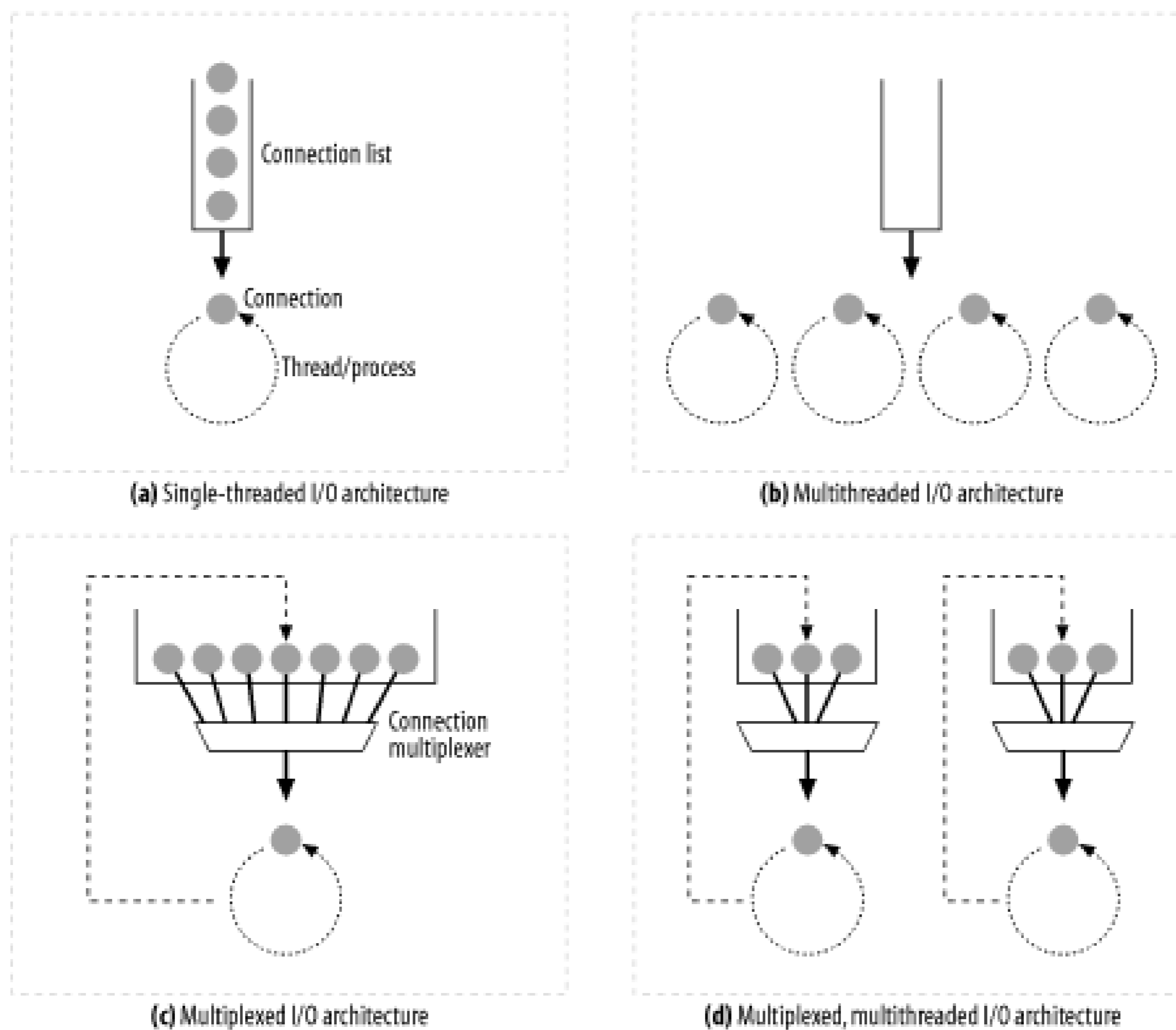
Figure 5-7. Web server input/output architectures
