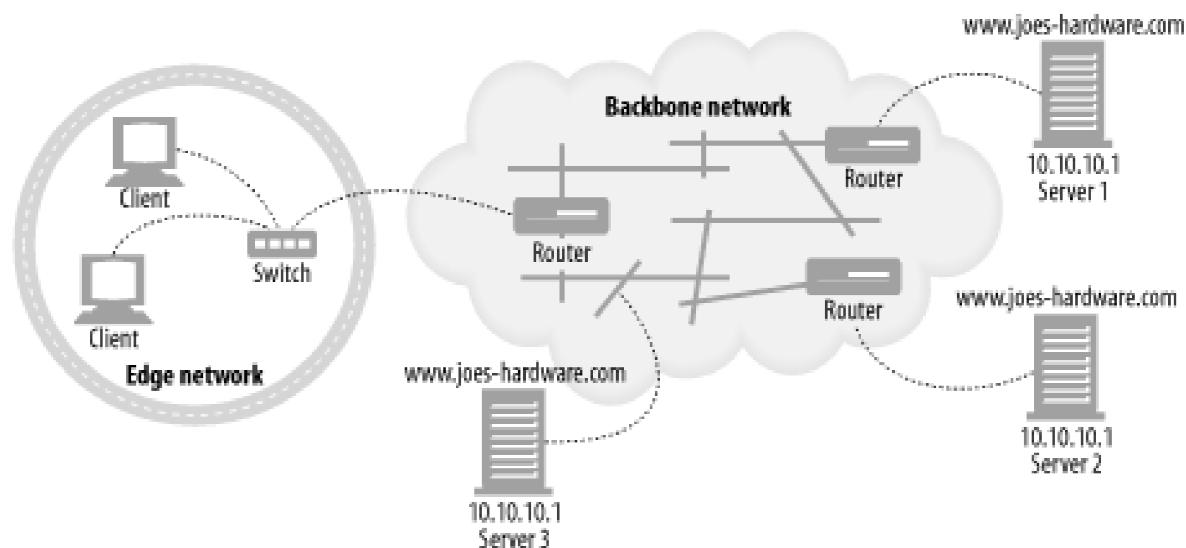
Figure 20-5. Distributed anycast addressing
