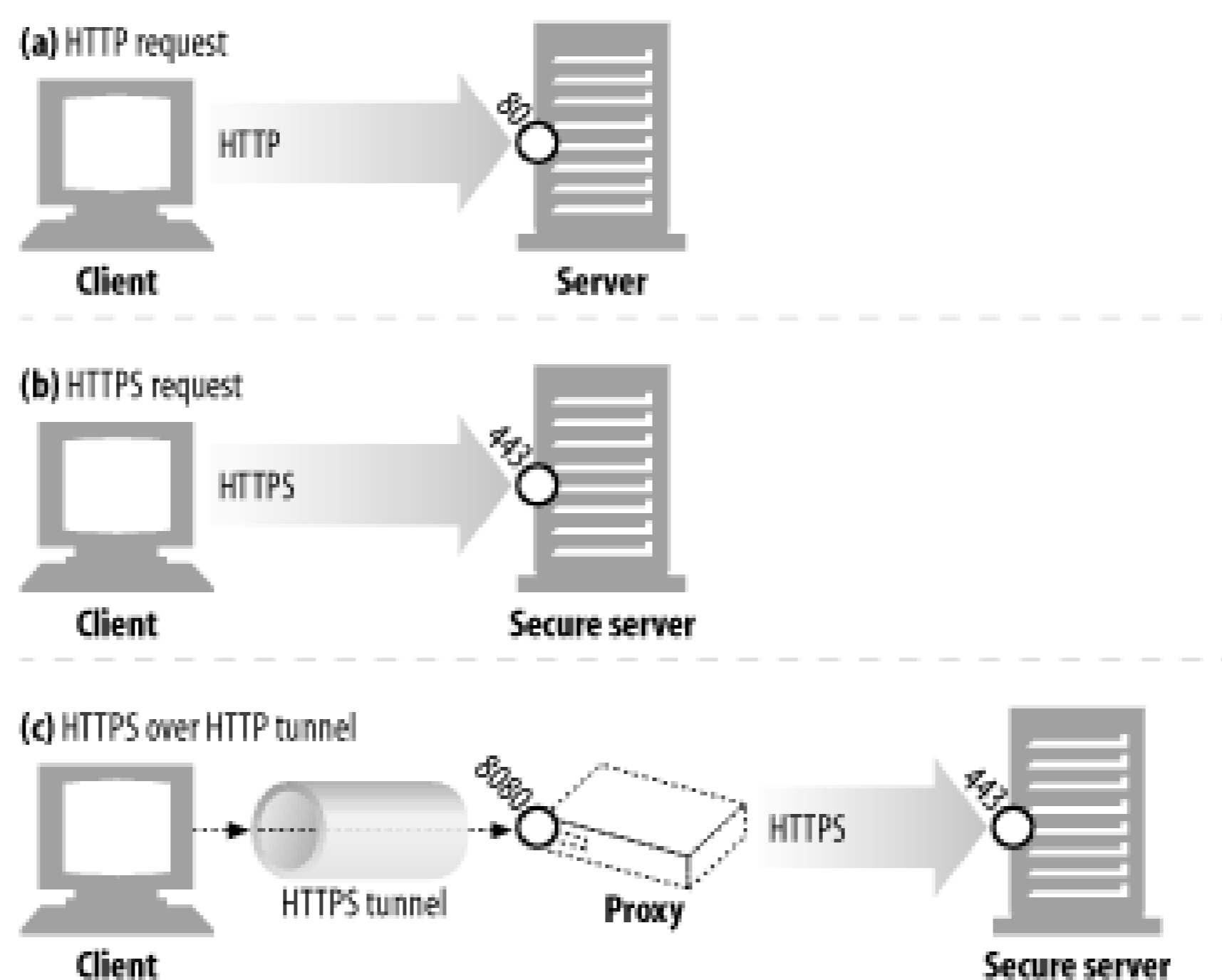
Figure 14-14. HTTP and HTTPS port numbers
