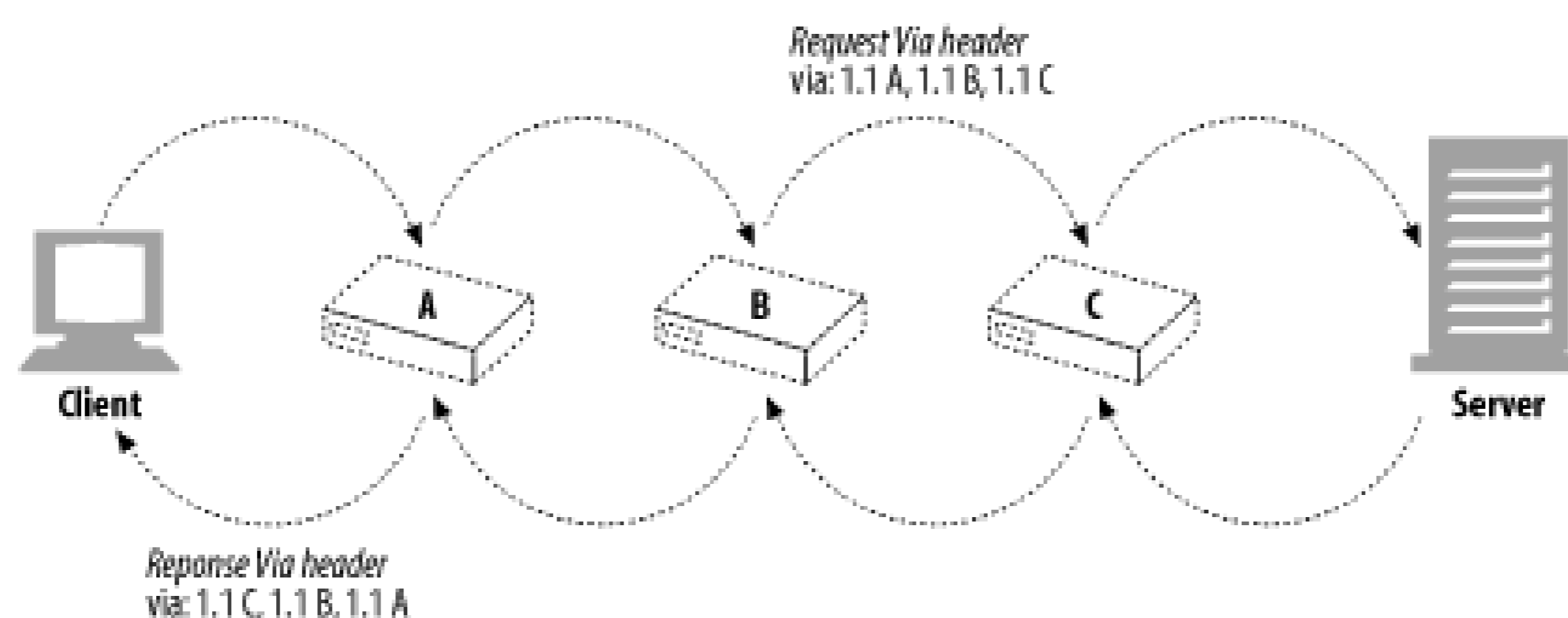
Figure 6-21. The response Via is usually the reverse of the request Via
