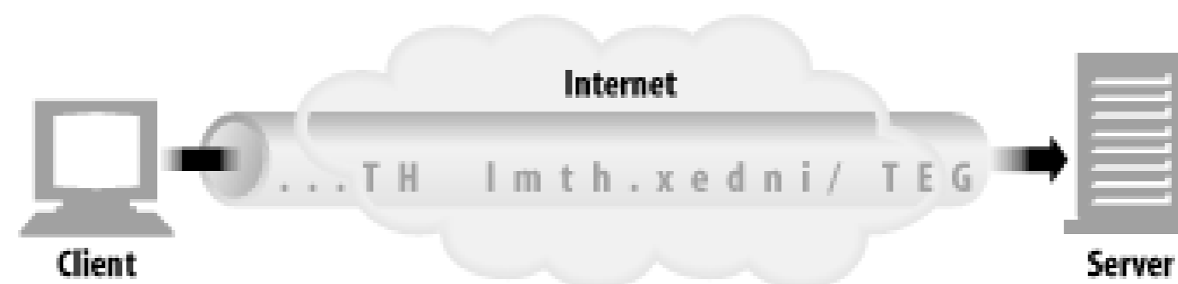
Figure 4-2. TCP carries HTTP data in order, and without corruption
