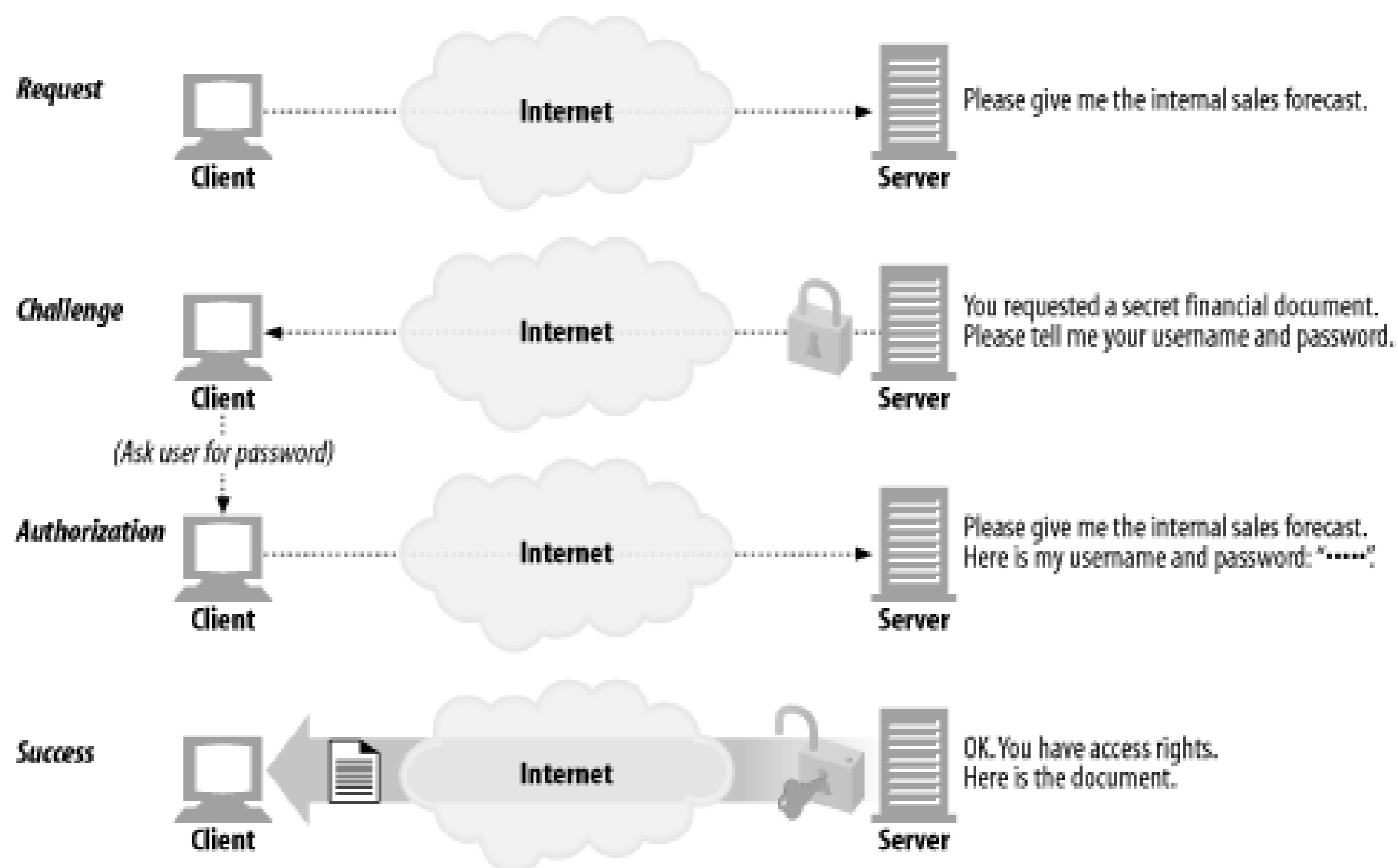
Figure 12-1. Simplified challenge/response authentication
