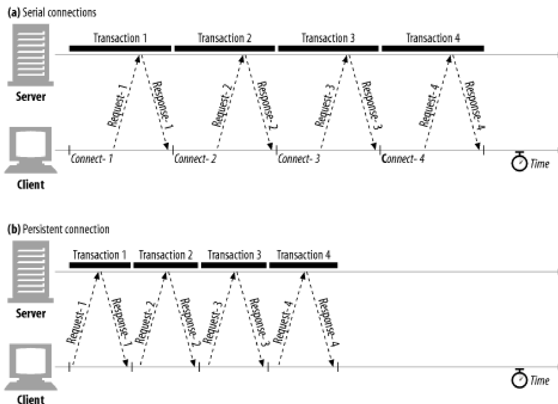
Figure 4-13. Four transactions (serial versus persistent)
