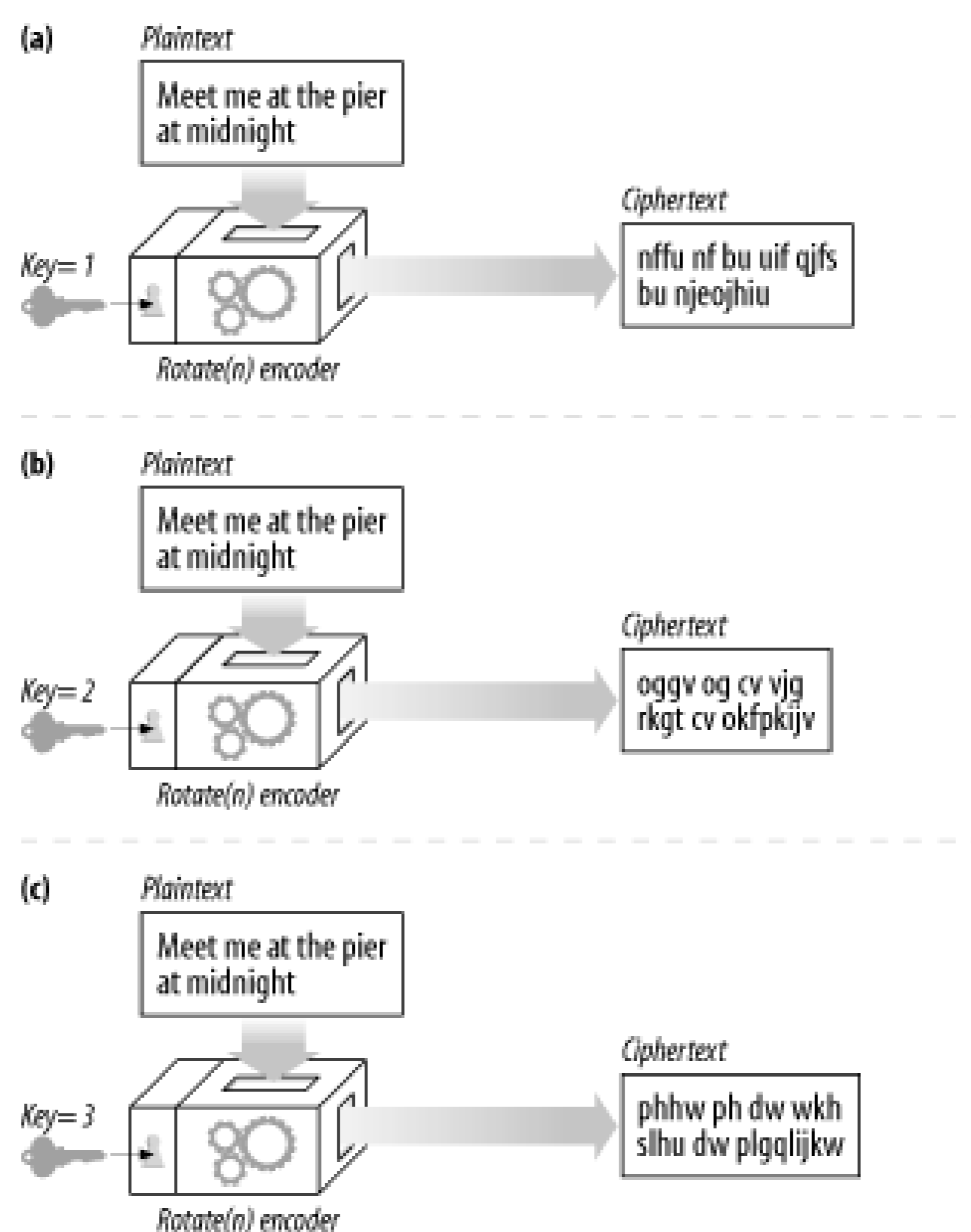
Figure 14-5. The rotate-by-N cipher, using different keys
