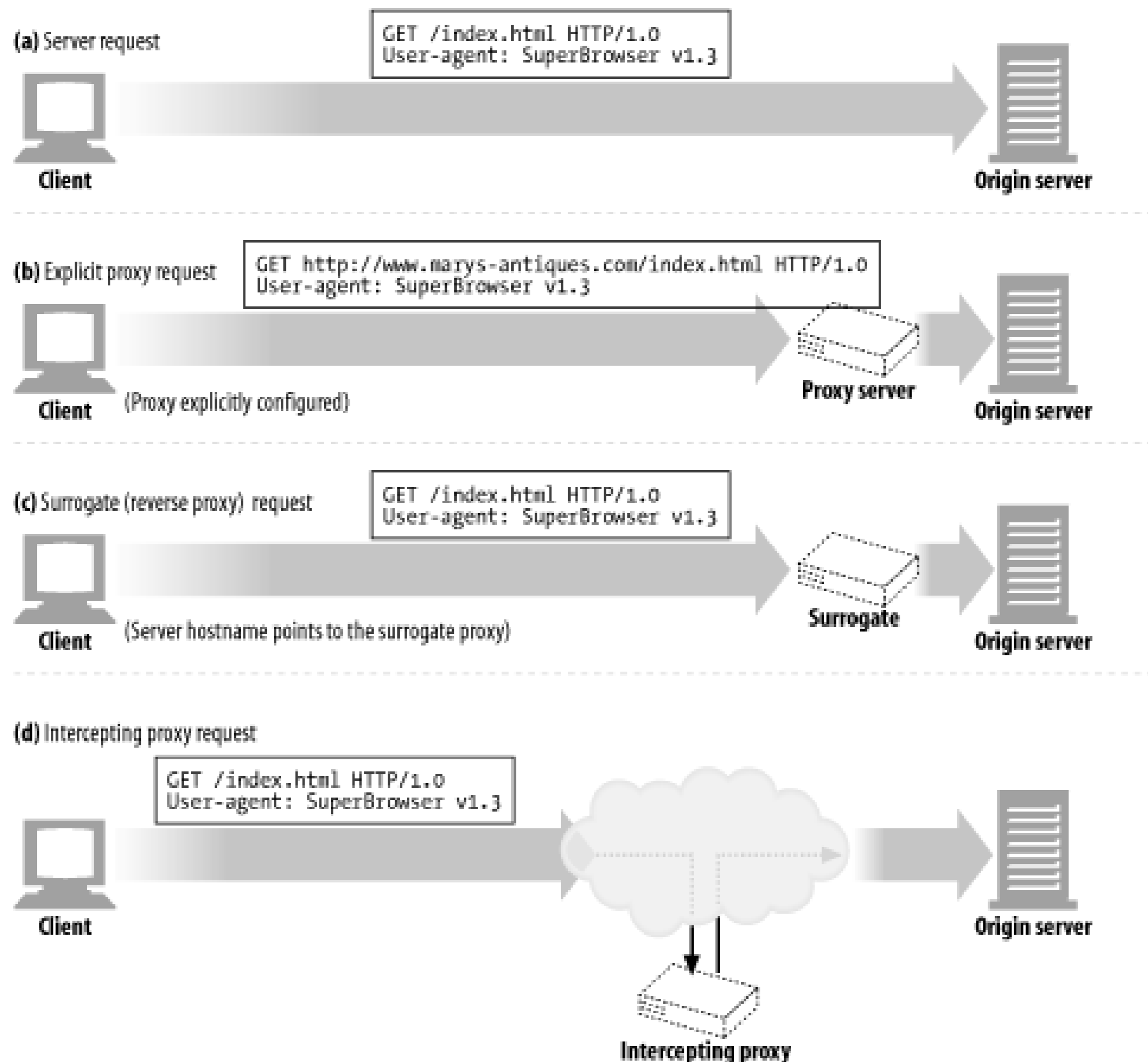
Figure 6-15. Intercepting proxies will get server requests
