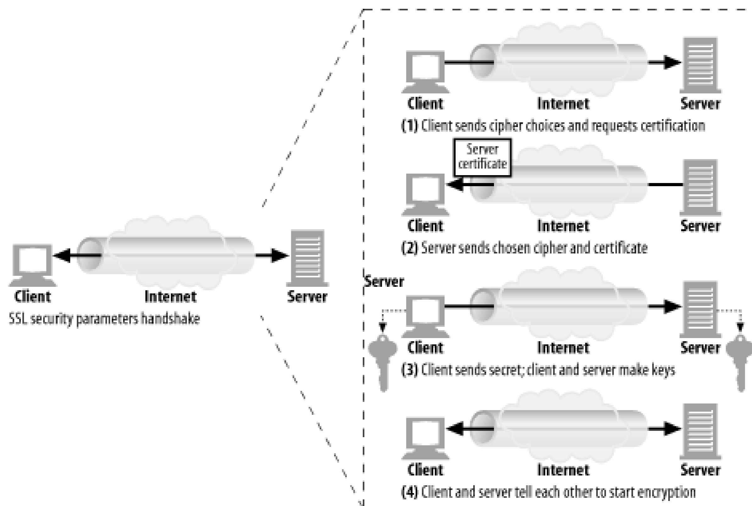
Figure 14-16. SSL handshake (simplified)
