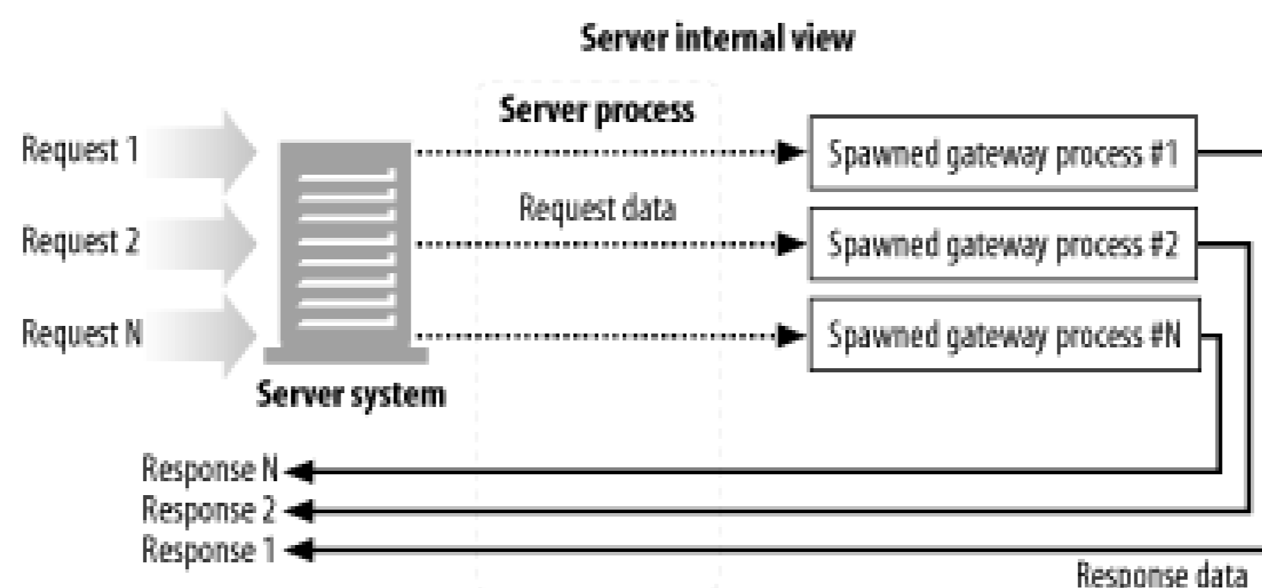
Figure 8-9. Server gateway application mechanics
