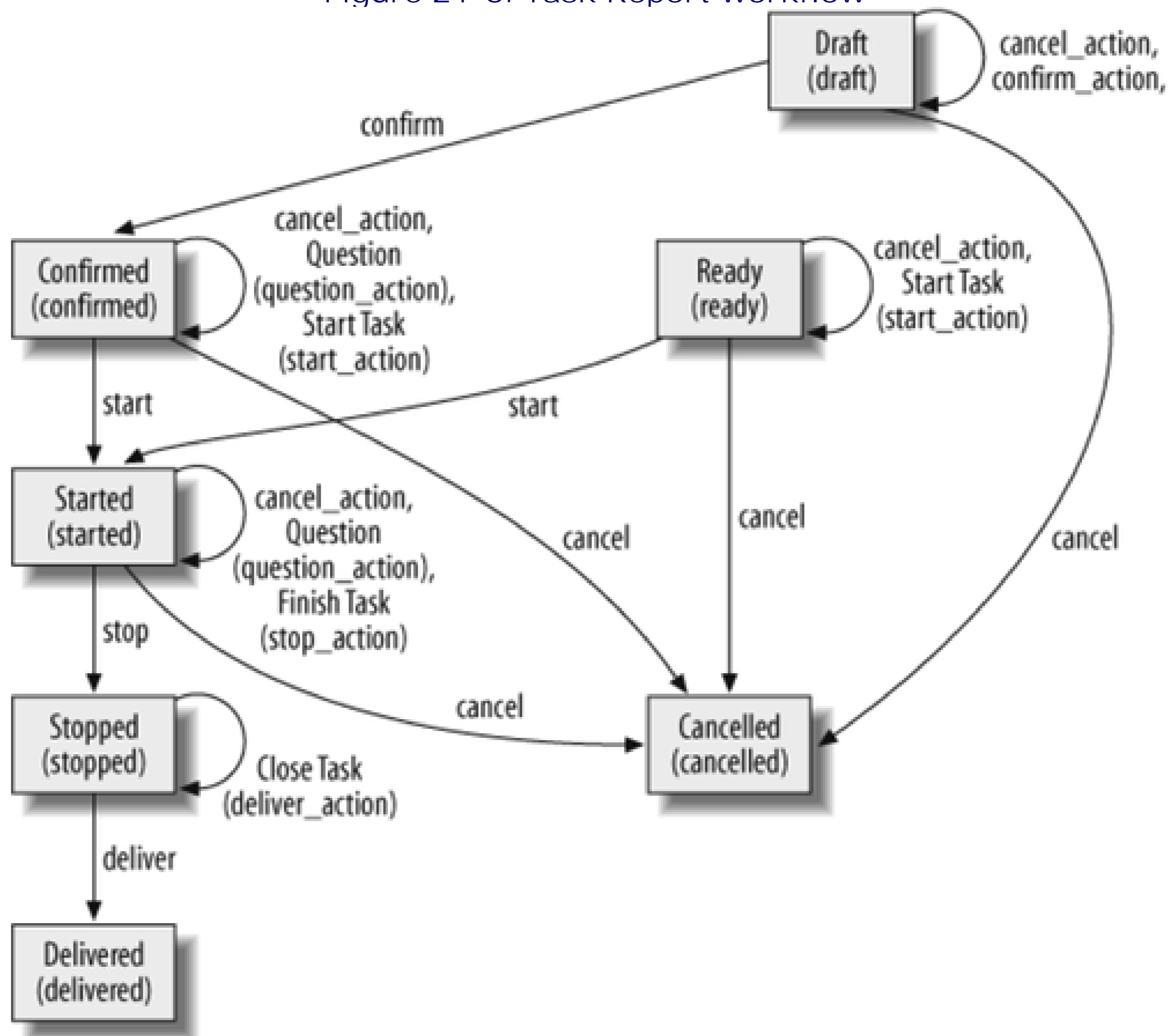
Figure 21-6. Task Report workflow
