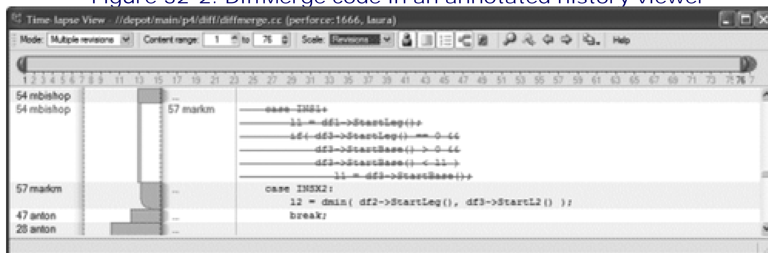
Figure 32-2. DiffMerge code in an annotated history viewer
