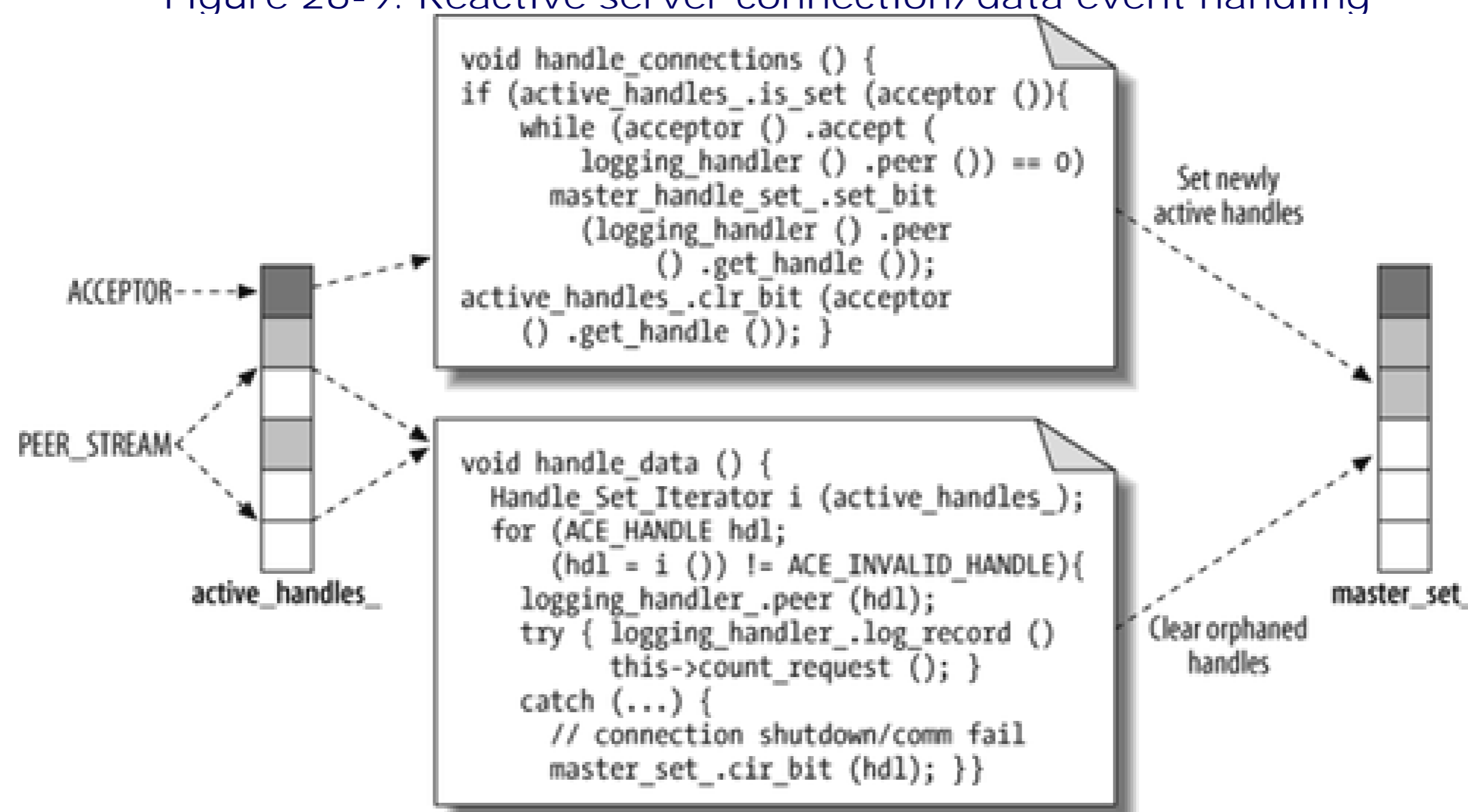
Figure 26-9. Reactive server connection/data event handling
