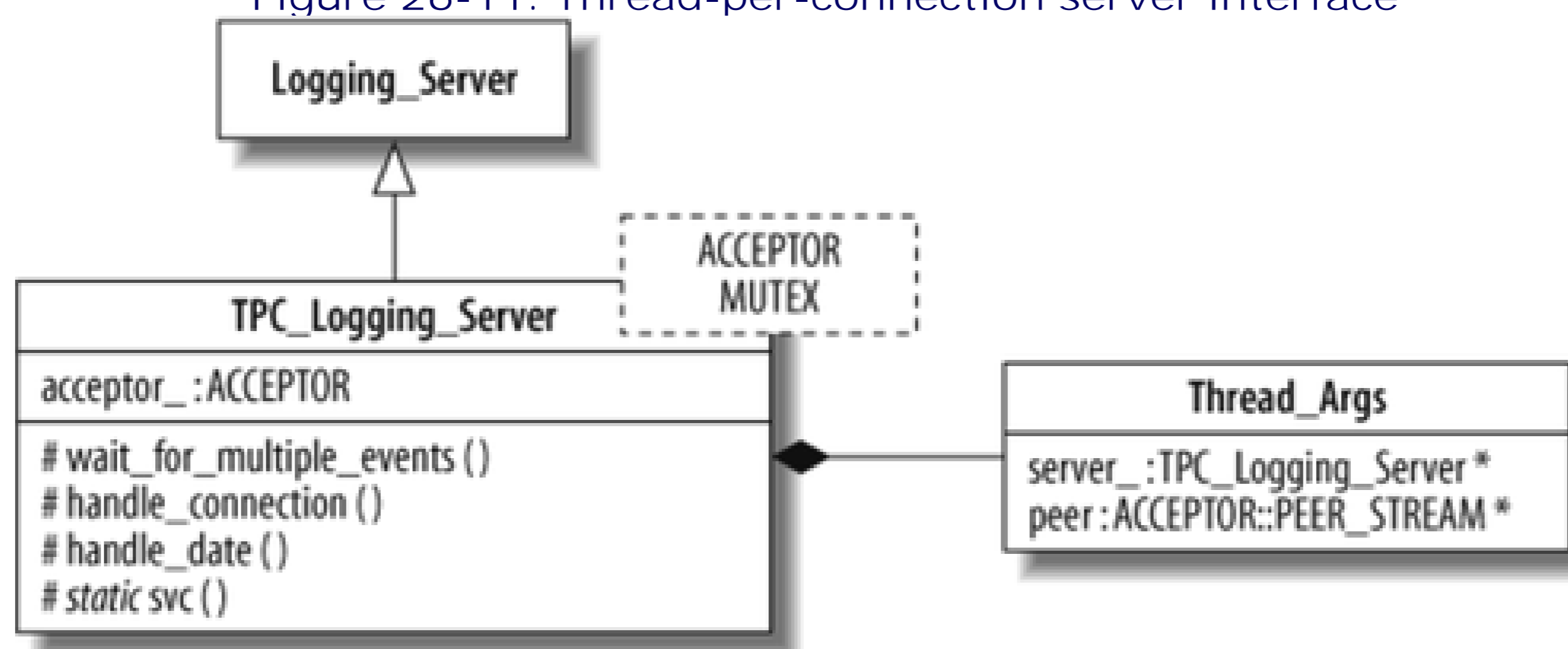
Figure 26-11. Thread-per-connection server interface
