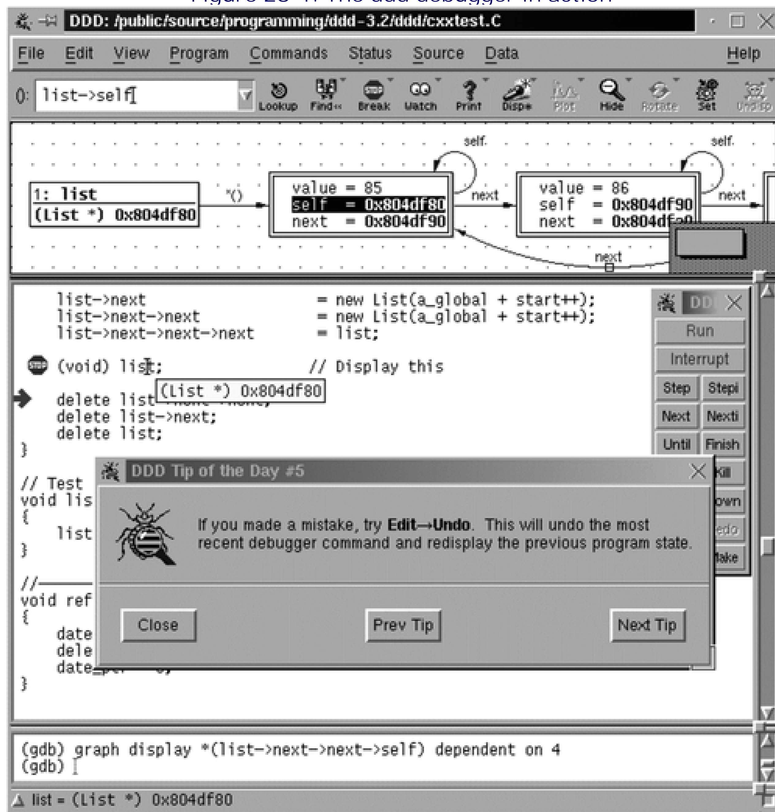
Figure 28-1. The ddd debugger in action
