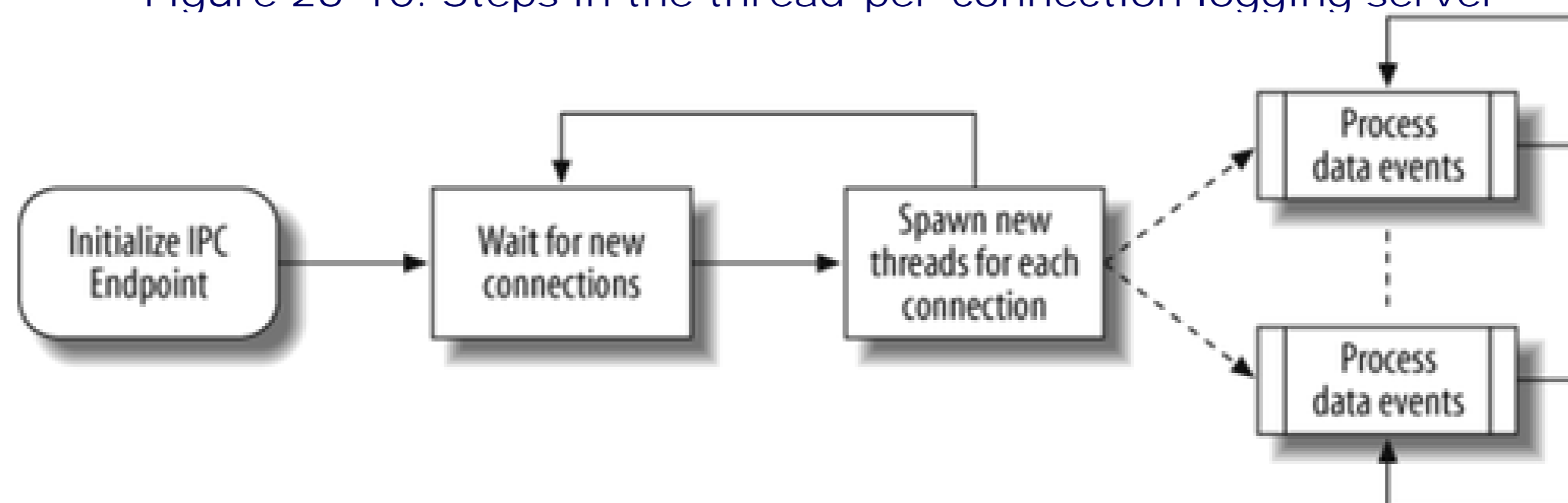
Figure 26-10. Steps in the thread-per-connection logging server
