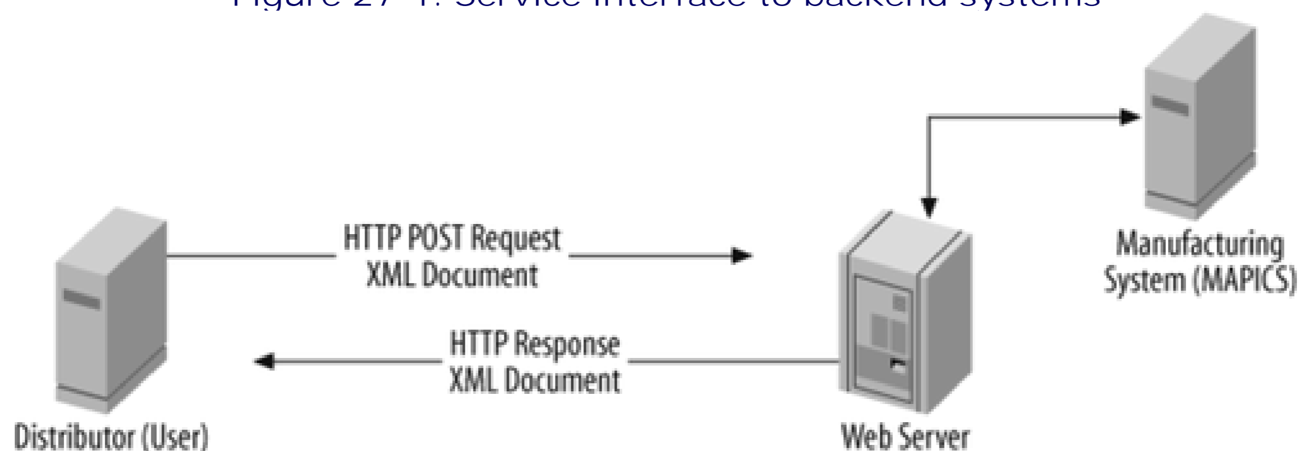
Figure 27-1. Service interface to backend systems
