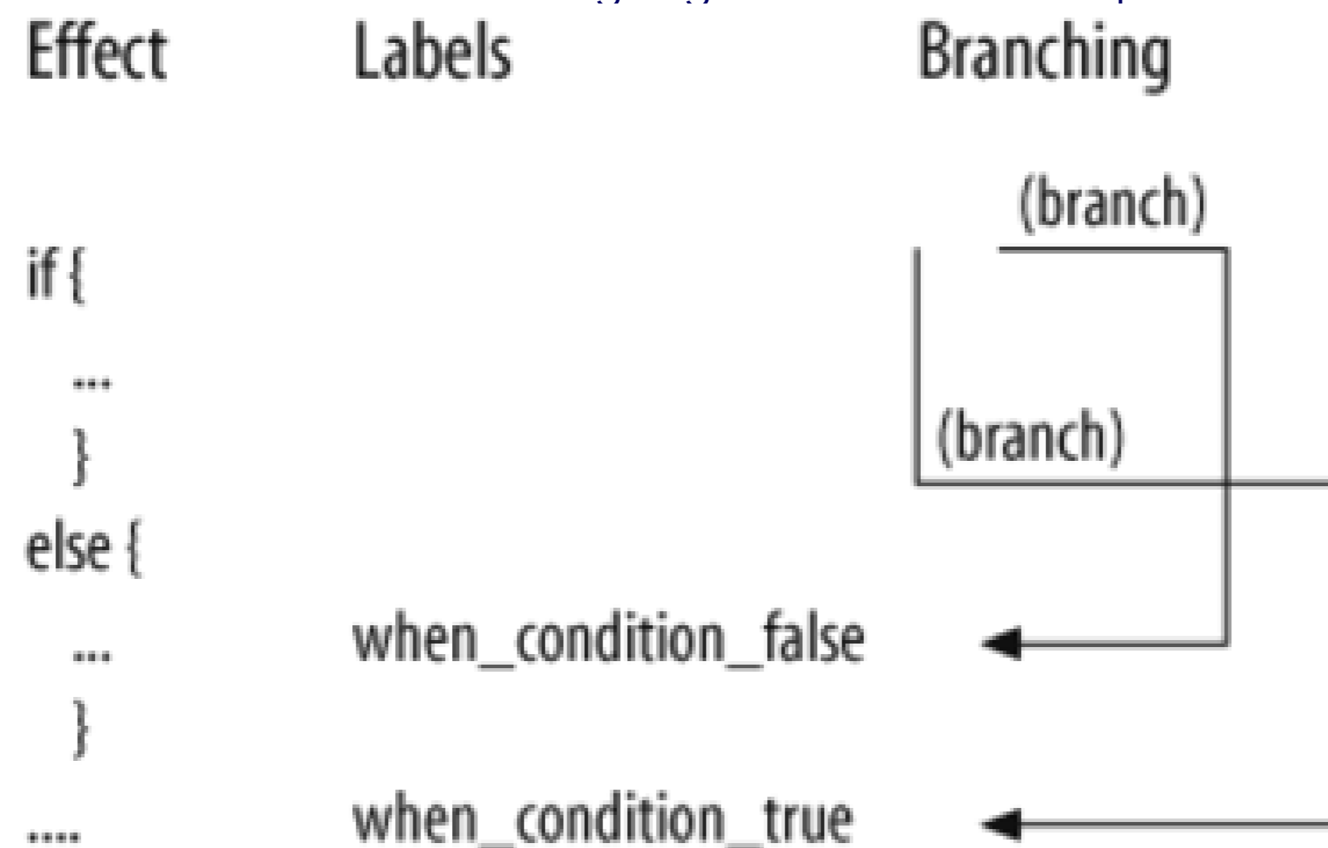
Figure 8-4. Intermediate Language branches to implement if/else
