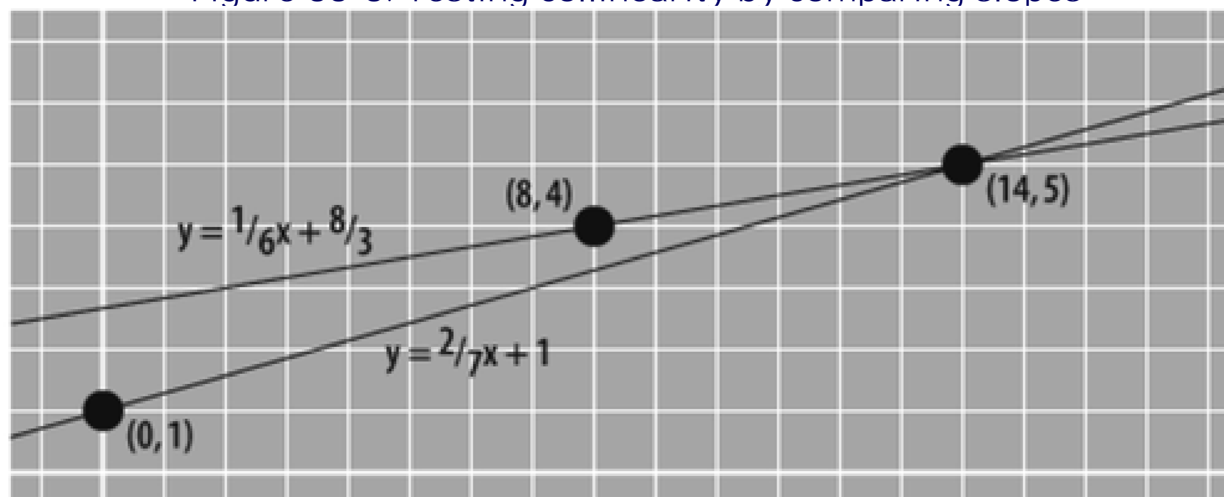
Figure 33-3. Testing collinearity by comparing slopes
