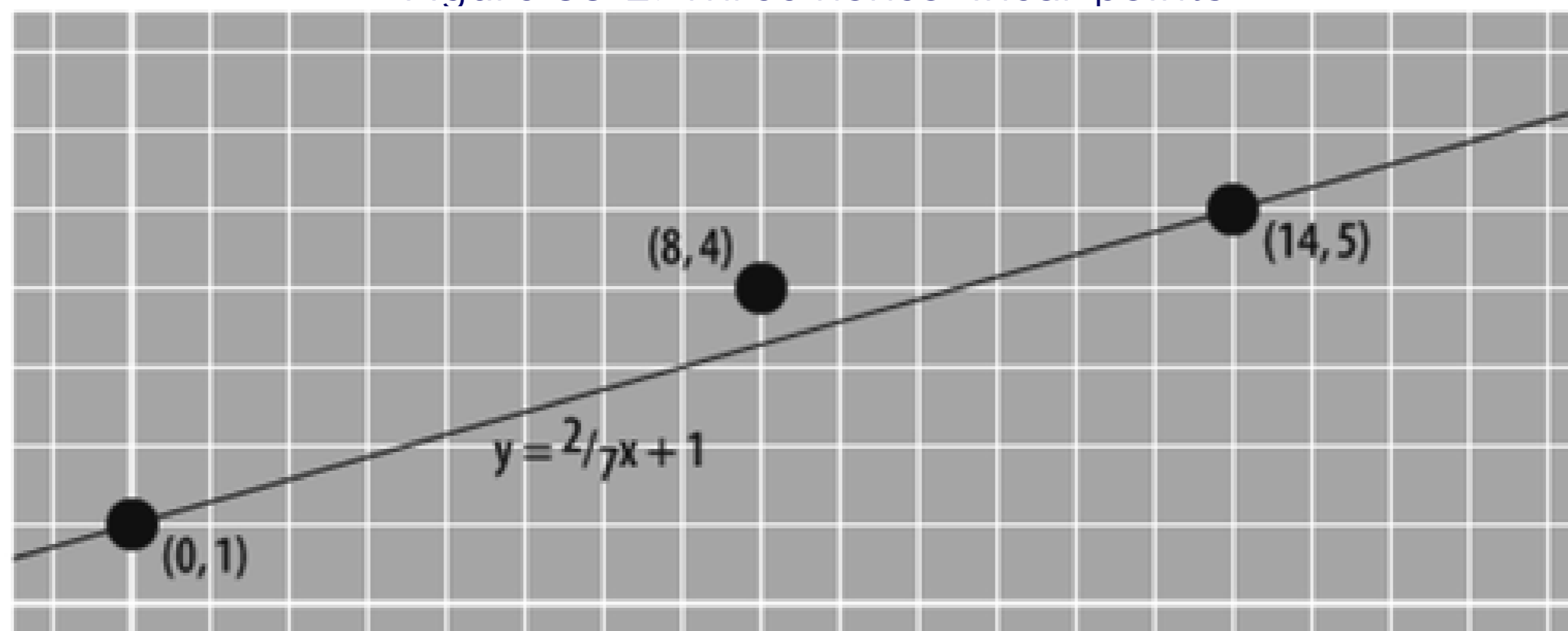
Figure 33-2. Three noncollinear points
