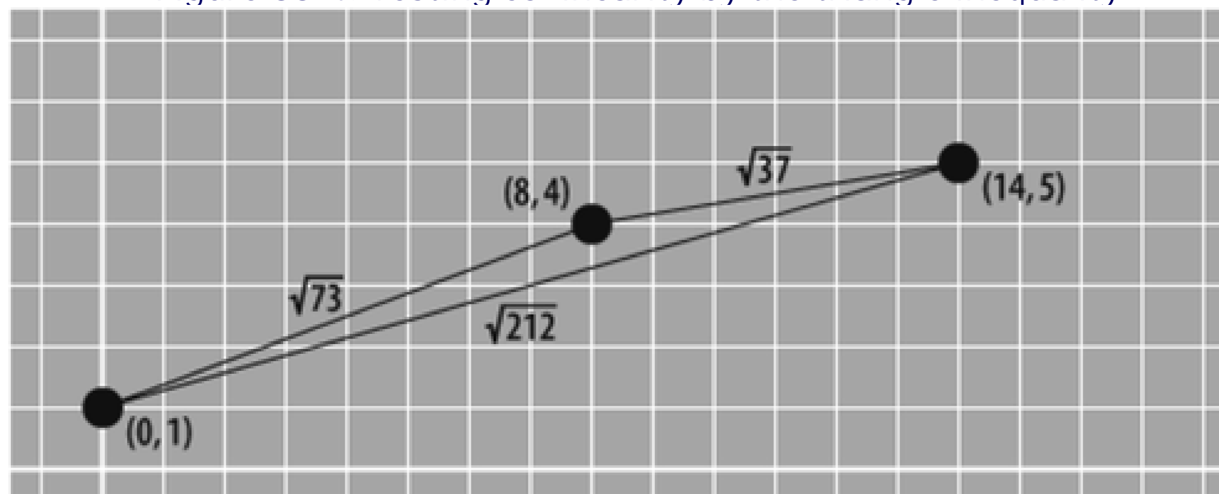
Figure 33-4. Testing collinearity by the triangle inequality
