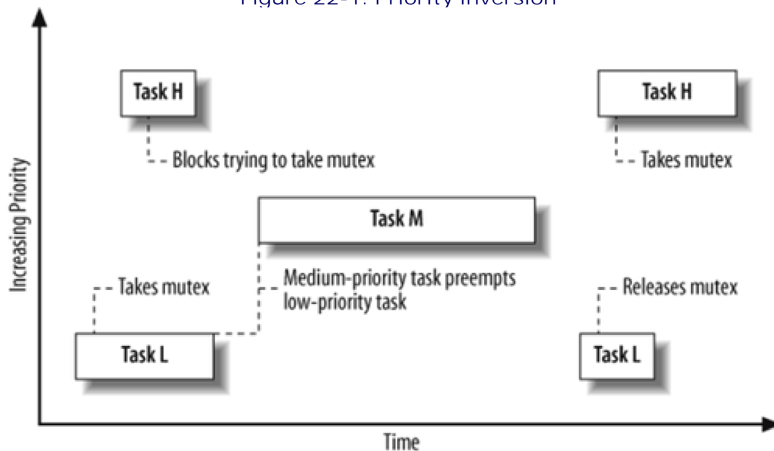
Figure 22-1. Priority inversion
