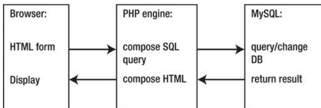
Figure 10-25. Three-tier interactions
