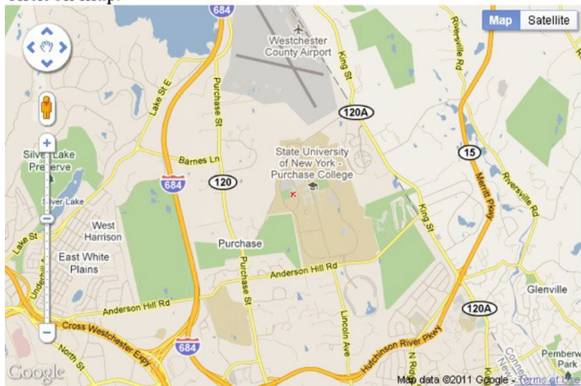
Figure 5-1. Opening screen
