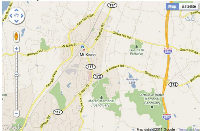
Figure 5-4. Image-and-audio combination
