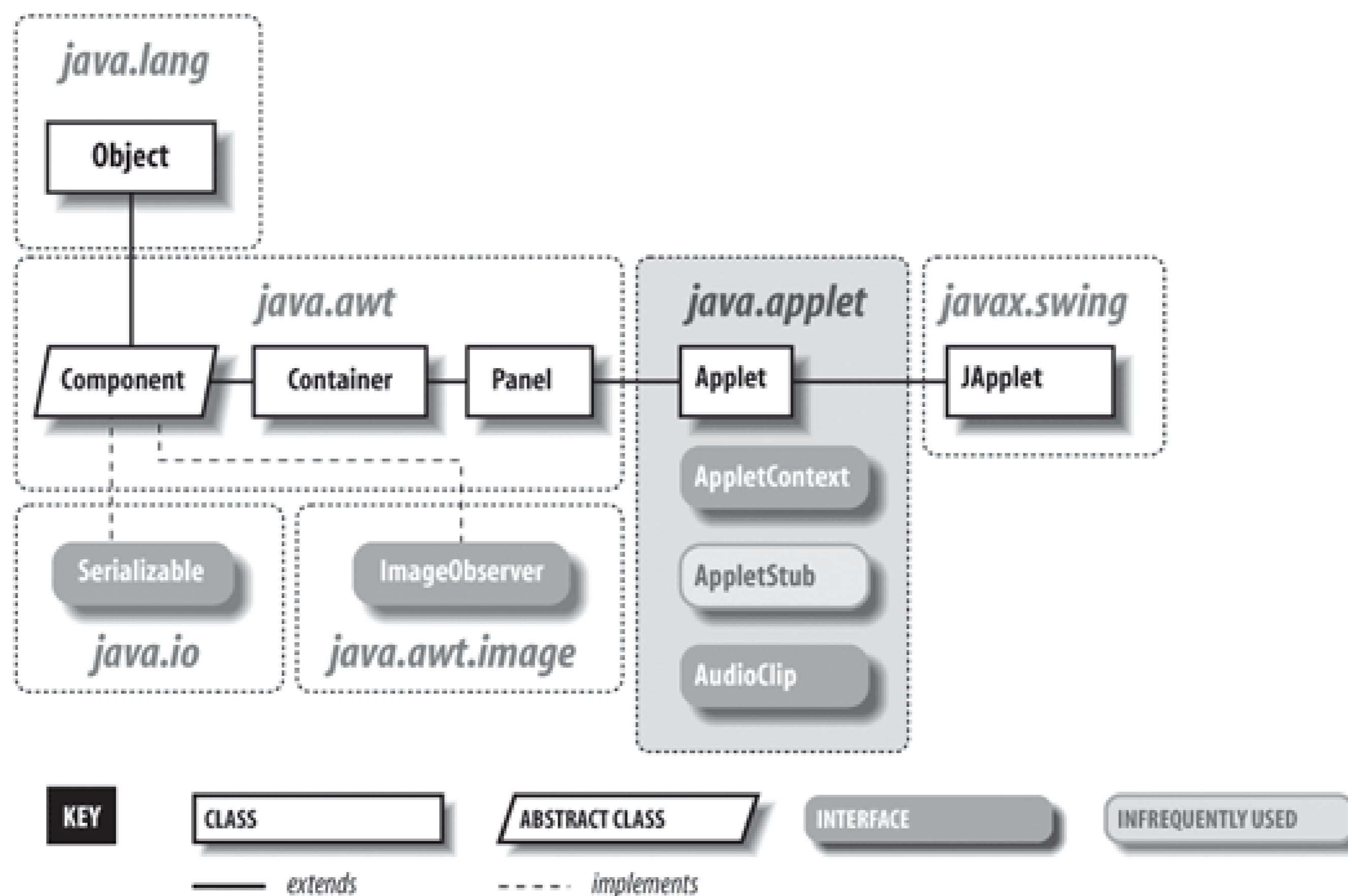
Figure 23-1. The java.applet package
