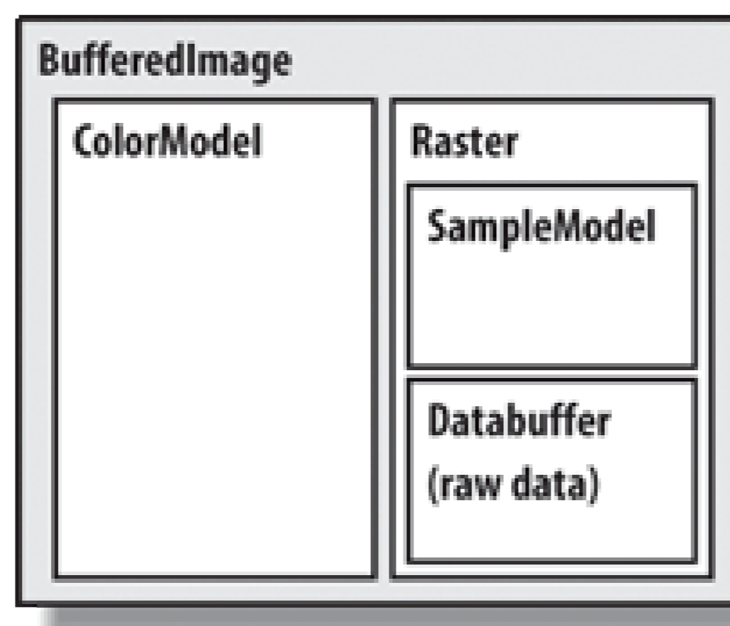
Figure 21-3. Inside a BufferedImage
