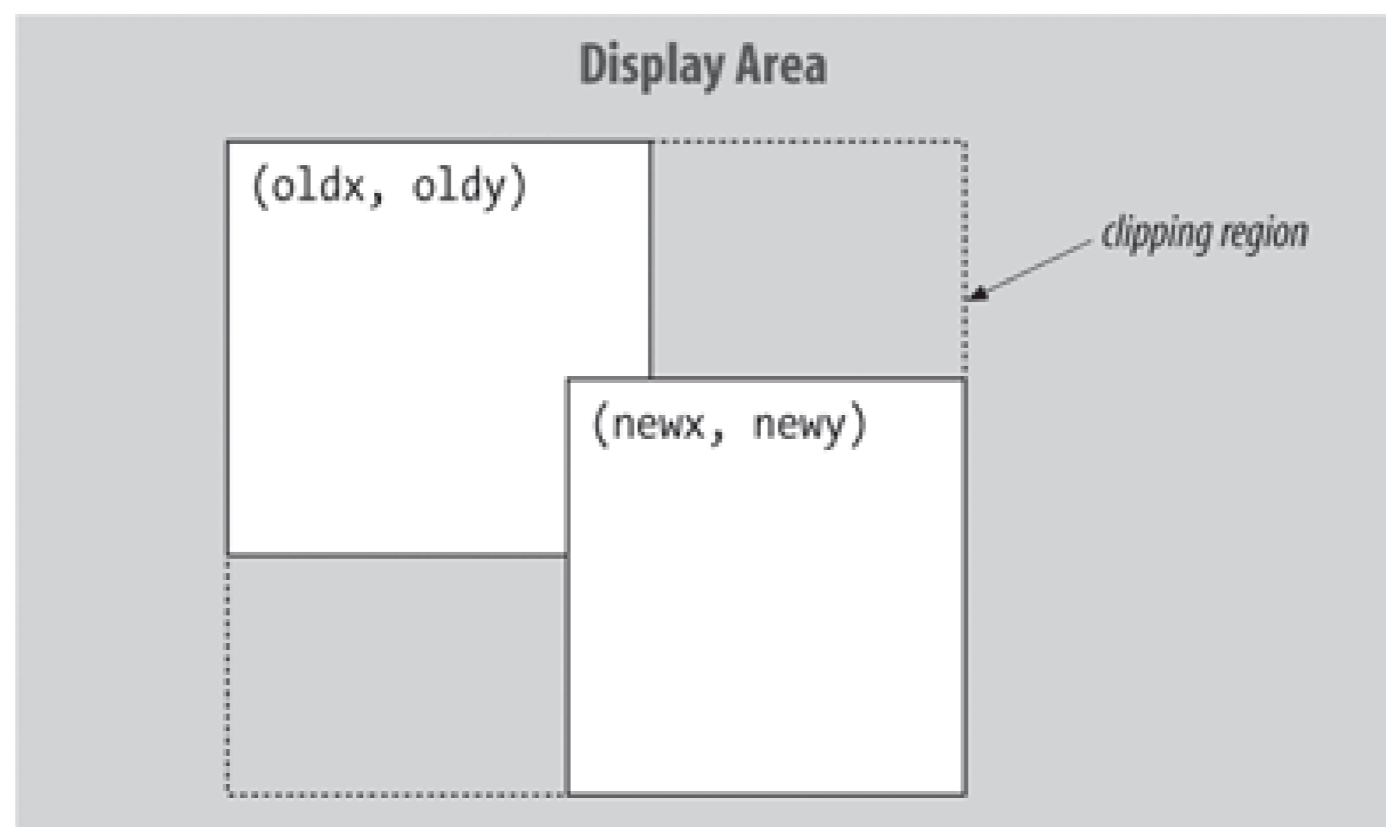
Figure 20-6. Determining the clipping region
