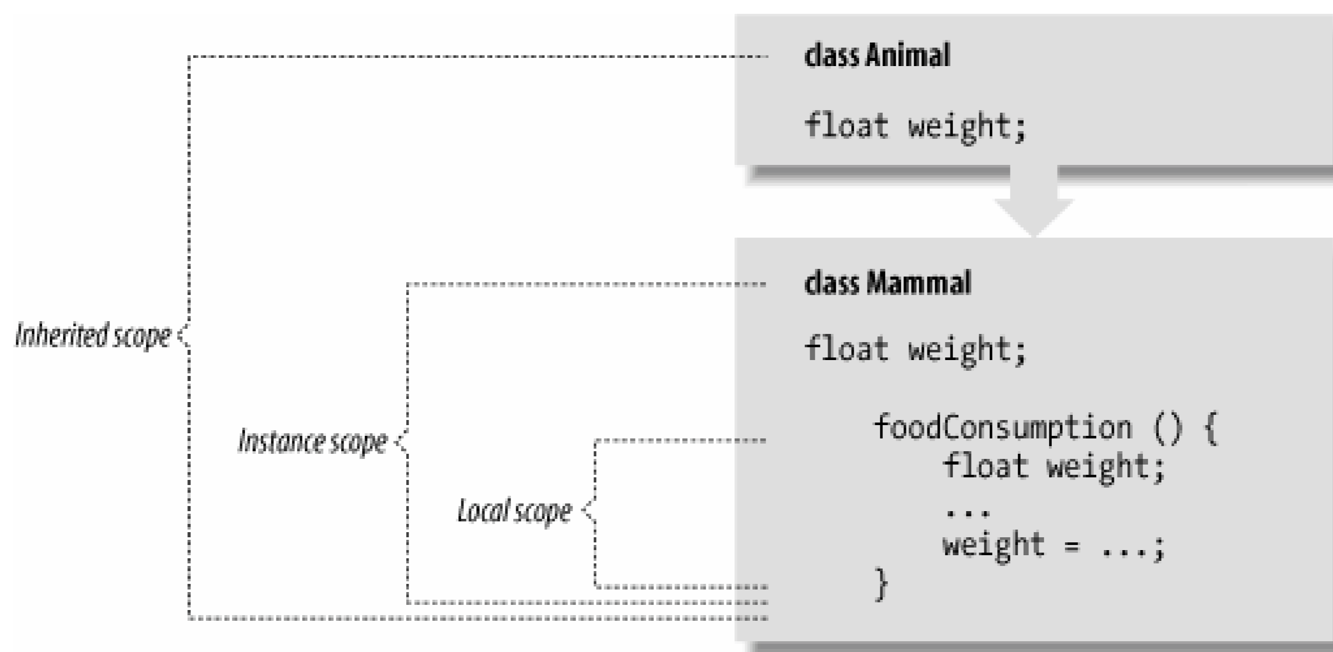
Figure 6.2. The scope of shadowed variables
