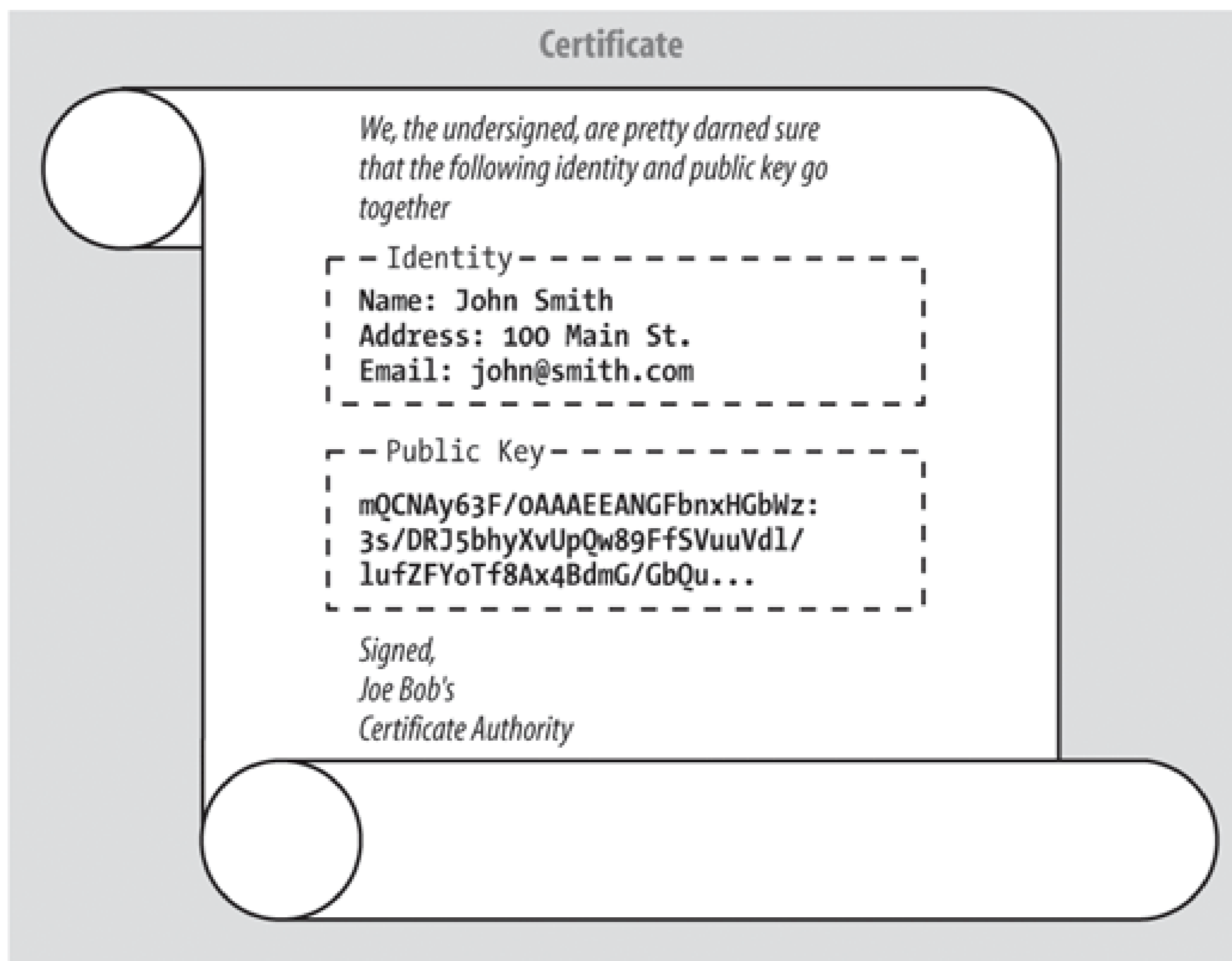
Figure 23-3. An old-fashioned certificate
