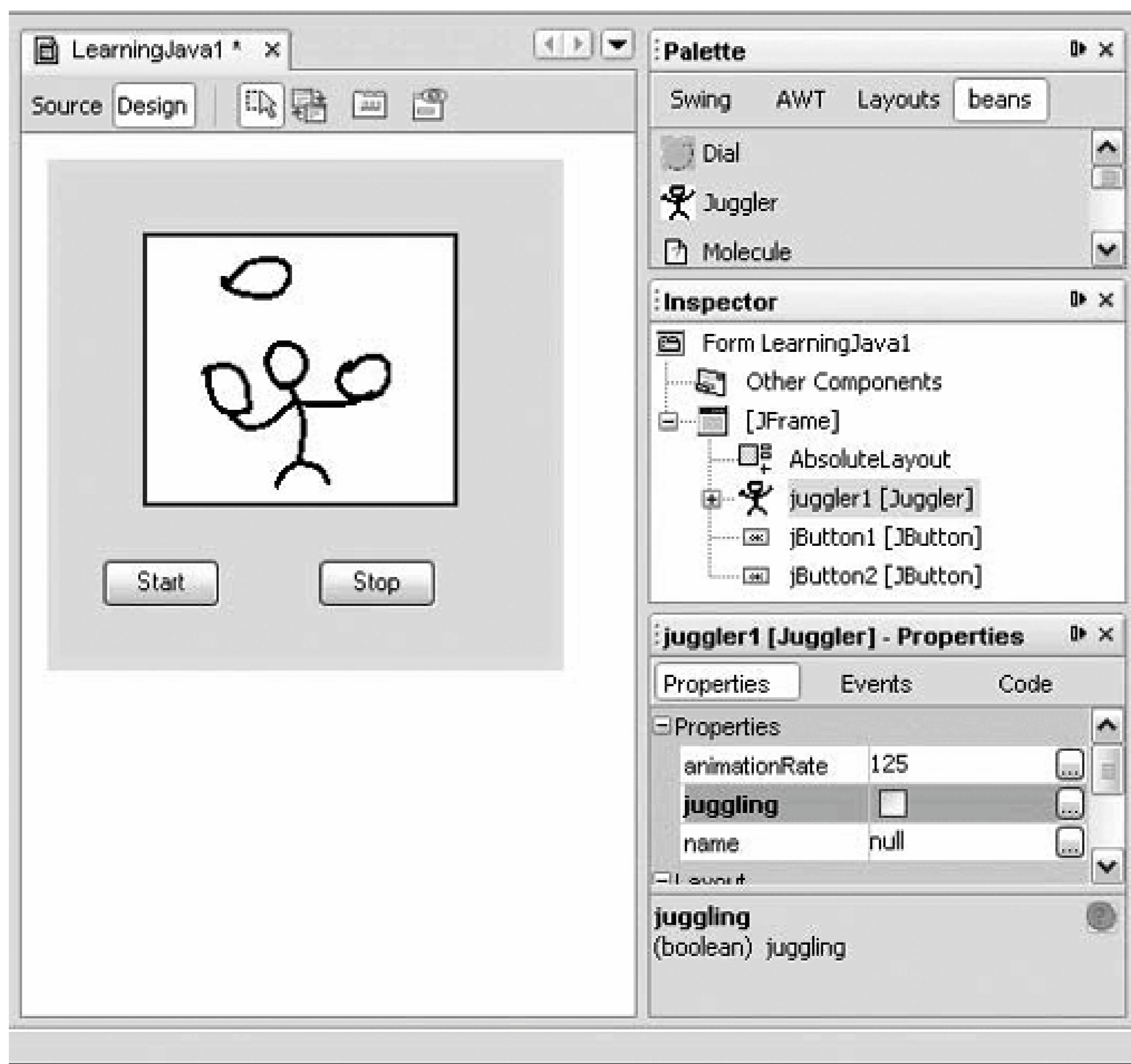
Figure 22-3. Juggling beans
