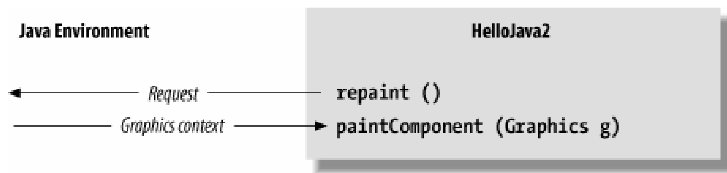
Figure 2-4. Invoking the repaint( ) method
