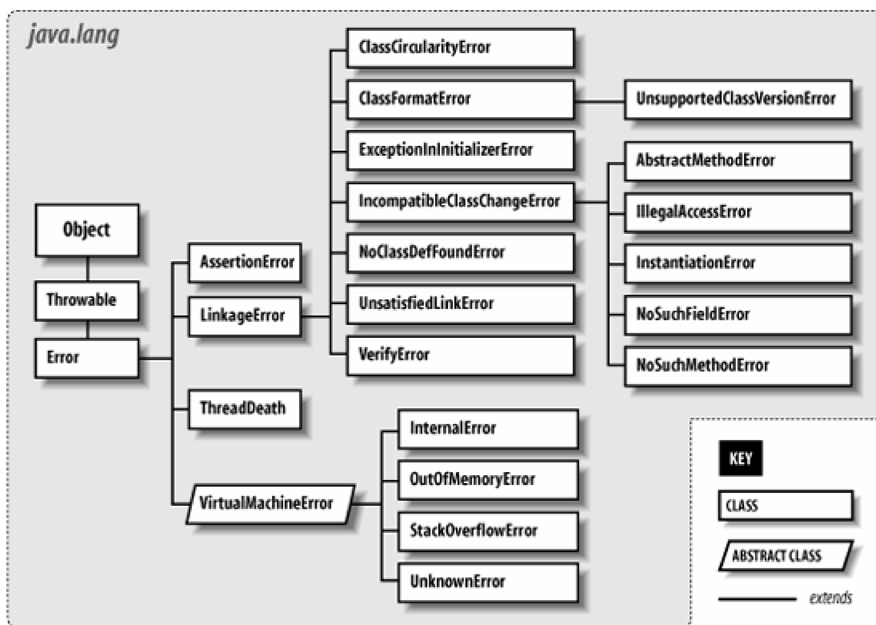
Figure 4-2. The java.lang.Error subclasses
