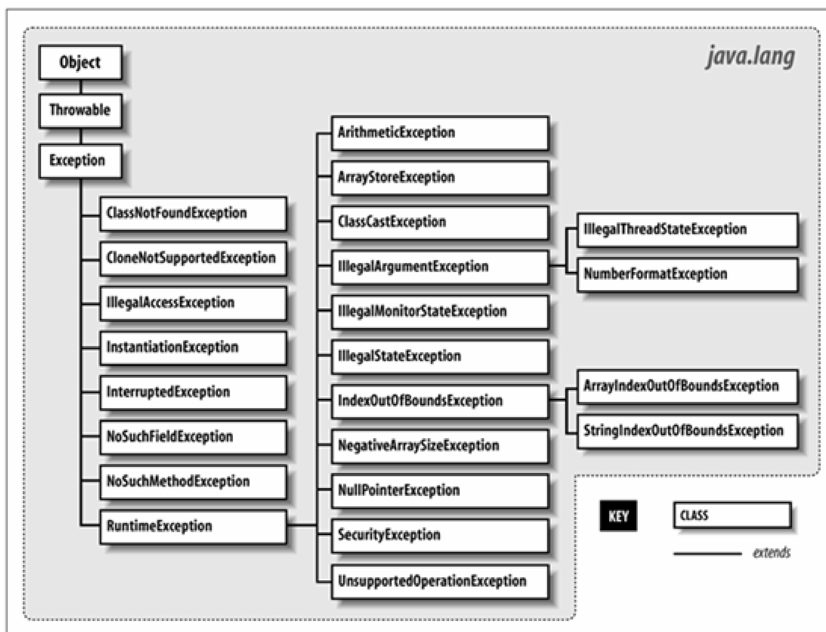
Figure 4-1. The java.lang.Exception subclasses
