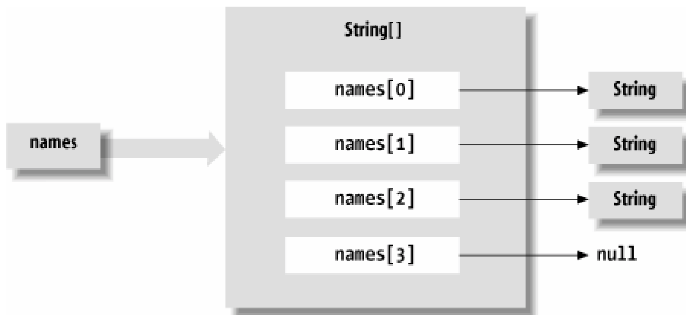
Figure 4-4. A Java array
