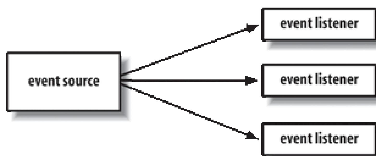
Figure 16-3. Event delivery
