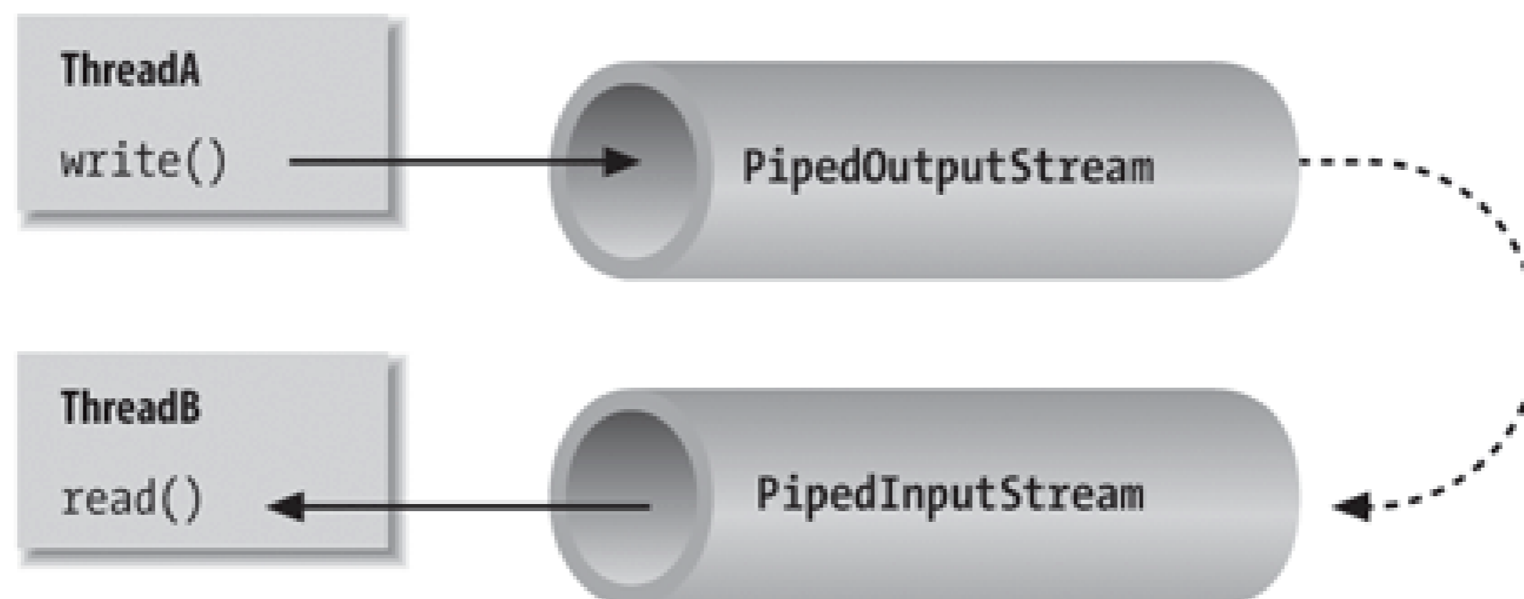
Figure 12-4. Piped streams
