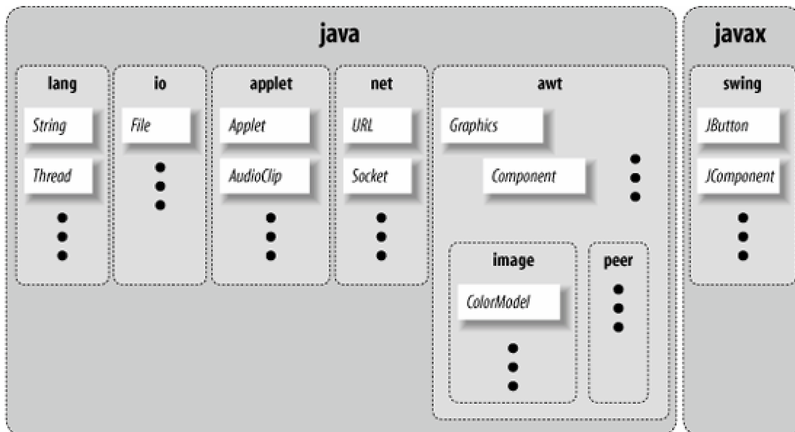
Figure 2-3. Some core Java packages
