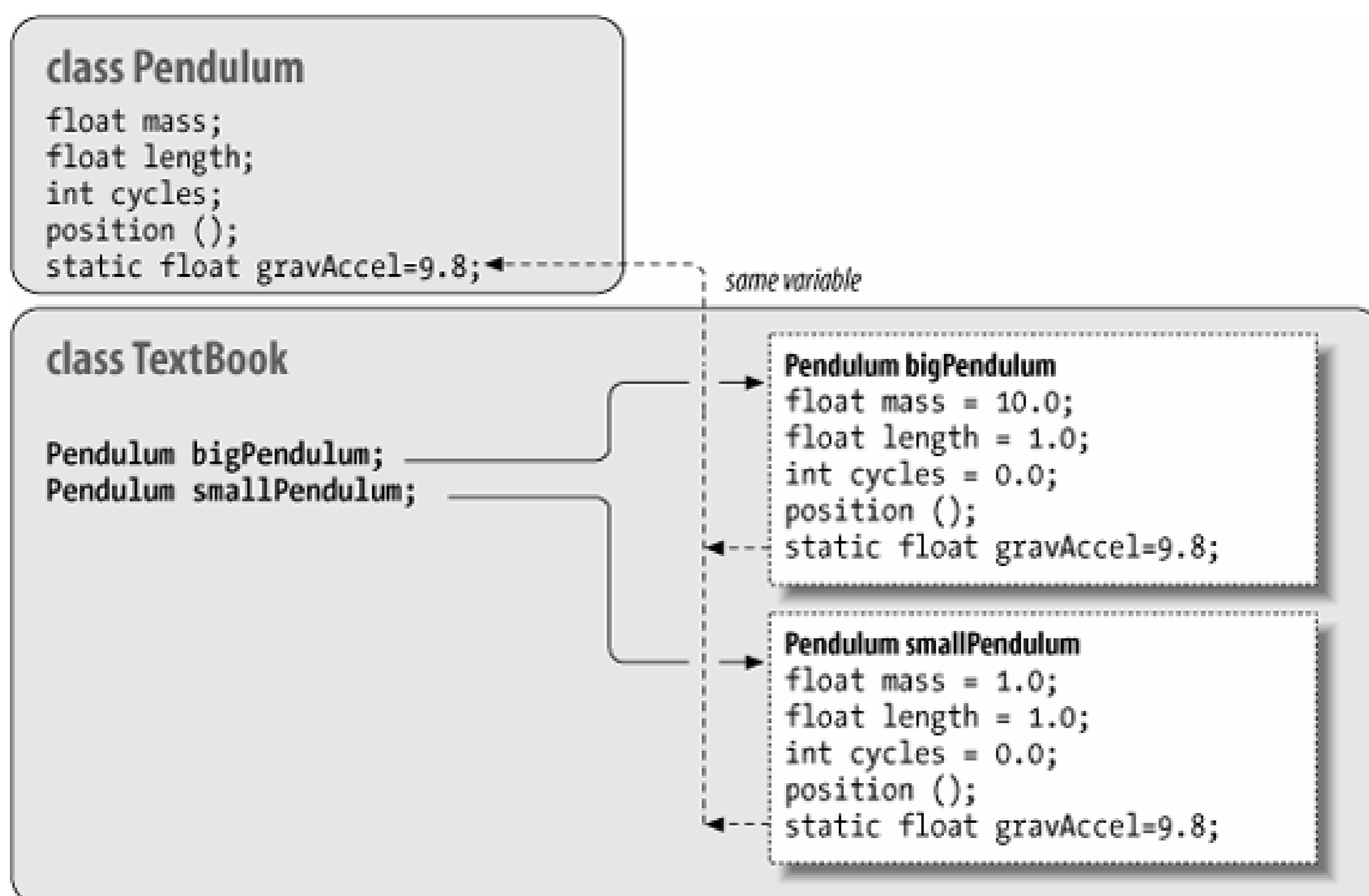
Figure 5-2. Static variables shared by all instances of a class
