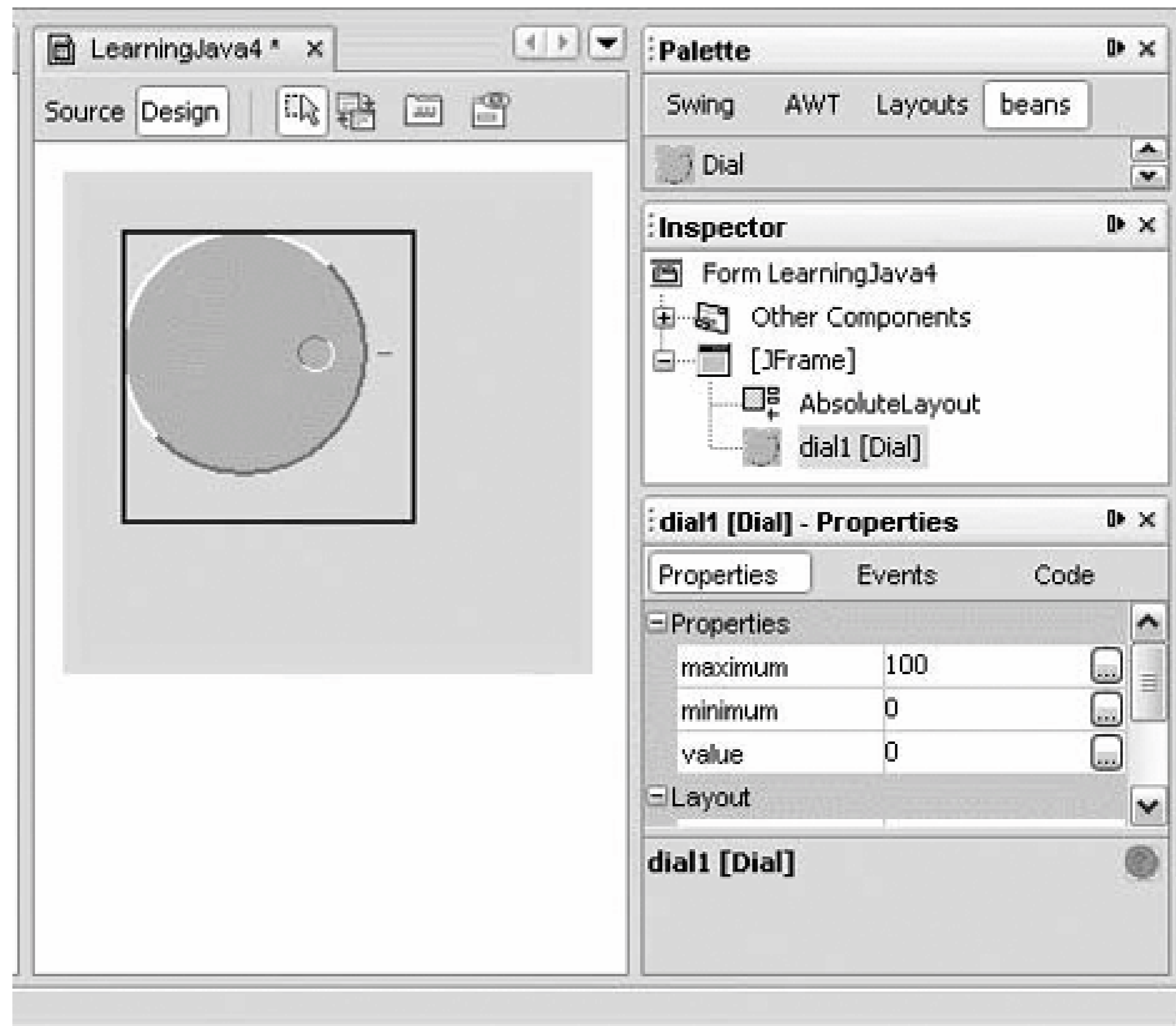
Figure 22-8. The Dial component as a bean
