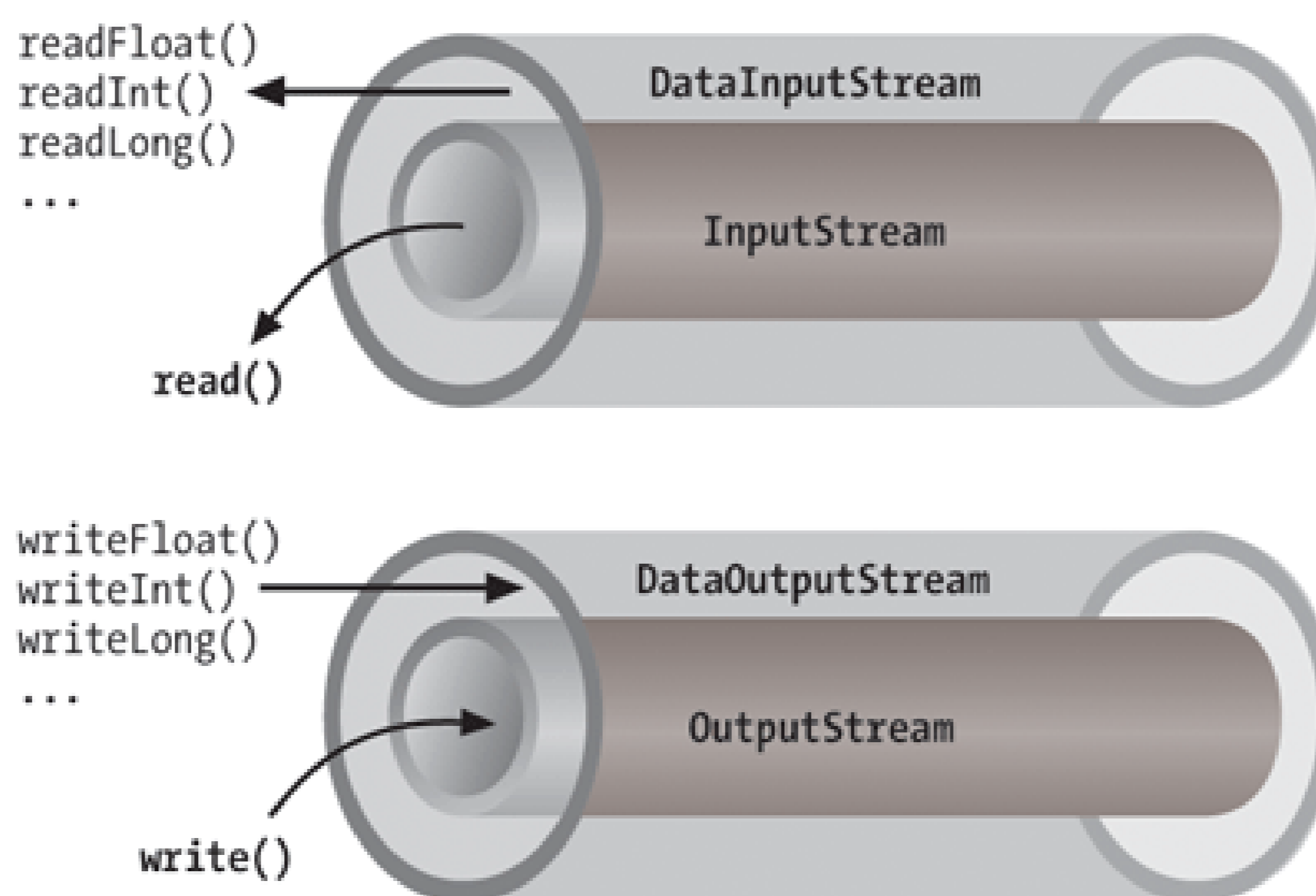
Figure 12-3. Layered streams
