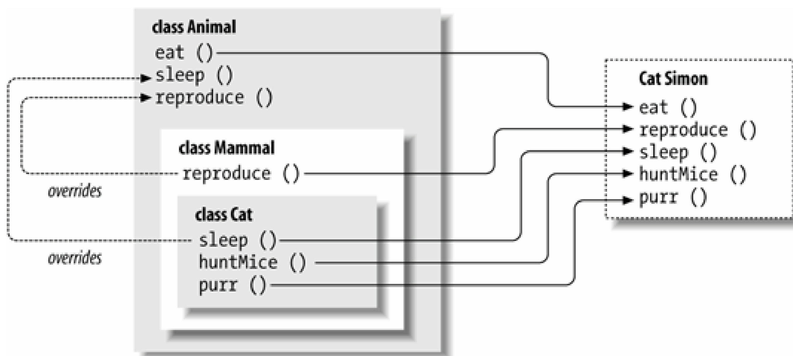
Figure 6.3. Method overriding
