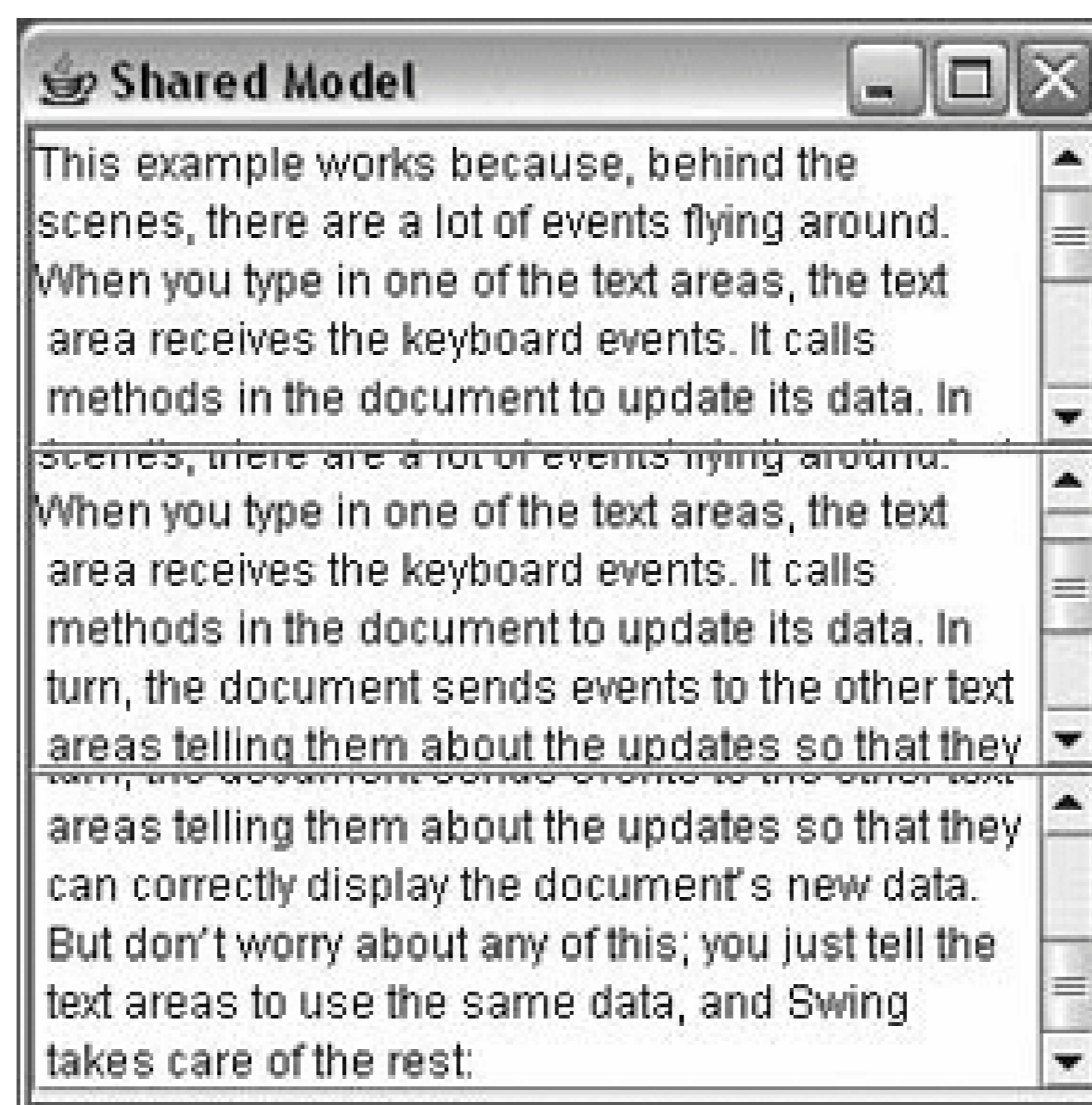
Figure 18-3. Three views of the same data model
