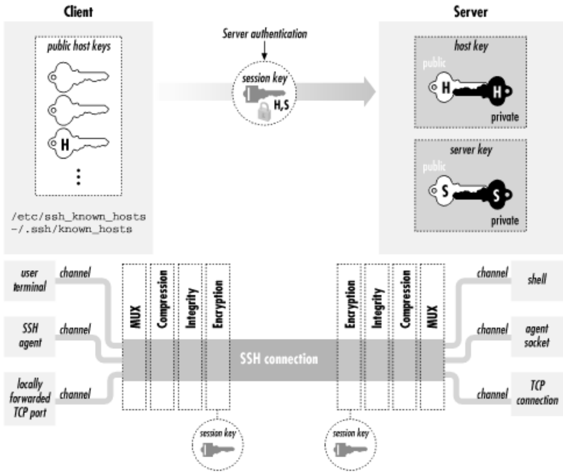
Figure 3.2. SSH-1 architecture
