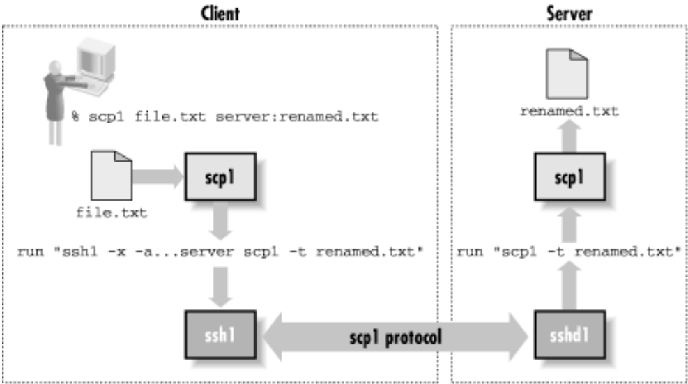
Figure 3.6. scp1 operation
