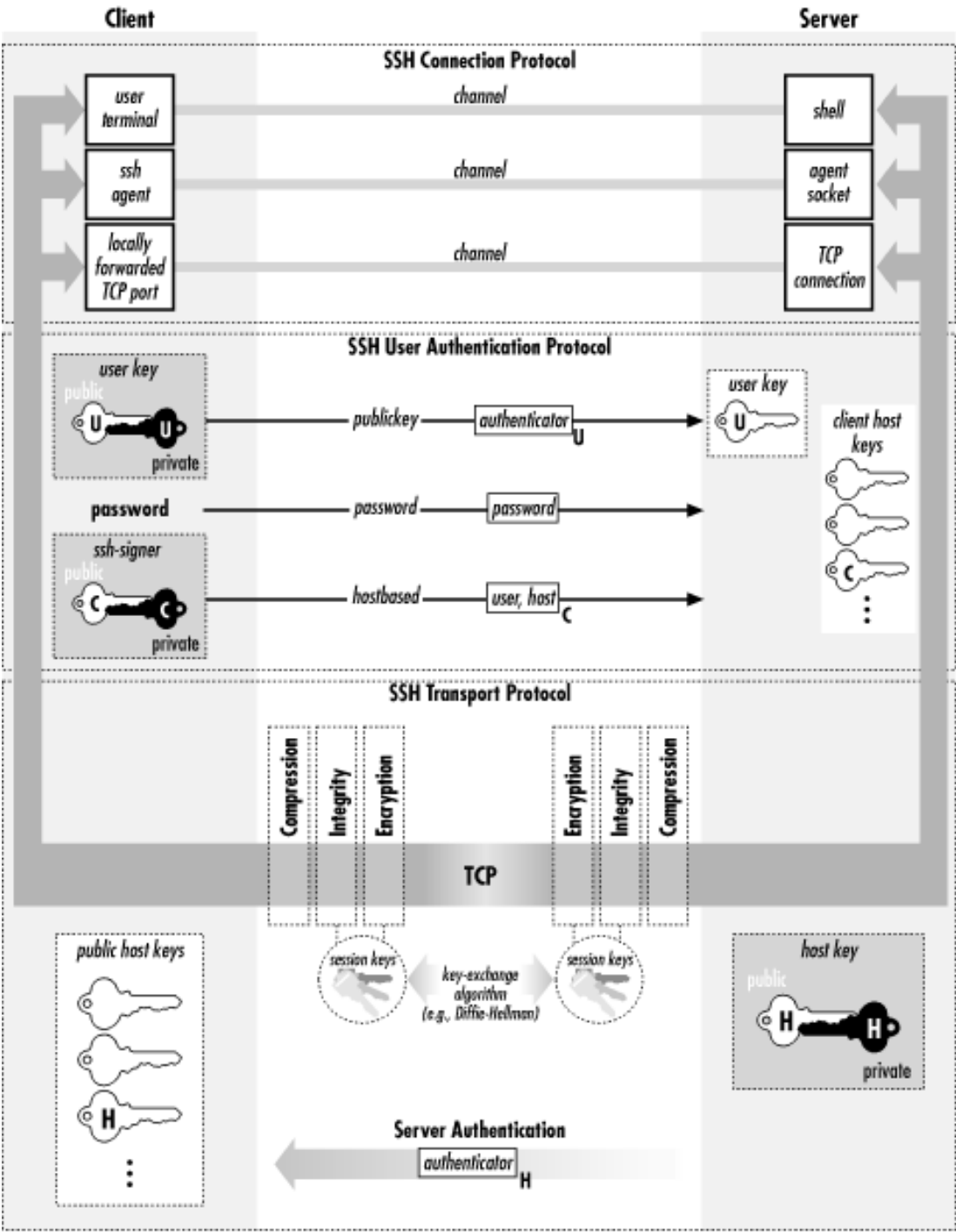
Figure 3.4. SSH-2 architecture
