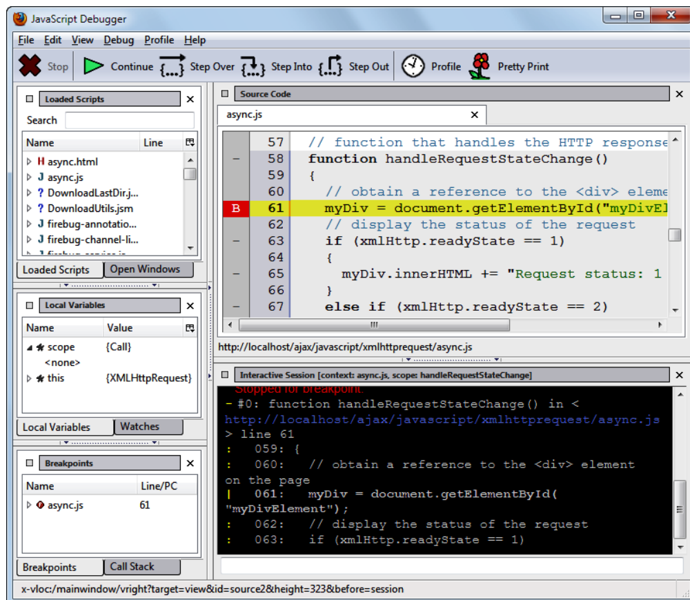
Figure 6-17: The Venkman debugger in action
