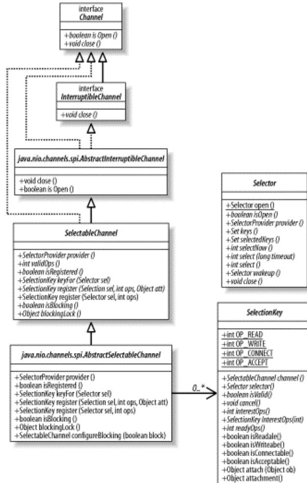
Figure 4-1. Selection class family tree
