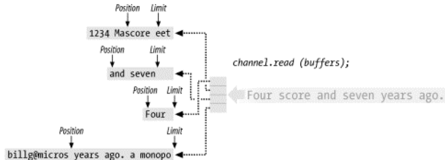
Figure 3-6. A scattering read using four buffers
