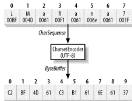
Figure 6-1. Characters encoded as UTF-8
