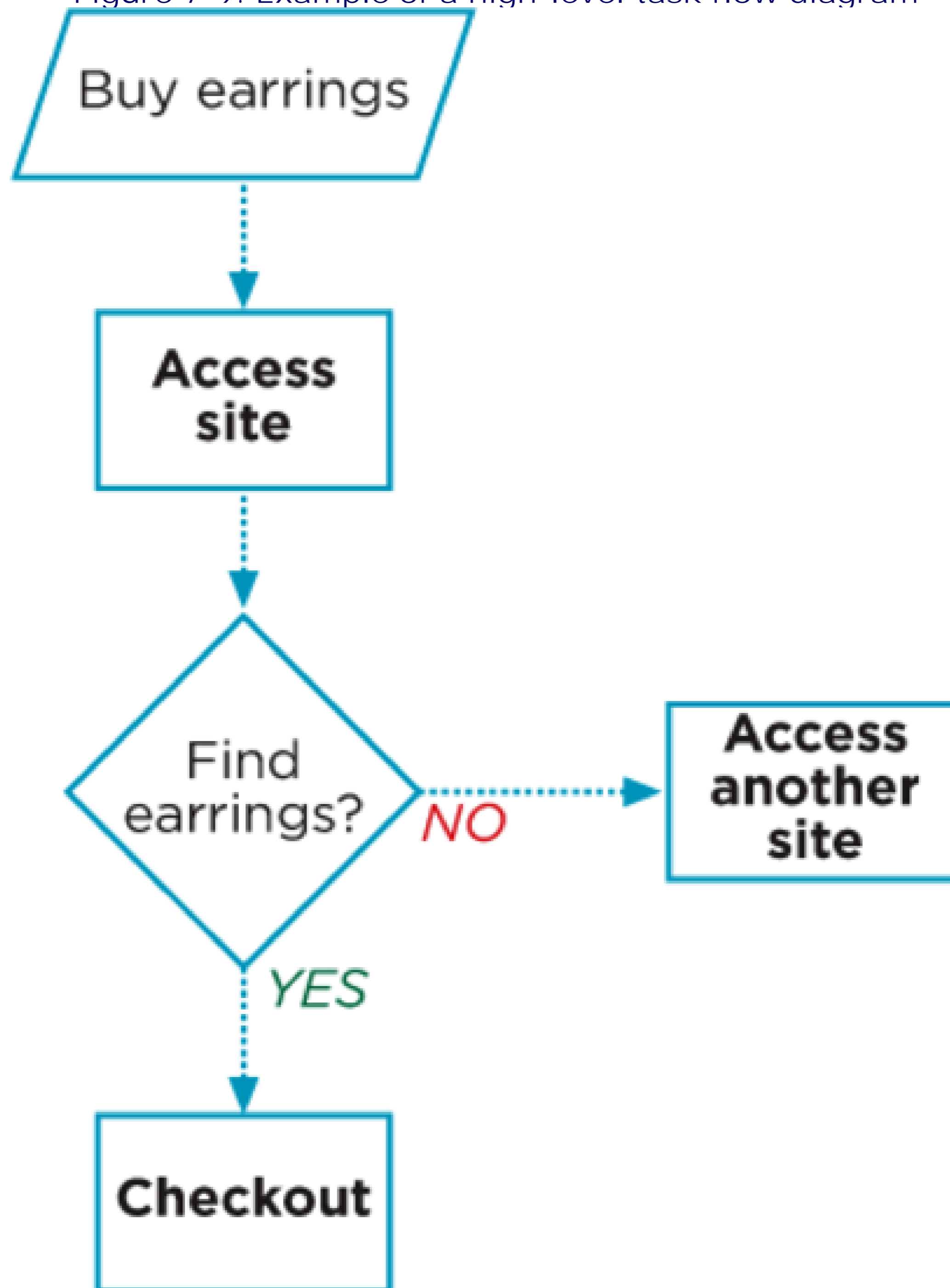
Figure 7-9. Example of a high-level task flow diagram
