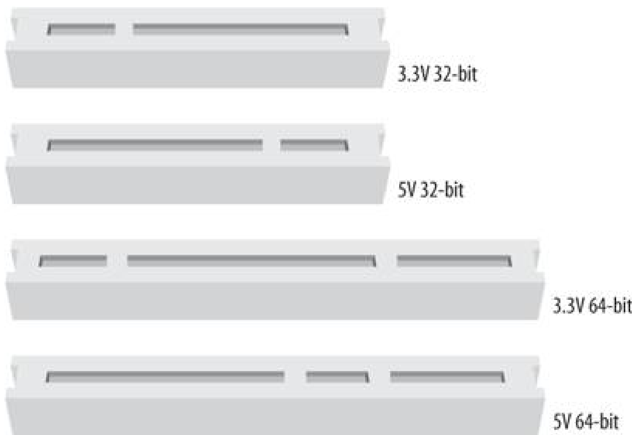
Figure 2-1. Visual identification of PCI slots
