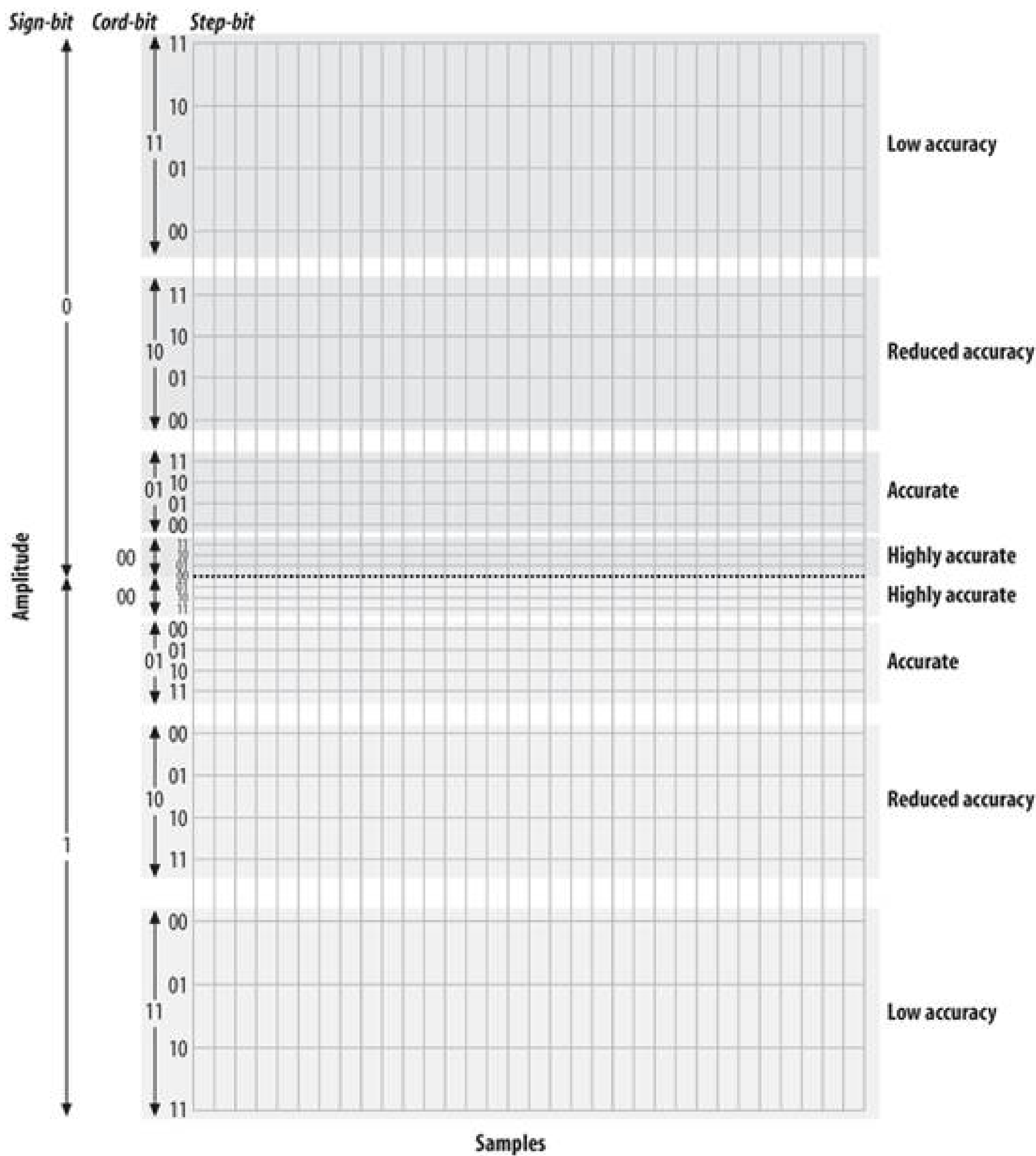
Figure 7-11. Five-bit companding
