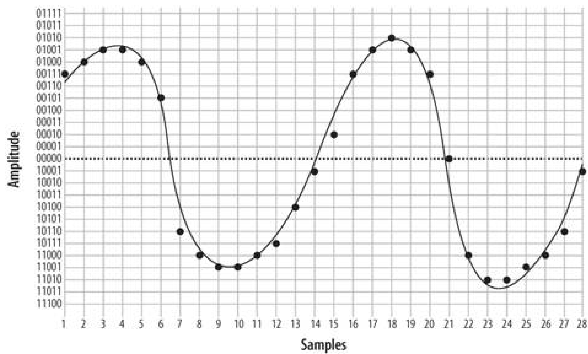
Figure 7-8. The same waveform at double the resolution
