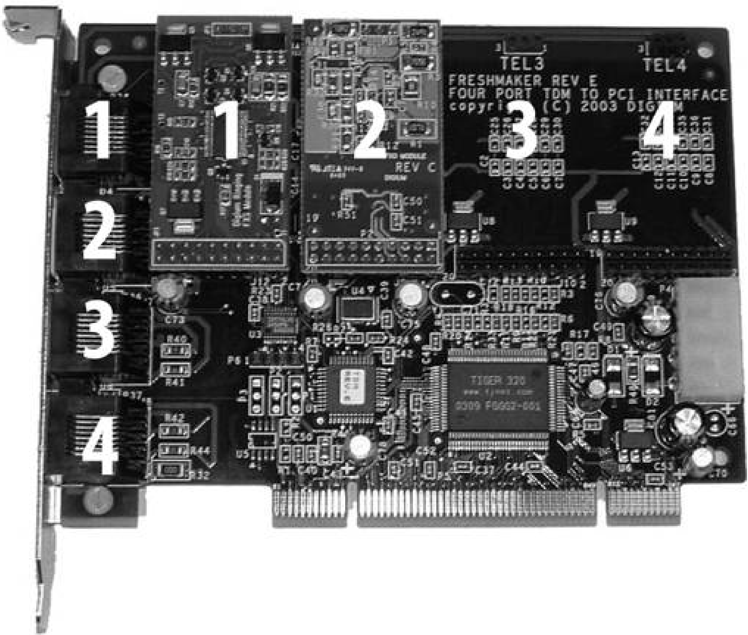
Figure 4-1. A TDM400P with an FXS module (1 across) and an FXO module (2 across)
