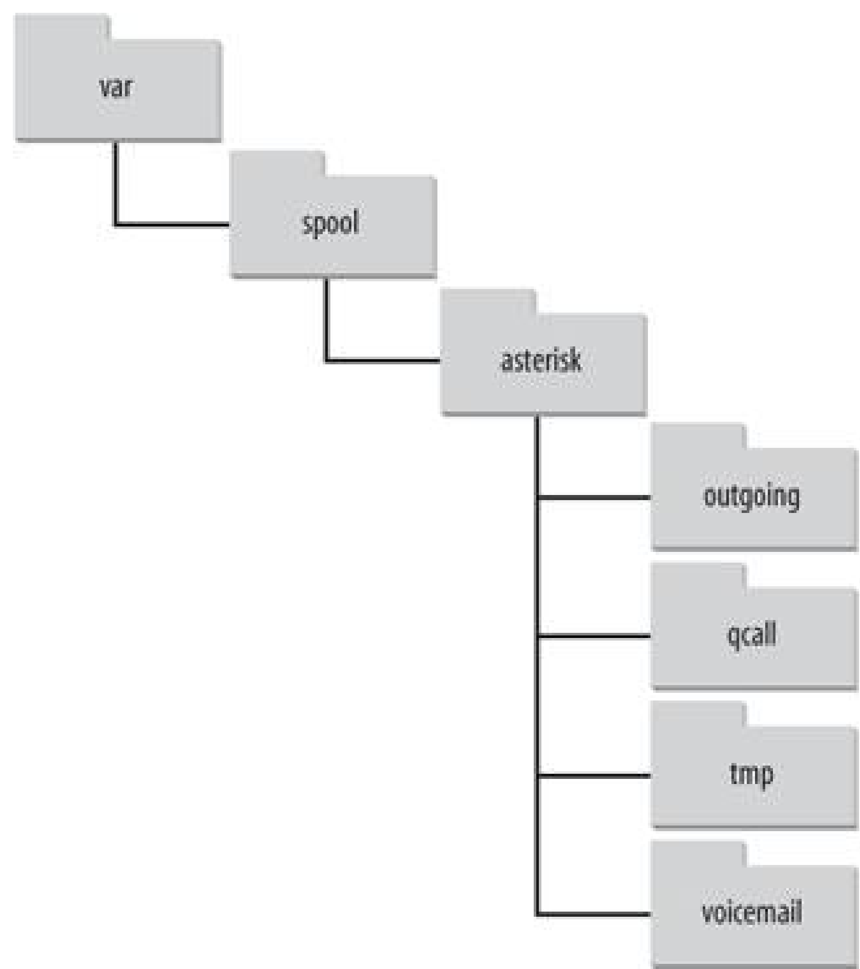
Figure 3-2. /var/spool/asterisk/ directory structure
