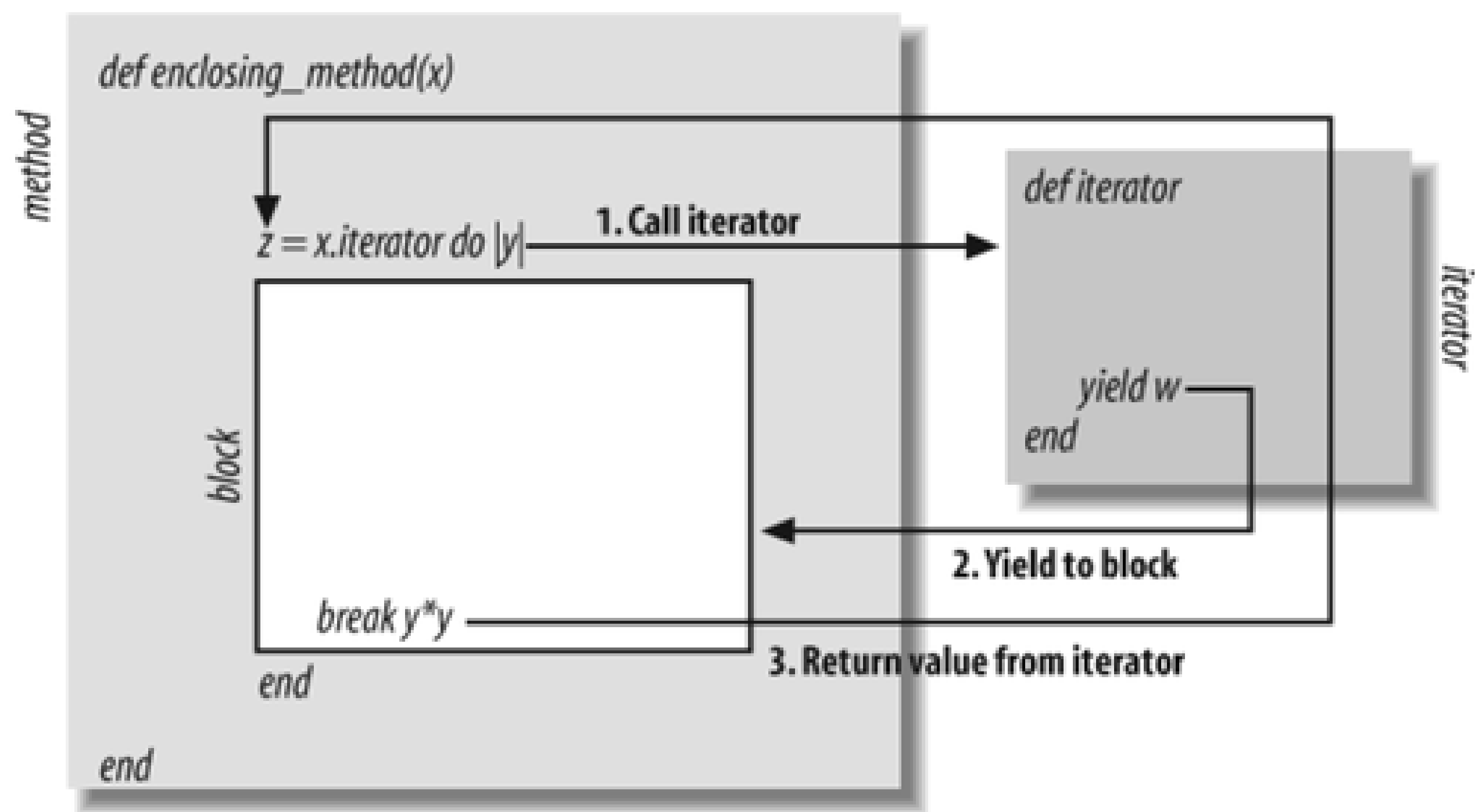
Figure 5-3. The break statement in a block
