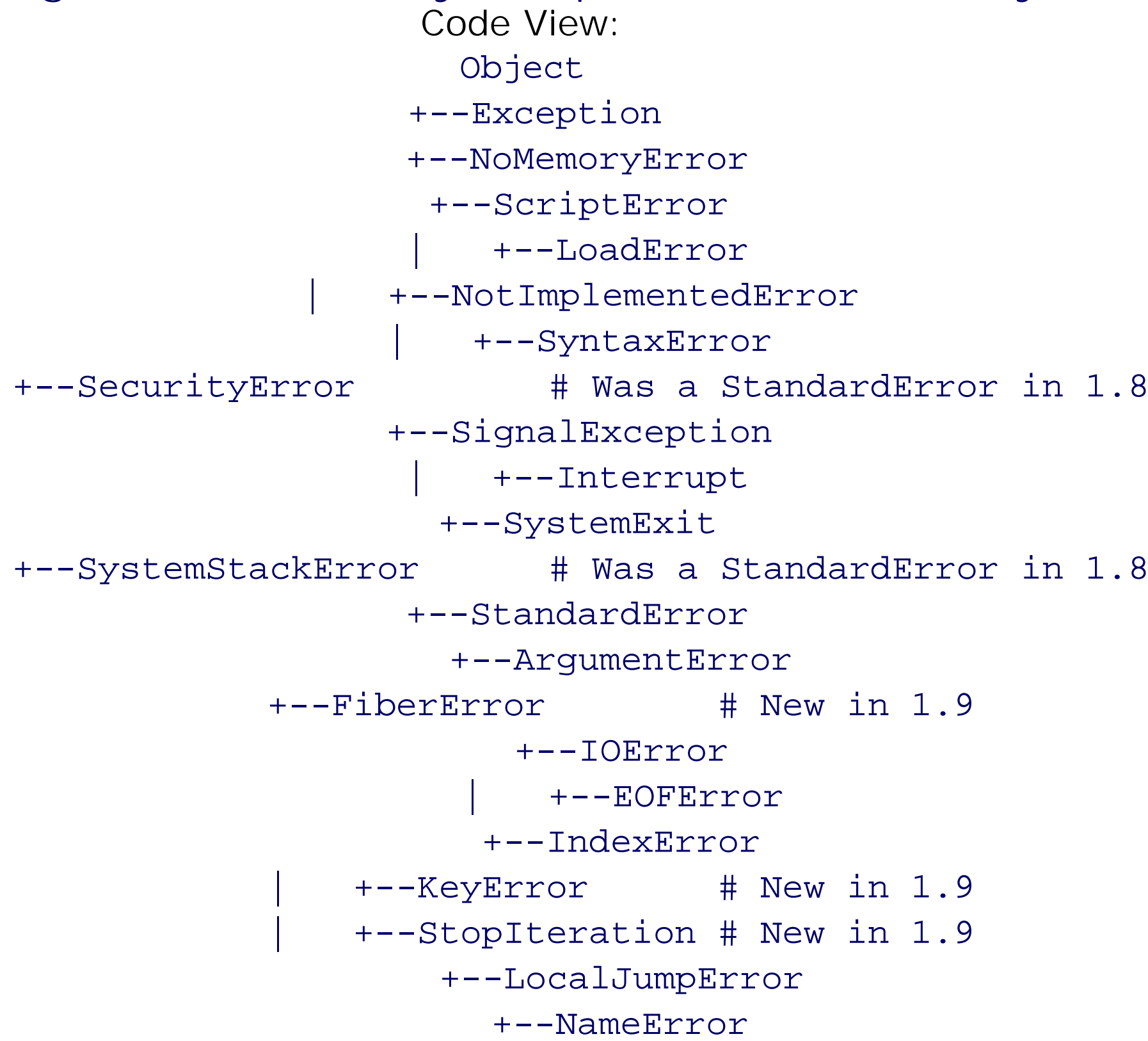
Figure 5-5. The Ruby Exception Class Hierarchy
