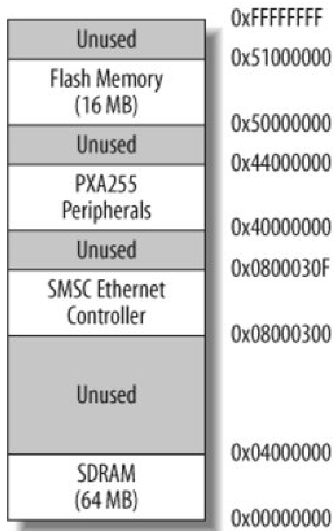
Figure 2-6. Memory map for the Arcom board
