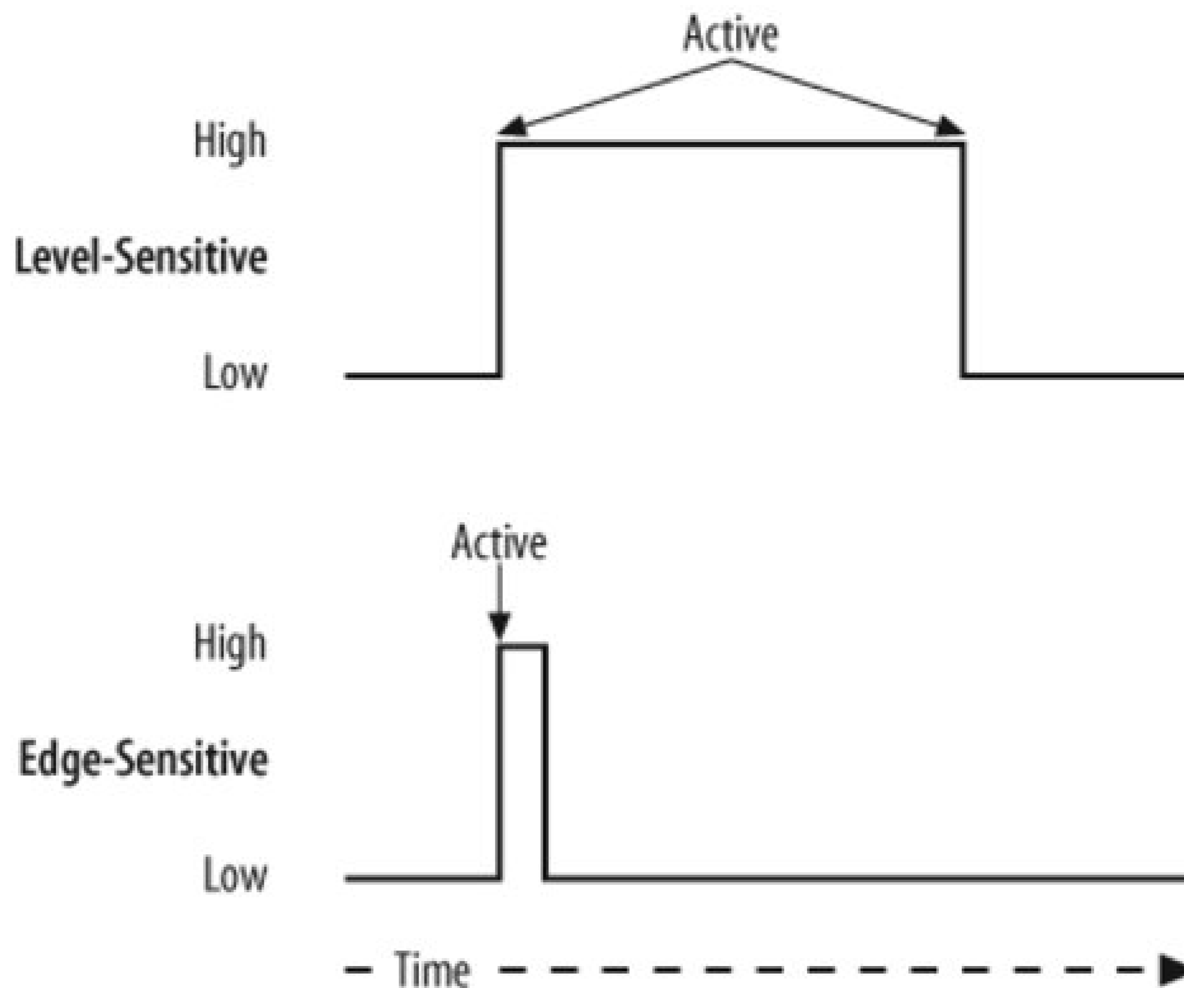
Figure 8-2. Level- and edge-sensitive interrupt signals
