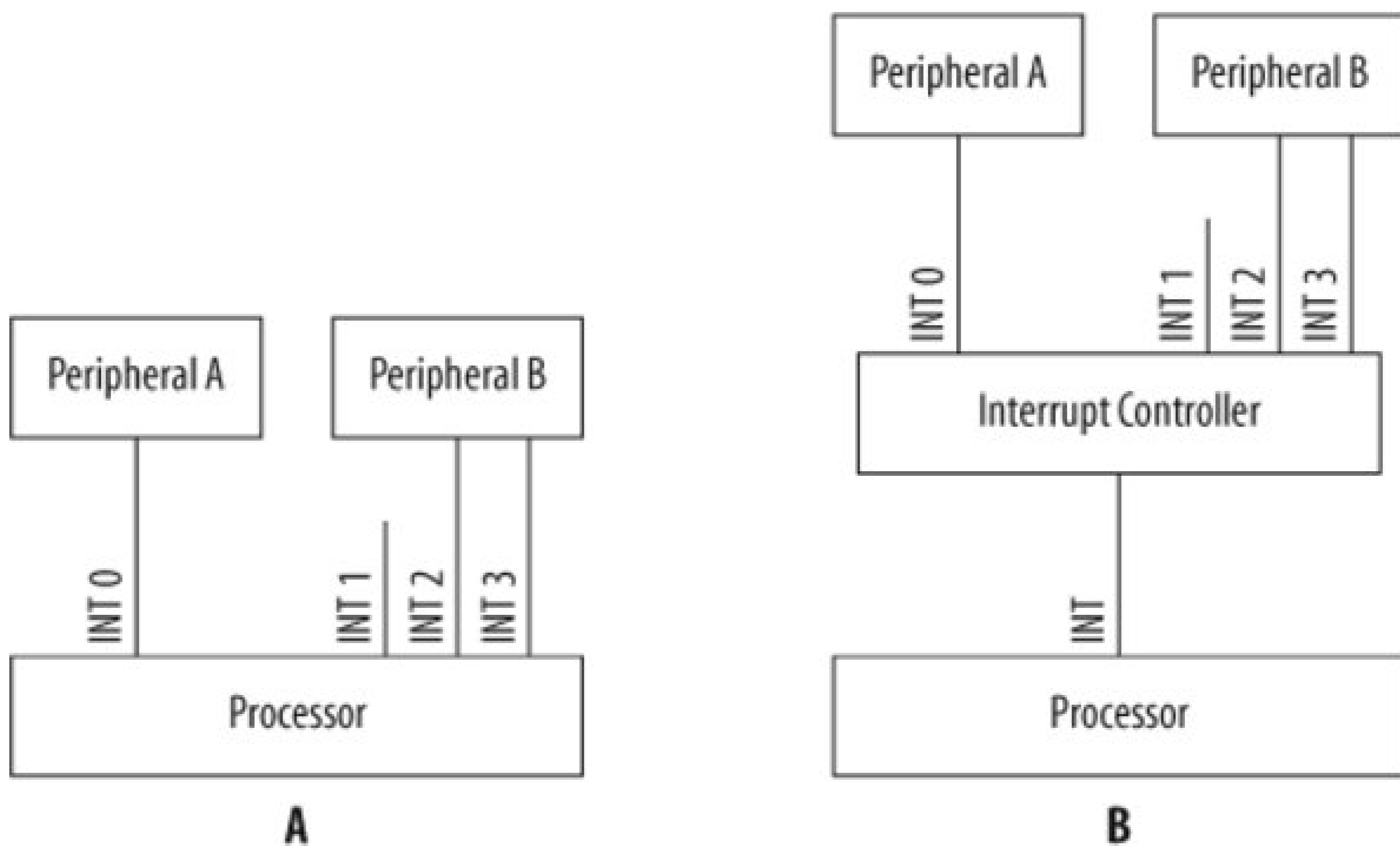
Figure 8-1. Interrupt wiring
