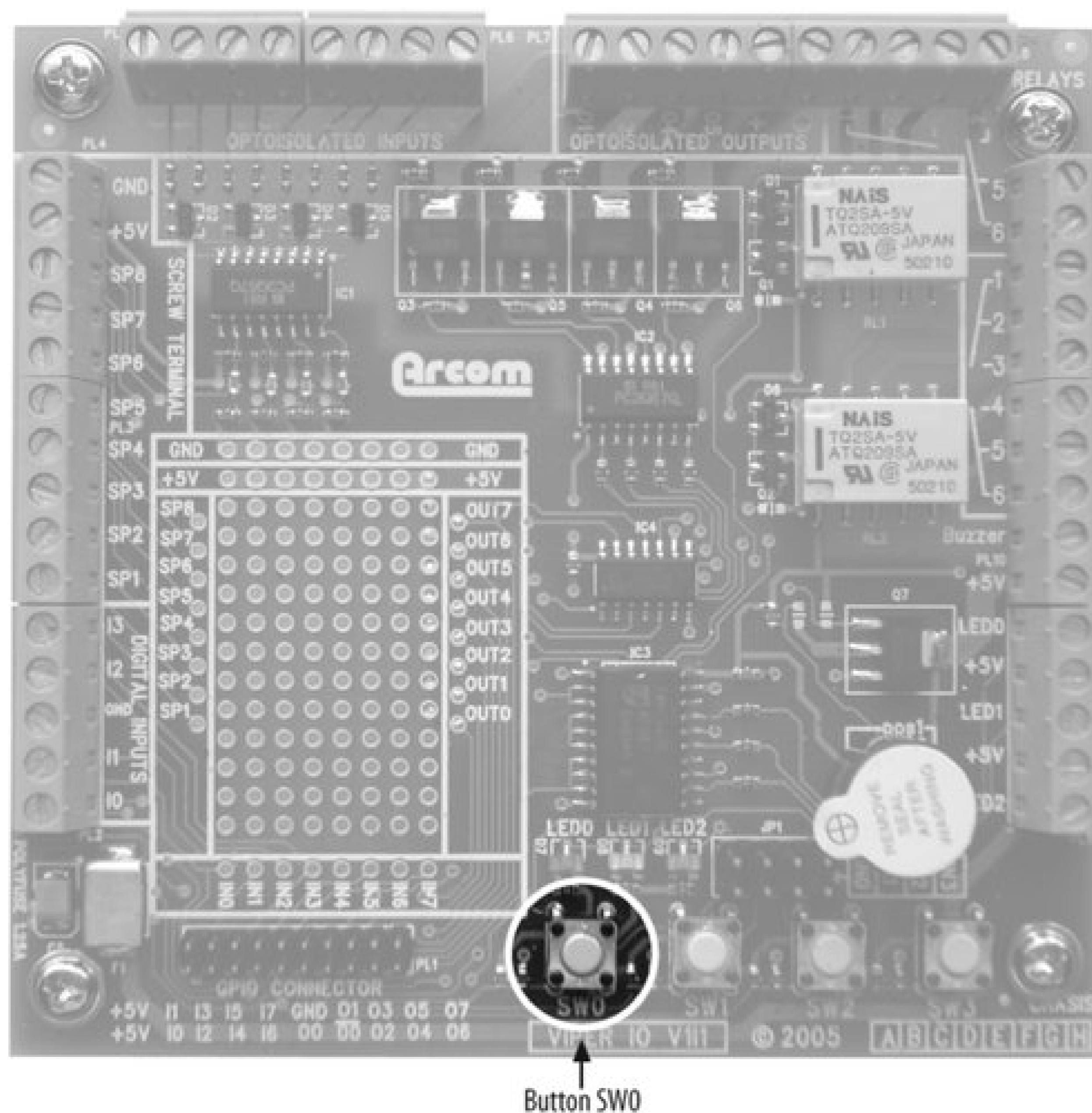
Figure 11-1. Arcom board add-on module's SW0 button
