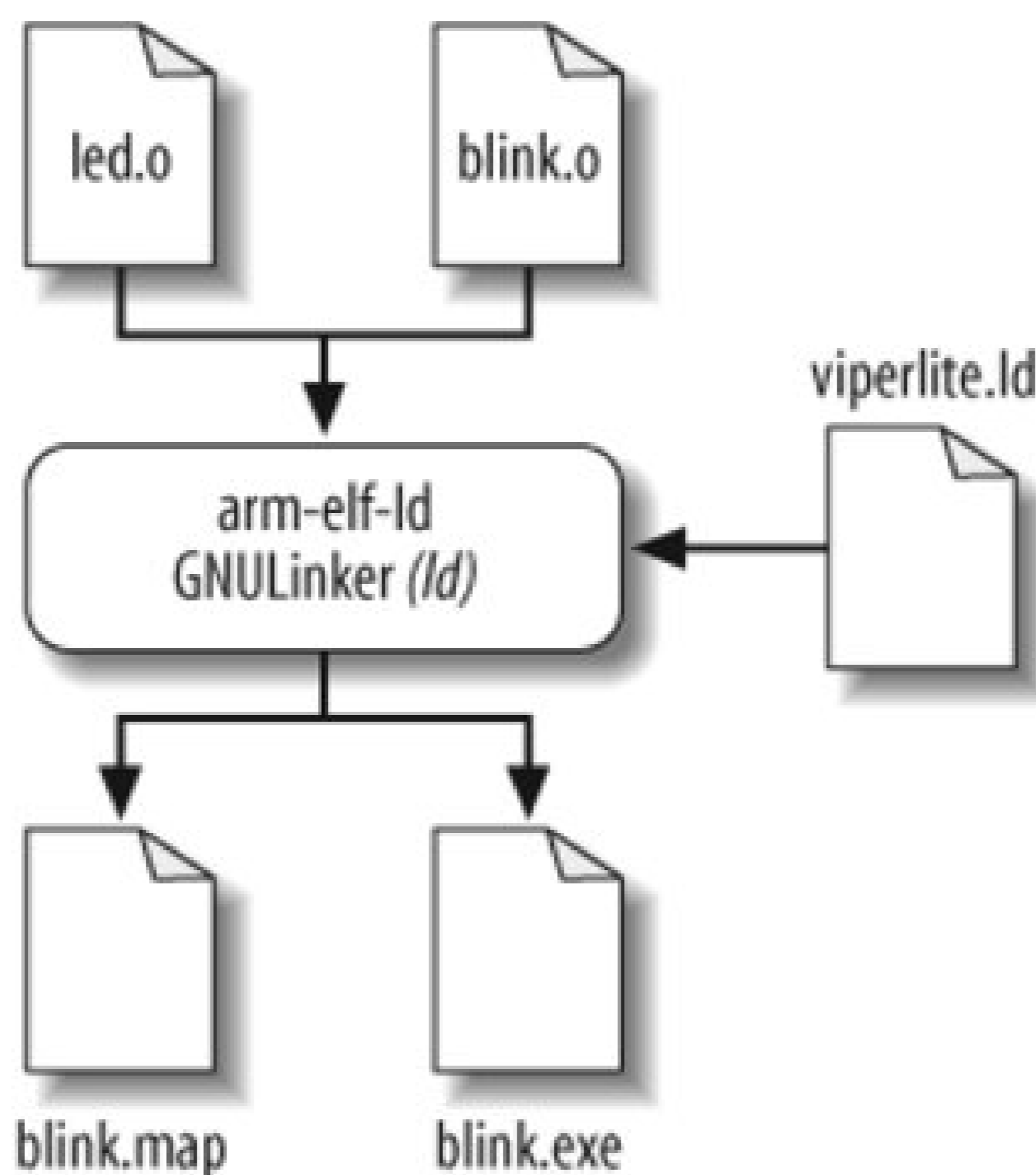
Figure 4-4. Linking and locating the Blinking LED program
