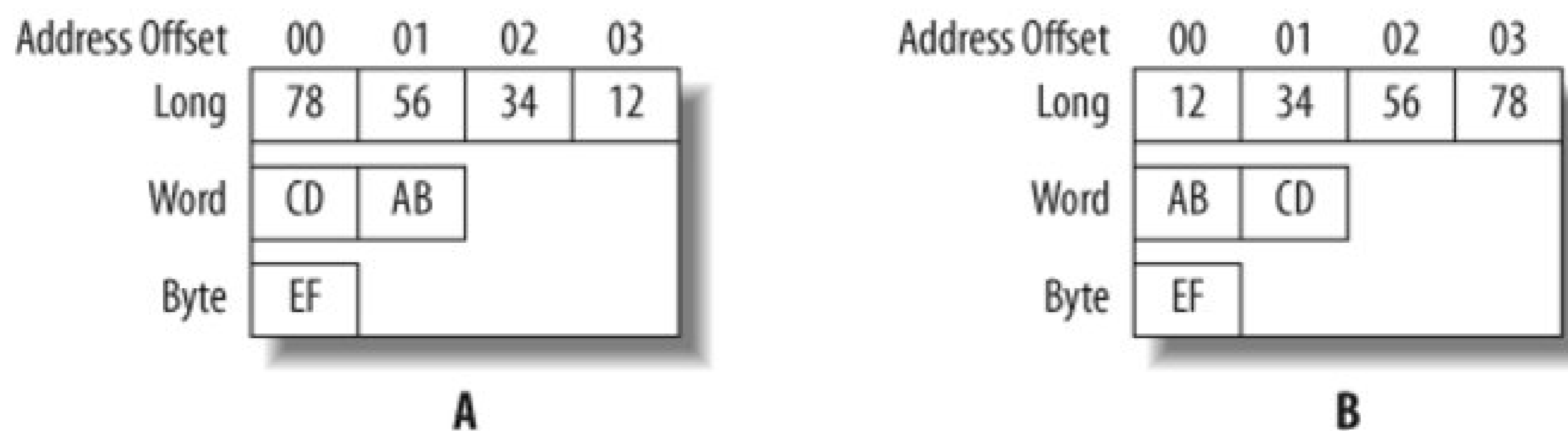
Figure 6-2. (a) Little-endian memory, (b) big-endian memory
