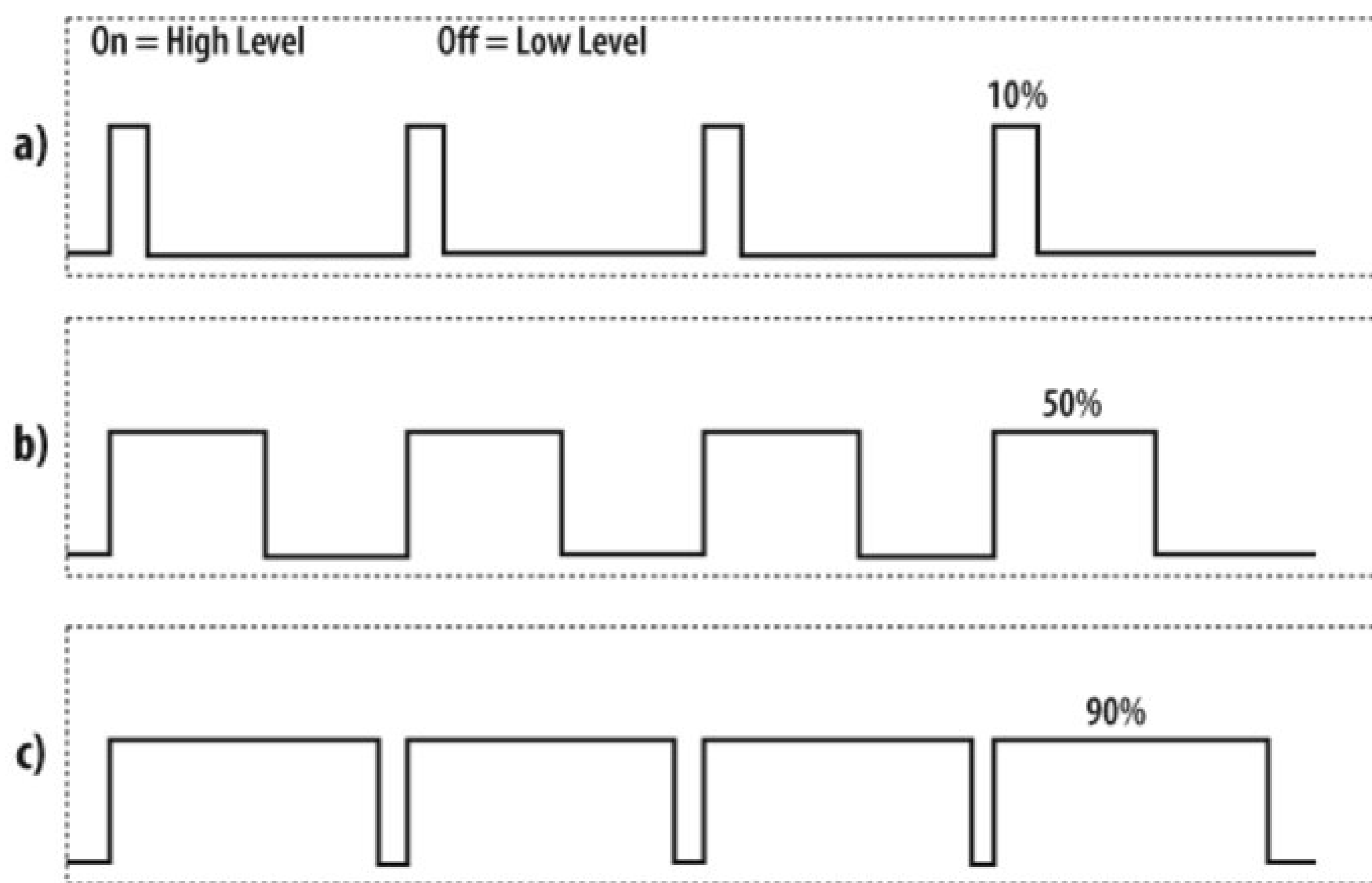
Figure 13-6. PWM signals with varying duty cycles
