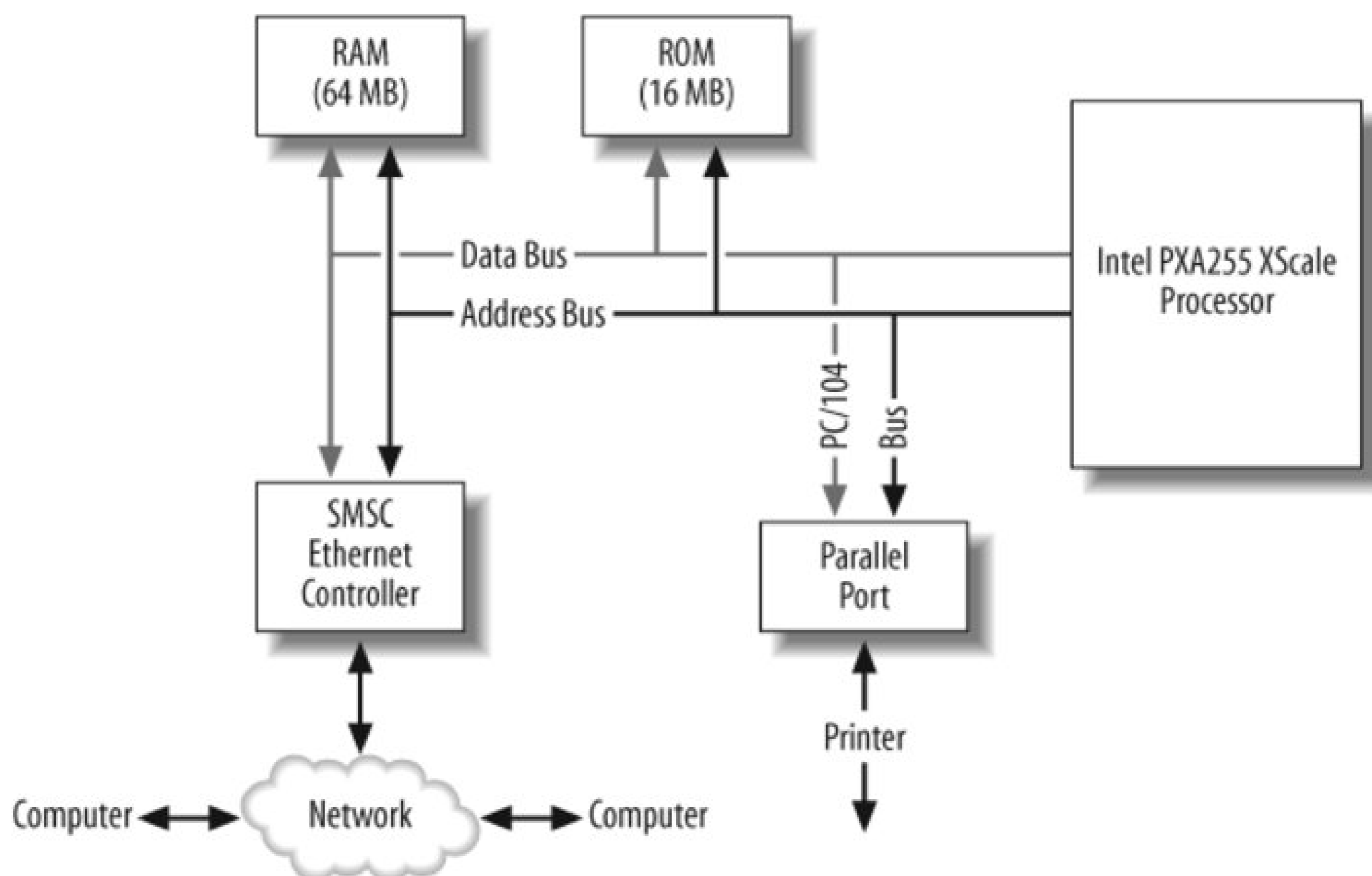
Figure 2-1. Block diagram for the print server
