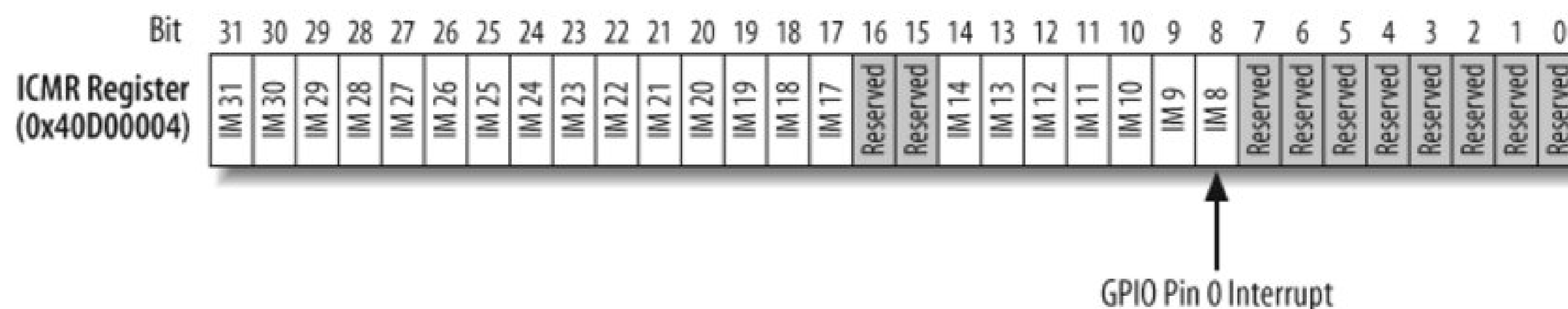
Figure 8-3. PXA255 Interrupt Controller Mask Register
