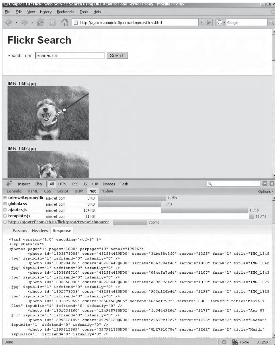
FIGURE 10-2 URL forwarding proxy to enable Ajax Web Service calls in action
