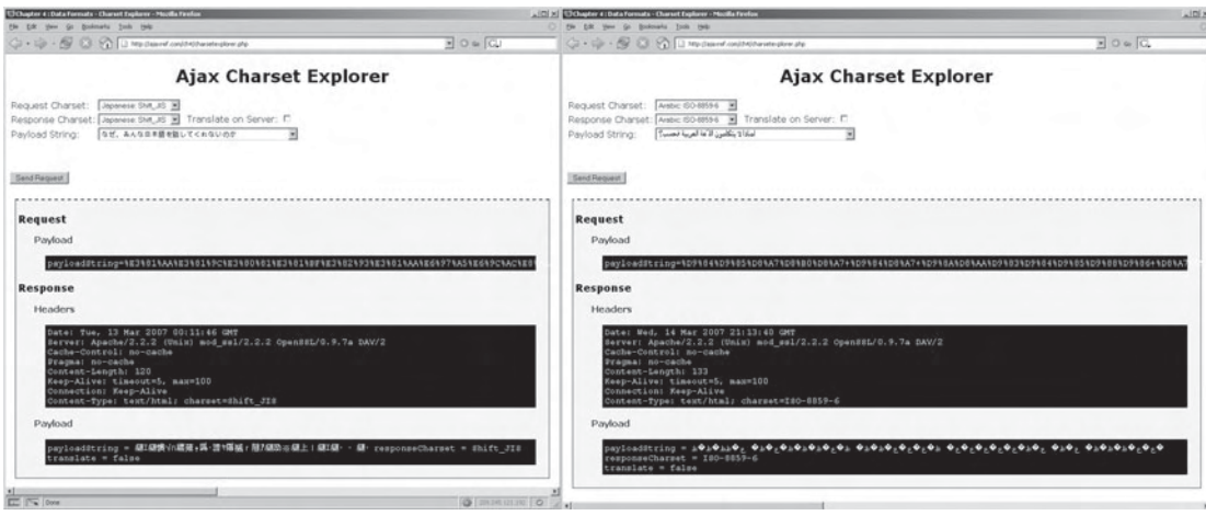
FIGURE 4-1 Example of character set confusion in Ajax
