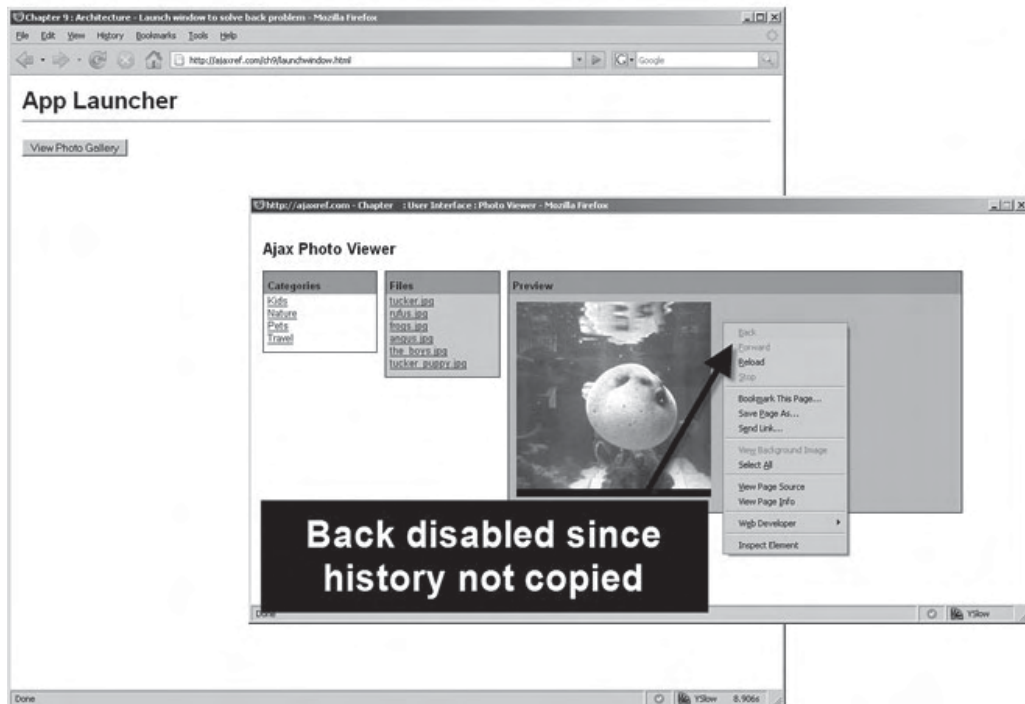
FIGURE 9-9 Window spawning eliminates history problems, but at a cost
