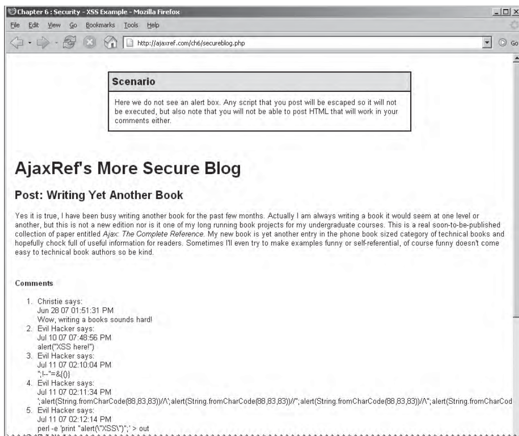
FIGURE 7-10 Escaping output significantly reduces the chance of XSS.
