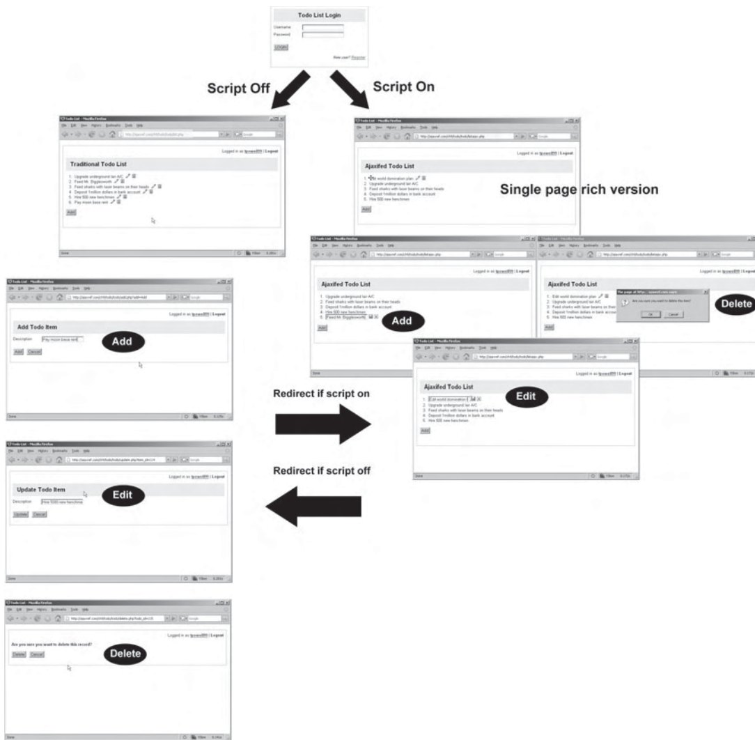
FIGURE 9-15 Ajax and traditional to-do lists side by side
