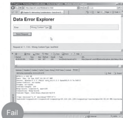
Incorrect Mime - expected XML, but received HTML
