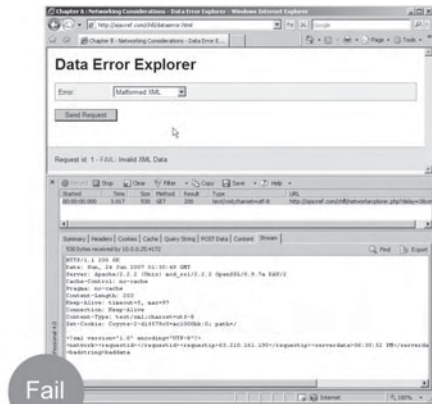
Malformed XML received
