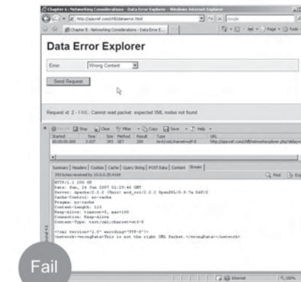
Correct Mime and well formed, but missing expected elements
