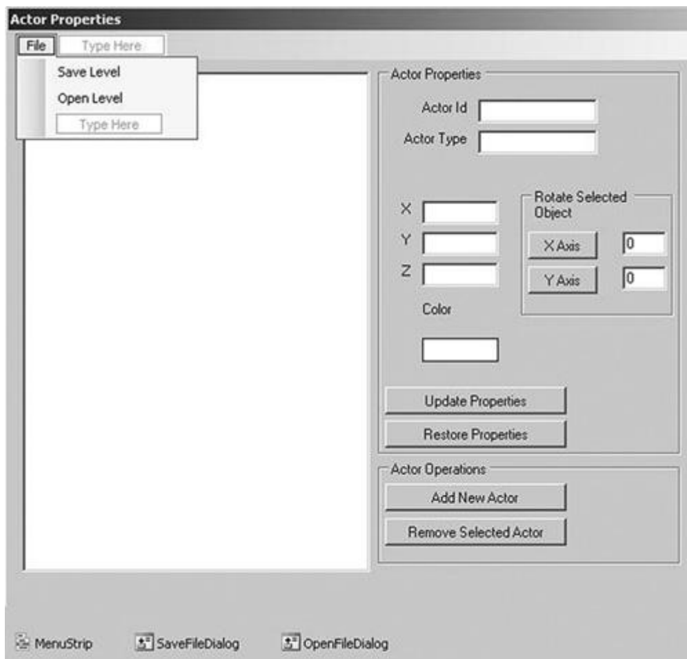
Figure 20.3. The ActorPropertiesForm.
