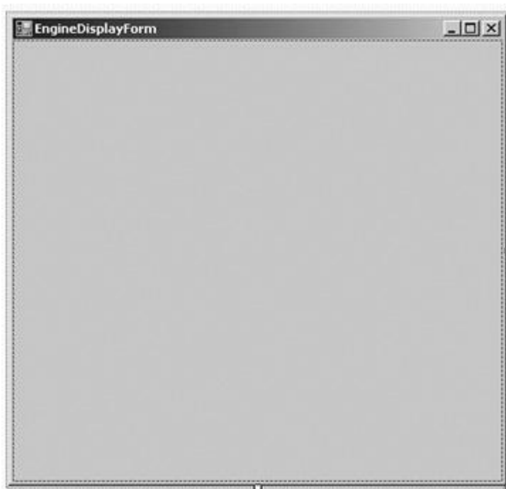
Figure 20.2. EngineDisplayForm.
