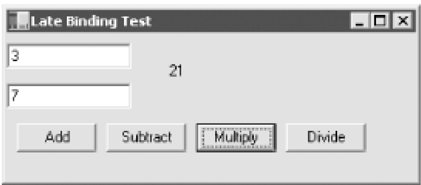
Figure 22-16. Late-binding test
