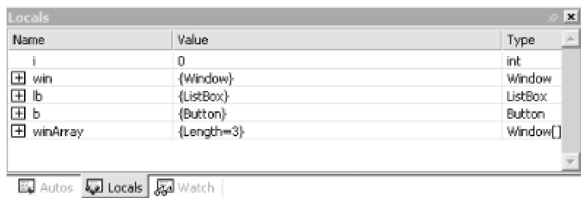
Figure 2-8. Locals window
