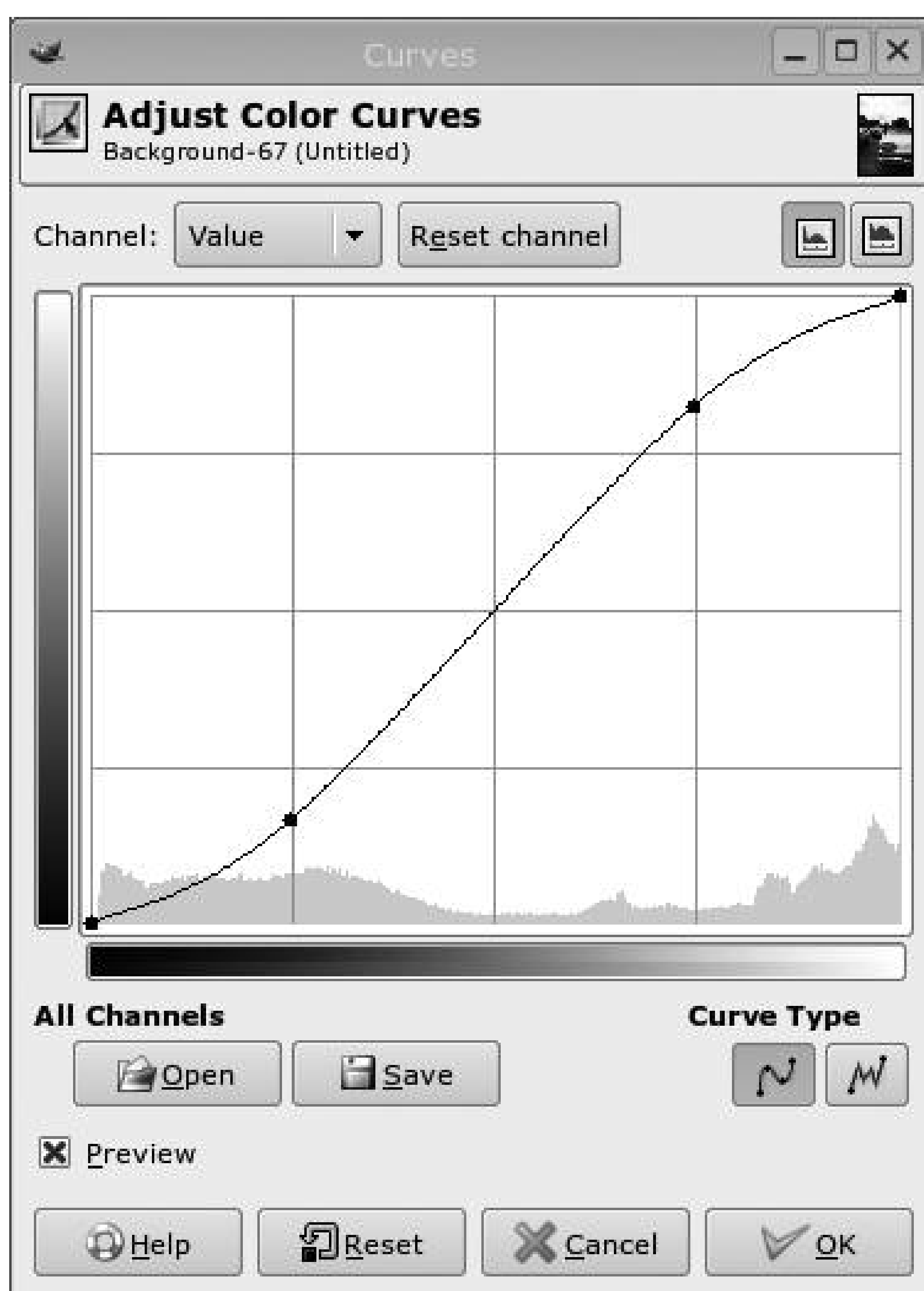
Figure 9-22. Contrast-enhancing curve
