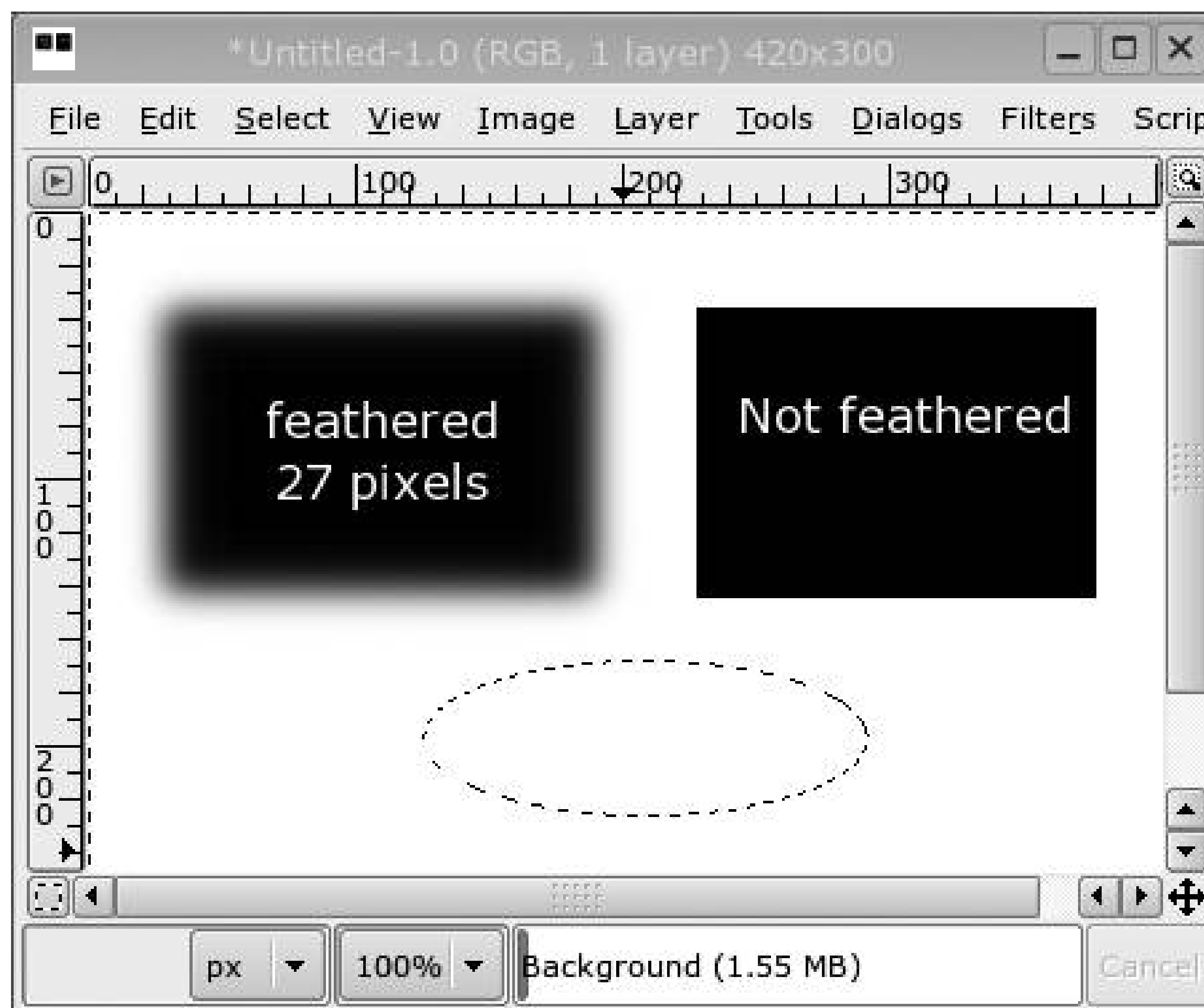
Figure 9-15. GIMP selections
