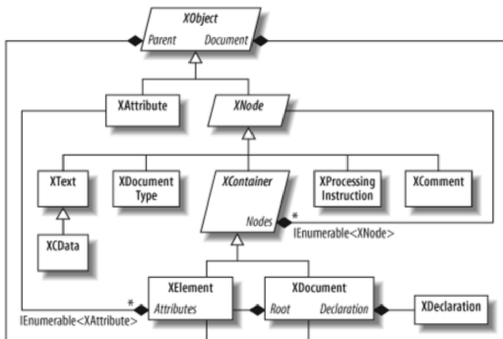
Figure 1-11. Core X-DOM types
