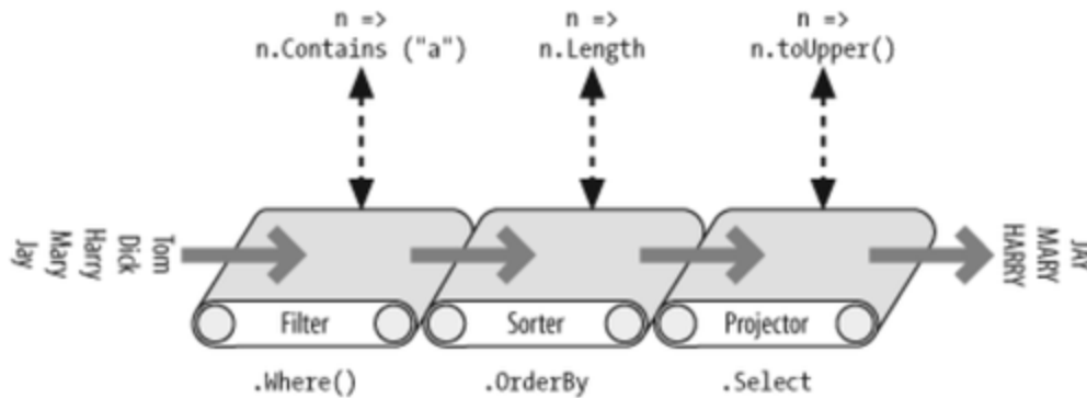
Figure 1-1. Chaining query operators
