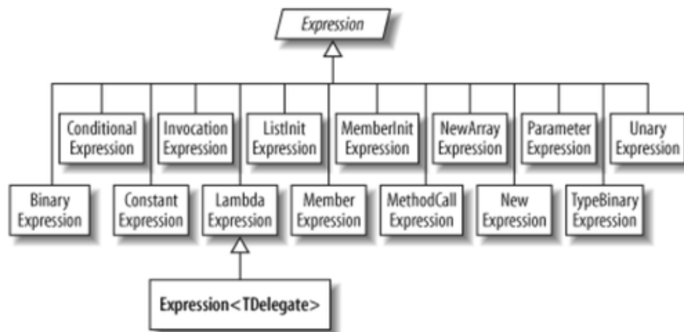
Figure 1-8. Expression types
