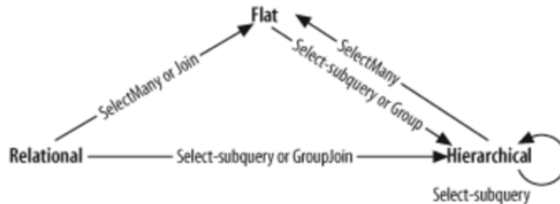
Figure 1-10. Projecting an object hierarchy
