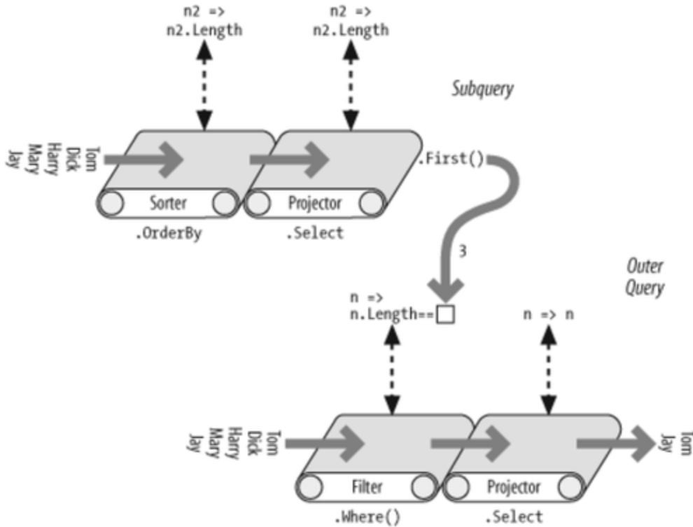
Figure 1-6. Subquery composition
