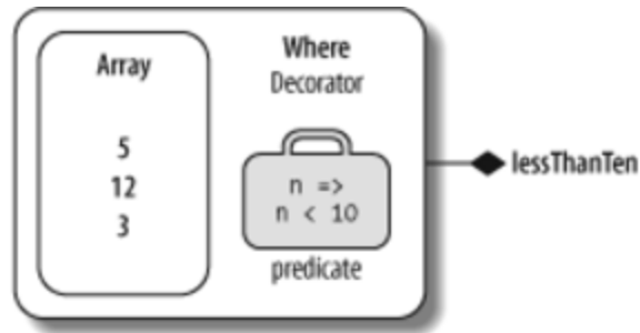
Figure 1-3. Decorator sequence
