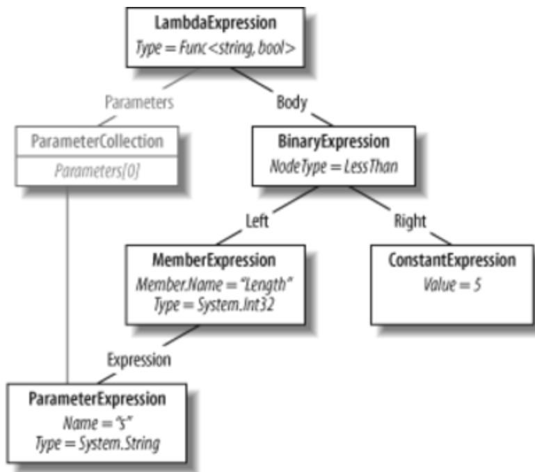
Figure 1-9. Expression tree
