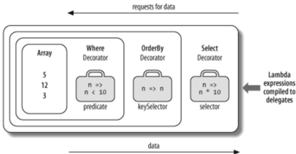
Figure 1-4. Layered decorator sequences
