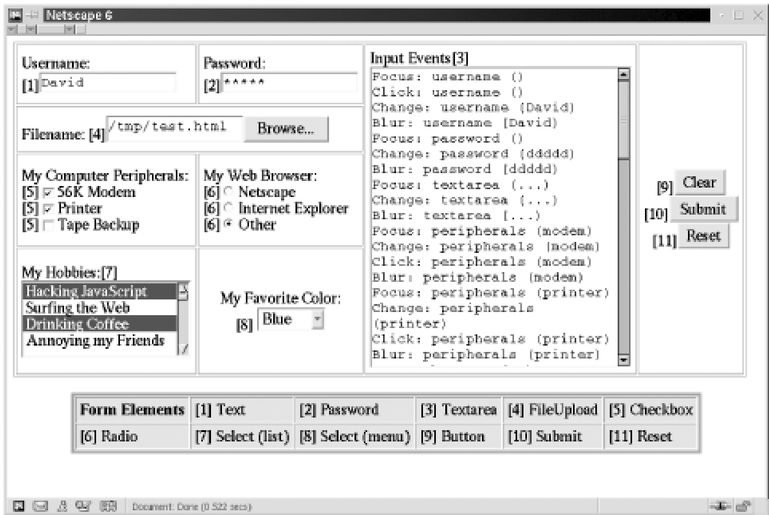
Figure 15-1. HTML form elements
