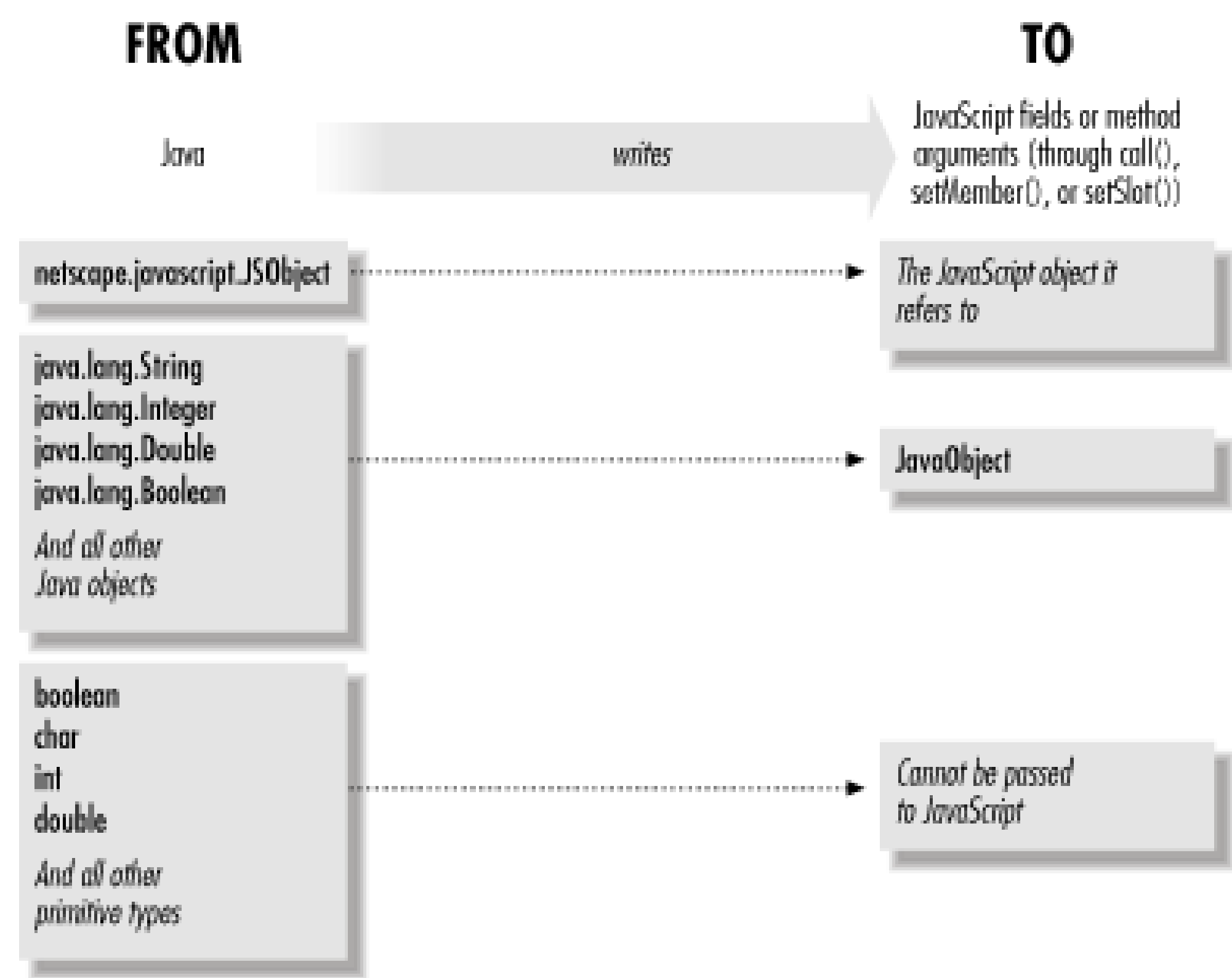
Figure 22-5. Data conversions performed when Java reads JavaScript values
