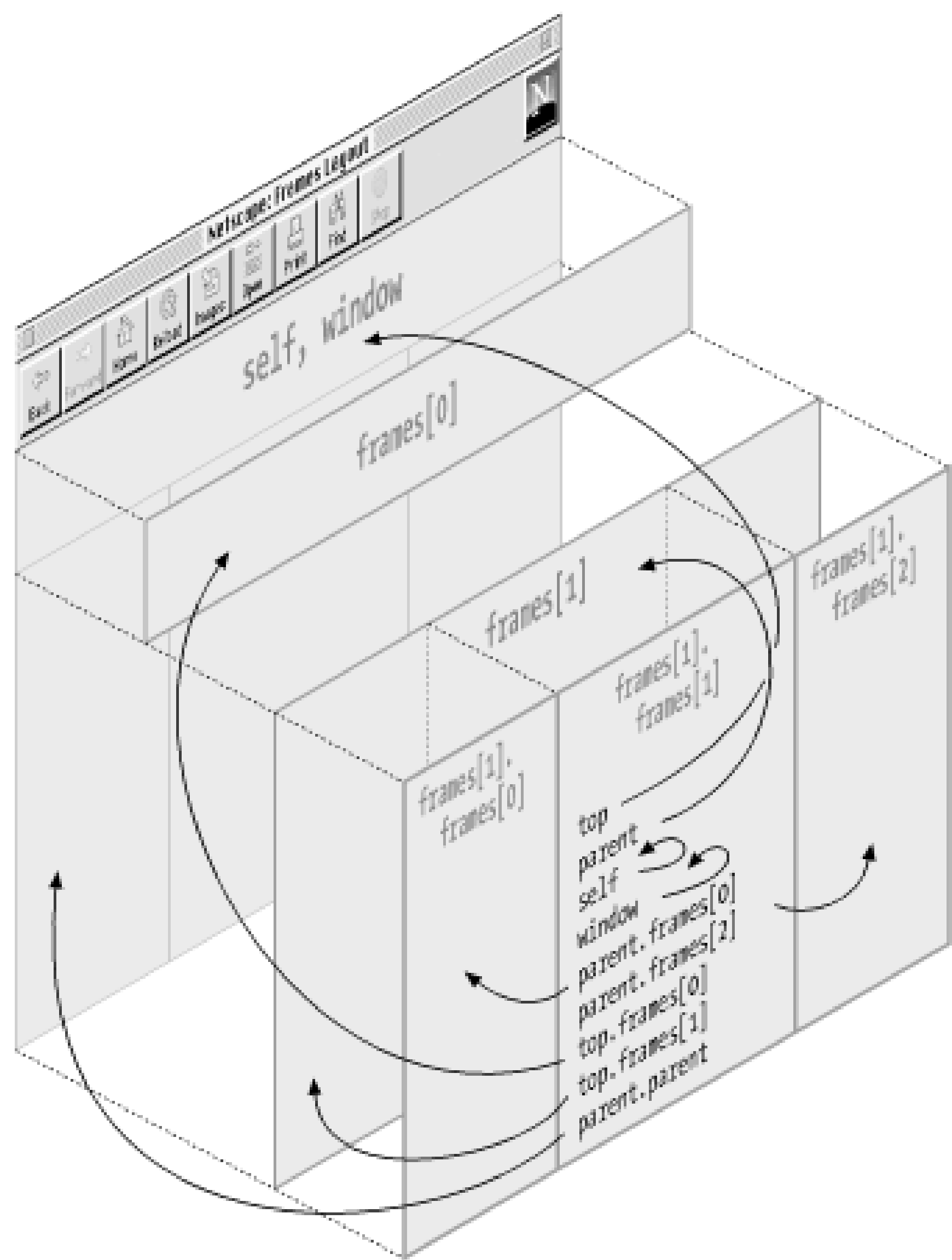
Figure 13-4. Relationships between frames
