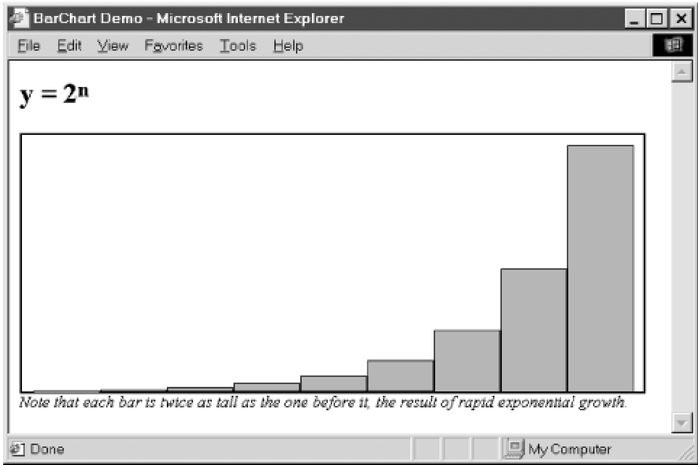
Figure 18-3. A dynamically created bar chart
