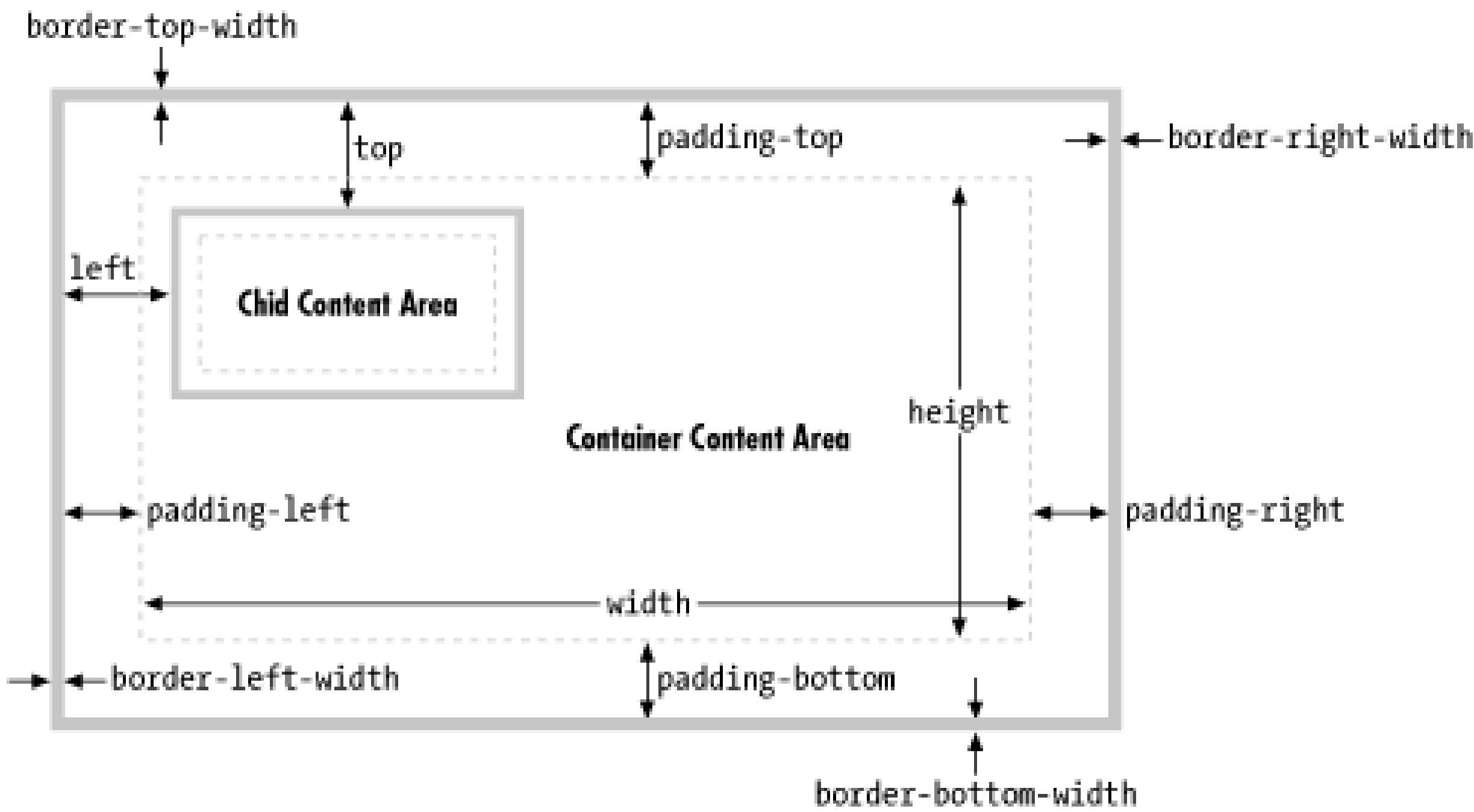
Figure 18-1. Dynamically positioned container and child elements with some CSS attributes
