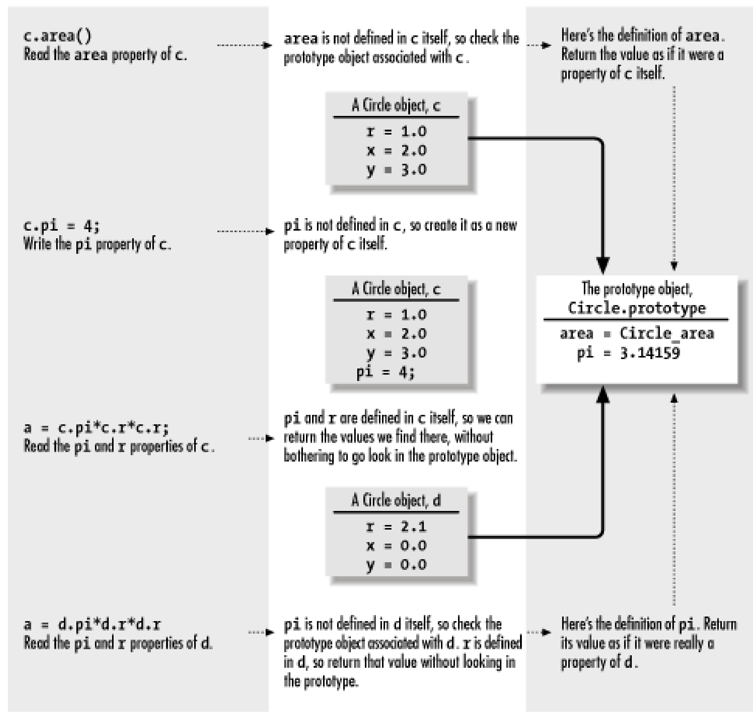
Figure 8-1. Objects and prototypes
