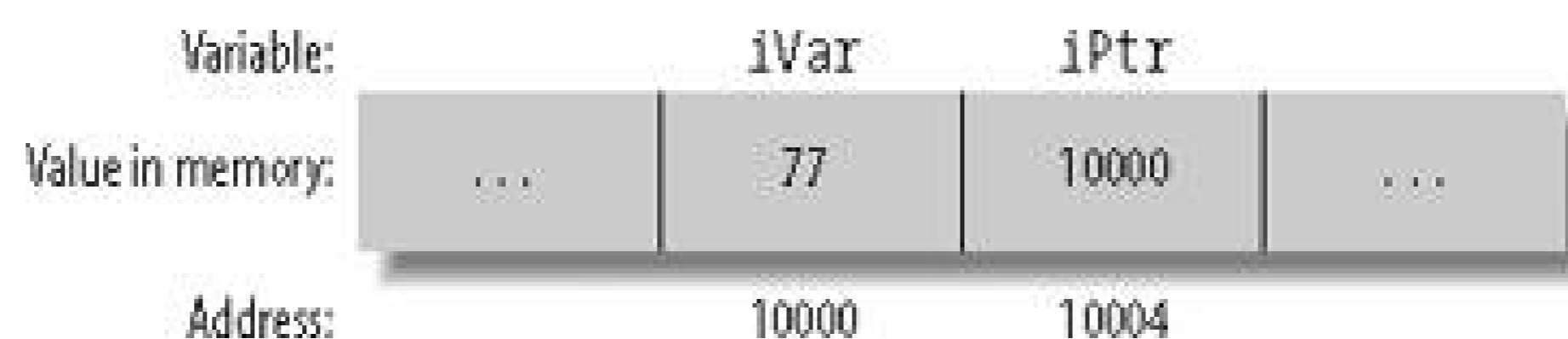
Figure 9-1. A pointer and another object in memory
