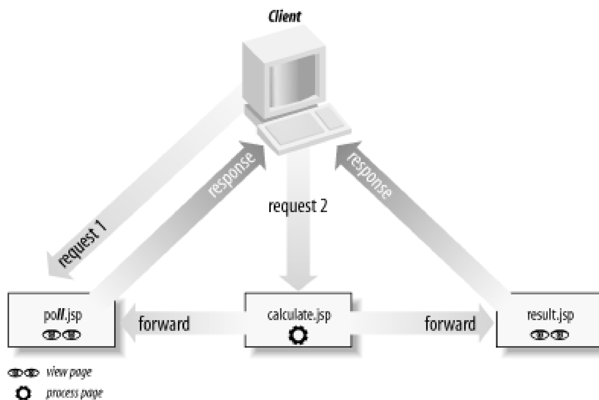
Figure 14-1. Localized poll application pages
