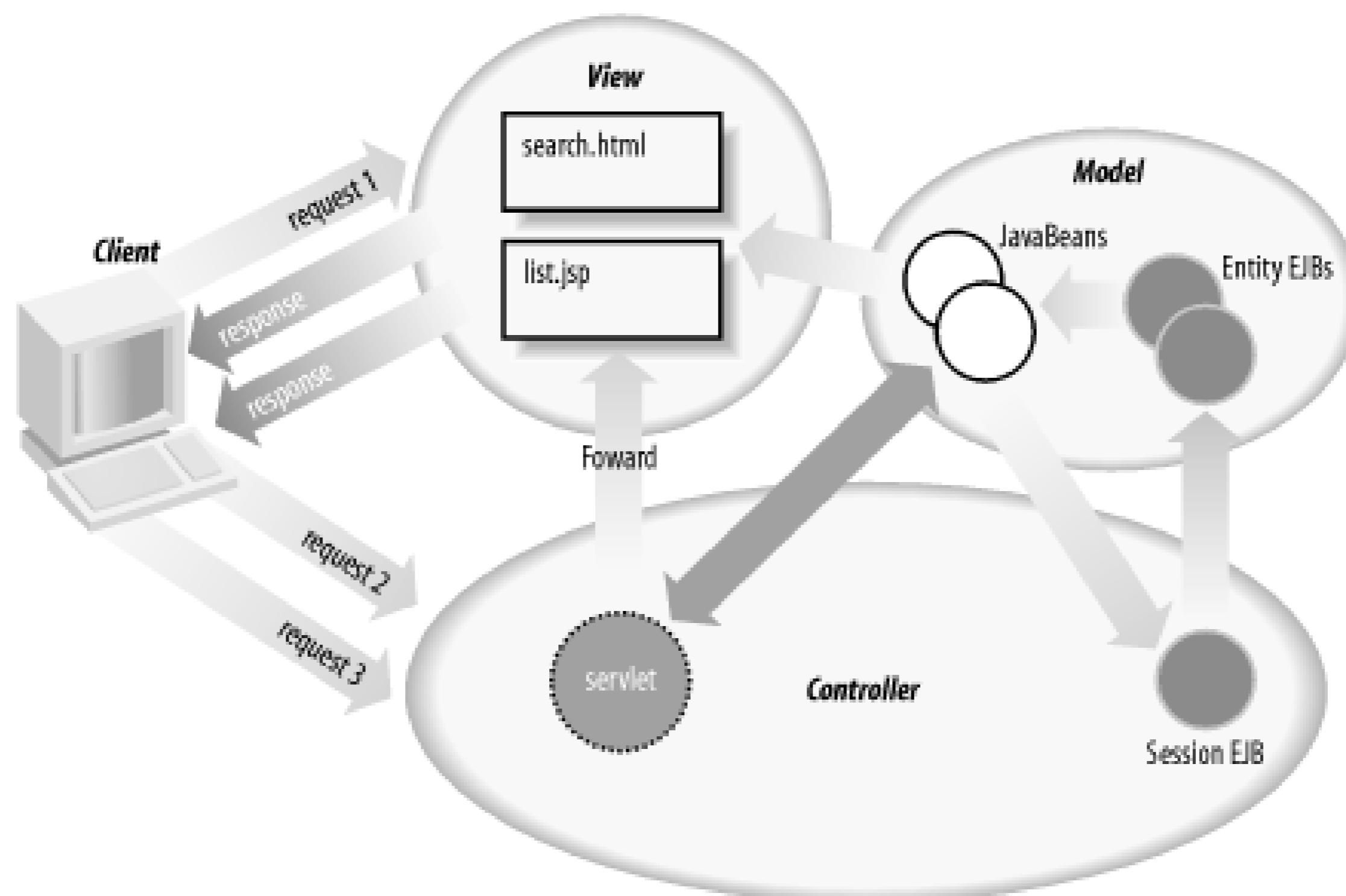
Figure 18-4. MVC roles in a servlet/JSP/EJB scenario
