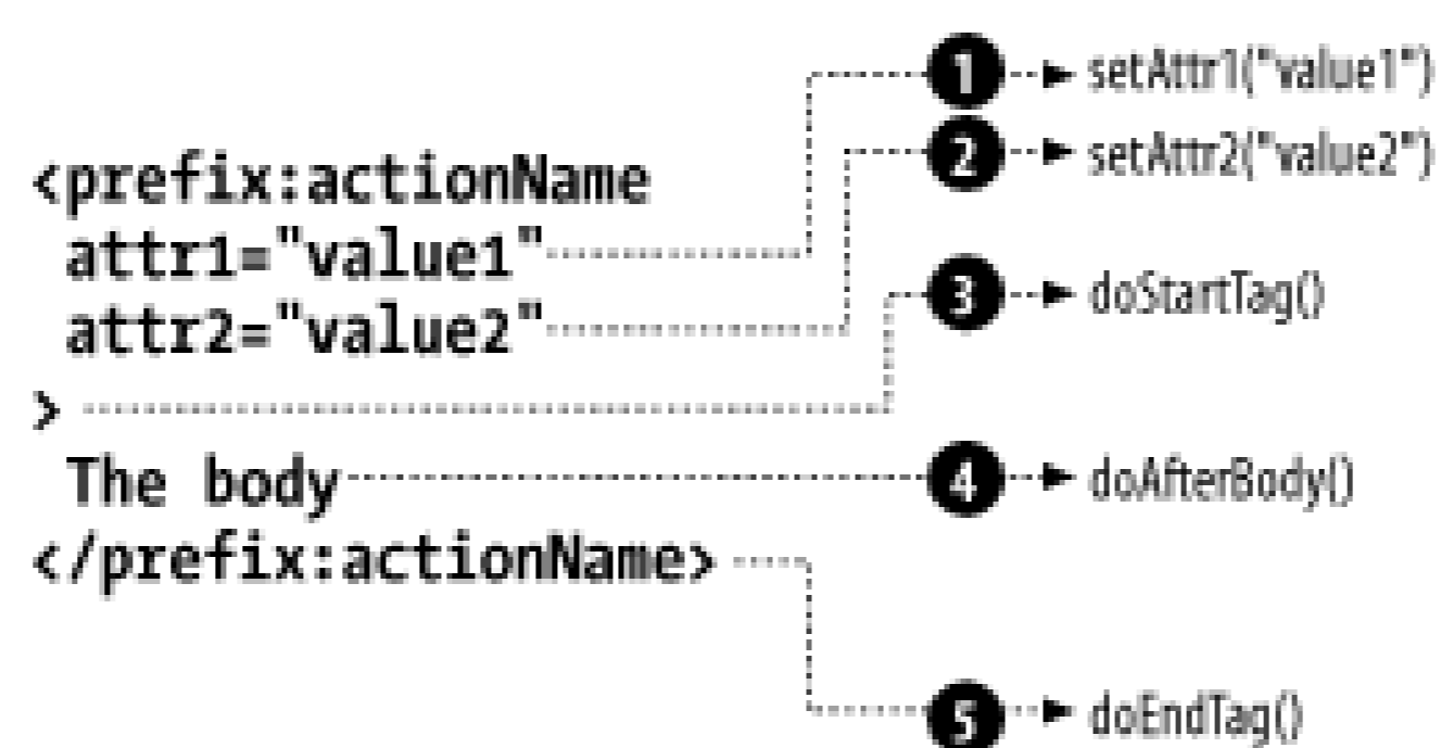
Figure 21-5. IterationTag interface methods
