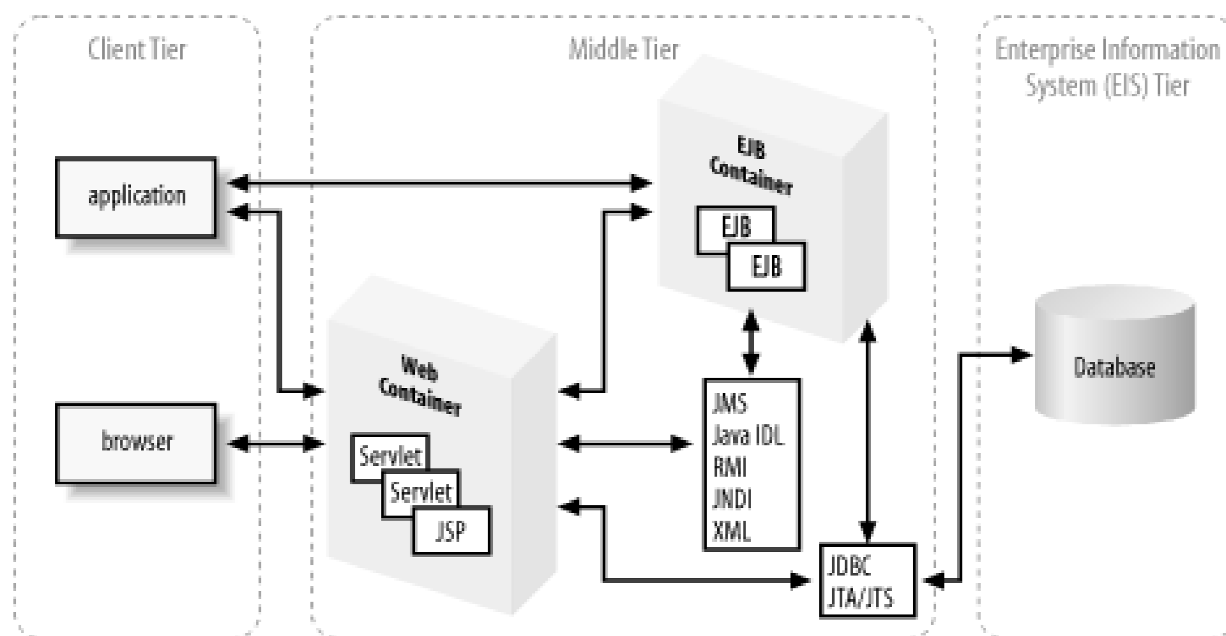
Figure 18-1. EE overview
