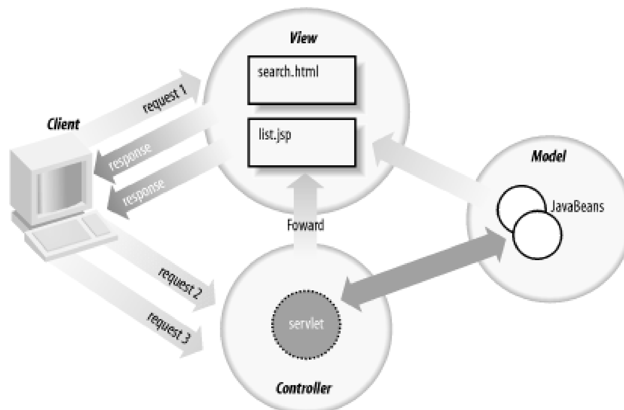
Figure 18-3. MVC roles in a servlet/JSP scenario
