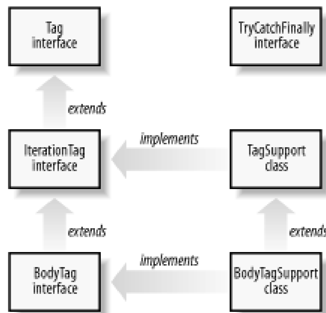
Figure 21-3. The primary classic tag handler interfaces and support classes
