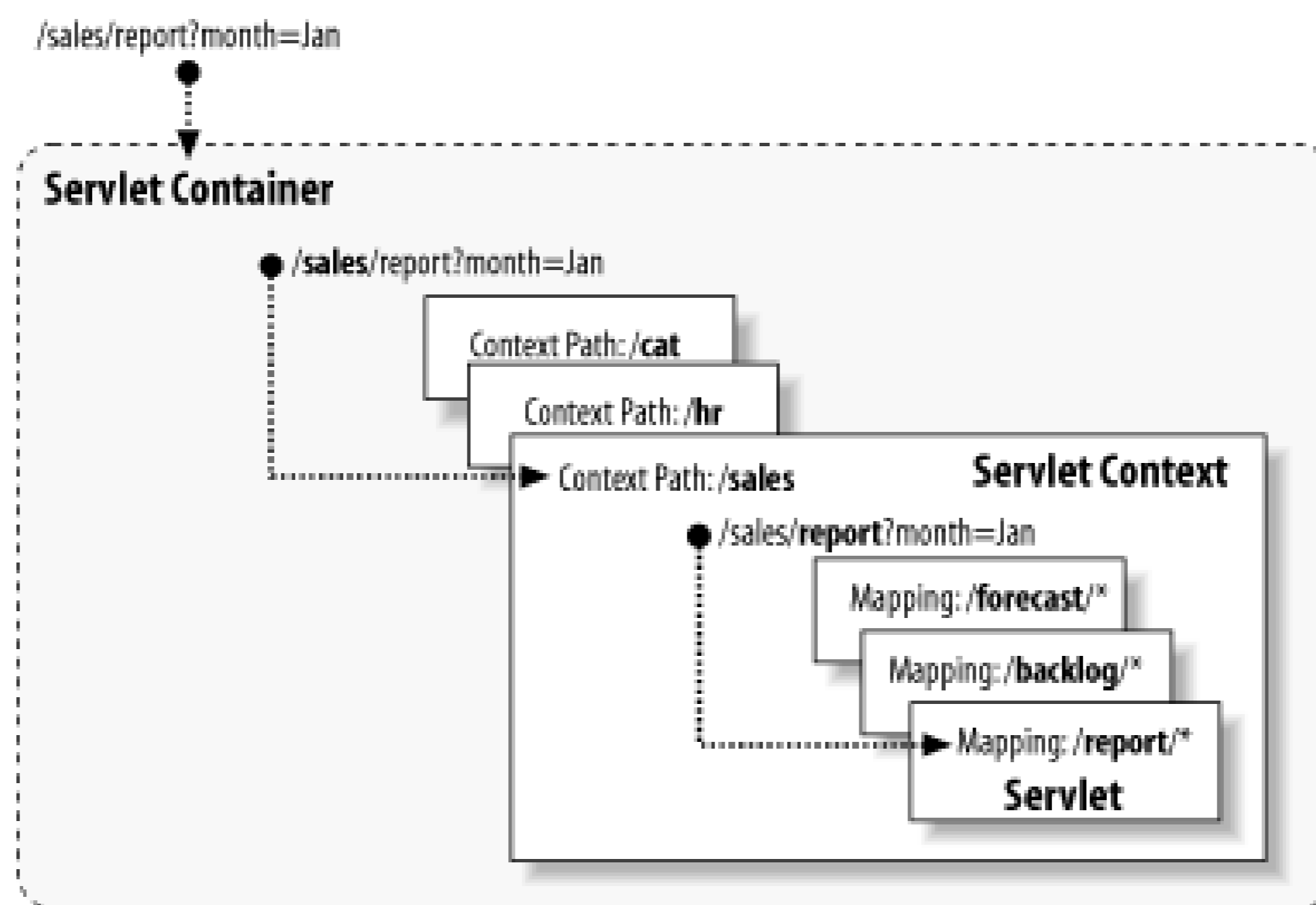
Figure 2-4. Request dispatching
