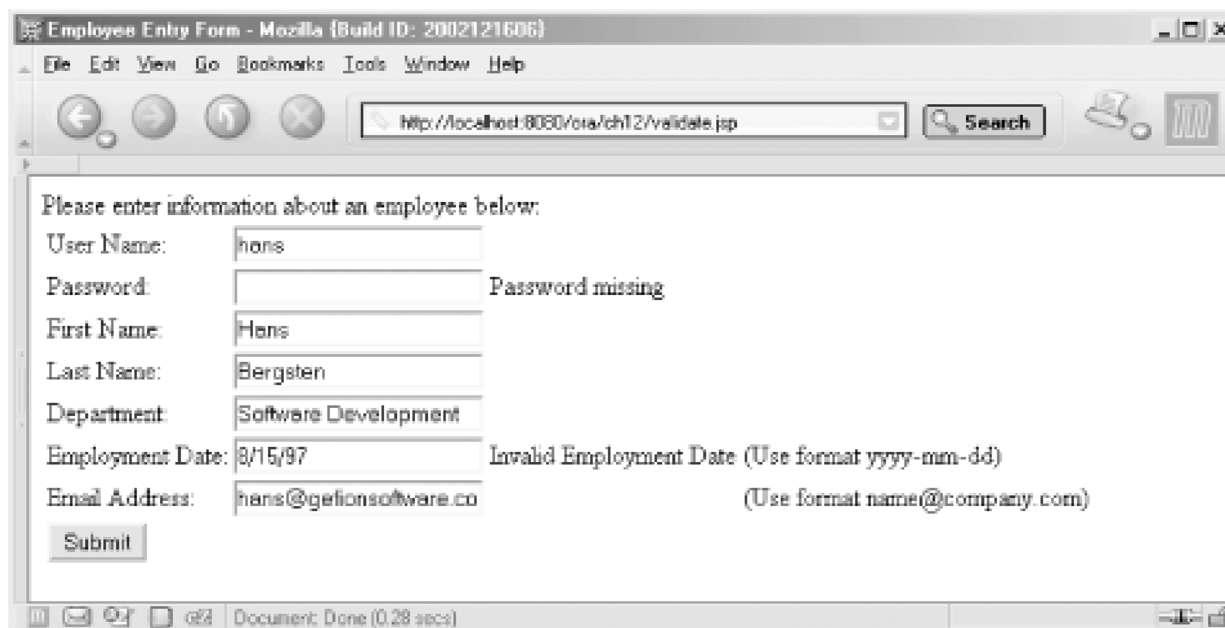
Figure 12-8. The input page with error messages
