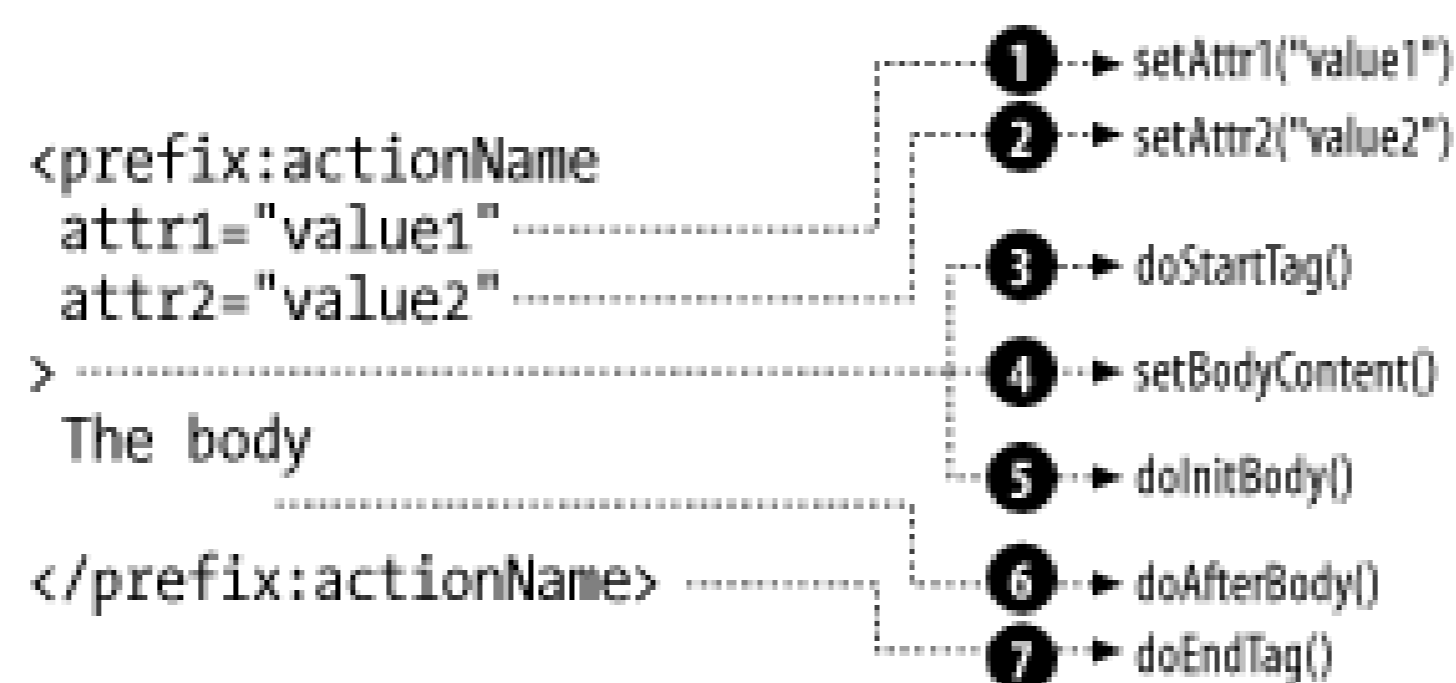
Figure 21-6. BodyTag interface methods
